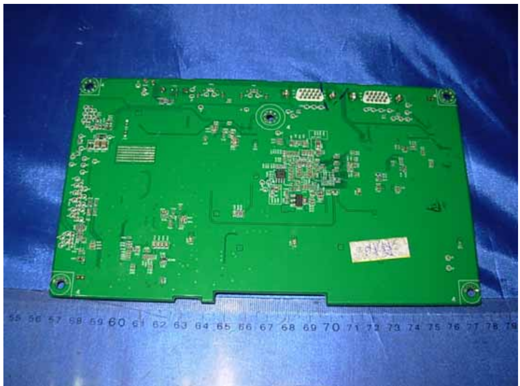
FIGURE 4 LCD MONITOR (M/N: N225WUZ) MAIN BOARD (COMPONENT SIDE)
