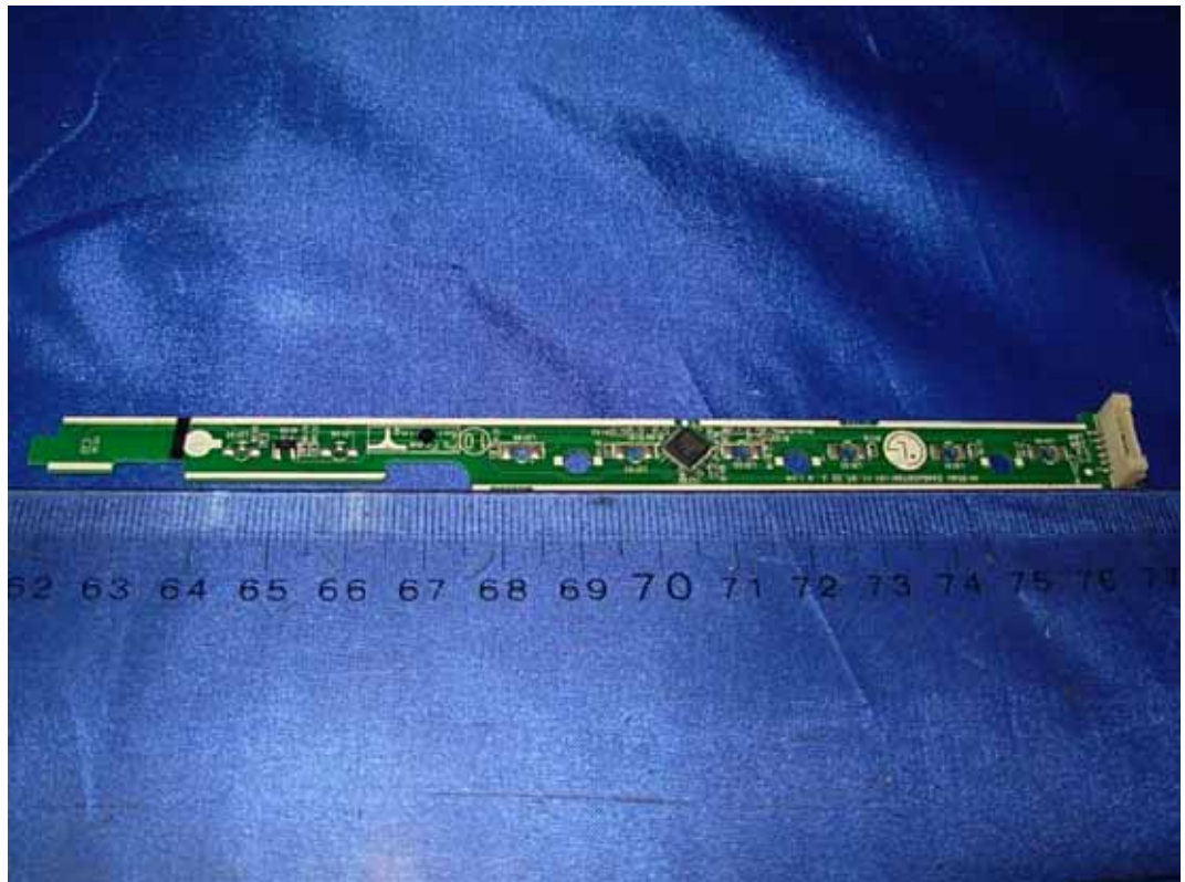
FIGURE 10 LCD MONITOR (M/N: N225WUZ) KEY BOARD (COMPONENT SIDE)
