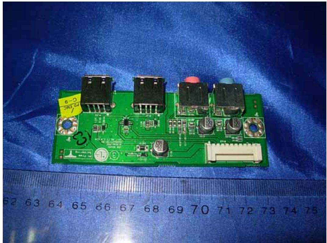
FIGURE 12 LCD MONITOR (M/N: N225WUZ) SIDE BOARD (COMPONENT SIDE)
