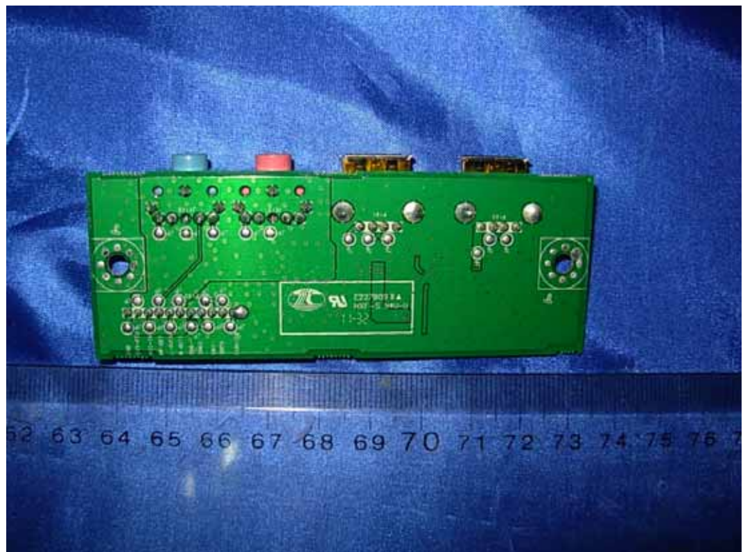
FIGURE 13 LCD MONITOR (M/N: N225WUZ) SIDE BOARD (SOLDERED SIDE)
