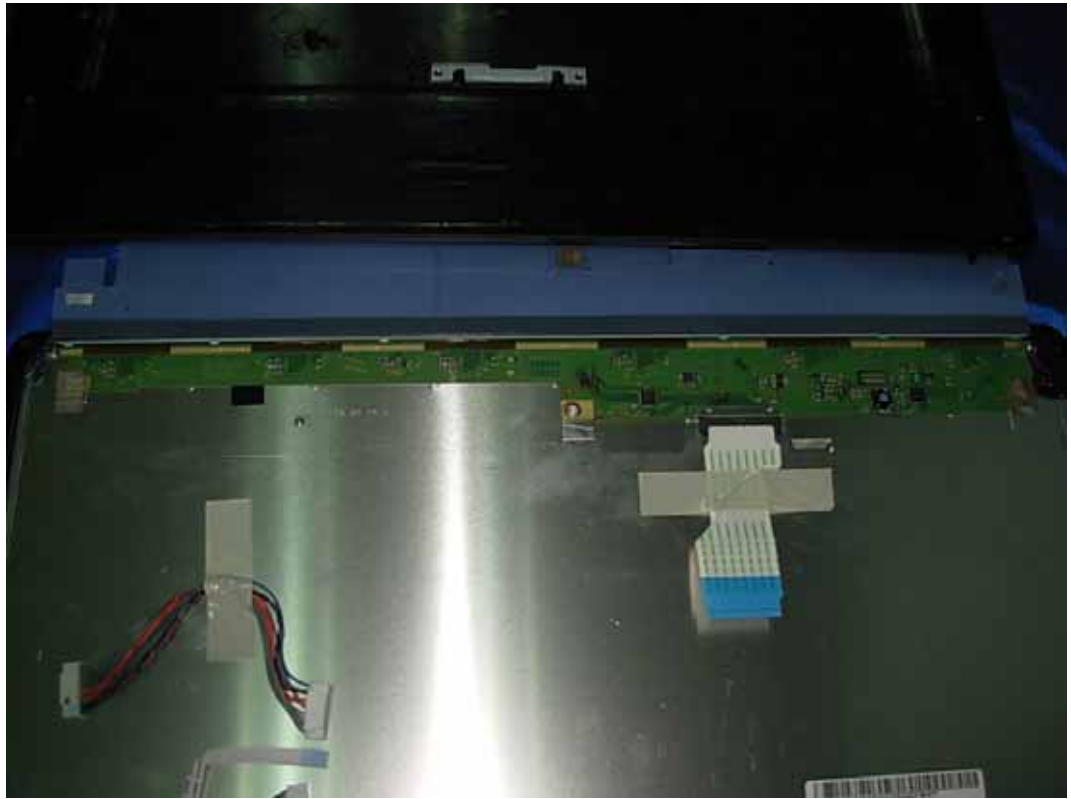
FIGURE 8 LCD MONITOR (M/N: N225WUZ) DISPLAY BOARD (COMPONENT SIDE)
