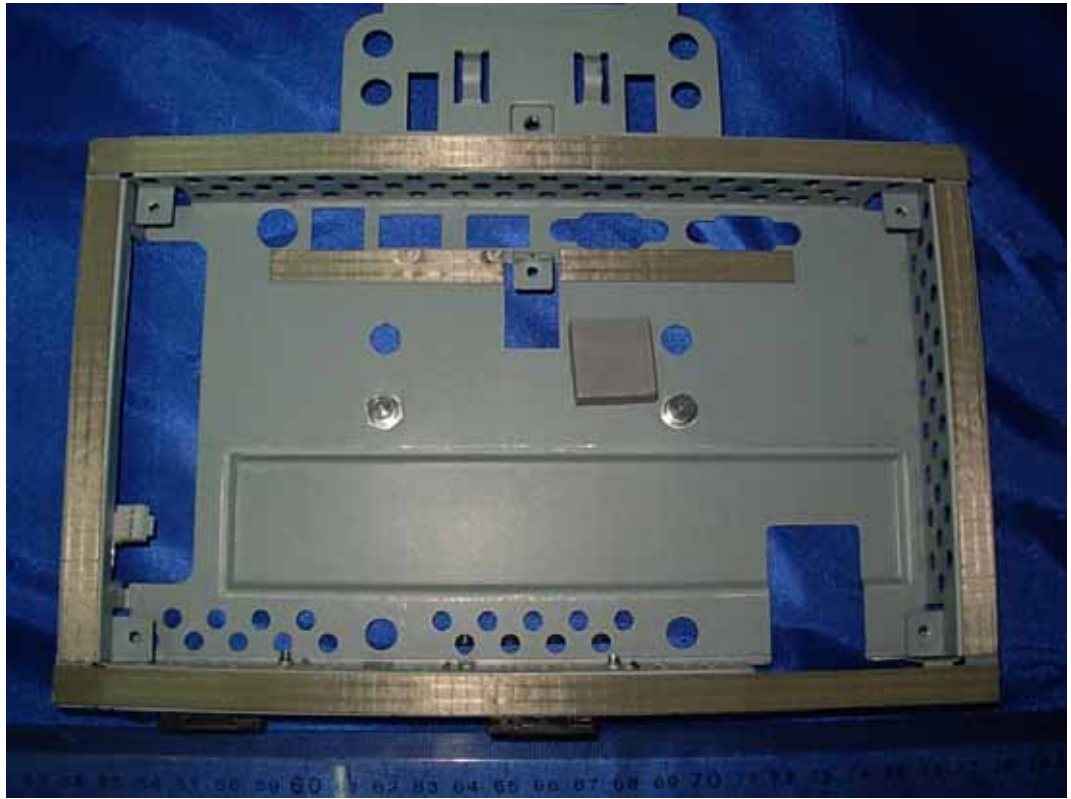
FIGURE 14 LCD MONITOR (M/N: N225WUZ) DEBUG #1
