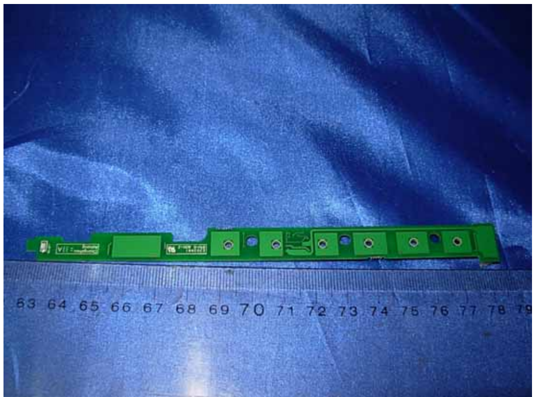
FIGURE 11 LCD MONITOR (M/N: N225WUZ) KEY BOARD (SOLDERED SIDE)
