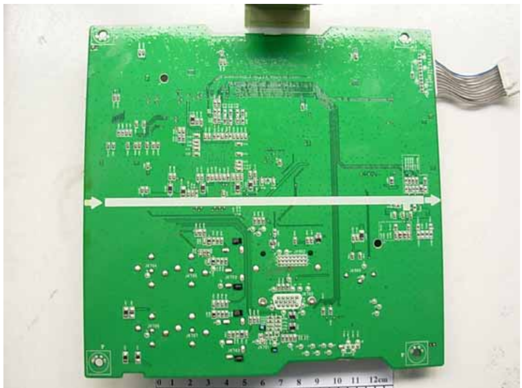
FIGURE 3 LCD MONITOR (M/N: LSM1850HU) MAIN BOARD (SOLDERED SIDE)
