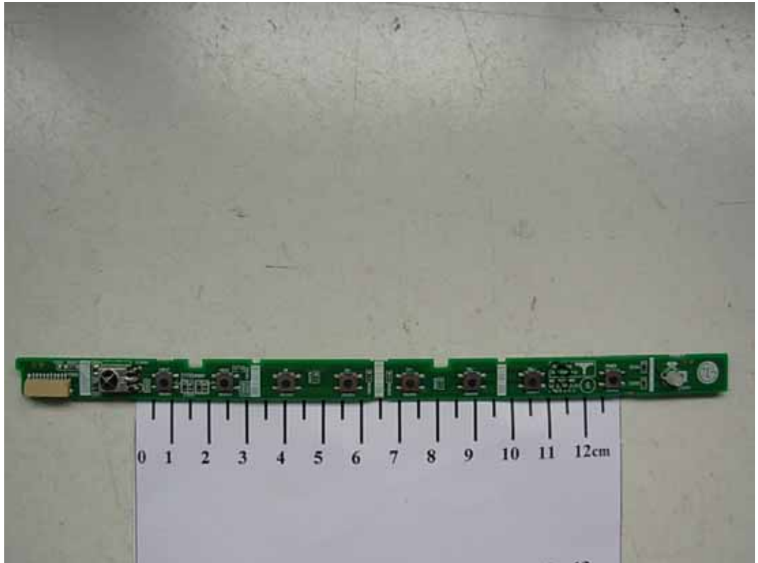
FIGURE 6 LCD MONITOR (M/N: LSM1850HU) KEY BOARD (COMPONENT SIDE)
