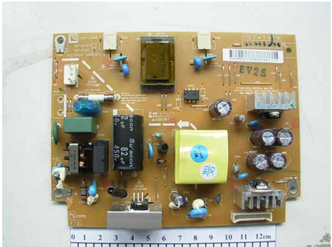
FIGURE 8 LCD MONITOR (M/N: LSM1850HU) POWER BOARD (COMPONENT SIDE)
