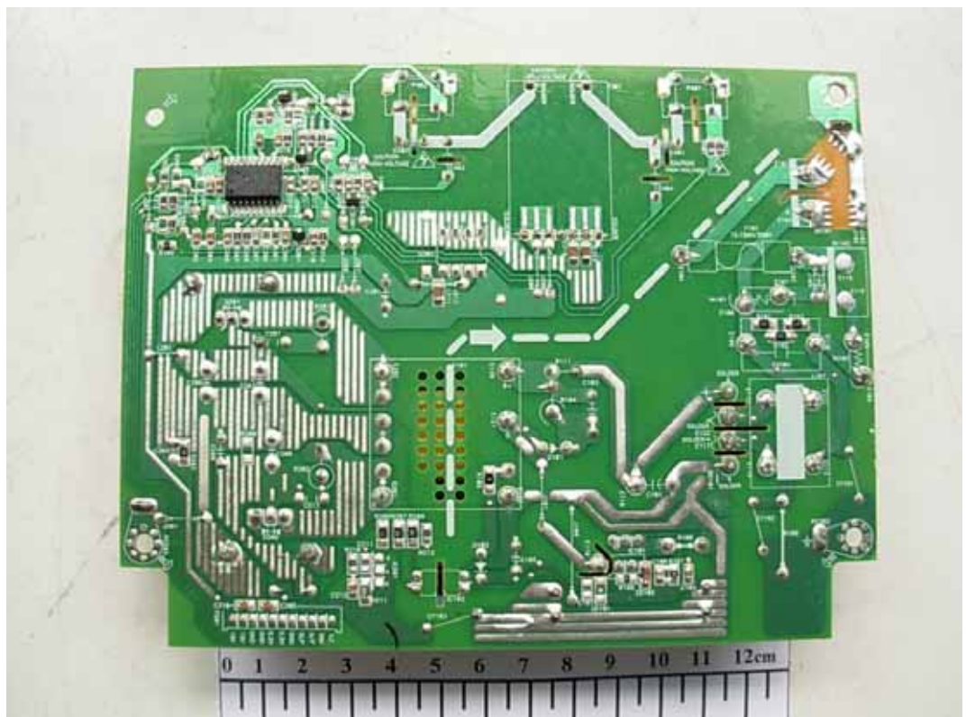
FIGURE 9 LCD MONITOR (M/N: LSM1850HU) POWER BOARD (SOLDERED SIDE)
