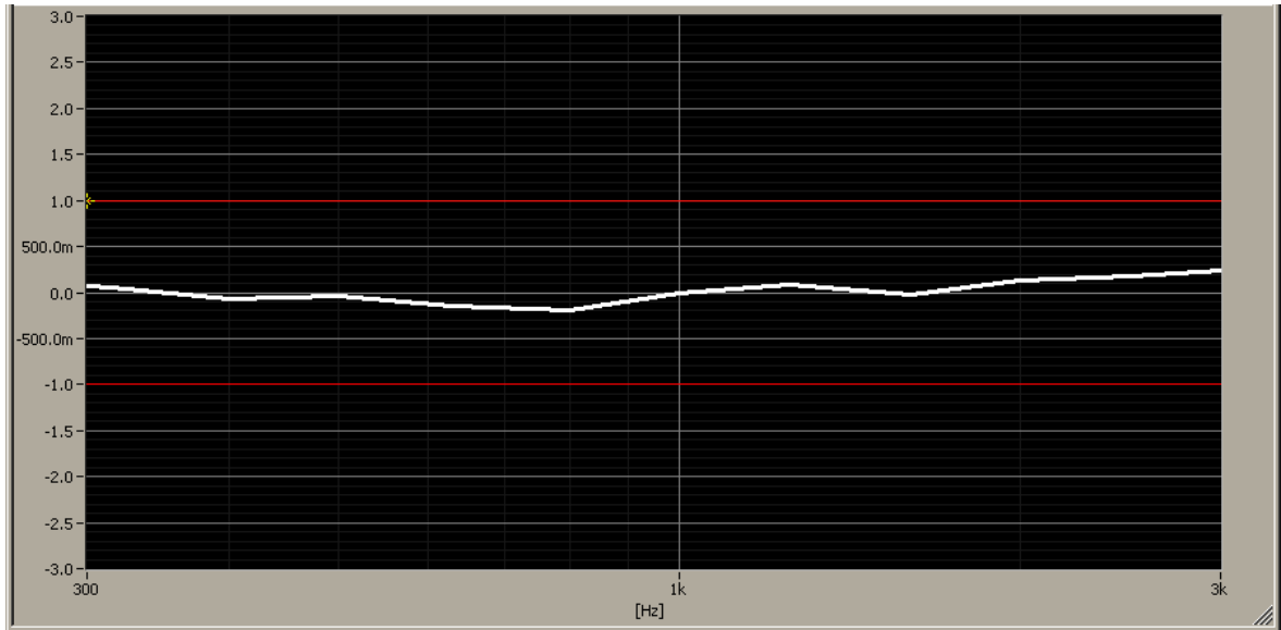
Figure 6-2 Helmholtz Coil Validation for Frequency Response
