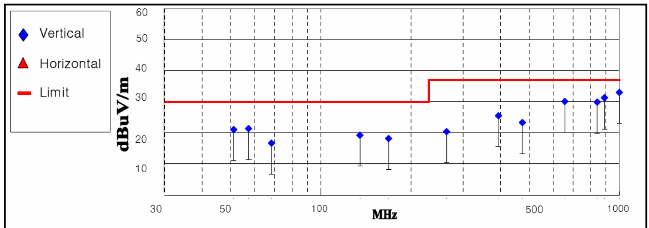
< Fig 6. Radiated emission result _ Digital (30MHz ~ 1000MHz)>
