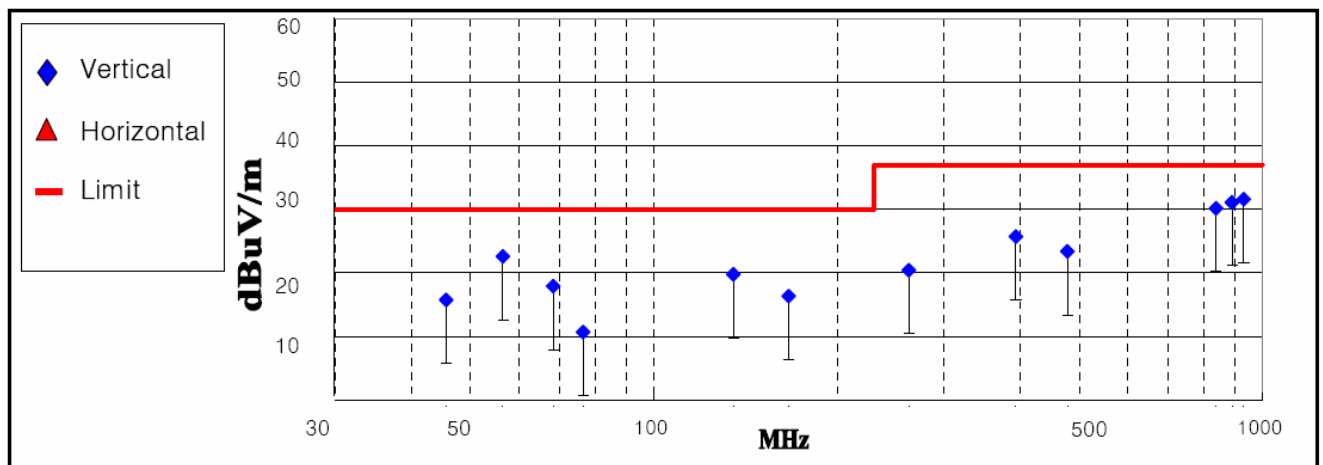
< Fig 4. Radiated emission result _ Analog (30MHz ~ 1000MHz)>
