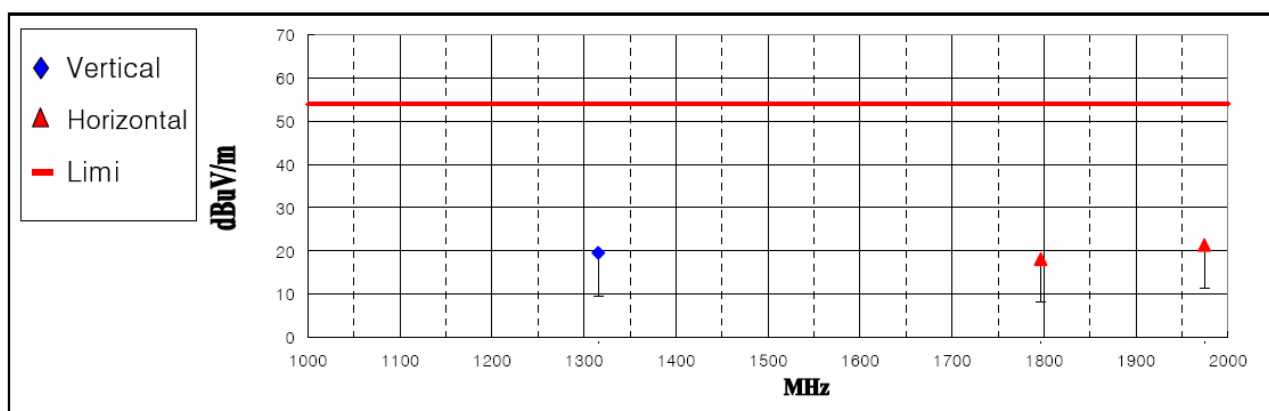
< Fig 5. Radiated Emission result _ Analog (1000MHz ~ 2000MHz) >
