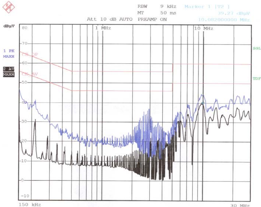
< Neutral line >
