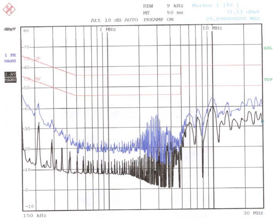
< Neutral line >
