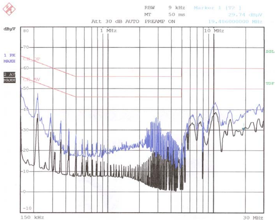
< Hot line >
