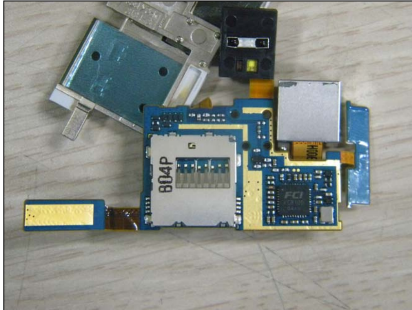
Top view of Camera module
