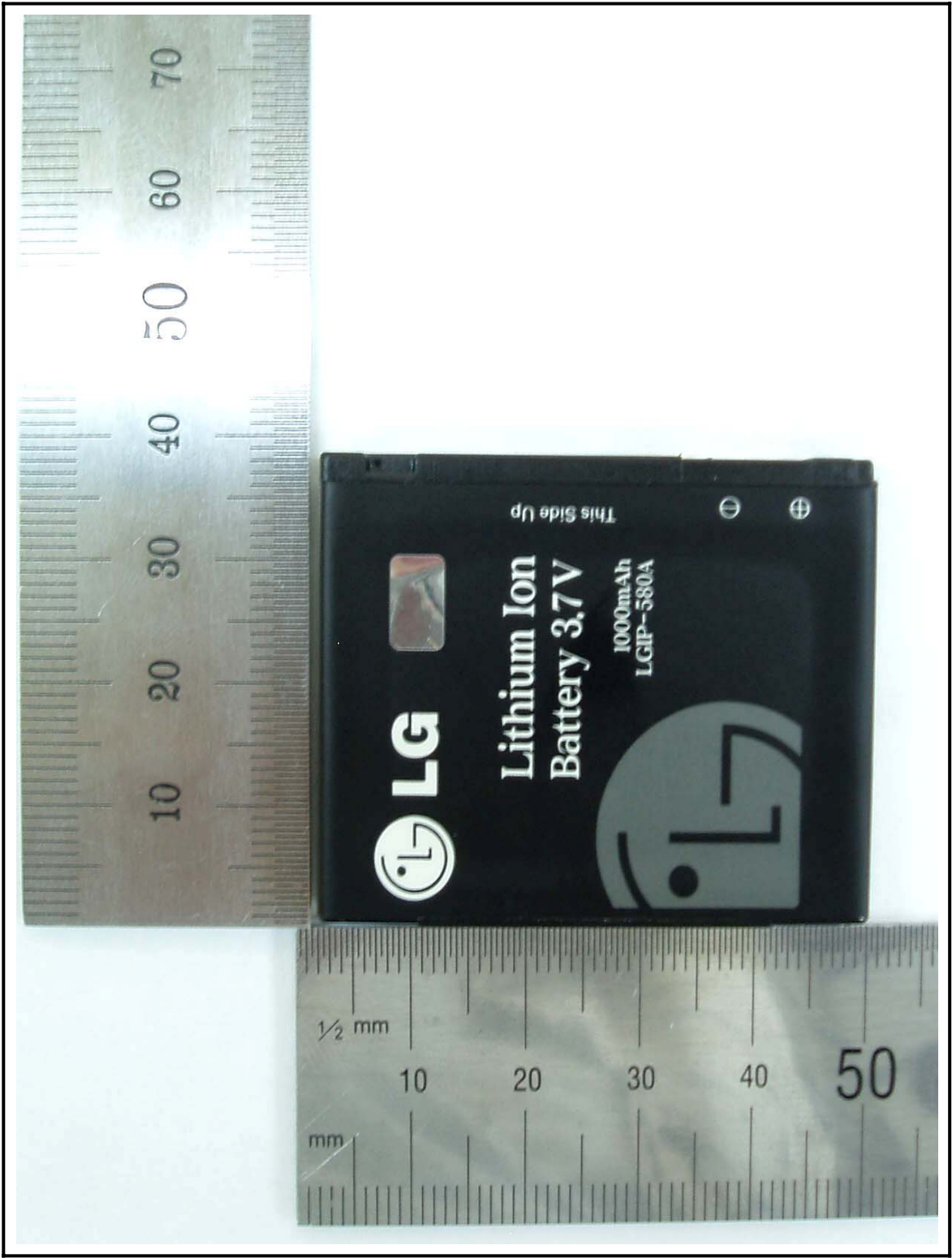
Figure 19 DUT Photo
