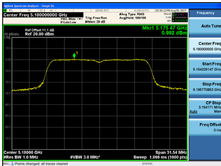
802.11ac_VHT20 UNII 1 BAND PSD CH 36
