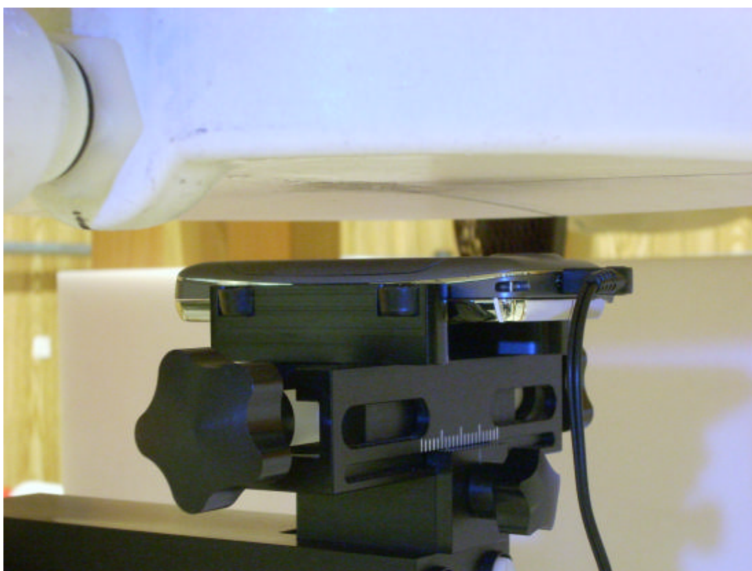
Figure 8: Body SAR, Back Side with 20mm Space
