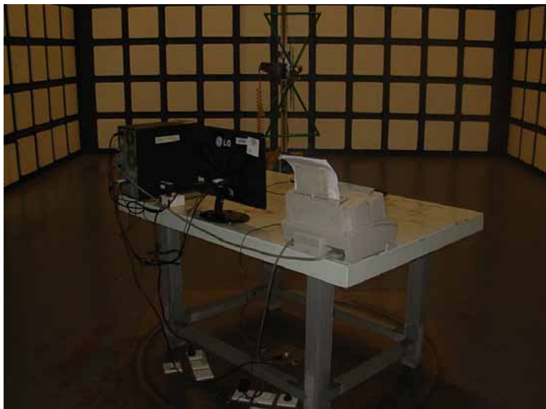
SETUP WITH MAXIMUM DETECTED EMISSION AT VERTICAL POLARIZATION (TEST MODE: DVI 1600*900@60Hz) (ADAPTER: DSA-36W-12 1 24)
