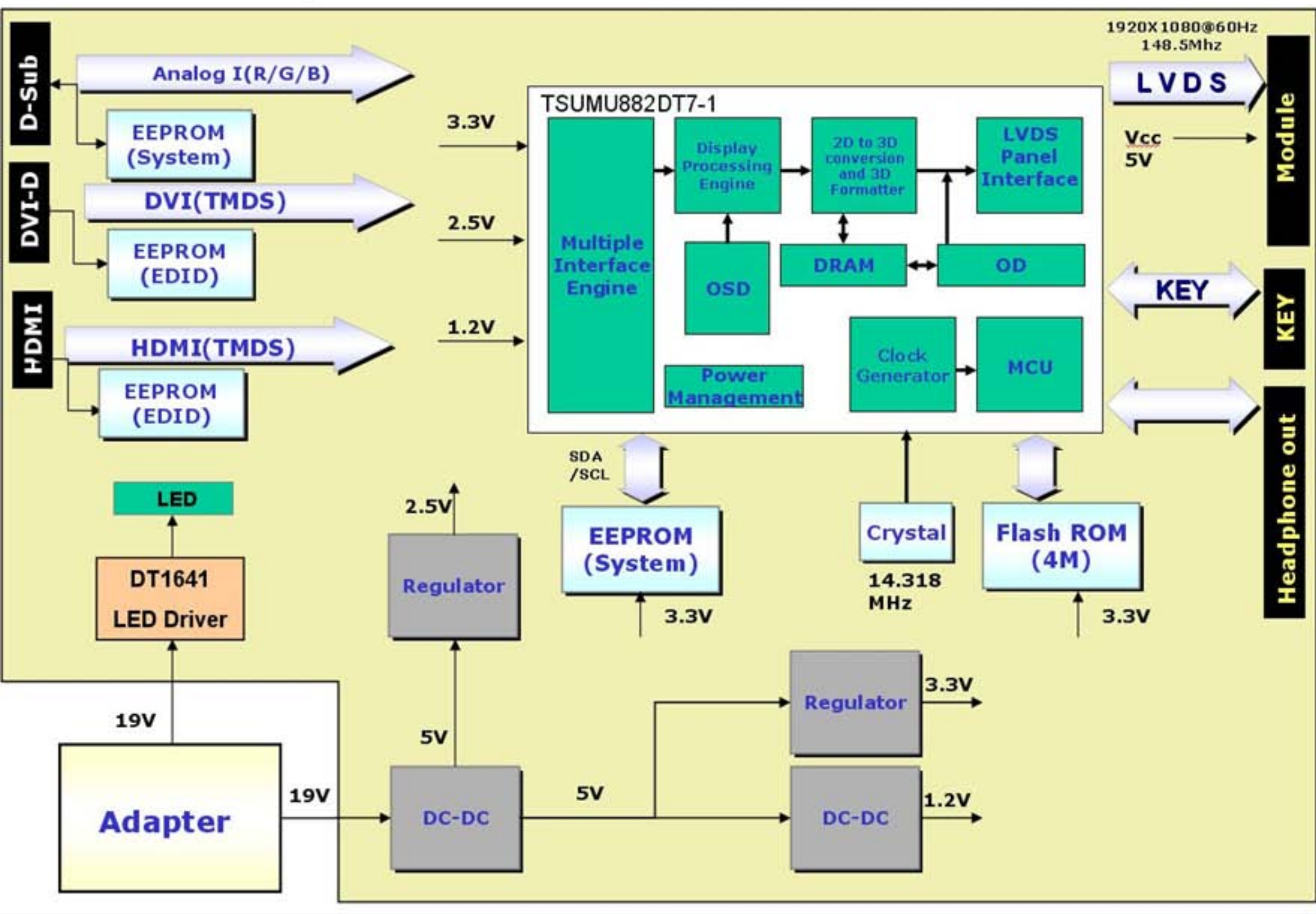
D43P - Block diagram
