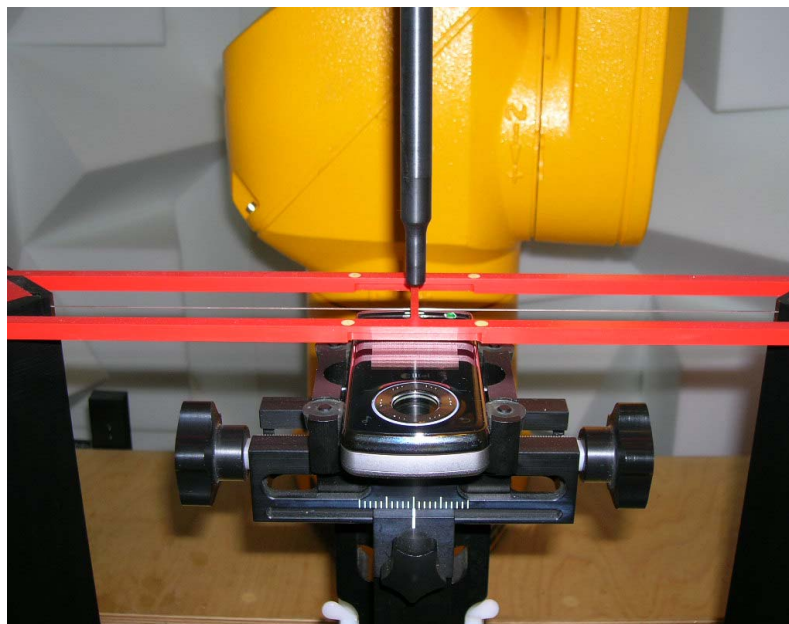
Figure 17-2 HAC Phantom Plane Alignment
