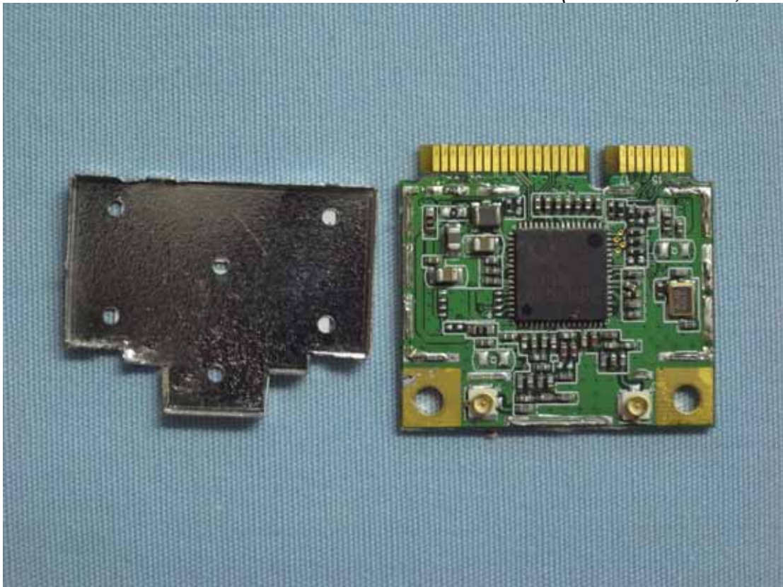
Figure 18 Internal View (Wireless Module, Front View)
