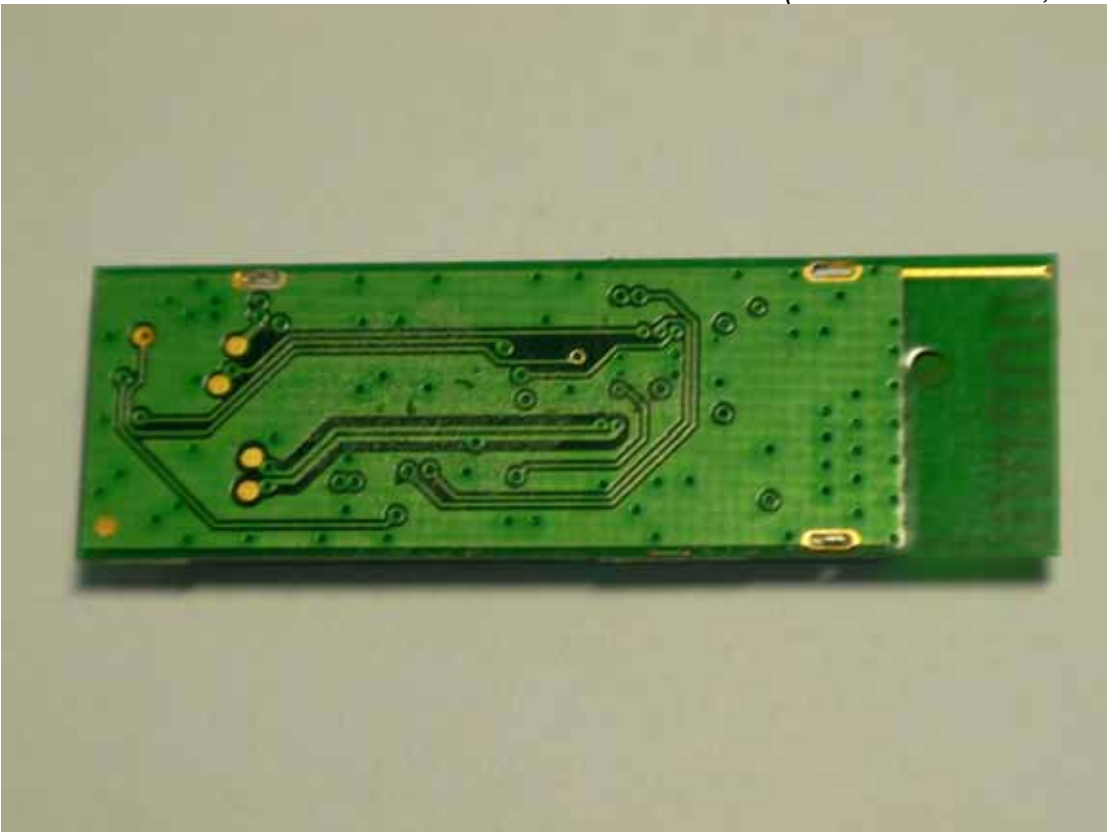
Figure 24 Internal View (Bluetooth Module, Back View)
