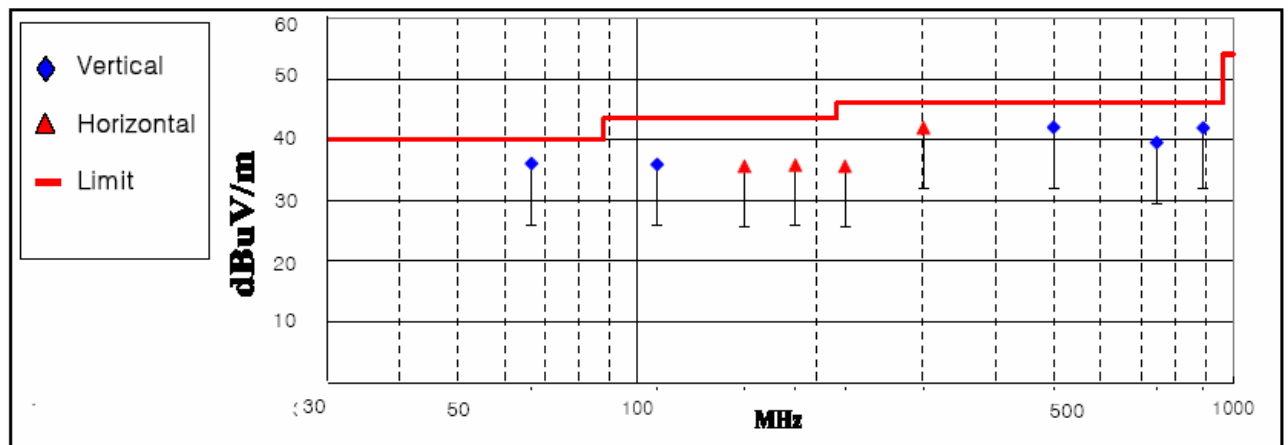
< Fig 4. Radiated emission result (30MHz ~ 1000MHz)>
