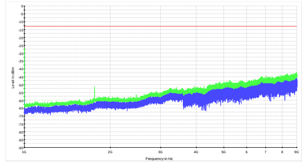
Figure 8.7-2: 1GHz to 9 GHz Radiated
