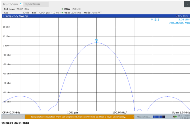
Figure 8.4-4: AGC+3 dB 940.5 MHz input power
