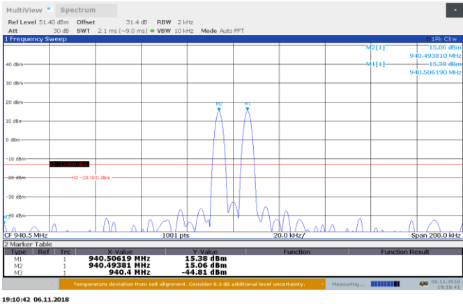
Figure 8.5-2: 940.49375 and 940.50625 MHz AGC + 3dB Out-of-block
