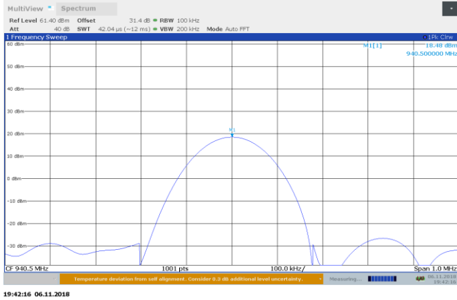
Figure 8.4-2: AGC+3 dB 940.5 MHz output power
