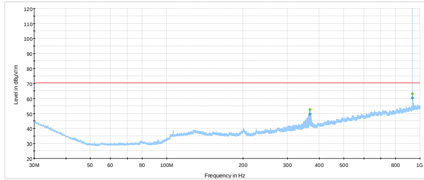
Figure 8.7-1: 30 MHz to 1 GHz Radiated
