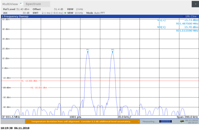
Figure 8.5-1: 931.4875 and 931.5125 MHz AGC + 0.5 Out-of-block
