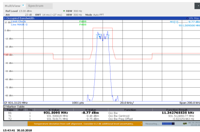
Figure 8.3-3: 11K2F1D AGC +3 dB 931.5125 MHz input 99% BW Emission Mask G
