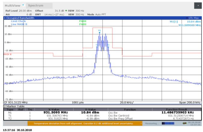
Figure 8.3-8: 11Kof3E AGC +3 dB 931.5125 MHz output 99% BW Emission Mask B
