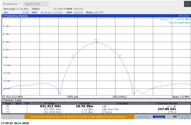
Figure 8.4-1: AGC-0.5 dB 931.5125 MHz output power
