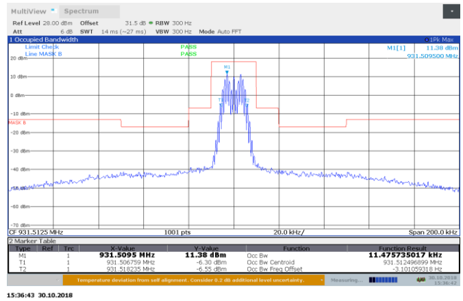
Figure 8.3-6: 11Kof3E AGC-0.5 dB 931.5125 MHz output 99% BW Emission Mask B
