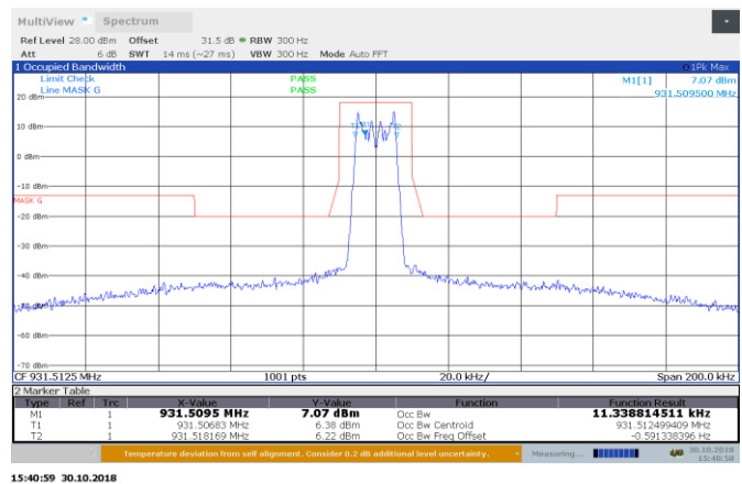
Figure 8.3-4: 11K2F1D AGC +3 dB 931.5125 MHz output 99% BW Emission Mask G
