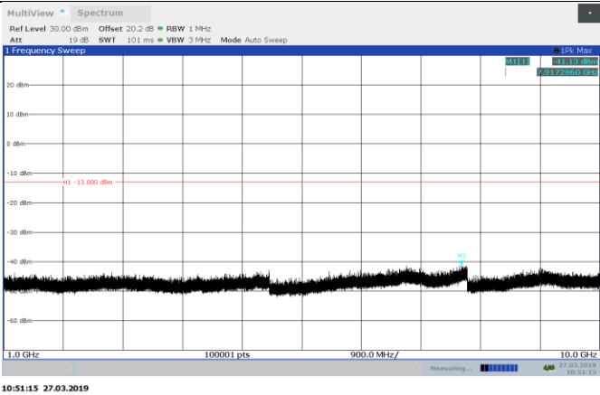
Figure 8.6-2: 931.5125 MHz, 1-10 GHz conducted emission
