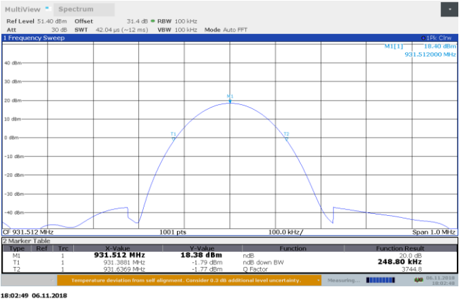
Figure 8.4-2: AGC+3 dB 931.5125 MHz output power
