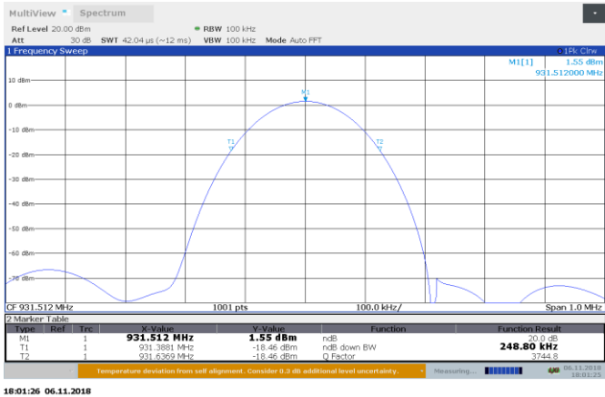
Figure 8.4-3: AGC-0.5 dB 931.5125 MHz input power
