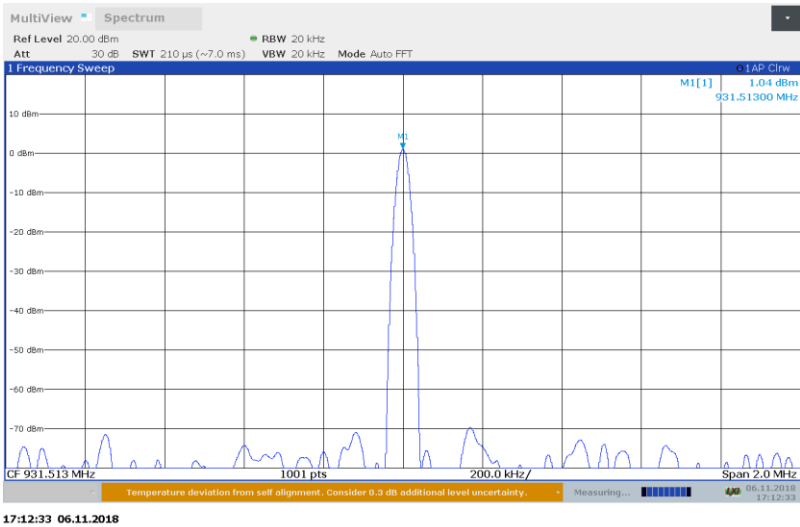
Figure 8.1-1: AGC +1 dB 931.513 MHz input power
