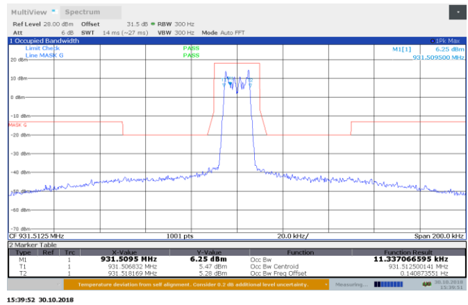
Figure 8.3-2: 11K2F1D AGC-0.5 dB 931.5125 MHz output 99% BW Emission Mask G
