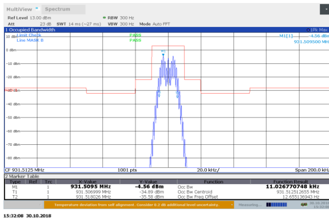
Figure 8.3-7: 11Kof3E AGC +3 dB 931.5125 MHz input 99% BW Emission Mask B
