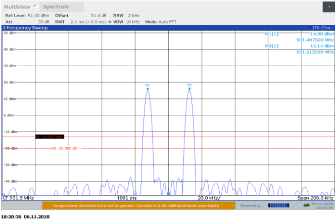
Figure 8.5-2: 931.4875 and 931.5125 MHz AGC + 3dB Out-of-block
