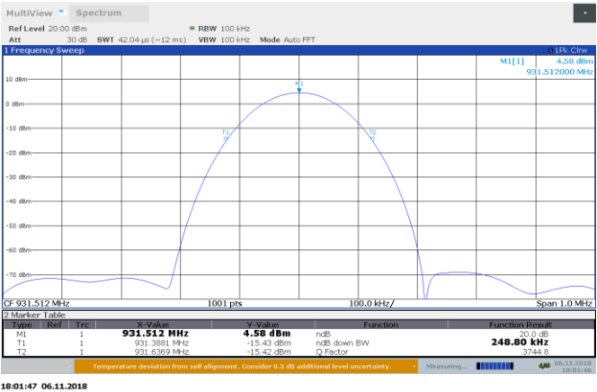
Figure 8.4-4: AGC+3 dB 931.5125 MHz input power
