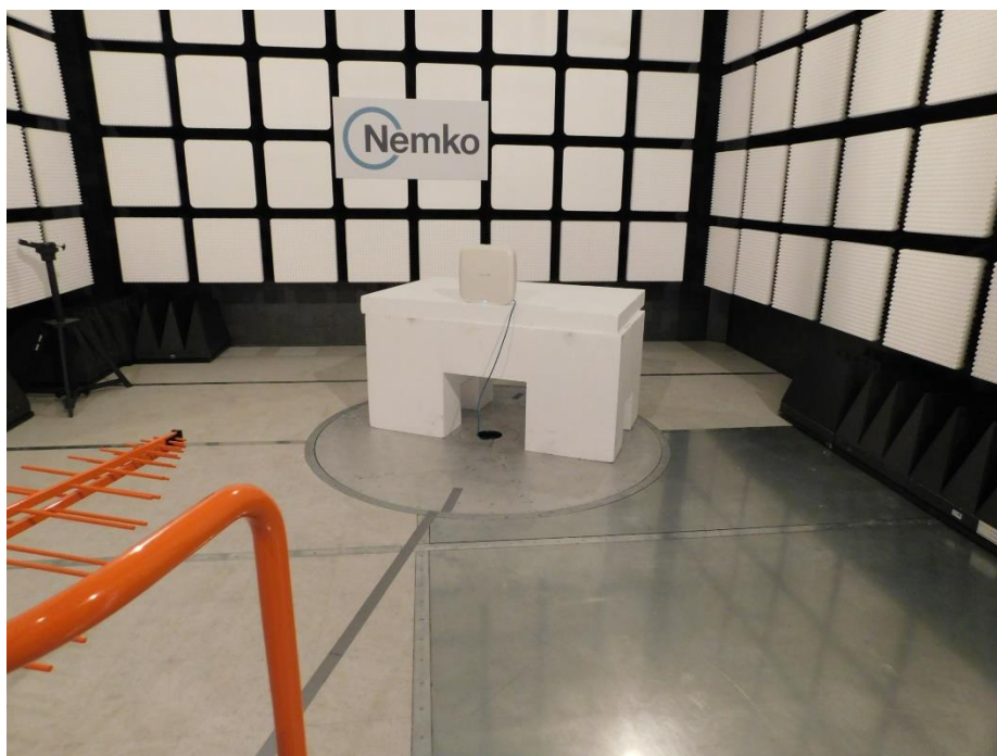
Figure 9.1-1: Radiated setup photo - Front
