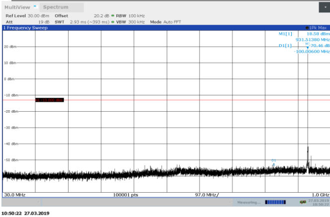
Figure 8.6-1: 931.5125 MHz, 30-1000 MHz conducted emission
