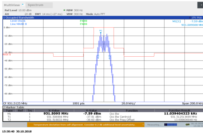
Figure 8.3-5: 11Kof3E AGC-0.5 dB 931.5125 MHz input 99% BW Emission Mask B
