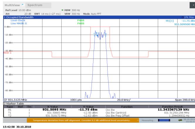
Figure 8.3-1: 11K2F1D AGC-0.5 dB 931.5125 MHz input 99% BW Emission Mask G
