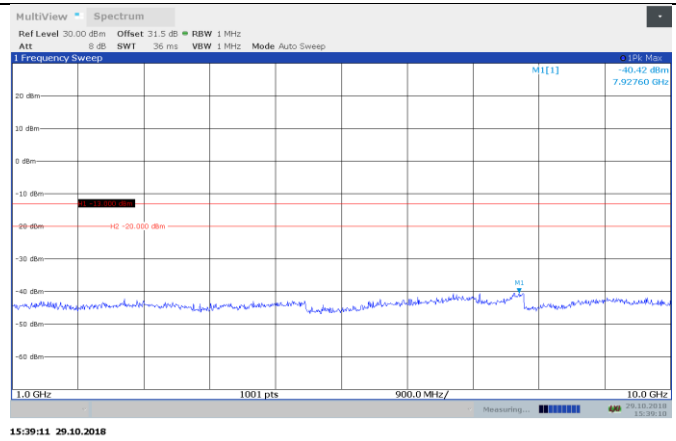
Figure 8.6-2: 929.5125 MHz 1-10 GHz conducted emission
