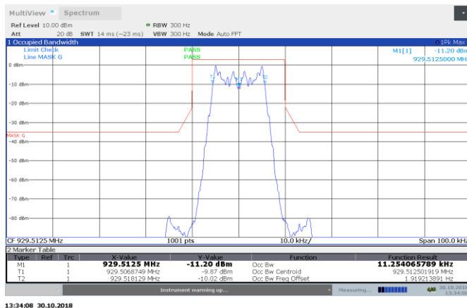
Figure 8.3-3: 11K2F1D AGC +3 dB 929.5125 MHz input 99% BW Emission Mask G
