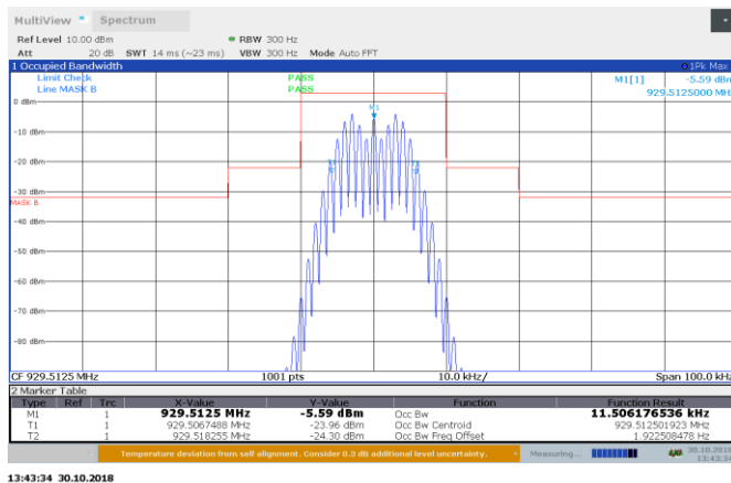
Figure 8.3-7: 11Kof3E AGC +3 dB 929.5125 MHz input 99% BW Emission Mask B
