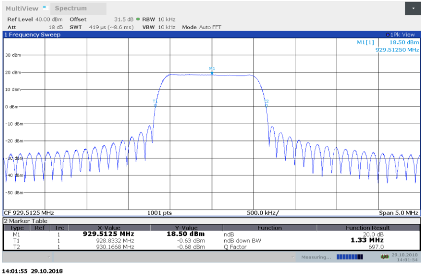
Figure 8.2-1: Passband
