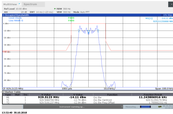
Figure 8.3-1: 11K2F1D AGC-0.5 dB 929.5125 MHz input 99% BW Emission Mask G
