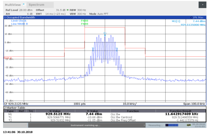
Figure 8.3-6: 11Kof3E AGC-0.5 dB 929.5125 MHz output 99% BW Emission Mask B
