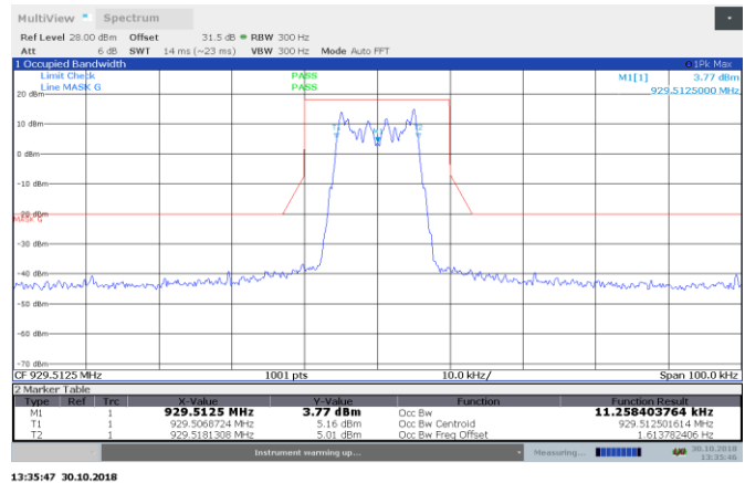
Figure 8.3-2: 11K2F1D AGC-0.5 dB 929.5125 MHz output 99% BW Emission Mask G
