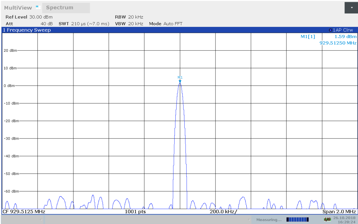
Figure 8.1-1: AGC +1 dB 929.5125 MHz input power
