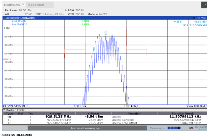
Figure 8.3-5: 11Kof3E AGC-0.5 dB 929.5125 MHz input 99% BW Emission Mask B
