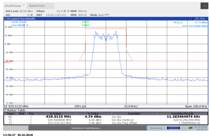
Figure 8.3-4: 11K2F1D AGC +3 dB 929.5125 MHz output 99% BW Emission Mask G
