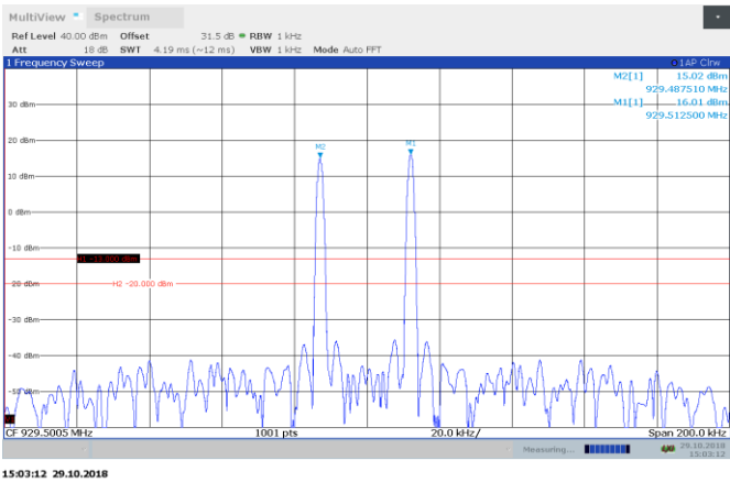
Figure 8.5-1: 929.4875 and 929.5125 MHz AGC + 0.5 Out-of-block
