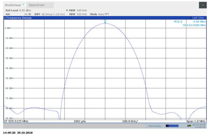
Figure 8.4-4: AGC+3 dB 929.5125 MHz input power
