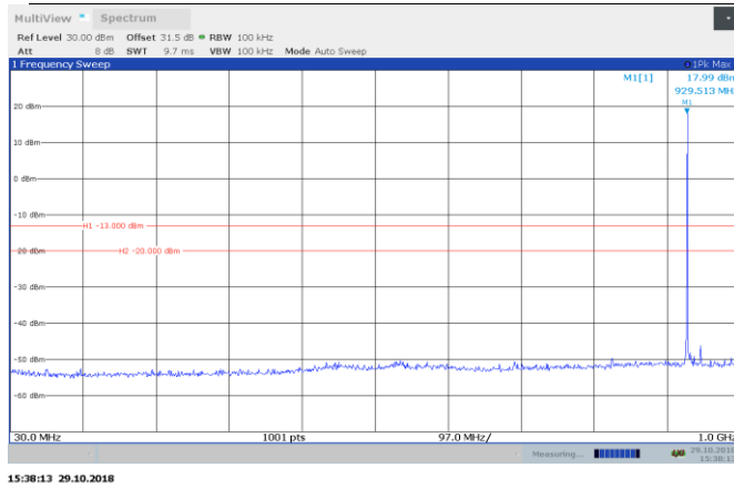
Figure 8.6-1: 929.5125 MHz 30-1000 MHz conducted emission
