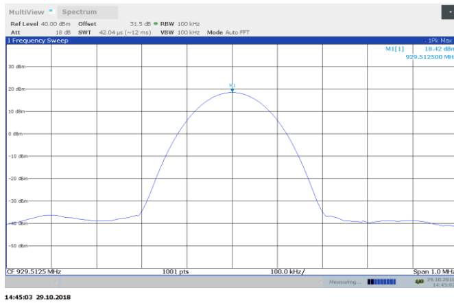
Figure 8.4-1: AGC-0.5 dB 929.5125 MHz output power
