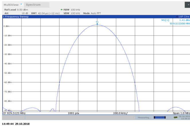
Figure 8.4-3: AGC-0.5 dB 929.5125 MHz input power
