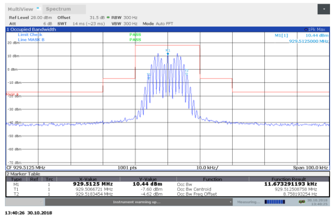
Figure 8.3-8: 11Kof3E AGC +3 dB 929.5125 MHz output 99% BW Emission Mask B
