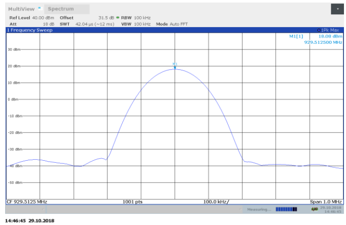
Figure 8.4-2: AGC+3 dB 929.5125 MHz output power
