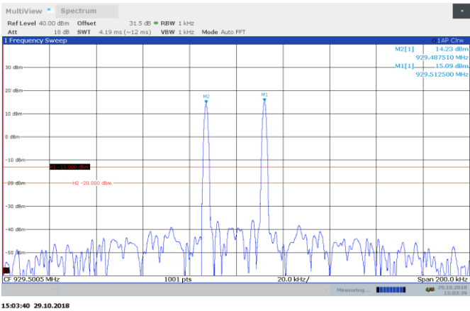
Figure 8.5-2: 929.4875 and 929.5125 MHz AGC + 3dB Out-of-block
