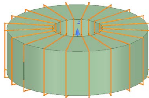
Figure 14: Toroid model.
