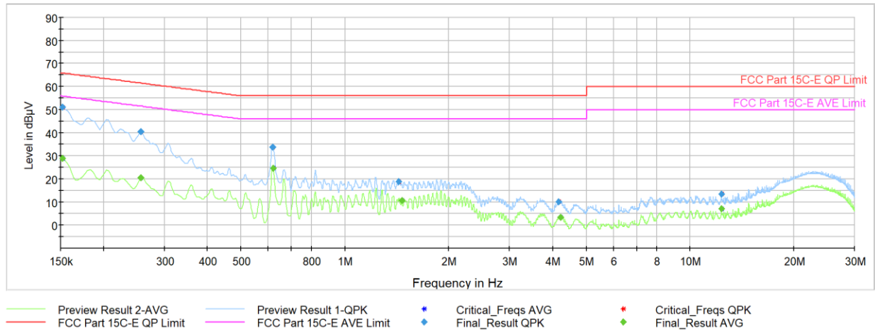
Plot 7-32. AC Line Conducted Plot with Bluetooth LE (L1, 1Mbps – Ch.19 with host PC via USB-C cable with charger)
