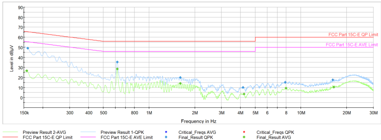
Plot 7-33. AC Line Conducted Plot with Bluetooth LE (N, 1Mbps – Ch.19, with host PC via USB-C cable with charger)
