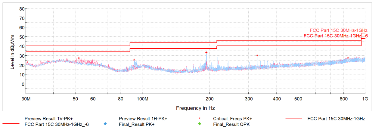
Plot 7-31. Radiated Spurious Emissions Below 1GHz (1Mbps – Ch.19, Pol. H & V, with AC/DC Adapter via USB-C cable)
