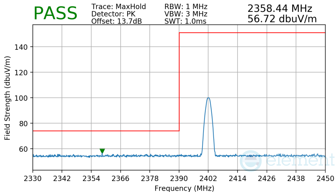
Plot 7-34. Radiated Restricted Lower Band Edge Measurement
