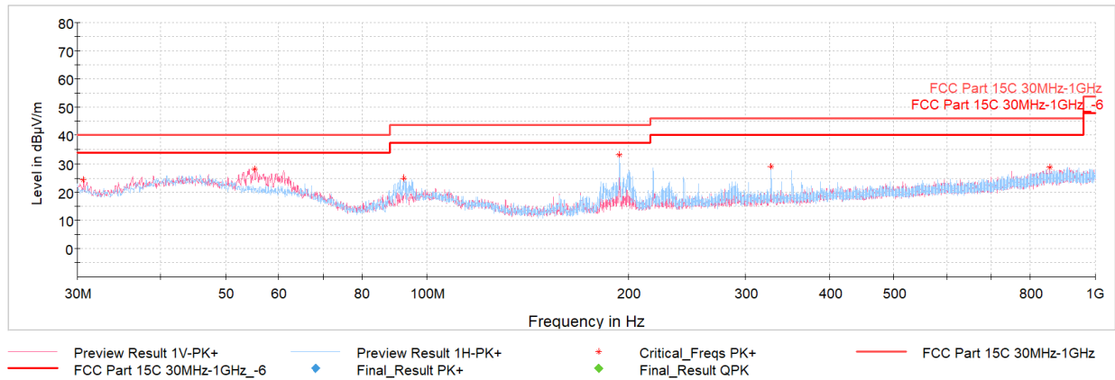
Plot 7-37. Radiated Spurious Emissions Below 1GHz (GFSK – Ch.39, with AC/DC adaptor via USB-C cable)
