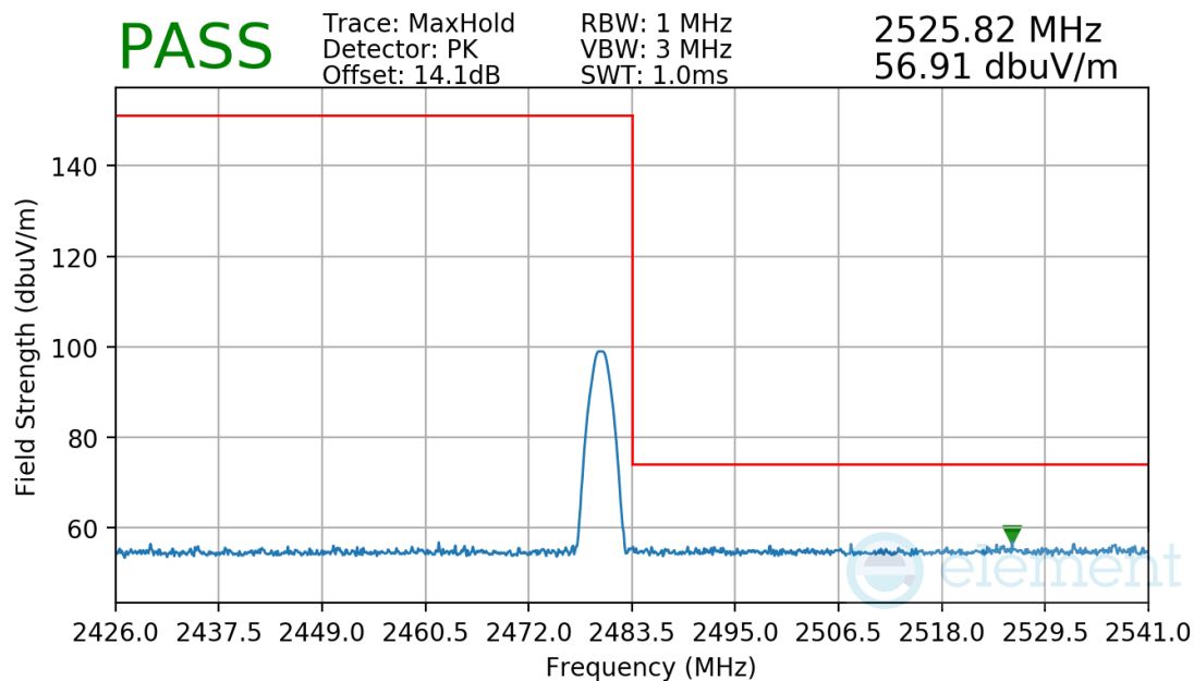
Plot 7-36. Radiated Restricted Upper Band Edge Measurement
