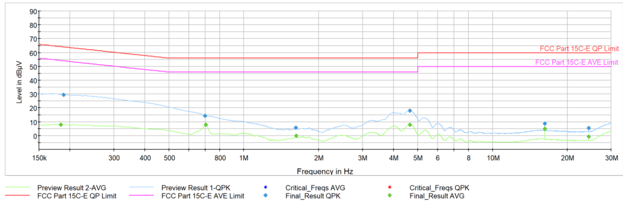
Plot 7-39. AC Line-Conducted Test Plot (N, GFSK – Ch.39, with AC/DC adaptor via USB-C cable)
