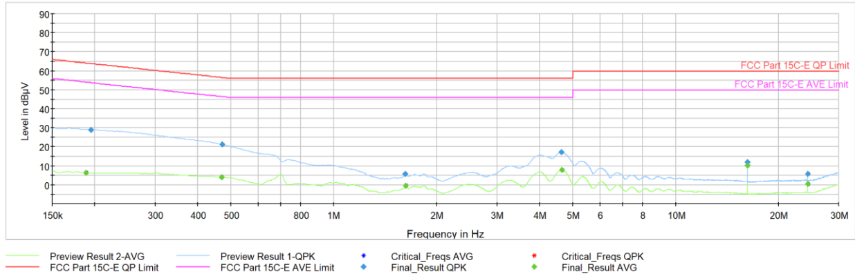
Plot 7-38. AC Line-Conducted Test Plot (L1, GFSK – Ch.39, with AC/DC adaptor via USB-C cable)
