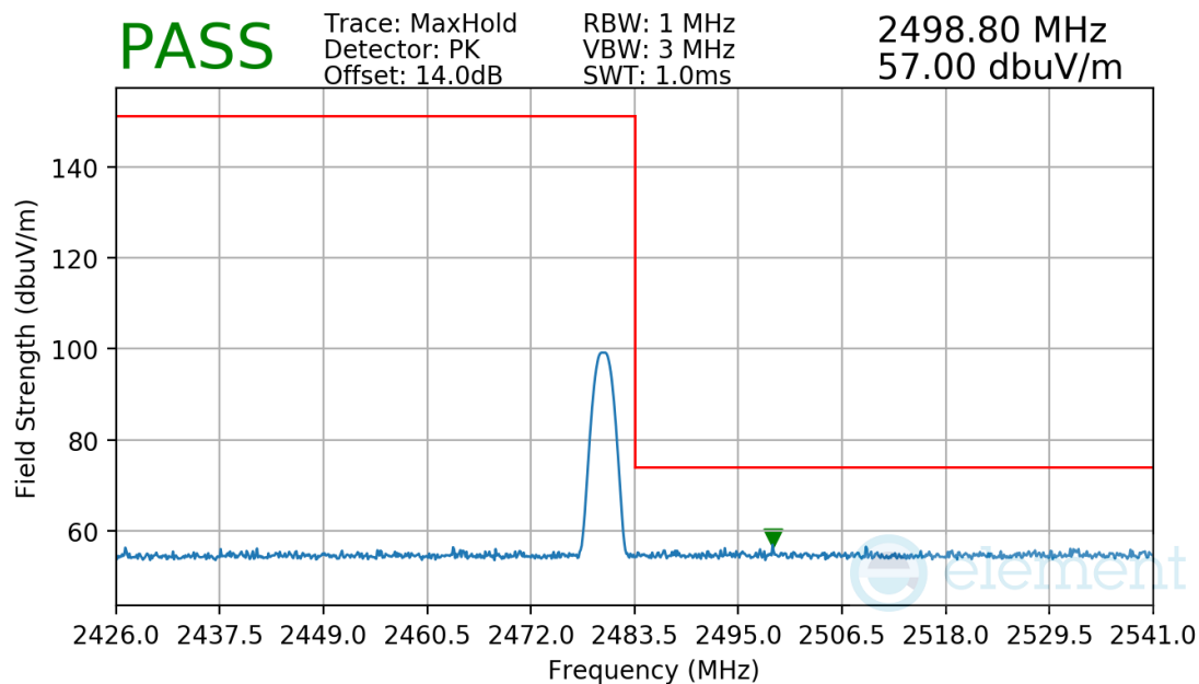
Plot 7-35. Radiated Restricted Upper Band Edge Measurement
