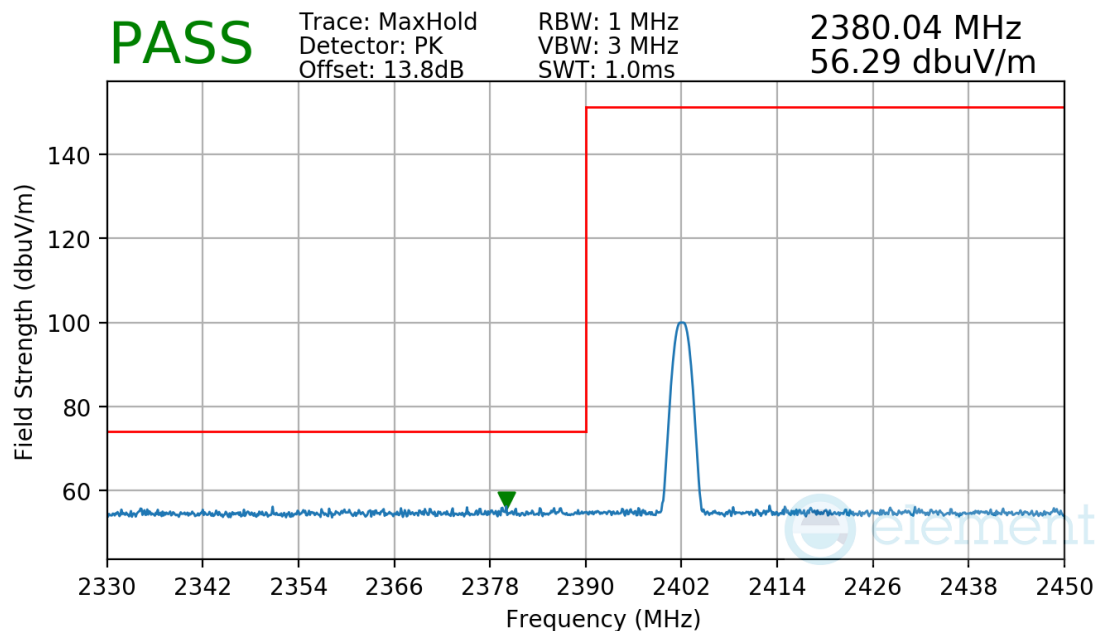
Plot 7-33. Radiated Restricted Lower Band Edge Measurement
