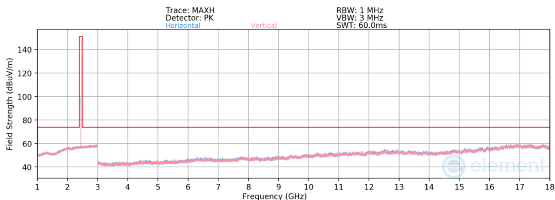
Plot 7-30. Radiated Spurious Emissions 1-18GHz (BT GFSK – Ch. 39)
