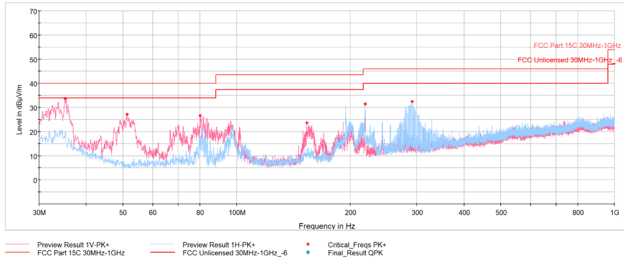
Plot 7-37. Radiated Spurious Emissions Below 1GHz (GFSK – Ch.39, with AC/DC adaptor via USB-C cable)
