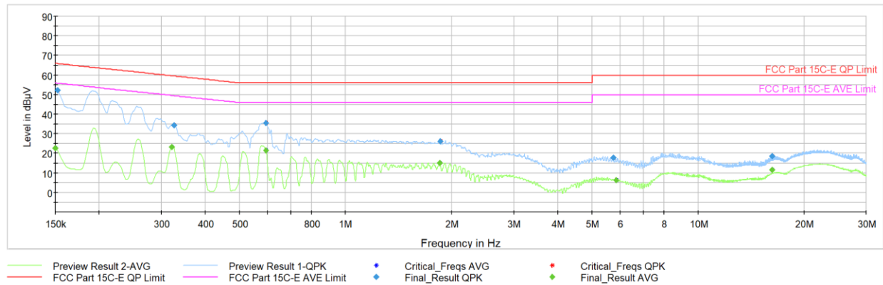
Plot 7-32. AC Line Conducted Plot with Bluetooth LE (L1, 1Mbps – Ch.19 with host PC via USB-C cable with charger)
