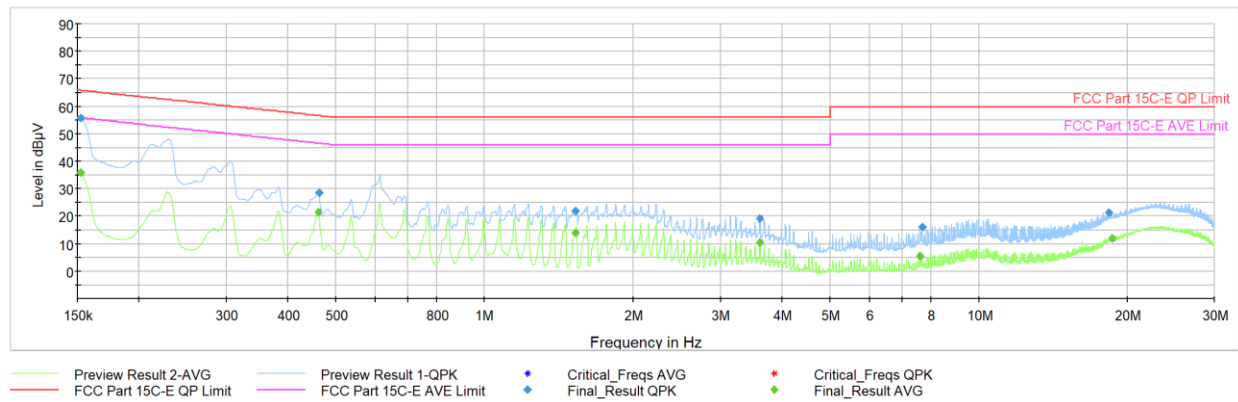
Plot 7-33. AC Line Conducted Plot with Bluetooth LE (N, 1Mbps – Ch.19, with host PC via USB-C cable with charger)
