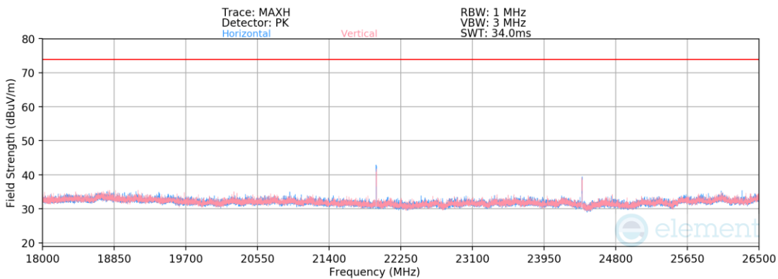
Plot 7-25. Radiated Spurious Emissions Above 18GHz (1Mbps- Ch. 19)
