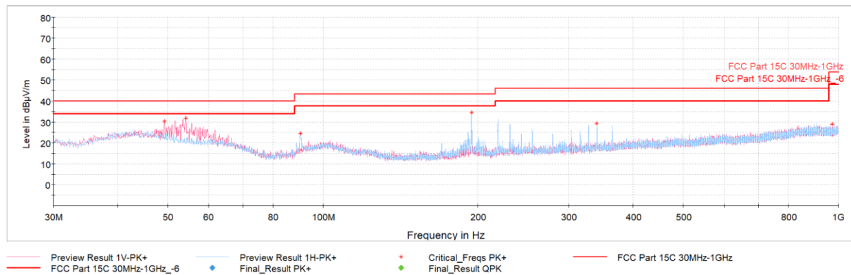
Plot 7-31. Radiated Spurious Emissions Below 1GHz (1Mbps – Ch.19, Pol. H & V, with AC/DC Adapter via USB-C cable)
