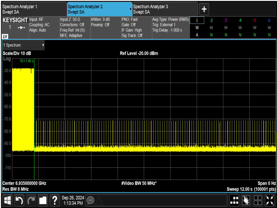
Figure 359 - U-NII-8, Minimum Bandwidth (AWGN High)
