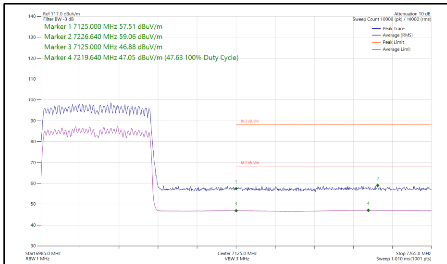
Figure 225 - 802.11ax HE80, SU, CDD, Core 0 - Core 1 - 7025 MHz Band Edge Frequency 7125 MHz
