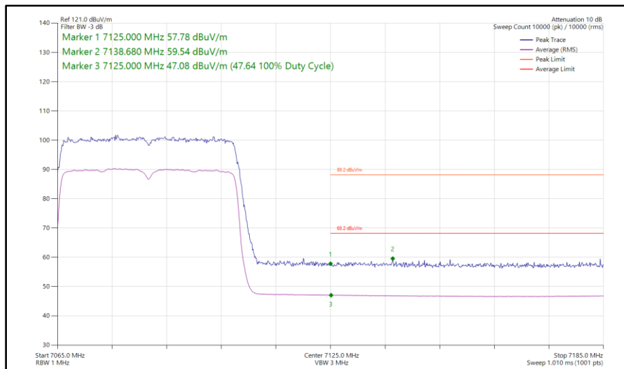
Figure 203 - 802.11ax HE40, SU, SISO, Core 1 - 7085 MHz Band Edge Frequency 7125 MHz
