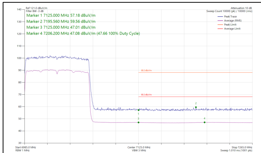
Figure 217 - 802.11ax HE80, SU, SISO, Core 0 - 7025 MHz Band Edge Frequency 7125 MHz
