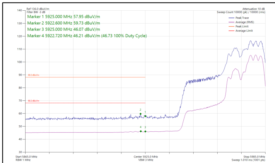
Figure 210 - 802.11ax HE40, RU 106-56, SDM, Core 0 - Core 1 - 5965 MHz Band Edge Frequency 5925 MHz
