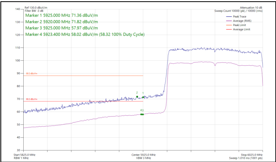
Figure 215 - 802.11ax HE80, SU, SISO, Core 0 - 5985 MHz Band Edge Frequency 5925 MHz
