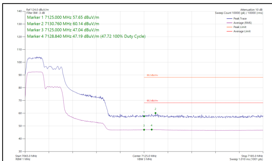
Figure 204 - 802.11ax HE40, RU 106-53, SISO, Core 1 - 7085 MHz Band Edge Frequency 7125 MHz
