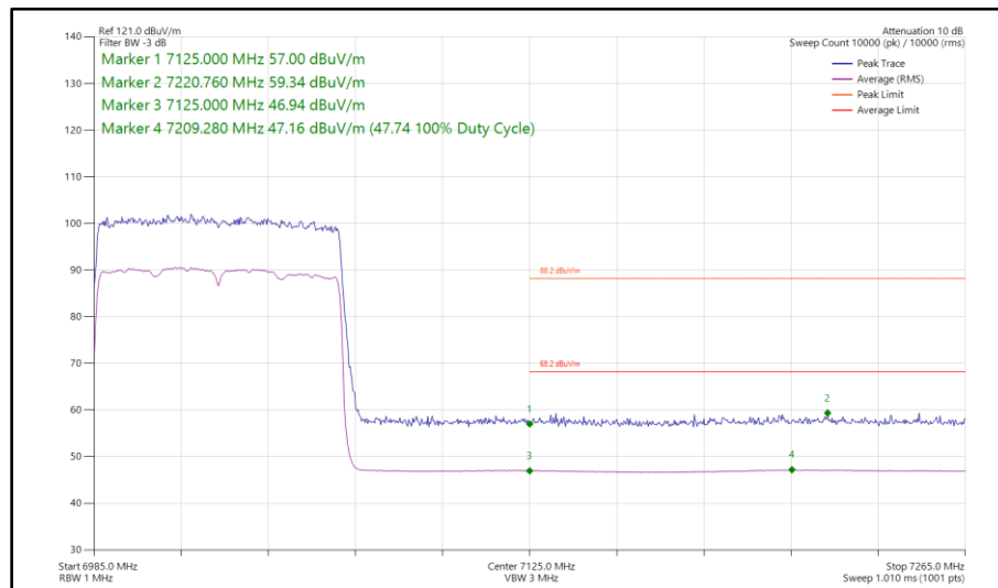
Figure 221 - 802.11ax HE80, SU, SISO, Core 1 - 7025 MHz Band Edge Frequency 7125 MHz
