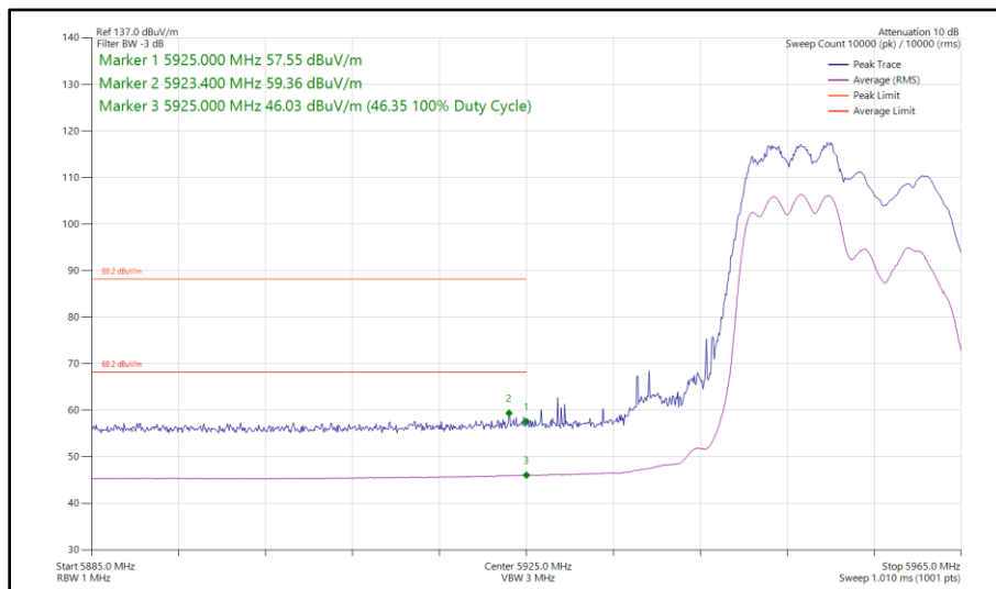
Figure 193 - 802.11ax HE20, RU 106-53, SDM, Core 0 - Core 1 - 5955 MHz Band Edge Frequency 5925 MHz
