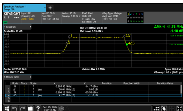
Figure 115 - 802.11ax HE40 SU VLP Minimum 26 dB EBW
