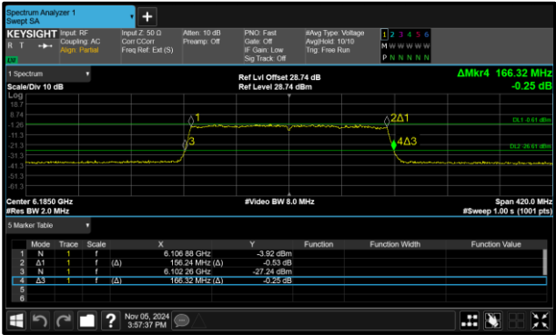
Figure 143 - 802.11ax HE160 SU VLP Minimum 99% OBW
