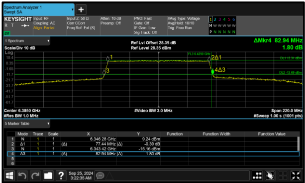
Figure 102 - 802.11ax HE80 SU SP Maximum 99% OBW
