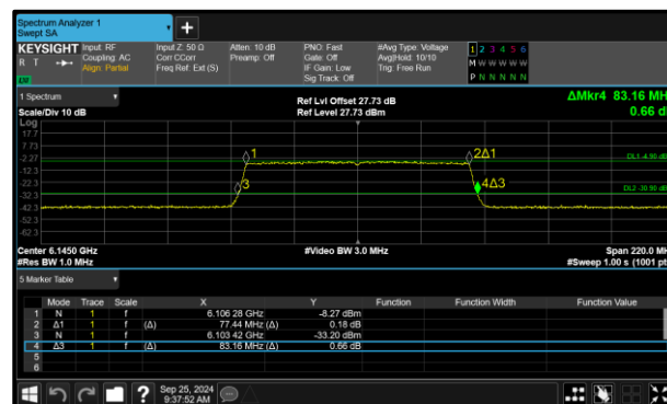
Figure 118 - 802.11ax HE80 SU VLP Maximum 26 dB EBW
