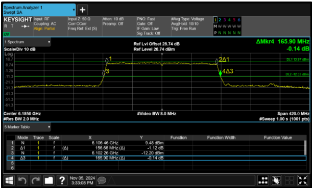
Figure 127 - 802.11ax HE160 SU SP Minimum 26 dB EBW
