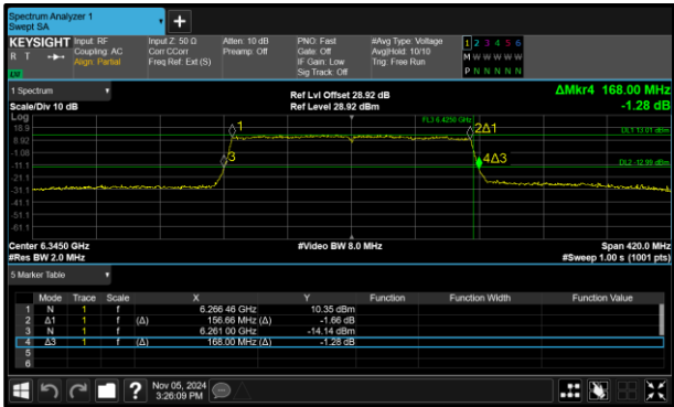
Figure 82 - 802.11ax HE160 SU SP Maximum 26 dB EBW
