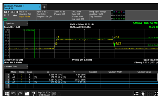
Figure 96 - 802.11ax HE160 SU VLP Maximum 99% OBW
