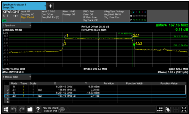
Figure 128 - 802.11ax HE160 SU SP Maximum 26 dB EBW
