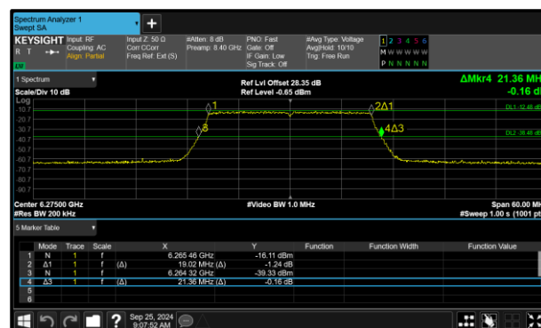
Figure 114 - 802.11ax HE20 SU VLP Maximum 26 dB EBW
