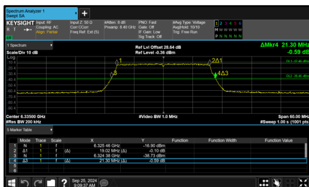
Figure 113 - 802.11ax HE20 SU VLP Minimum 26 dB EBW
