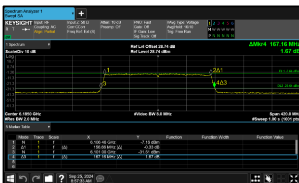
Figure 95 - 802.11ax HE160 SU VLP Minimum 99% OBW
