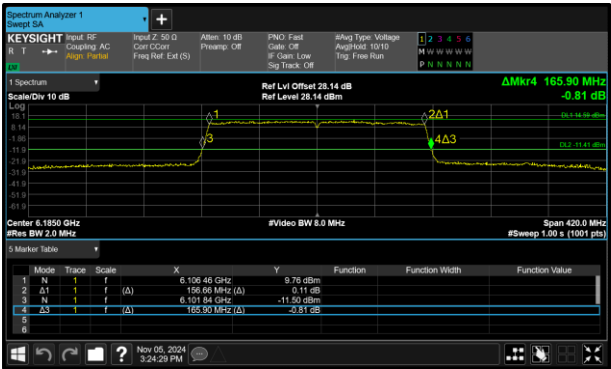
Figure 81 - 802.11ax HE160 SU SP Minimum 26 dB EBW
