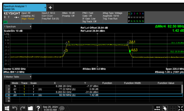
Figure 117 - 802.11ax HE80 SU VLP Minimum 26 dB EBW
