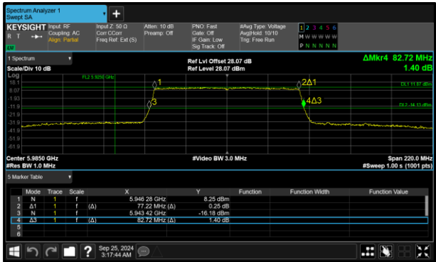
Figure 101 - 802.11ax HE80 SU SP Minimum 99% OBW
