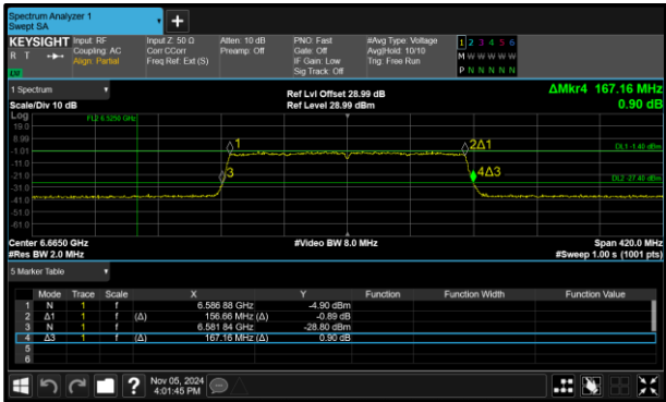
Figure 120 - 802.11ax HE160 SU VLP Maximum 26 dB EBW
