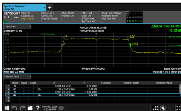
Figure 151 - 802.11ax HE160 SU SP Minimum 99% OBW
