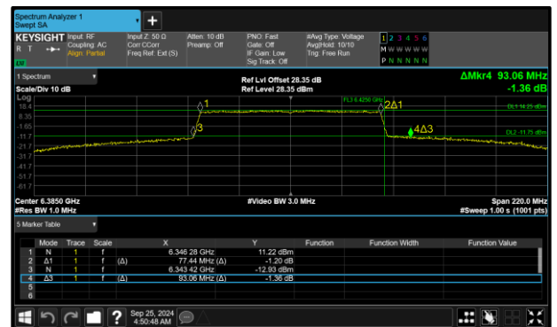
Figure 150 - 802.11ax HE80 SU SP Maximum 99% OBW
