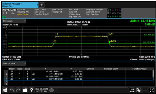
Figure 142 - 802.11ax HE80 SU VLP Maximum 99% OBW
