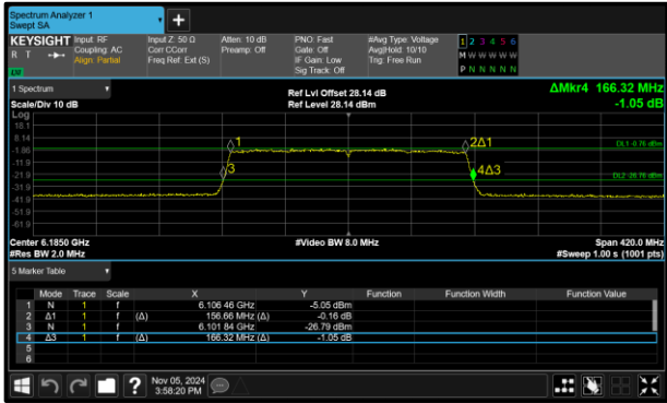
Figure 144 - 802.11ax HE160 SU VLP Maximum 99% OBW
