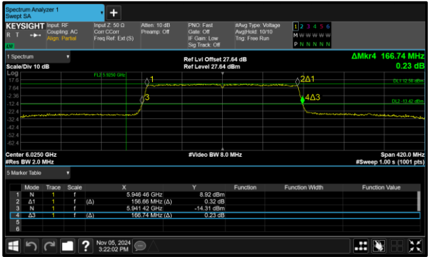
Figure 104 - 802.11ax HE160 SU SP Maximum 99% OBW
