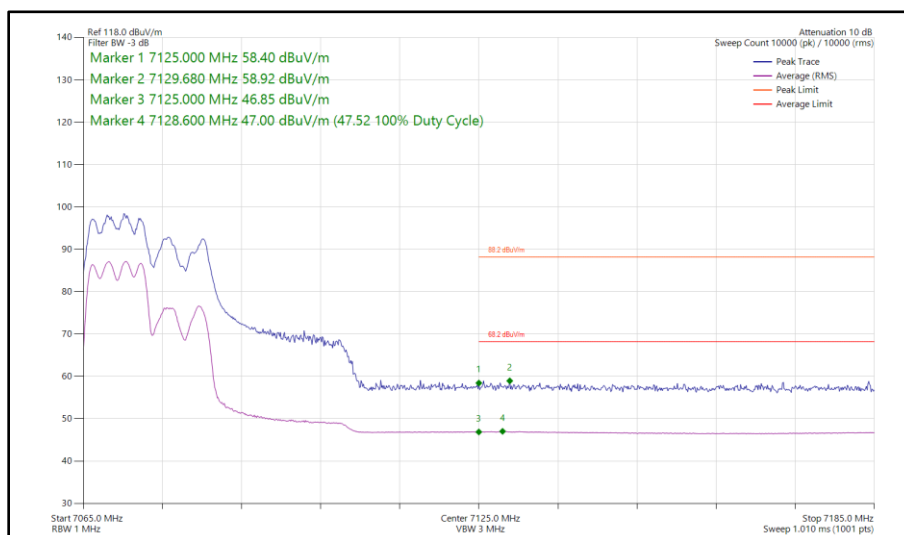
Figure 209 - 802.11ax HE40, RU 106-53, CDD, Core 0 - Core 1 - 7085 MHz Band Edge Frequency 7125 MHz
