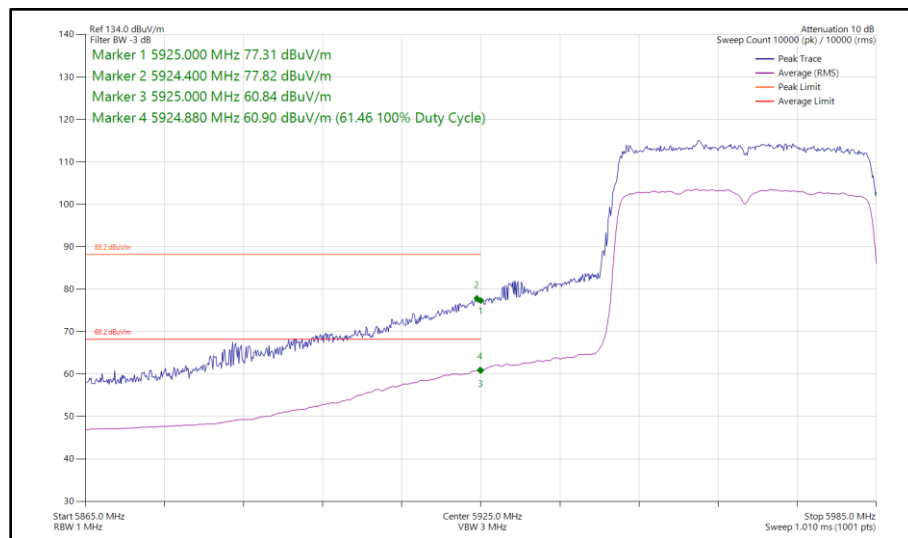
Figure 198 - 802.11ax HE40, SU, SISO, Core 0 - 5965 MHz Band Edge Frequency 5925 MHz
