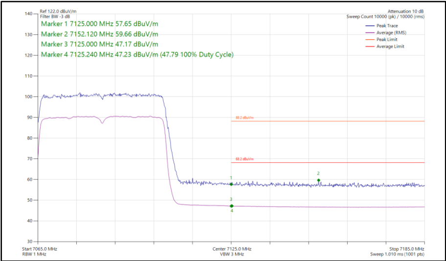
Figure 204 - 802.11ax HE40, SU, SISO, Core 1 - 7085 MHz Band Edge Frequency 7125 MHz
