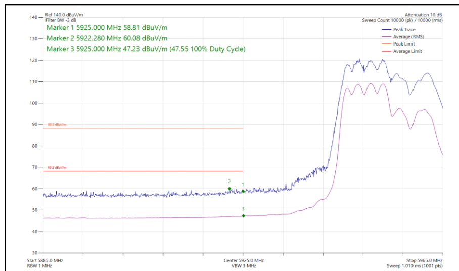
Figure 193 - 802.11ax HE20, RU 106-53, SDM, Core 0 - Core 1 - 5955 MHz Band Edge Frequency 5925 MHz
