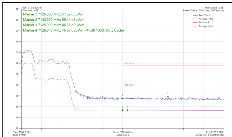
Figure 187 - 802.11ax HE20, RU 52-37, SISO, Core 1 - 7095 MHz Band Edge Frequency 7125 MHz
