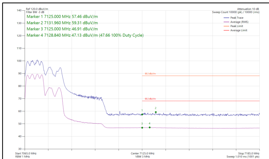
Figure 213 - 802.11ax HE40, RU 106-53, SDM, Core 0 - Core 1 - 7085 MHz Band Edge Frequency 7125 MHz
