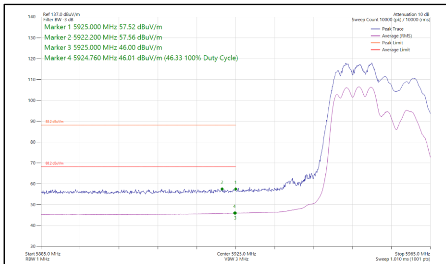
Figure 189 - 802.11ax HE20, RU 106-53, CDD, Core 0 - Core 1 - 5955 MHz Band Edge Frequency 5925 MHz
