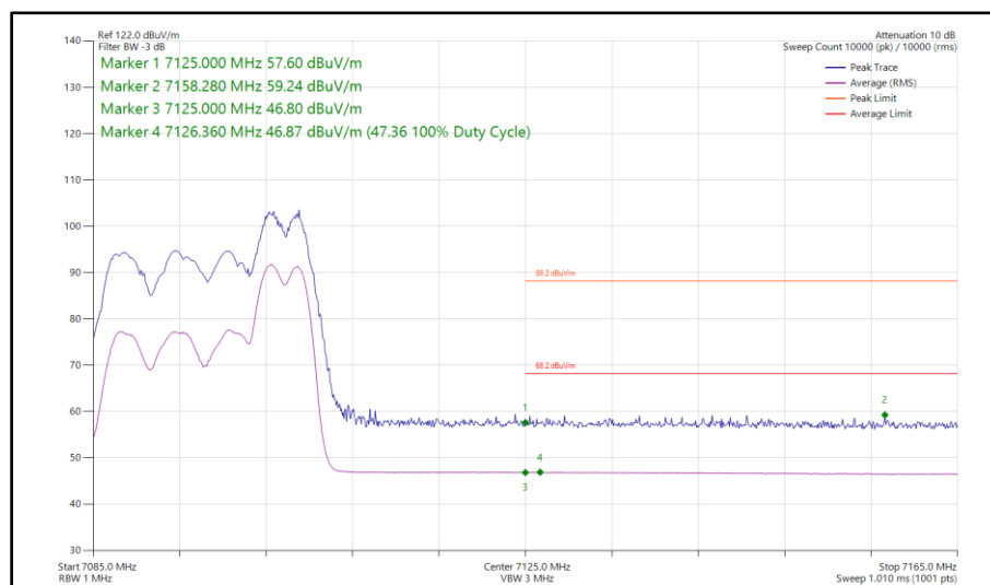
Figure 195 - 802.11ax HE20, RU 52-40, SDM, Core 0 - Core 1 - 7095 MHz Band Edge Frequency 7125 MHz
