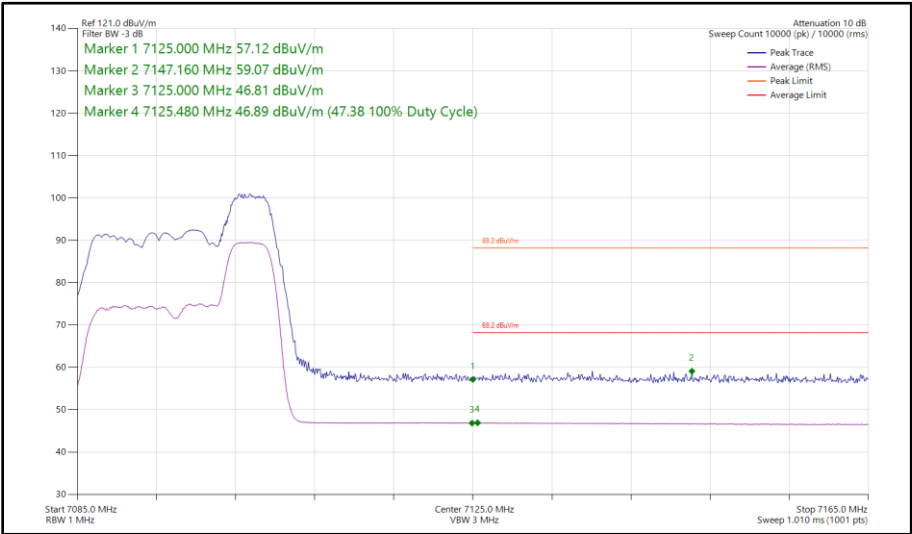
Figure 181 - 802.11ax HE20, RU 52-40, SISO, Core 0 - 7095 MHz Band Edge Frequency 7125 MHz
