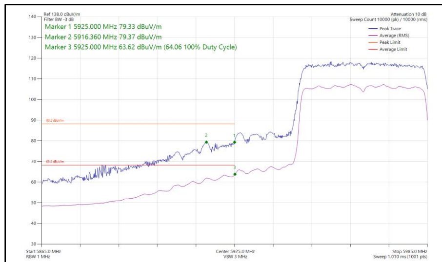
Figure 210 - 802.11ax HE40, SU, SDM, Core 0 - Core 1 - 5965 MHz Band Edge Frequency 5925 MHz
