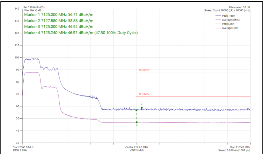
Figure 201 - 802.11ax HE40, RU 106-53, SISO, Core 0 - 7085 MHz Band Edge Frequency 7125 MHz
