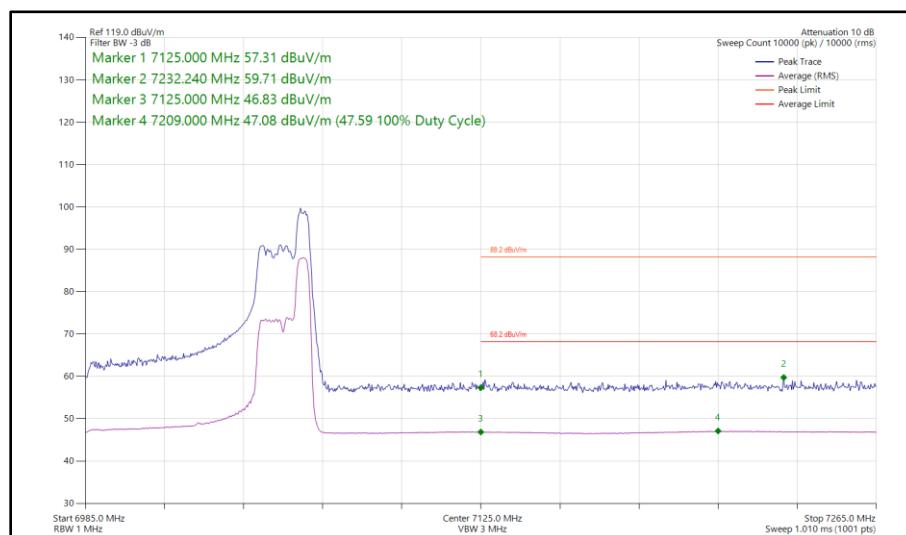
Figure 219 - 802.11ax HE80, RU 52-52, SISO, Core 0 - 7025 MHz Band Edge Frequency 7125 MHz
