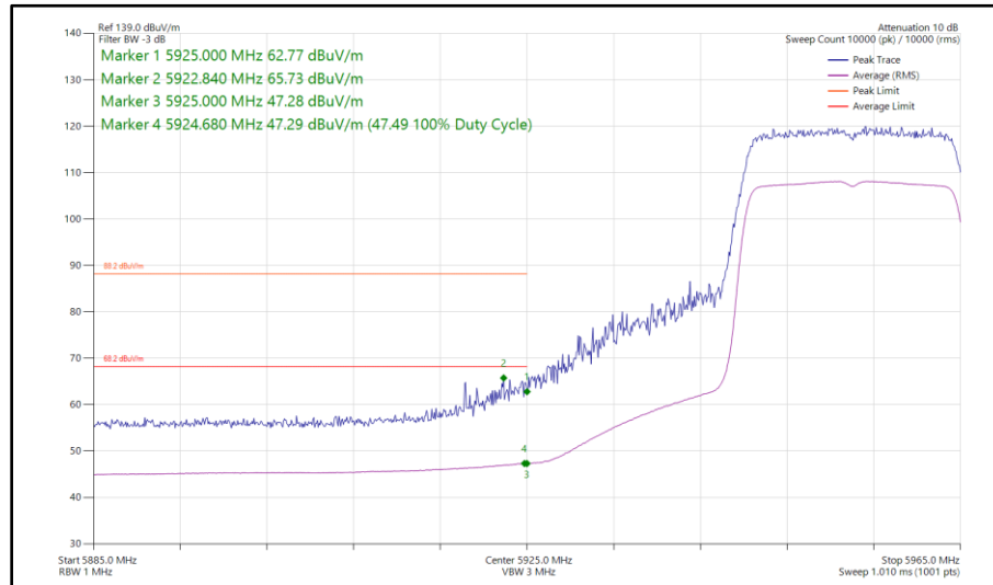
Figure 196 - 802.11ax HE20, SU, TxBF, Core 0 - Core 1 - 5955 MHz Band Edge Frequency 5925 MHz
