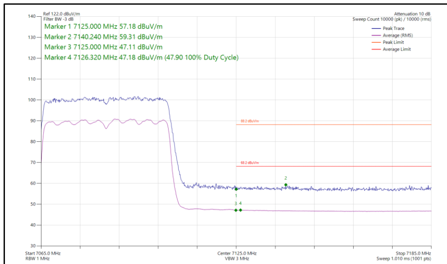
Figure 212 - 802.11ax HE40, SU, SDM, Core 0 - Core 1 - 7085 MHz Band Edge Frequency 7125 MHz
