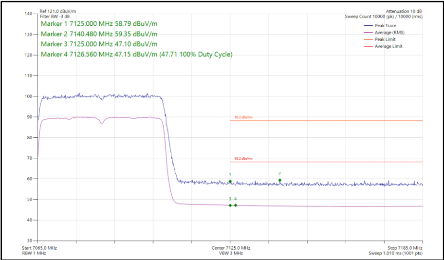
Figure 200 - 802.11ax HE40, SU, SISO, Core 0 - 7085 MHz Band Edge Frequency 7125 MHz
