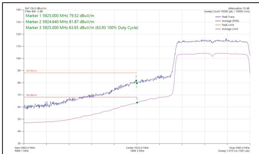
Figure 202 - 802.11ax HE40, SU, SISO, Core 1 - 5965 MHz Band Edge Frequency 5925 MHz
