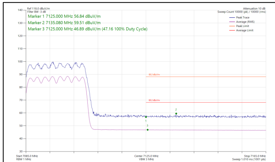
Figure 190 - 802.11ax HE20, SU, CDD, Core 0 - Core 1 - 7095 MHz Band Edge Frequency 7125 MHz
