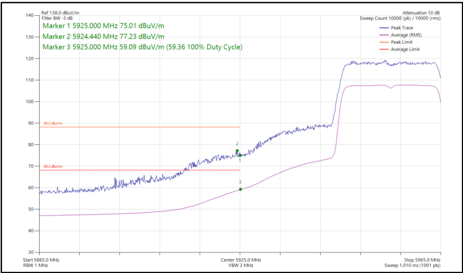
Figure 183 - 802.11ax HE20, SU, SISO, Core 1 - 5955 MHz Band Edge Frequency 5925 MHz
