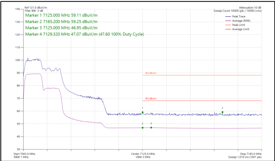
Figure 205 - 802.11ax HE40, RU 106-53, SISO, Core 1 - 7085 MHz Band Edge Frequency 7125 MHz
