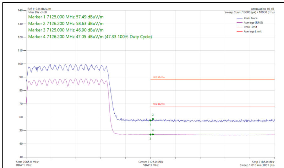
Figure 208 - 802.11ax HE40, SU, CDD, Core 0 - Core 1 - 7085 MHz Band Edge Frequency 7125 MHz
