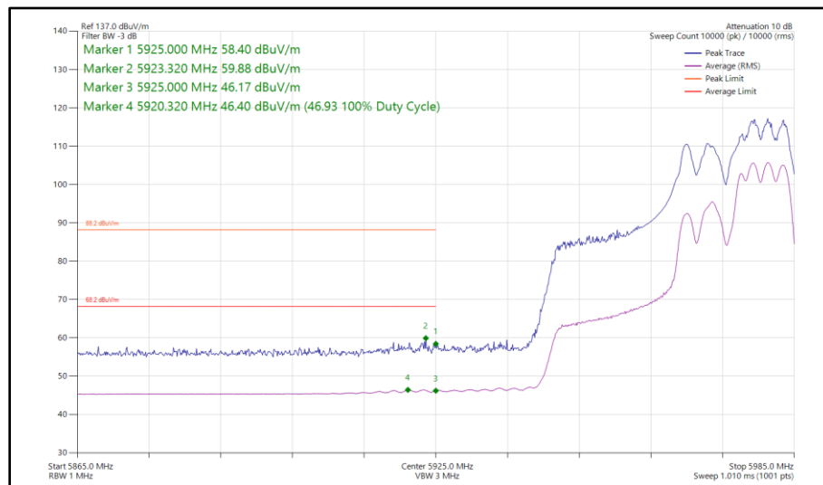
Figure 207 - 802.11ax HE40, RU 106-56, CDD, Core 0 - Core 1 - 5965 MHz Band Edge Frequency 5925 MHz
