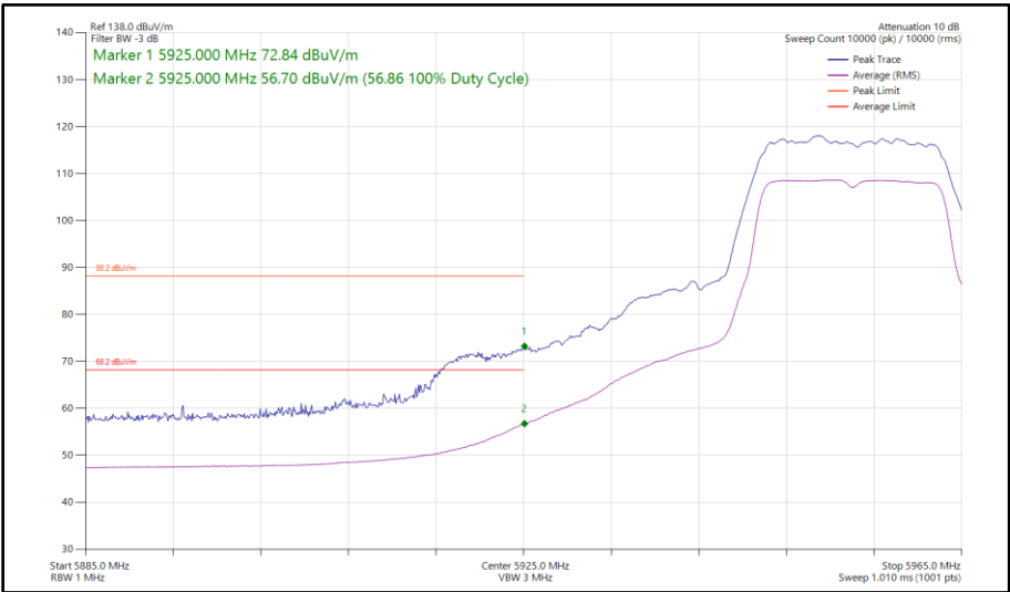
Figure 182 - 802.11a, SISO, Core 1 - 5955 MHz Band Edge Frequency 5925 MHz
