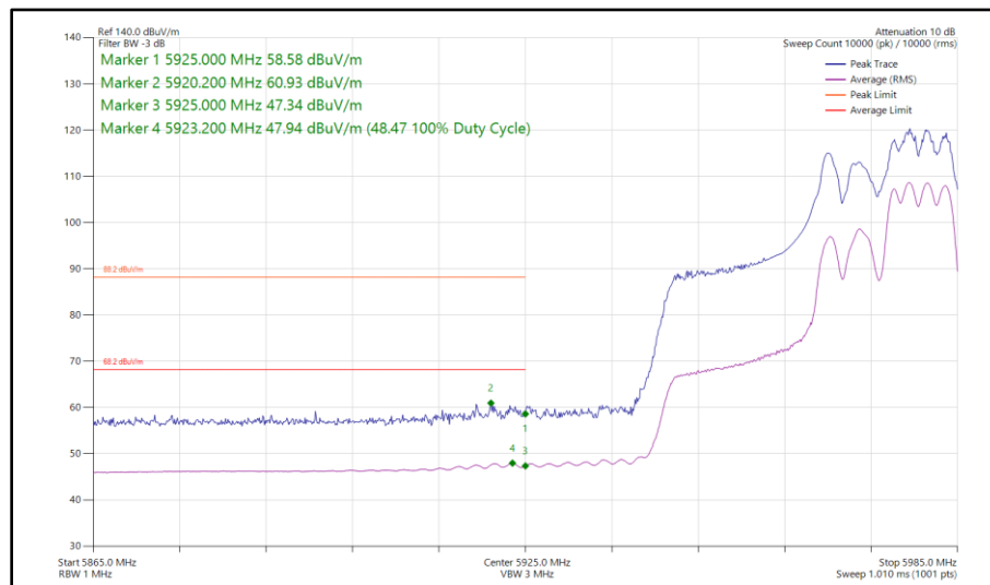
Figure 211 - 802.11ax HE40, RU 106-56, SDM, Core 0 - Core 1 - 5965 MHz Band Edge Frequency 5925 MHz
