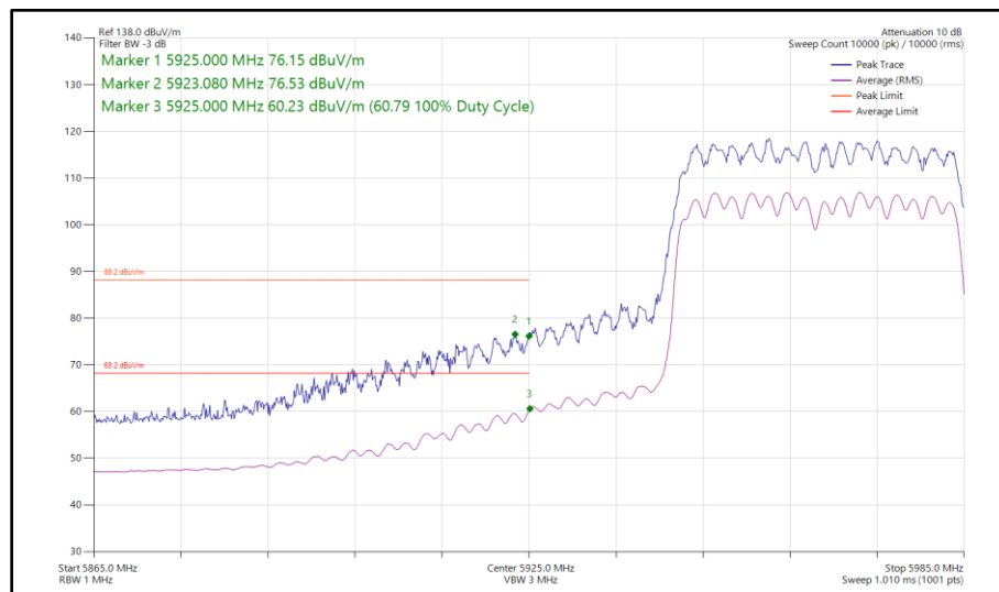
Figure 206 - 802.11ax HE40, SU, CDD, Core 0 - Core 1 - 5965 MHz Band Edge Frequency 5925 MHz
