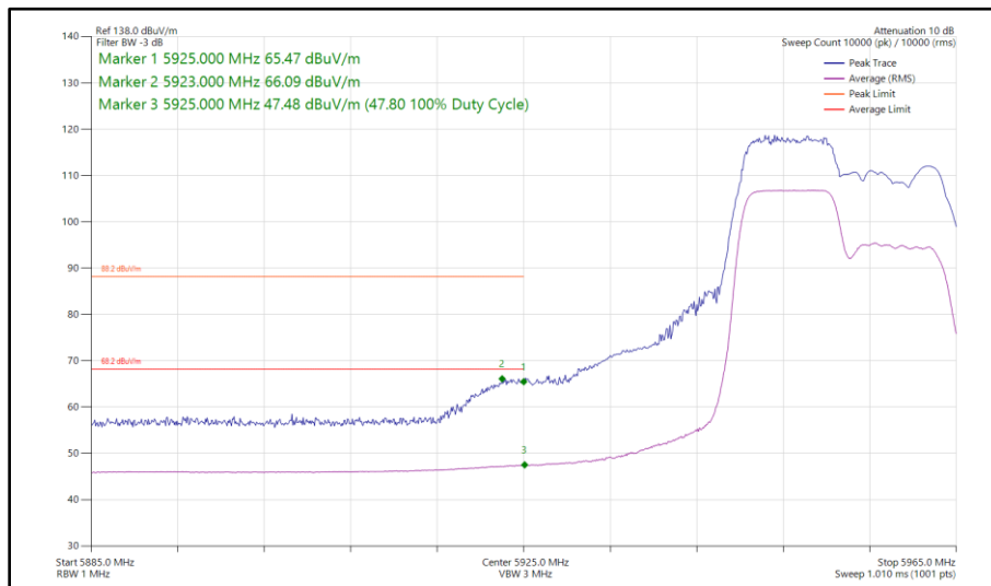
Figure 184 - 802.11ax HE20, RU 106-53, SISO, Core 1 - 5955 MHz Band Edge Frequency 5925 MHz
