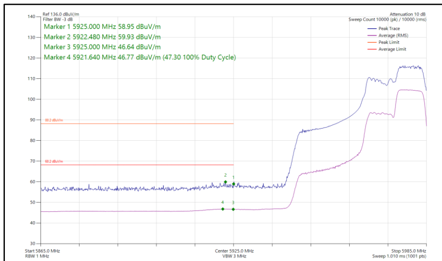
Figure 203 - 802.11ax HE40, RU 106-56, SISO, Core 1 - 5965 MHz Band Edge Frequency 5925 MHz
