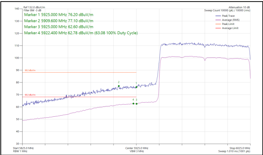
Figure 216 - 802.11ax HE80, SU, SISO, Core 0 - 5985 MHz Band Edge Frequency 5925 MHz
