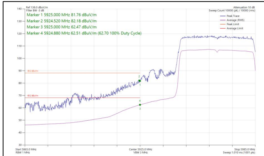
Figure 214 - 802.11ax HE40, SU, TxBF, Core 0 - Core 1 - 5965 MHz Band Edge Frequency 5925 MHz
