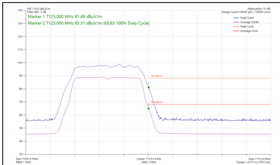
Figure 179 - 802.11a, SISO, Core 0 - 7115 MHz Band Edge Frequency 7125 MHz
