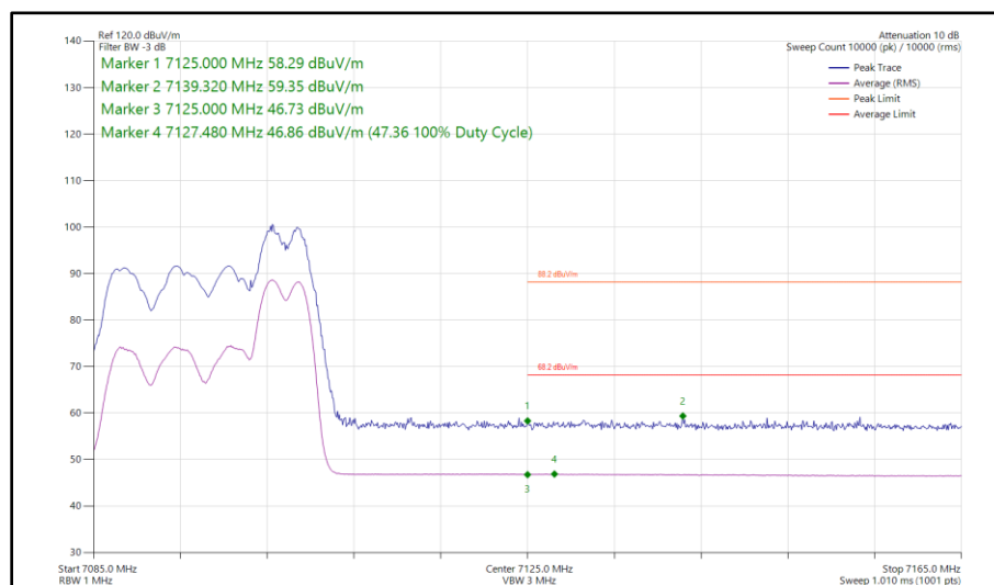
Figure 191 - 802.11ax HE20, RU 52-40, CDD, Core 0 - Core 1 - 7095 MHz Band Edge Frequency 7125 MHz
