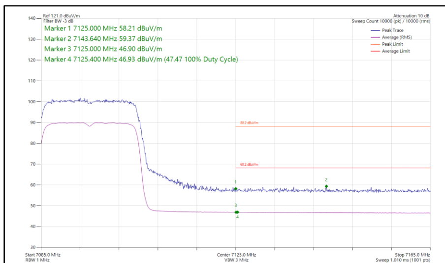
Figure 180 - 802.11ax HE20, SU, SISO, Core 0 - 7095 MHz Band Edge Frequency 7125 MHz
