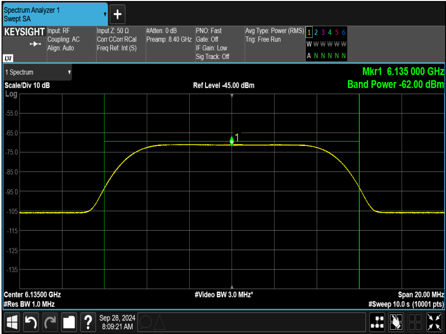
Figure 345 - Example of AWGN Signal
