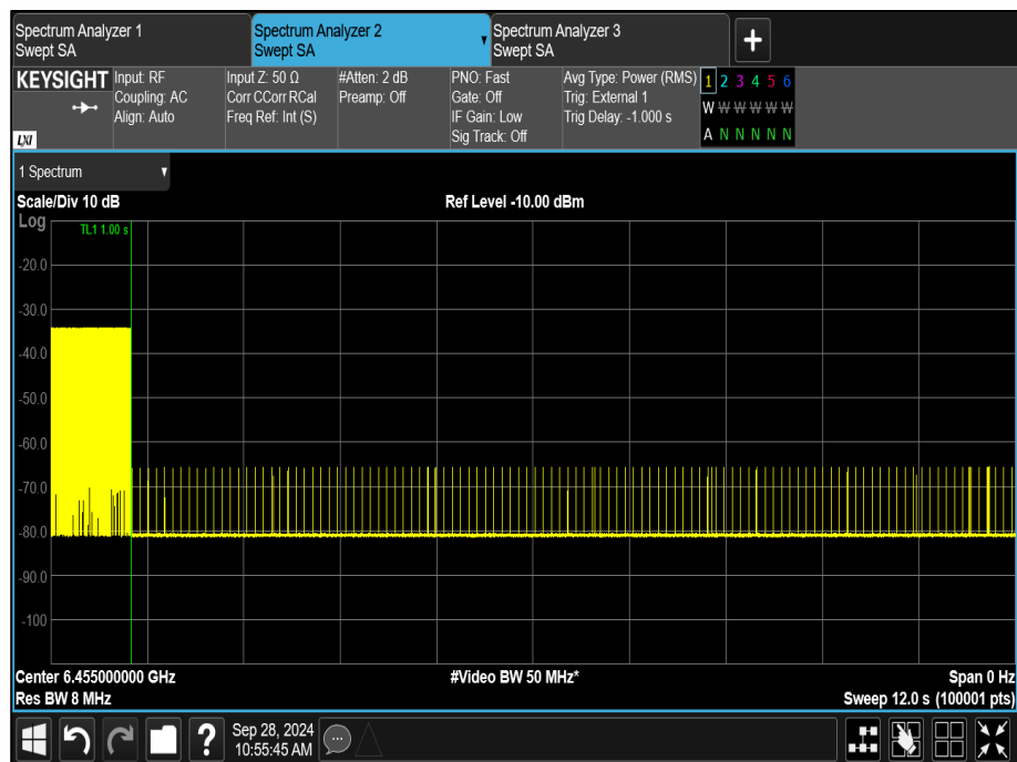
Figure 352 - U-NII-6, Minimum Bandwidth (AWGN Mid)
