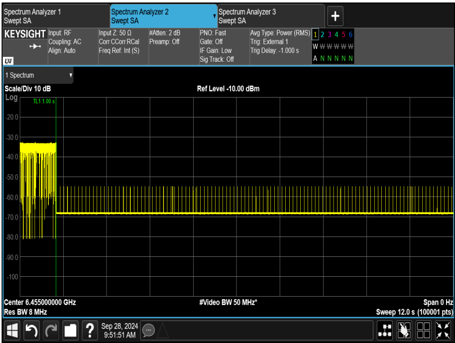
Figure 350 - U-NII-6, Minimum Bandwidth
