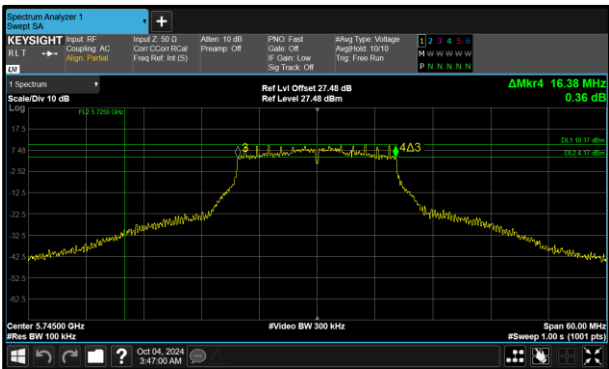
Figure 161 - 802.11a Maximum 6 dB EBW
