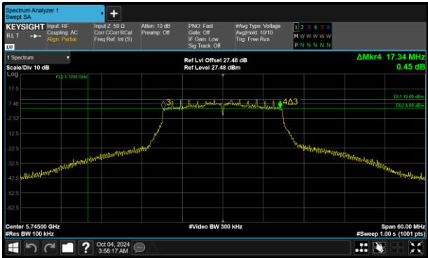
Figure 162 - 802.11n HT20 Minimum 6 dB EBW
