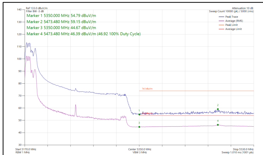
Figure 147 - 802.11ax HE160, RU 106-53P, CDD, Core 0 - Core 1 - 5250 MHz Band Edge Frequency 5350 MHz
