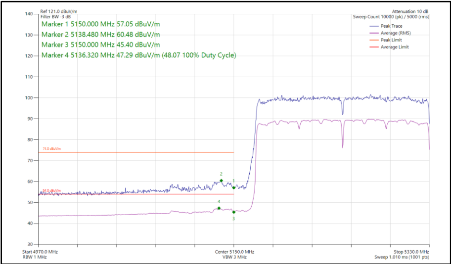
Figure 134 - 802.11ax HE160, SU, SISO, Core 1 - 5250 MHz Band Edge Frequency 5150 MHz
