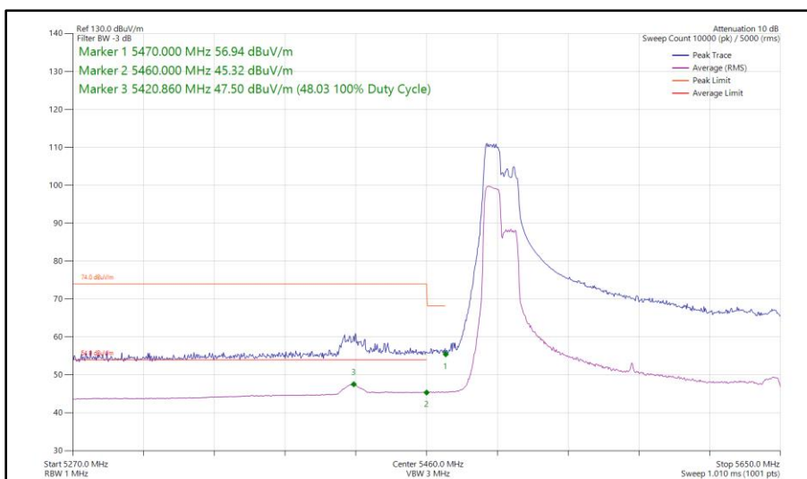
Figure 132 - 802.11ax HE160, RU 106-53P, SISO, Core 0 - 5570 MHz Band Edge Frequency 5460 MHz
