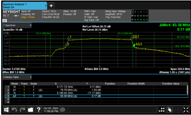
Figure 188 - 802.11ax HE80 SU Minimum 99% OBW
