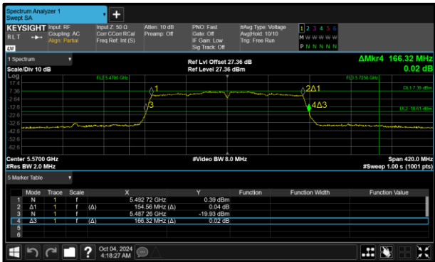
Figure 182 - 802.11ac VHT160 Minimum 99% OBW
