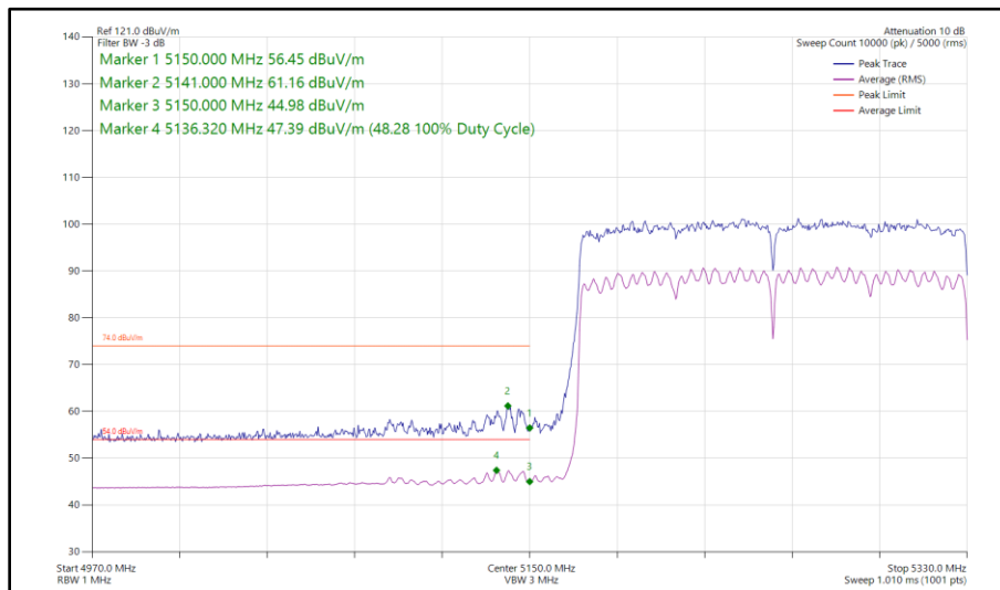
Figure 152 - 802.11ax HE160, SU, SDM, Core 0 - Core 1 - 5250 MHz Band Edge Frequency 5150 MHz
