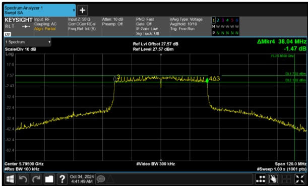
Figure 170 - 802.11ax HE40 SU Minimum 6 dB EBW
