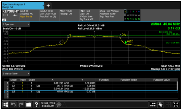
Figure 179 - 802.11n HT40 Maximum 99% OBW
