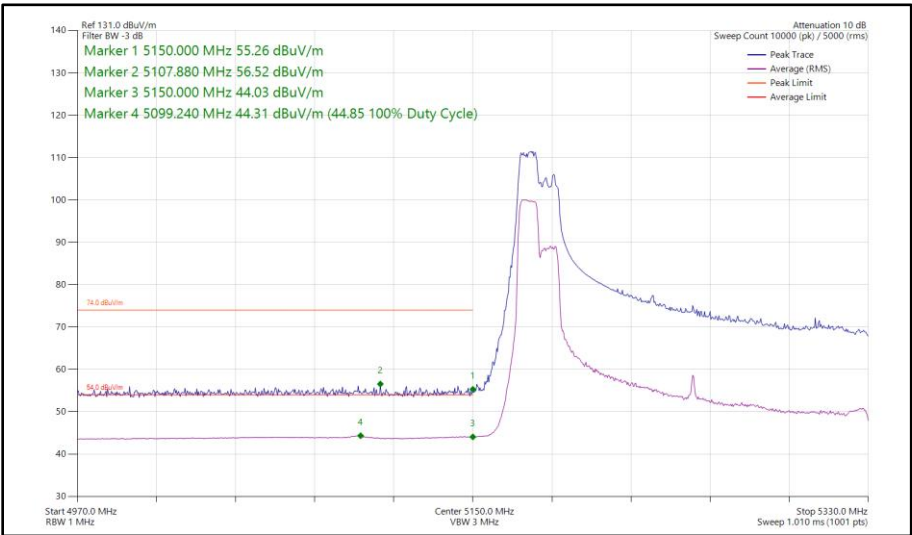
Figure 135 - 802.11ax HE160, RU 106-53P, SISO, Core 1 - 5250 MHz Band Edge Frequency 5150 MHz
