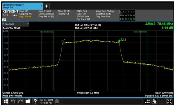
Figure 180 - 802.11ac VHT80 Minimum 99% OBW
