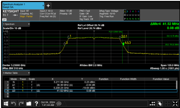
Figure 178 - 802.11n HT40 Minimum 99% OBW
