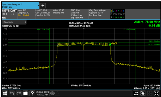
Figure 166 - 802.11ac VHT80 Minimum 6 dB EBW
