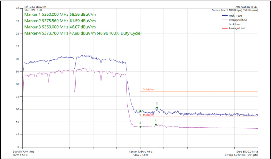
Figure 136 - 802.11ac VHT160, SISO, Core 1 - 5250 MHz Band Edge Frequency 5350 MHz
