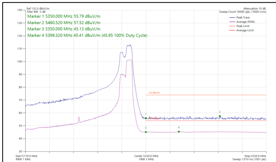
Figure 129 - 802.11ax HE160, RU 106-60S, SISO, Core 0 - 5250 MHz Band Edge Frequency 5350 MHz
