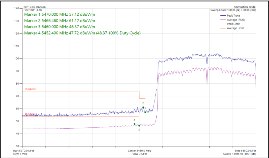
Figure 158 - 802.11ax HE160, SU, SDM, Core 0 - Core 1 - 5570 MHz Band Edge Frequency 5460 MHz
