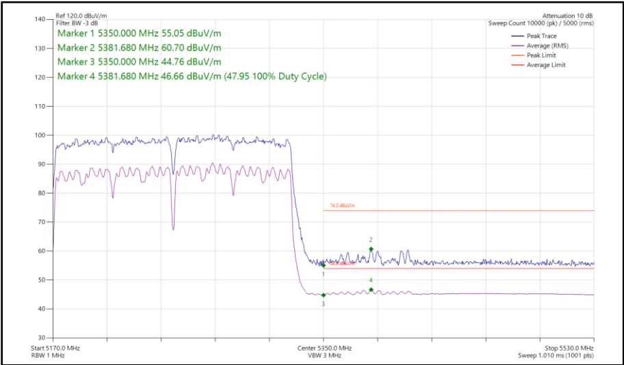
Figure 154 - 802.11ac VHT160, SDM, Core 0 - Core 1 - 5250 MHz Band Edge Frequency 5350 MHz
