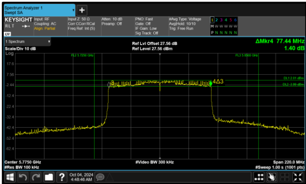
Figure 172 - 802.11ax HE80 SU Minimum 6 dB EBW
