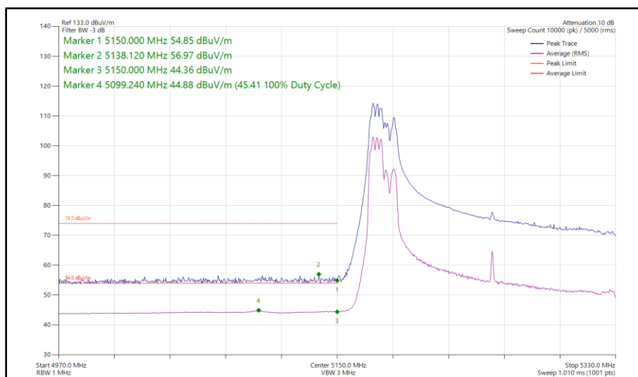
Figure 144 - 802.11ax HE160, RU 106-53P, CDD, Core 0 - Core 1 - 5250 MHz Band Edge Frequency 5150 MHz
