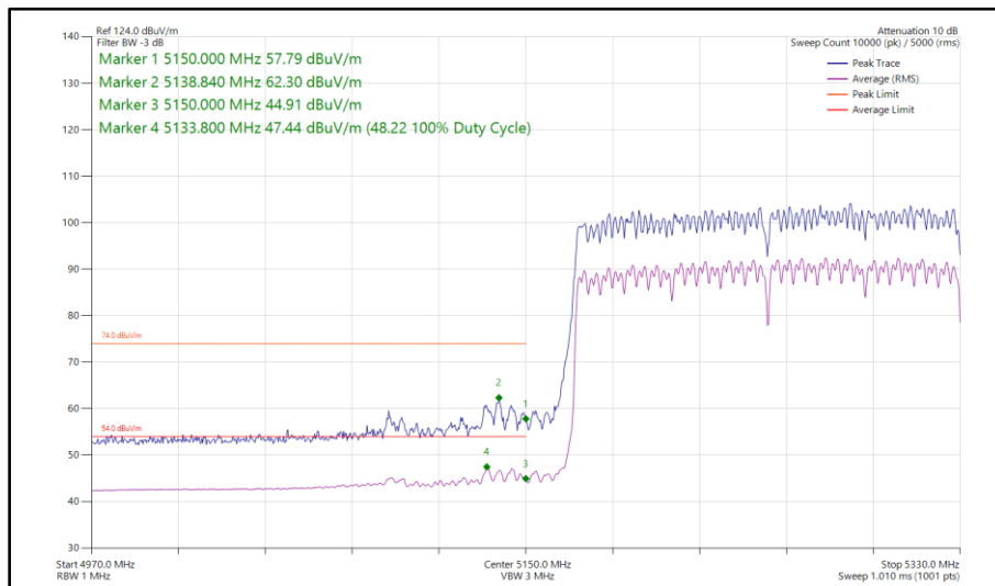
Figure 143 - 802.11ax HE160, SU, CDD, Core 0 - Core 1 - 5250 MHz Band Edge Frequency 5150 MHz
