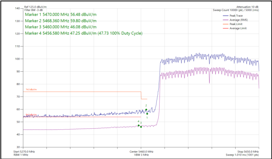
Figure 149 - 802.11ax HE160, SU, CDD, Core 0 - Core 1 - 5570 MHz Band Edge Frequency 5460 MHz
