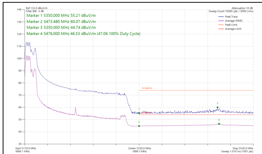
Figure 156 - 802.11ax HE160, RU 106-53P, SDM, Core 0 - Core 1 - 5250 MHz Band Edge Frequency 5350 MHz
