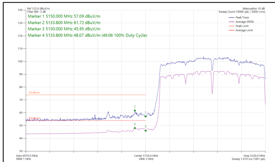
Figure 124 - 802.11ac VHT160, SISO, Core 0 - 5250 MHz Band Edge Frequency 5150 MHz
