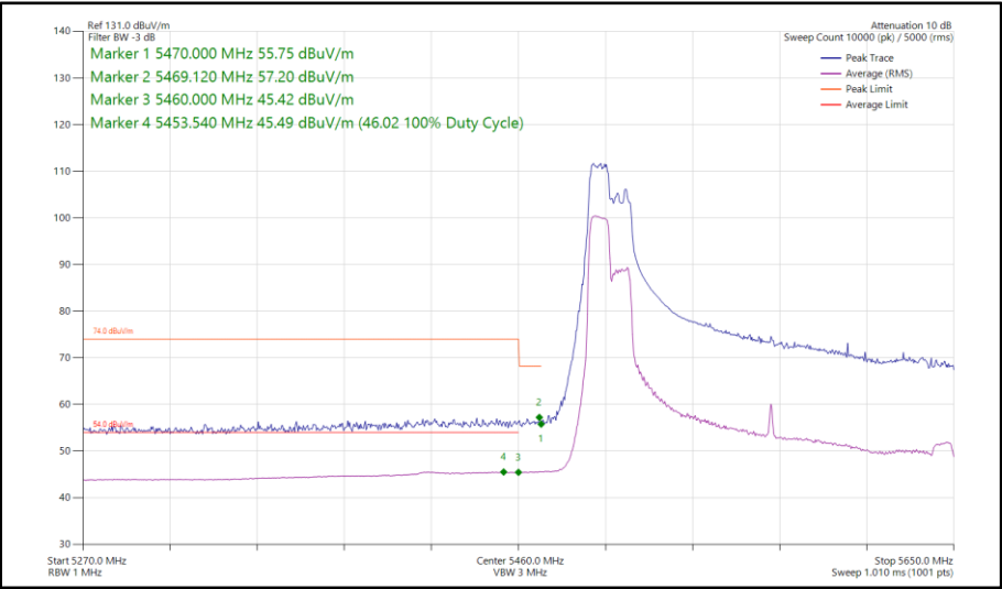
Figure 141 - 802.11ax HE160, RU 106-53P, SISO, Core 1 - 5570 MHz Band Edge Frequency 5460 MHz
