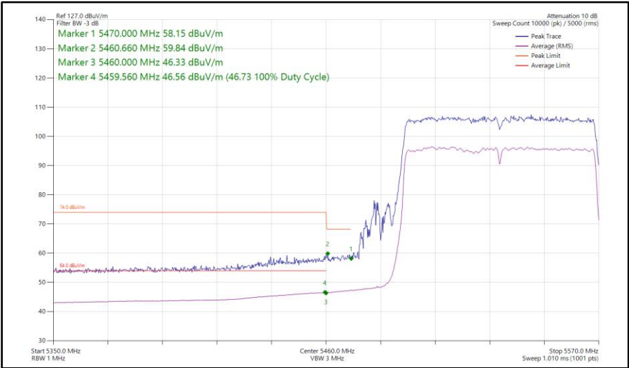
Figure 123 - 802.11ac VHT80, TxBF, Core 0 - Core 1 - 5530 MHz Band Edge Frequency 5460 MHz
