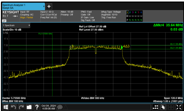
Figure 164 - 802.11n HT40 Minimum 6 dB EBW
