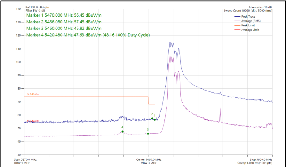
Figure 150 - 802.11ax HE160, RU 106-53P, CDD, Core 0 - Core 1 - 5570 MHz Band Edge Frequency 5460 MHz
