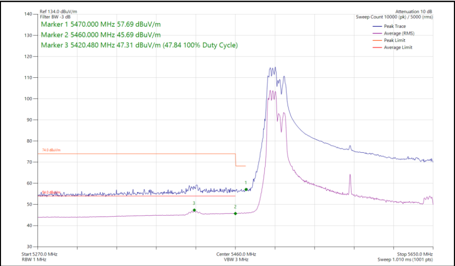
Figure 159 - 802.11ax HE160, RU 106-53P, SDM, Core 0 - Core 1 - 5570 MHz Band Edge Frequency 5460 MHz
