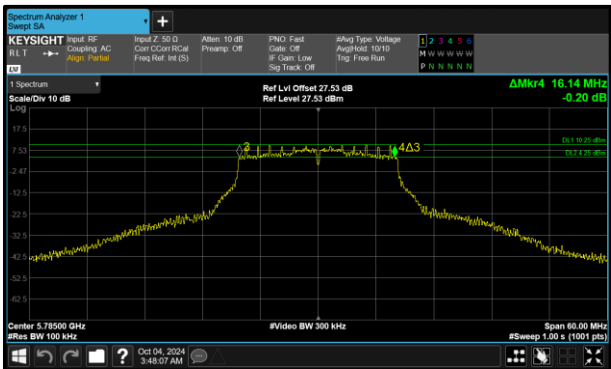
Figure 160 - 802.11a Minimum 6 dB EBW
