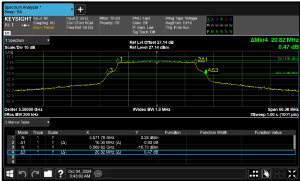
Figure 174 - 802.11a Minimum 99% OBW
