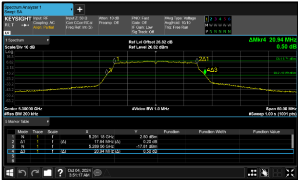
Figure 176 - 802.11n HT20 Minimum 99% OBW
