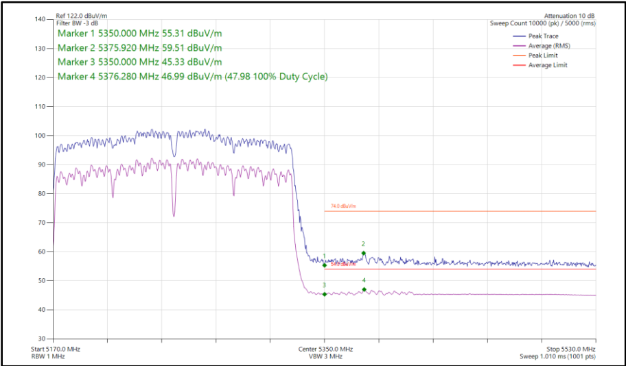
Figure 145 - 802.11ac VHT160, CDD, Core 0 - Core 1 - 5250 MHz Band Edge Frequency 5350 MHz
