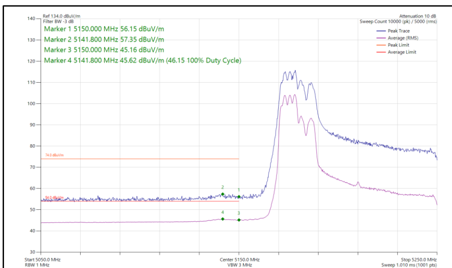
Figure 105 - 802.11ax HE80, RU 106-53, CDD, Core 0 - Core 1 - 5210 MHz Band Edge Frequency 5150 MHz
