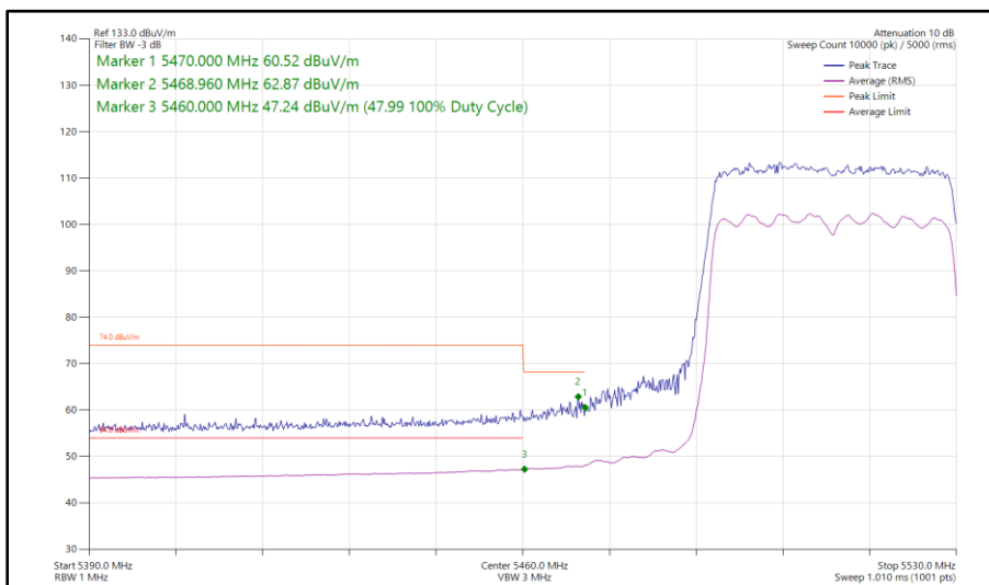
Figure 80 - 802.11ax HE40, SU, SDM, Core 0 - Core 1 - 5510 MHz Band Edge Frequency 5460 MHz
