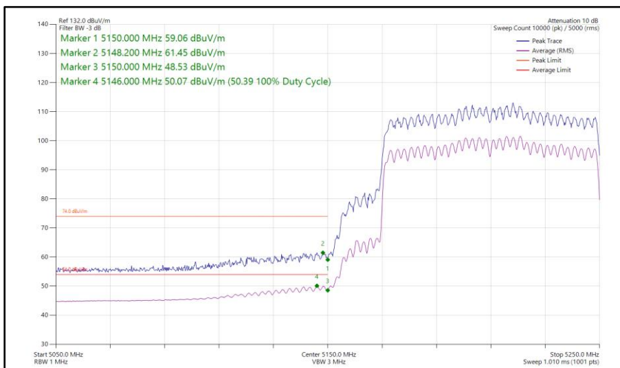
Figure 104 - 802.11ax HE80, SU, CDD, Core 0 - Core 1 - 5210 MHz Band Edge Frequency 5150 MHz
