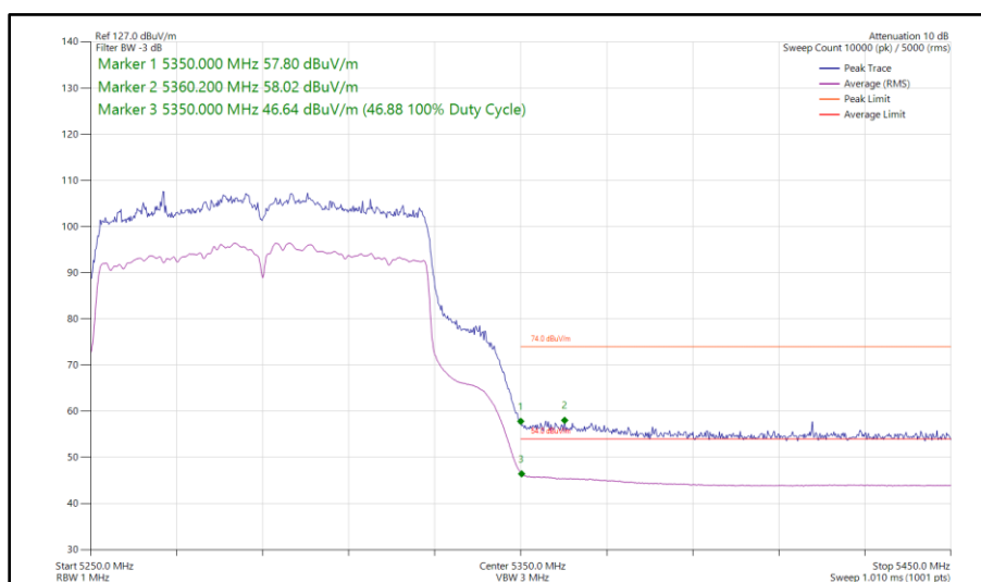
Figure 122 - 802.11ac VHT80, TxBF, Core 0 - Core 1 - 5290 MHz Band Edge Frequency 5350 MHz
