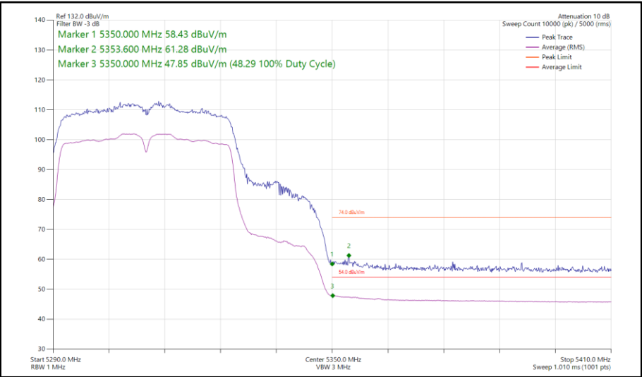
Figure 58 - 802.11n HT40, SISO, Core 1 - 5310 MHz Band Edge Frequency 5350 MHz
