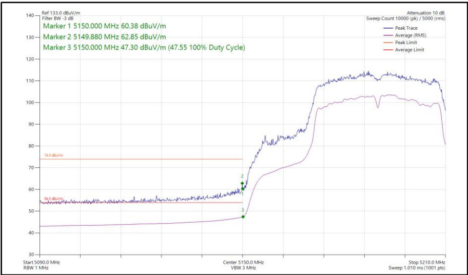
Figure 82 - 802.11ac VHT40, TxBF, Core 0 - Core 1 - 5190 MHz Band Edge Frequency 5150 MHz
