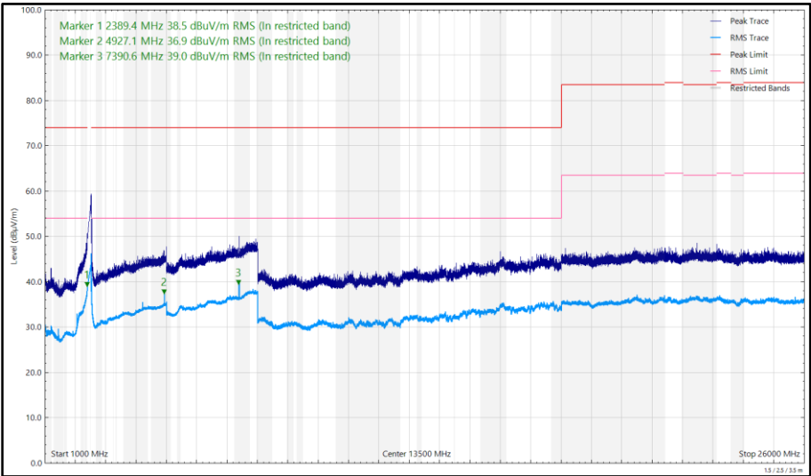
Figure 137 - 2472 MHz (CH13), HE20, RU26-0, CDD, Core 0 + Core 1, 1 GHz to 26 GHz, Vertical
