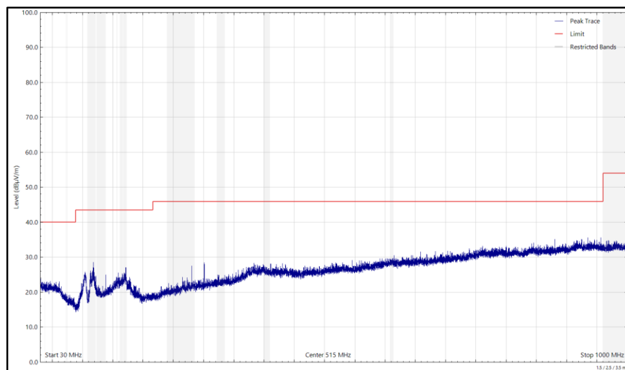
Figure 132 - 2442 MHz (CH7), HE20, RU26-0, CDD, Core 0 + Core 1, 30 MHz to 1 GHz, Horizontal (Peak)
