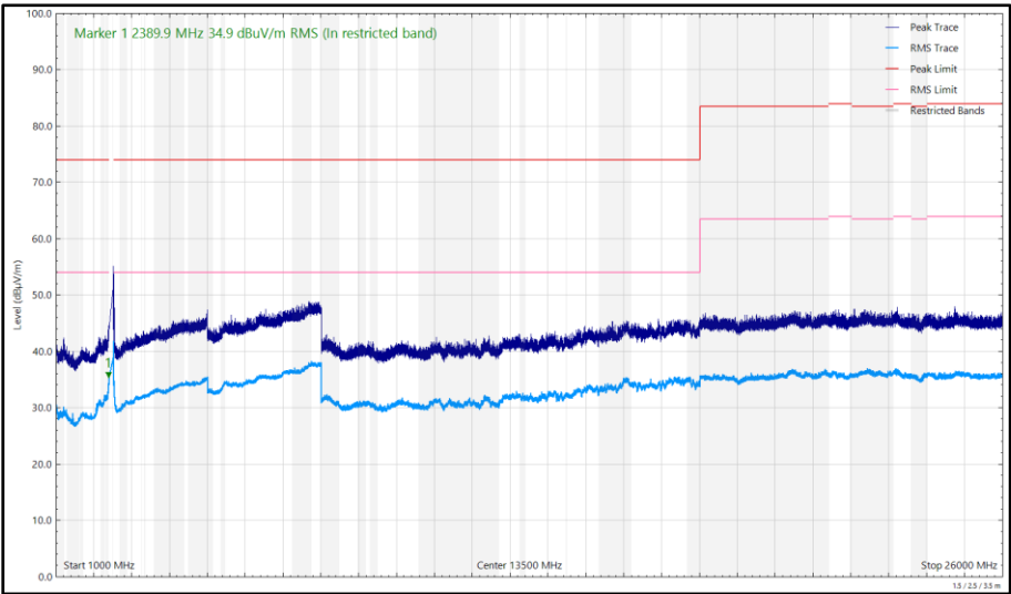
Figure 136 - 2472 MHz (CH13), HE20, RU26-0, CDD, Core 0 + Core 1, 1 GHz to 26 GHz, Horizontal
