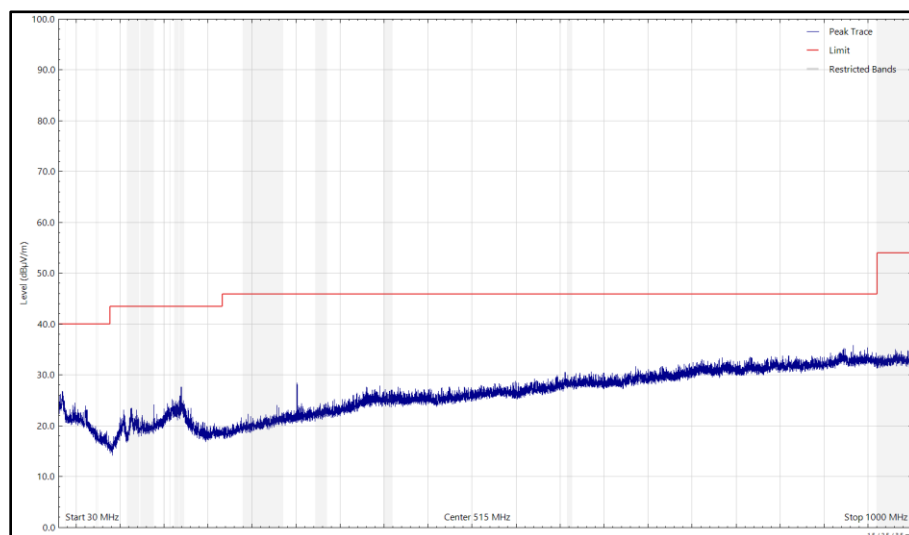
Figure 134 - 2442 MHz (CH7), HE20, RU26-0, CDD, Core 0 + Core 1, 30 MHz to 1 GHz, Vertical (Peak)
