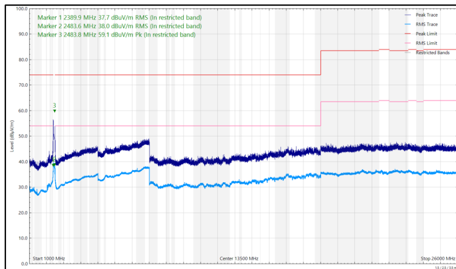
Figure 133 - 2442 MHz (CH7), HE20, RU26-0, CDD, Core 0 + Core 1, 1 GHz to 26 GHz, Horizontal
