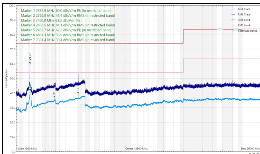
Figure 135 - 2442 MHz (CH7), HE20, RU26-0, CDD, Core 0 + Core 1, 1 GHz to 26 GHz, Vertical
