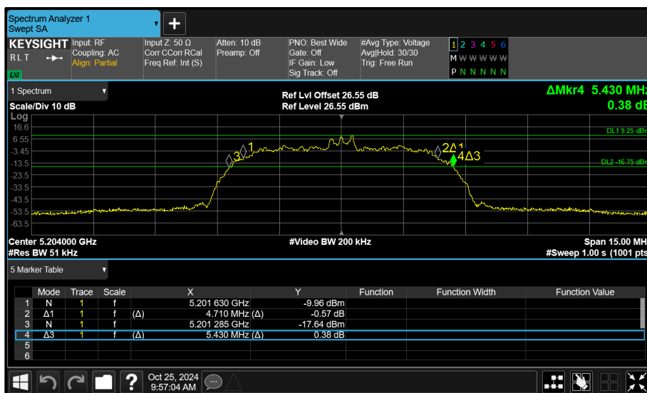
Figure 102 - Core 0 (A) 5204 MHz (CH54) 26 dB and 99% Bandwidth
