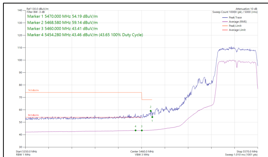
Figure 482 - 802.11ac VHT40, TxBF, Core 0 - Core 1 - 5550 MHz Band Edge Frequency 5470 MHz
