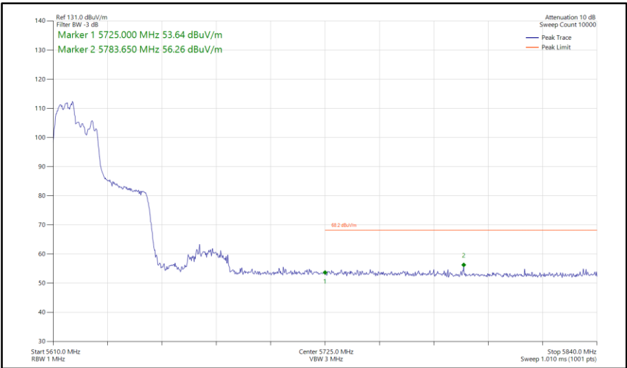
Figure 475 - 802.11ax HE40, RU 106-53, SDM, Core 0 - Core 1 - 5630 MHz Band Edge Frequency 5725 MHz
