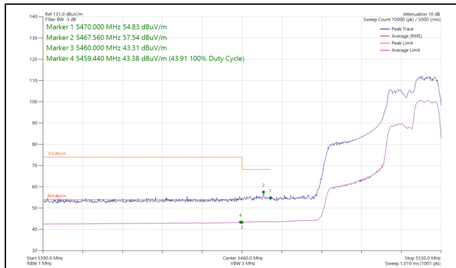
Figure 448 - 802.11ax HE40, RU 106-56, CDD, Core 0 - Core 1 - 5510 MHz Band Edge Frequency 5470 MHz
