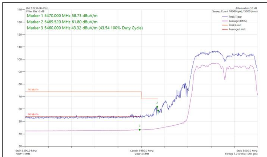
Figure 481 - 802.11ac VHT40, TxBF, Core 0 - Core 1 - 5510 MHz Band Edge Frequency 5470 MHz
