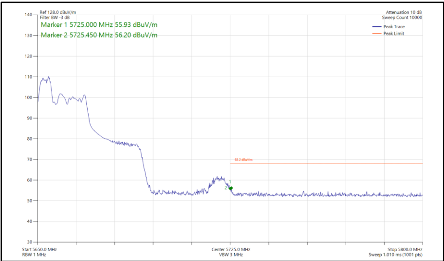
Figure 459 - 802.11ax HE40, RU 52-37, CDD, Core 0 - Core 1 - 5670 MHz Band Edge Frequency 5725 MHz
