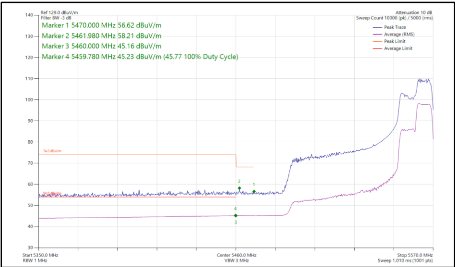
Figure 489 - 802.11ax HE80, RU 106-60, SISO, Core 0 - 5530 MHz Band Edge Frequency 5470 MHz
