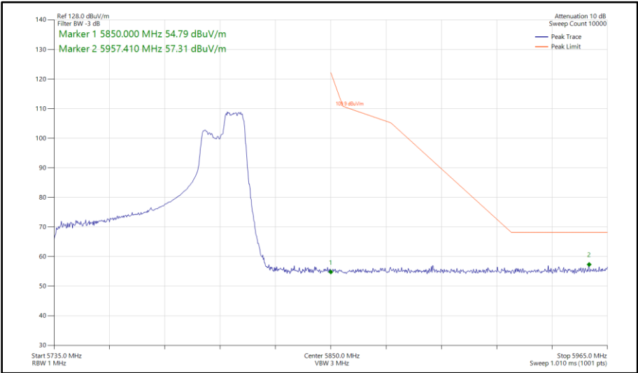
Figure 510 - 802.11ax HE80, RU 106-60, SISO, Core 1 - 5775 MHz Band Edge Frequency 5850 MHz
