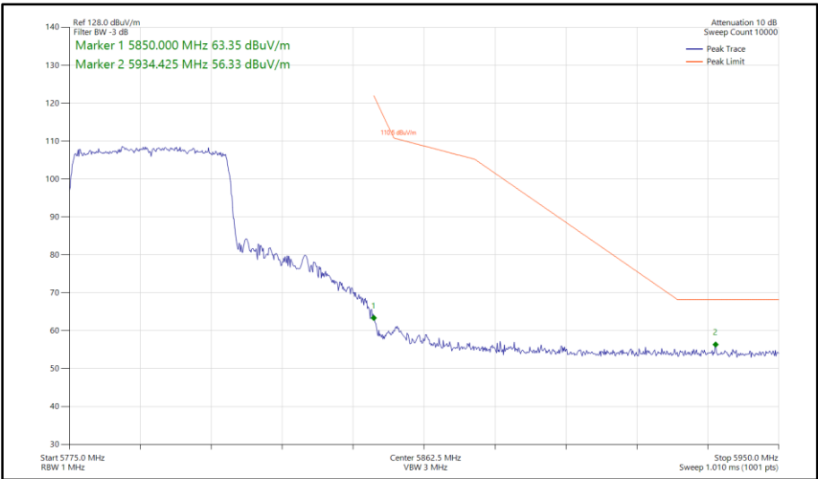
Figure 443 - 802.11ax HE40, SU, SISO, Core 1 - 5795 MHz Band Edge Frequency 5850 MHz
