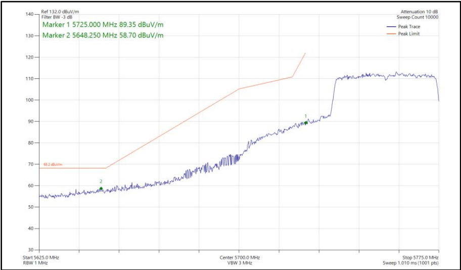
Figure 470 - 802.11ax HE40, SU, SDM, Core 0 - Core 1 - 5755 MHz Band Edge Frequency 5725 MHz
