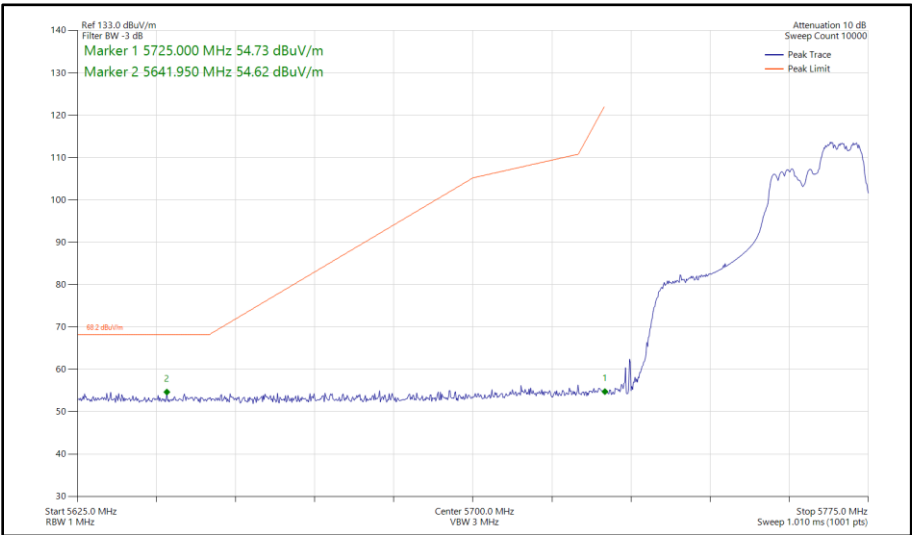
Figure 453 - 802.11ax HE40, RU 106-56, CDD, Core 0 - Core 1 - 5755 MHz Band Edge Frequency 5725 MHz
