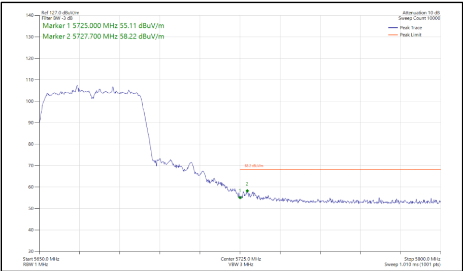
Figure 473 - 802.11n HT40, SDM, Core 0 - Core 1 - 5670 MHz Band Edge Frequency 5725 MHz
