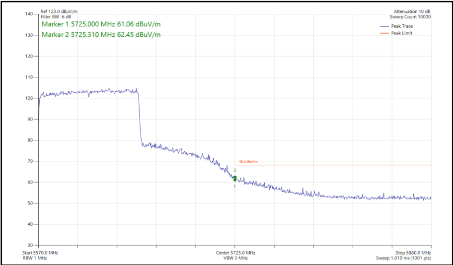
Figure 506 - 802.11ax HE80, SU, SISO, Core 1 - 5610 MHz Band Edge Frequency 5725 MHz
