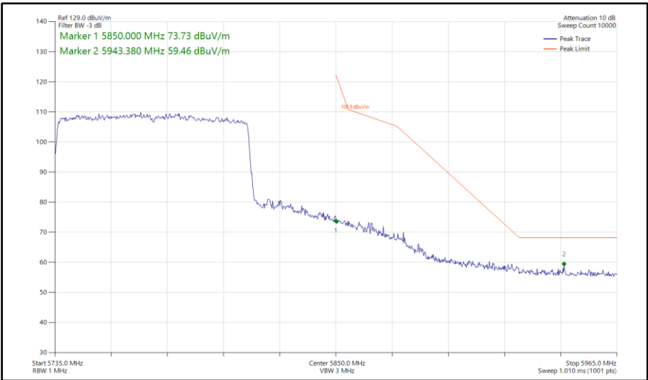
Figure 509 - 802.11ax HE80, SU, SISO, Core 1 - 5775 MHz Band Edge Frequency 5850 MHz
