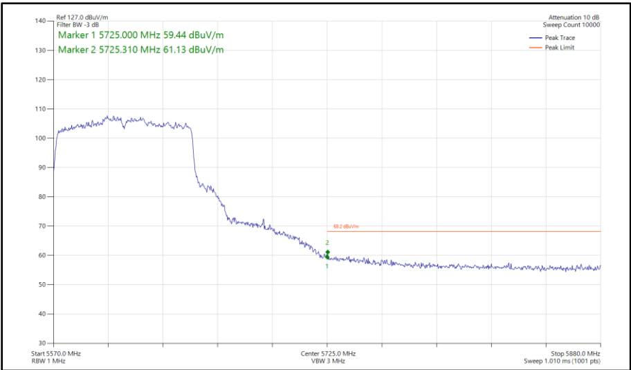
Figure 505 - 802.11ac VHT80, SISO, Core 1 - 5610 MHz Band Edge Frequency 5725 MHz
