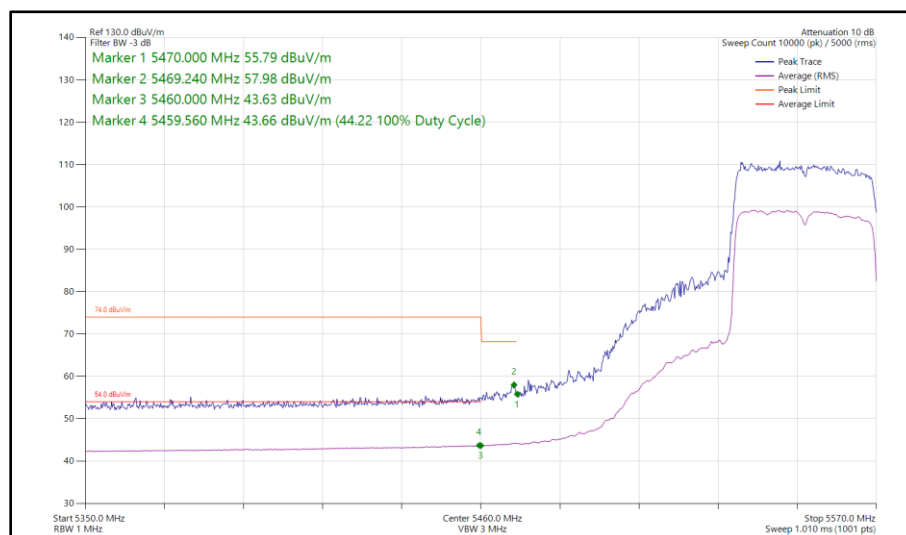
Figure 449 - 802.11ax HE40, SU, CDD, Core 0 - Core 1 - 5550 MHz Band Edge Frequency 5470 MHz
