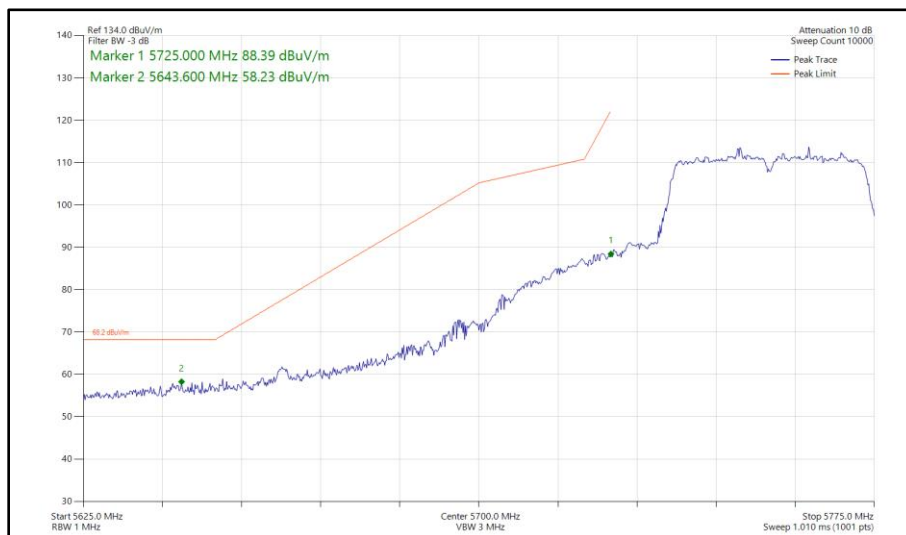
Figure 469 - 802.11n HT40, SDM, Core 0 - Core 1 - 5755 MHz Band Edge Frequency 5725 MHz
