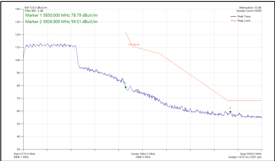
Figure 461 - 802.11ax HE40, SU, CDD, Core 0 - Core 1 - 5795 MHz Band Edge Frequency 5850 MHz
