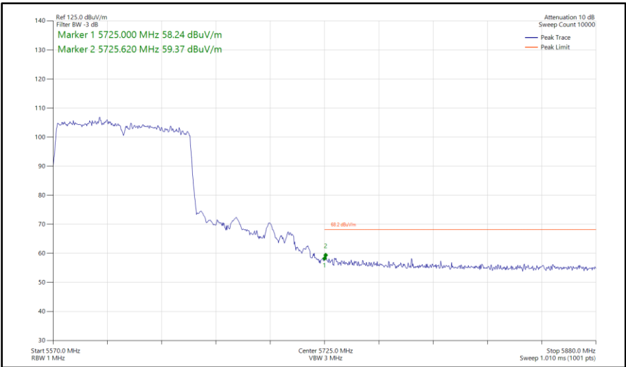
Figure 493 - 802.11ac VHT80, SISO, Core 0 - 5610 MHz Band Edge Frequency 5725 MHz
