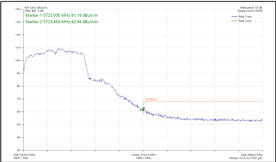
Figure 455 - 802.11n HT40, CDD, Core 0 - Core 1 - 5670 MHz Band Edge Frequency 5725 MHz
