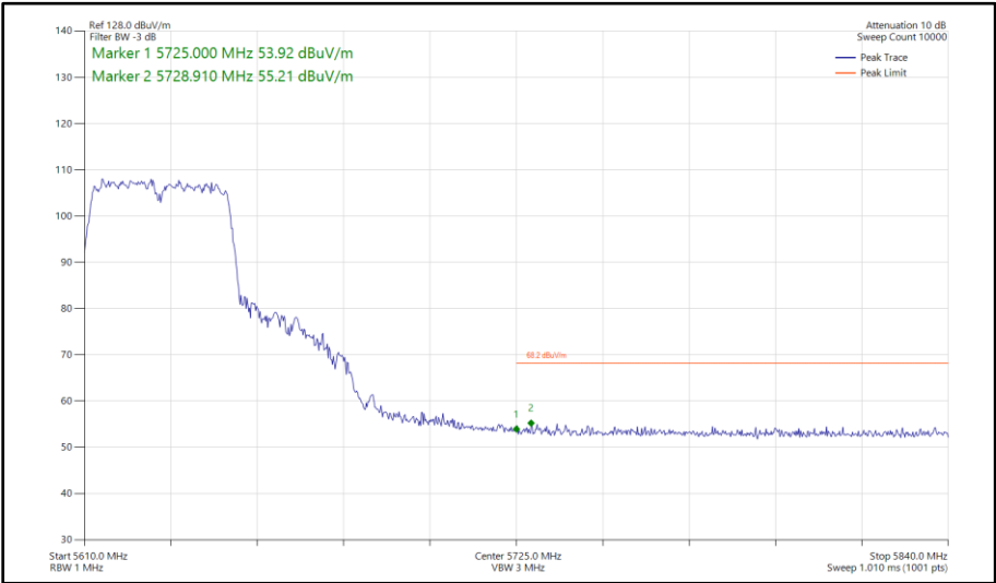
Figure 454 - 802.11n HT40, CDD, Core 0 - Core 1 - 5630 MHz Band Edge Frequency 5725 MHz
