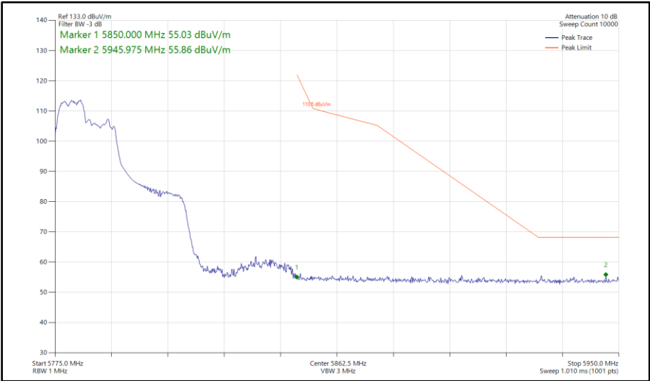
Figure 462 - 802.11ax HE40, RU 106-53, CDD, Core 0 - Core 1 - 5795 MHz Band Edge Frequency 5850 MHz
