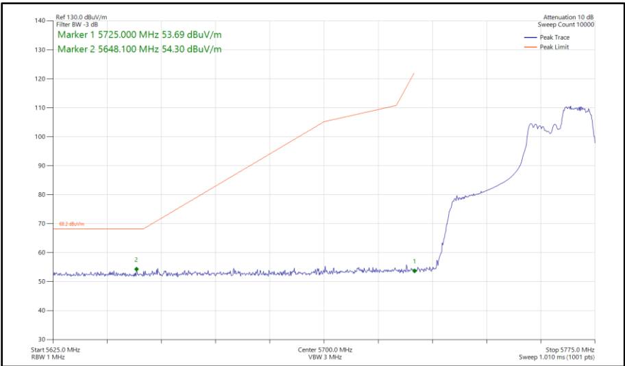
Figure 435 - 802.11ax HE40, RU 106-56, SISO, Core 1 - 5755 MHz Band Edge Frequency 5725 MHz
