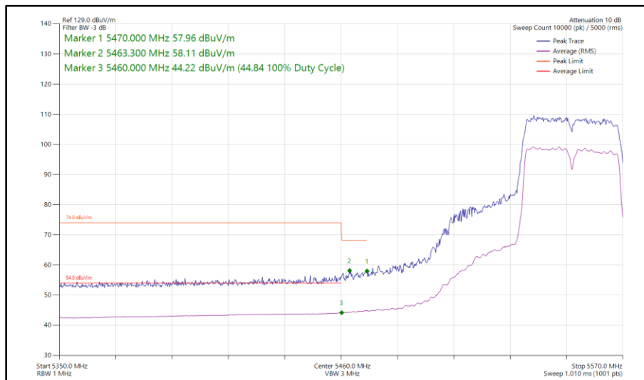
Figure 446 - 802.11n HT40, CDD, Core 0 - Core 1 - 5550 MHz Band Edge Frequency 5470 MHz
