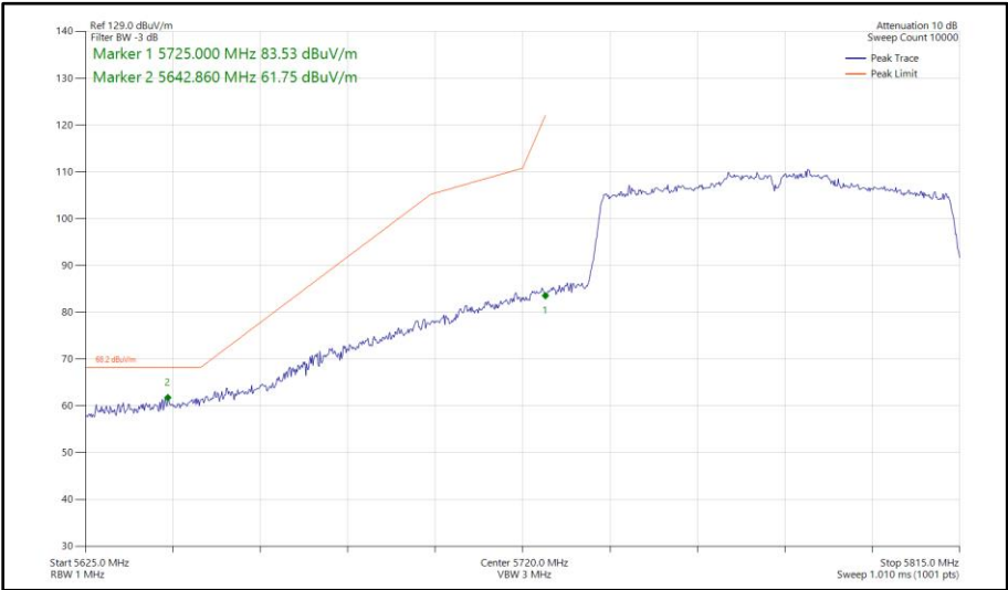
Figure 490 - 802.11ac VHT80, SISO, Core 0 - 5775 MHz Band Edge Frequency 5725 MHz
