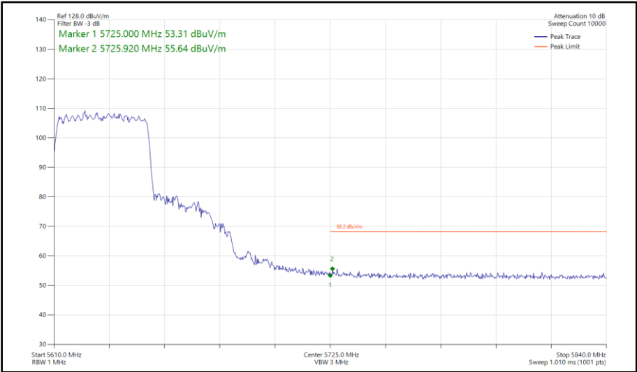
Figure 456 - 802.11ax HE40, SU, CDD, Core 0 - Core 1 - 5630 MHz Band Edge Frequency 5725 MHz
