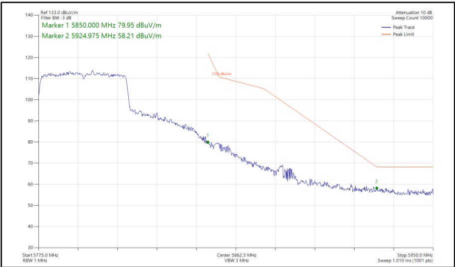
Figure 479 - 802.11ax HE40, SU, SDM, Core 0 - Core 1 - 5795 MHz Band Edge Frequency 5850 MHz
