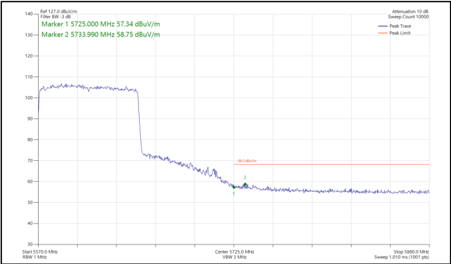
Figure 494 - 802.11ax HE80, SU, SISO, Core 0 - 5610 MHz Band Edge Frequency 5725 MHz
