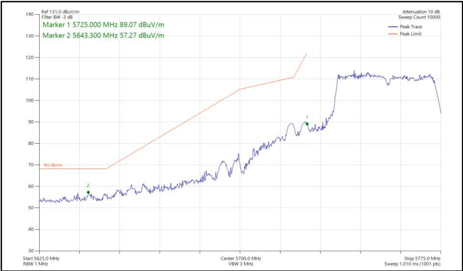
Figure 483 - 802.11ac VHT40, TxBF, Core 0 - Core 1 - 5755 MHz Band Edge Frequency 5725 MHz
