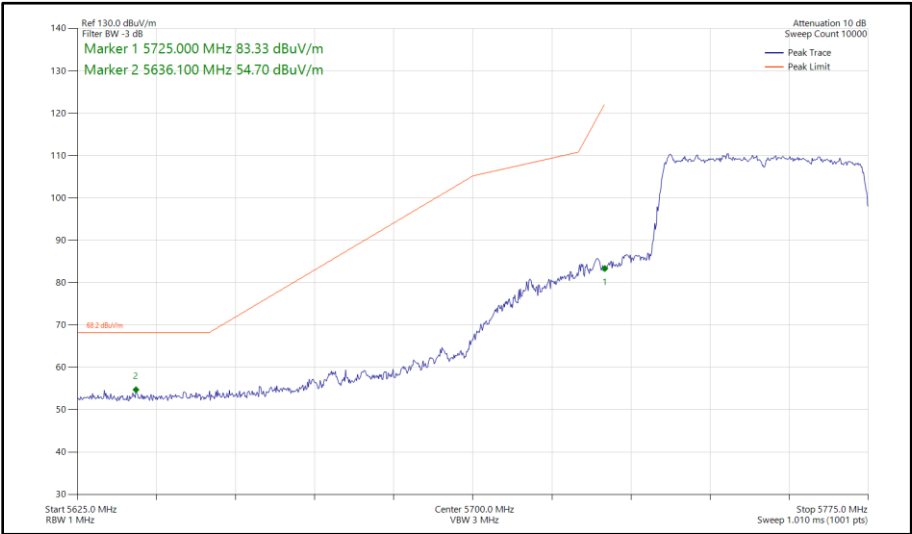
Figure 434 - 802.11ax HE40, SU, SISO, Core 1 - 5755 MHz Band Edge Frequency 5725 MHz
