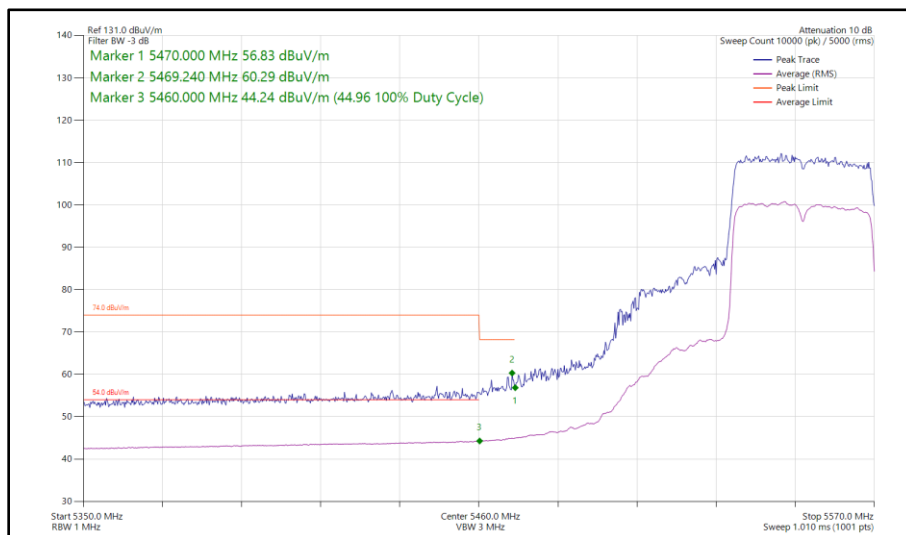
Figure 467 - 802.11ax HE40, SU, SDM, Core 0 - Core 1 - 5550 MHz Band Edge Frequency 5470 MHz
