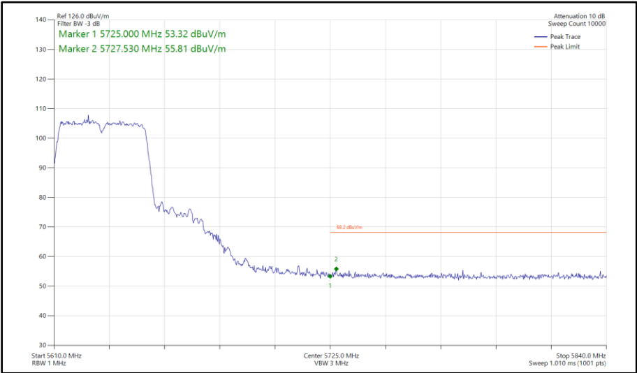
Figure 472 - 802.11n HT40, SDM, Core 0 - Core 1 - 5630 MHz Band Edge Frequency 5725 MHz
