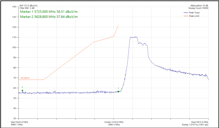
Figure 504 - 802.11ax HE80, RU 106-53, SISO, Core 1 - 5775 MHz Band Edge Frequency 5725 MHz
