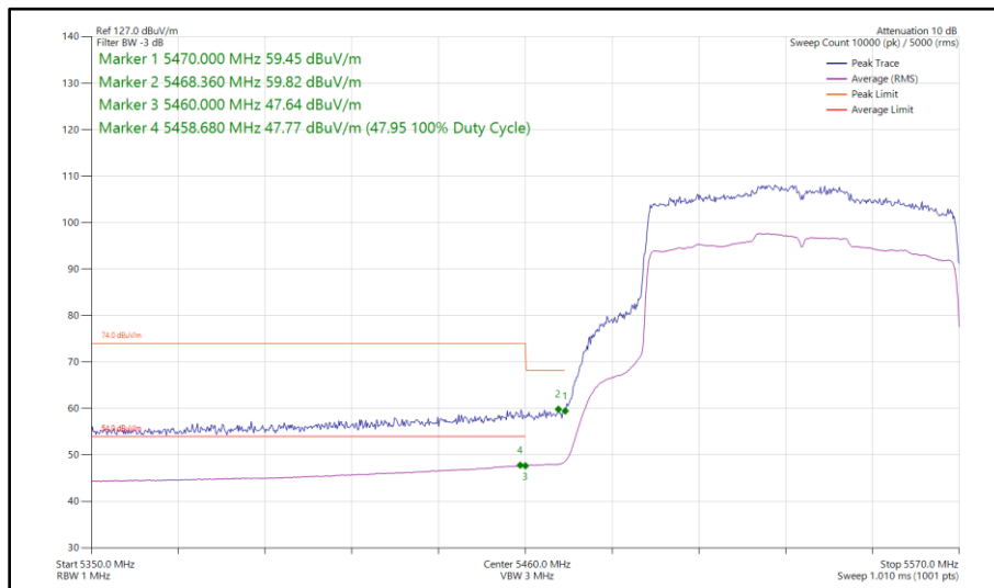
Figure 500 - 802.11ax HE80, SU, SISO, Core 1 - 5530 MHz Band Edge Frequency 5470 MHz
