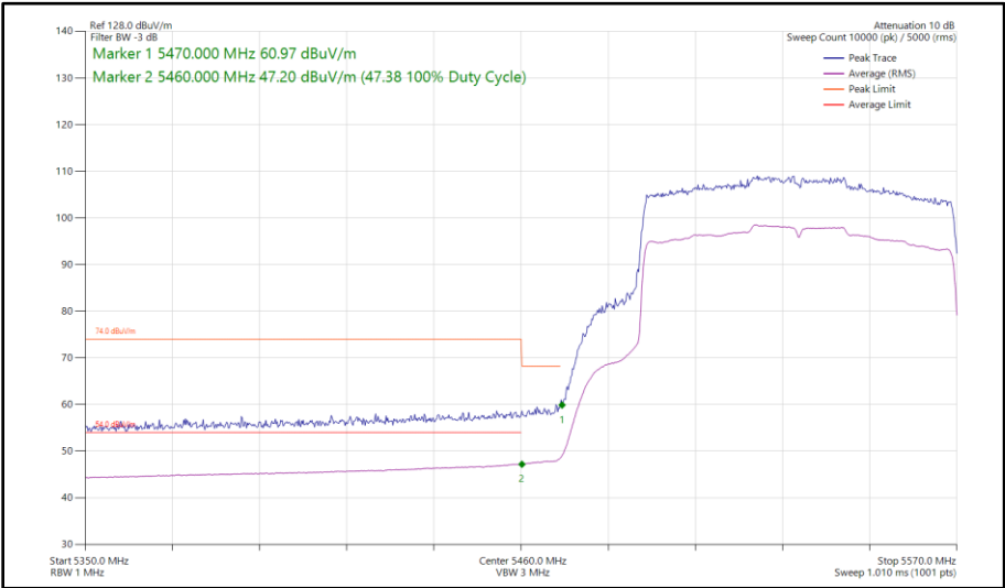
Figure 488 - 802.11ax HE80, SU, SISO, Core 0 - 5530 MHz Band Edge Frequency 5470 MHz
