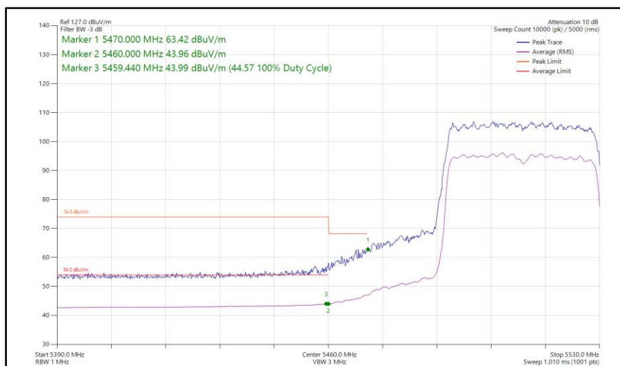
Figure 447 - 802.11ax HE40, SU, CDD, Core 0 - Core 1 - 5510 MHz Band Edge Frequency 5470 MHz
