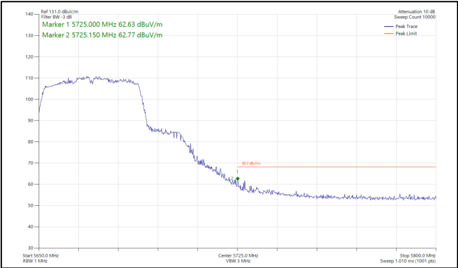
Figure 485 - 802.11ac VHT40, TxBF, Core 0 - Core 1 - 5670 MHz Band Edge Frequency 5725 MHz
