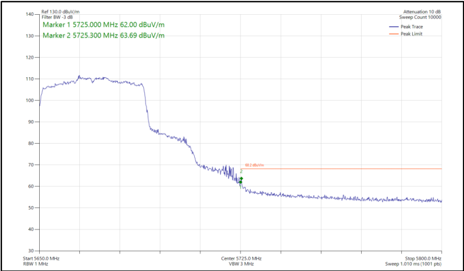
Figure 476 - 802.11ax HE40, SU, SDM, Core 0 - Core 1 - 5670 MHz Band Edge Frequency 5725 MHz
