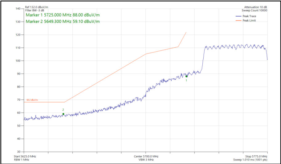
Figure 452 - 802.11ax HE40, SU, CDD, Core 0 - Core 1 - 5755 MHz Band Edge Frequency 5725 MHz
