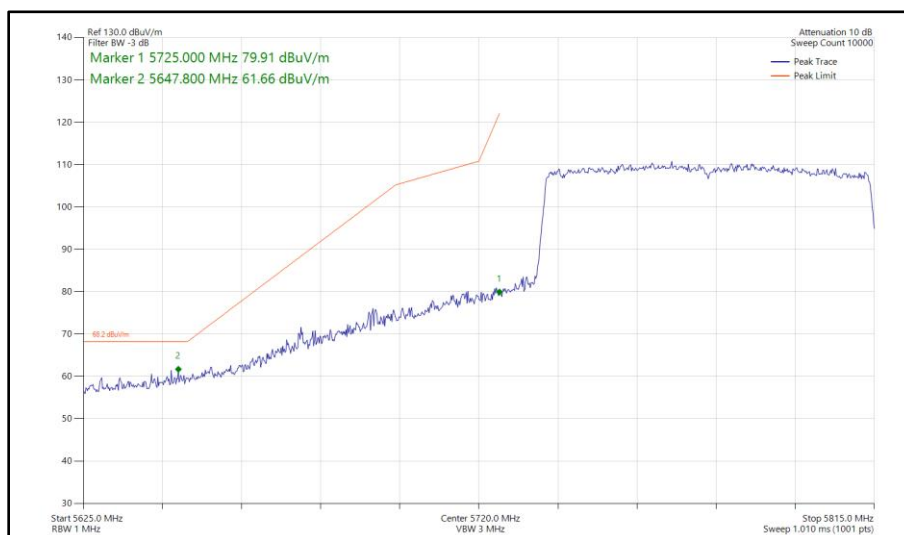
Figure 503 - 802.11ax HE80, SU, SISO, Core 1 - 5775 MHz Band Edge Frequency 5725 MHz
