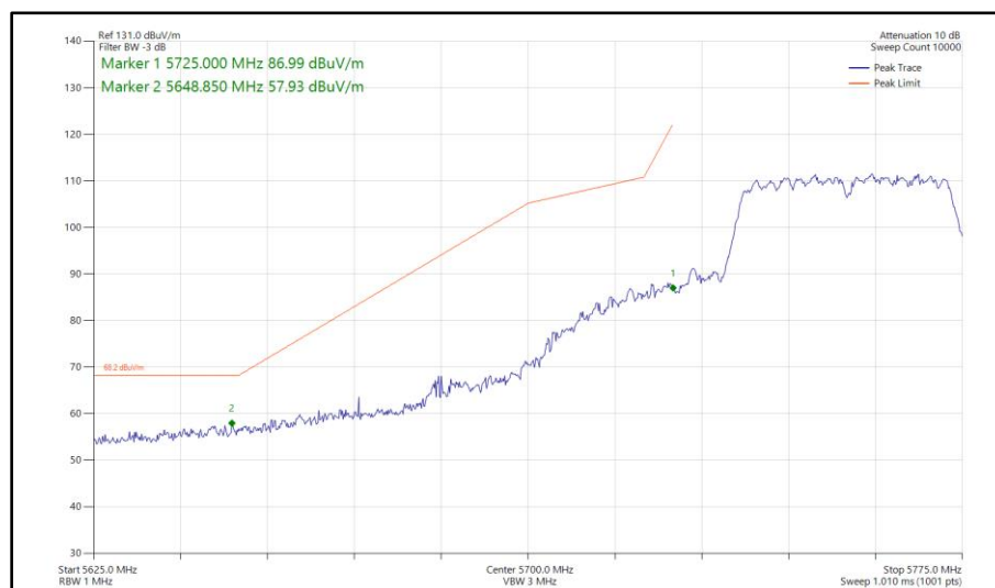
Figure 451 - 802.11n HT40, CDD, Core 0 - Core 1 - 5755 MHz Band Edge Frequency 5725 MHz
