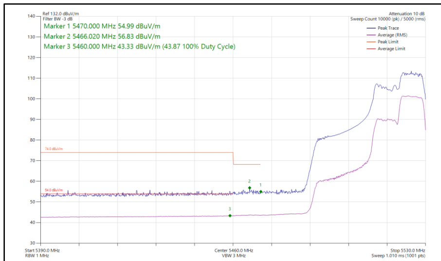
Figure 466 - 802.11ax HE40, RU 106-56, SDM, Core 0 - Core 1 - 5510 MHz Band Edge Frequency 5470 MHz
