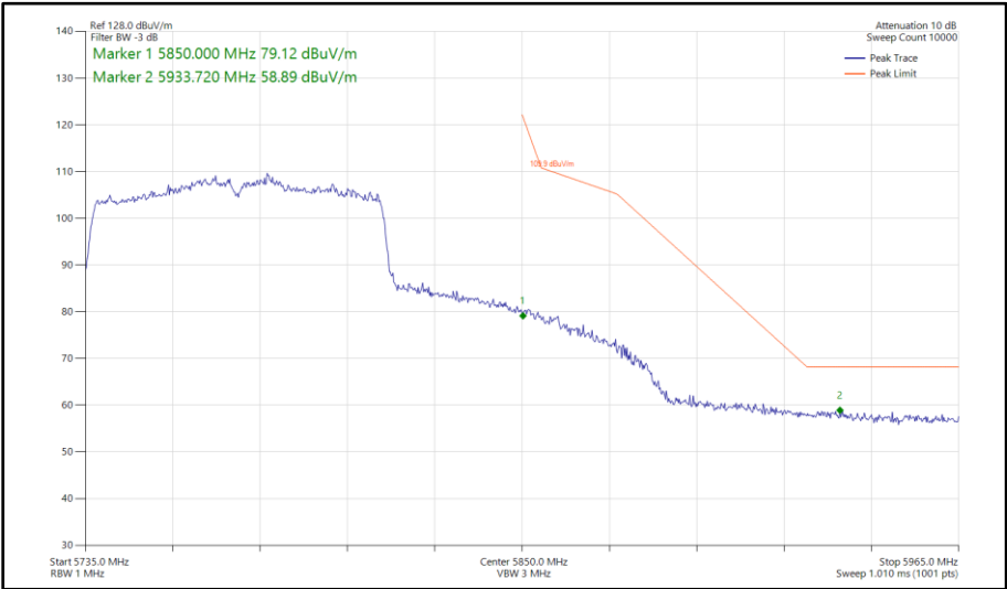
Figure 496 - 802.11ac VHT80, SISO, Core 0 - 5775 MHz Band Edge Frequency 5850 MHz
