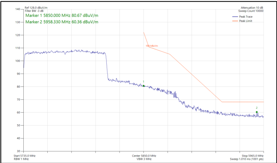
Figure 497 - 802.11ax HE80, SU, SISO, Core 0 - 5775 MHz Band Edge Frequency 5850 MHz
