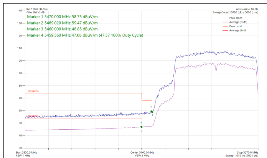
Figure 511 - 802.11ac VHT80, CDD, Core 0 - Core 1 - 5530 MHz Band Edge Frequency 5470 MHz
