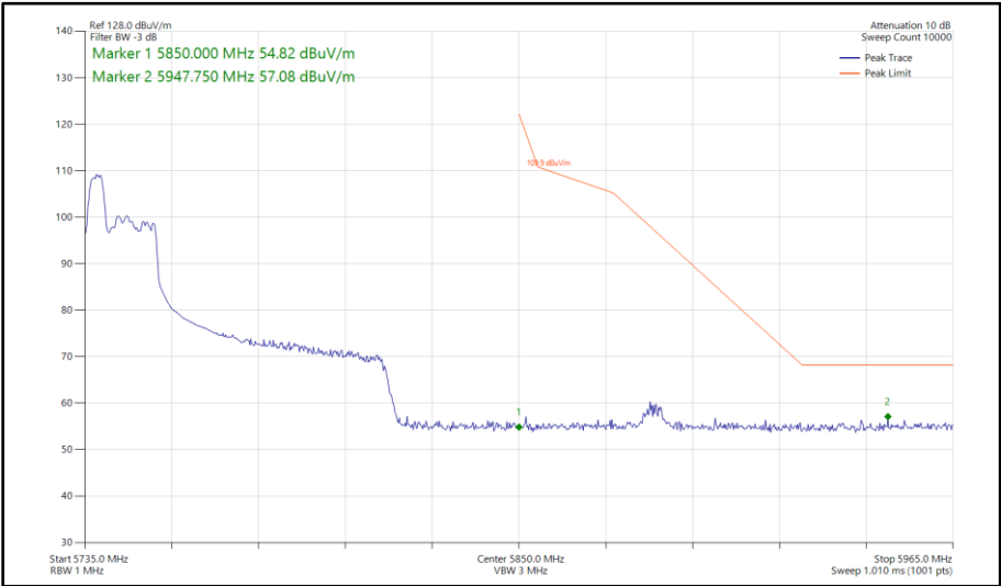
Figure 498 - 802.11ax HE80, RU 52-37, SISO, Core 0 - 5775 MHz Band Edge Frequency 5850 MHz
