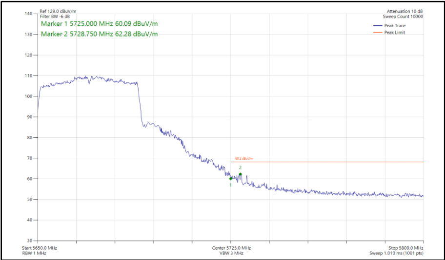
Figure 440 - 802.11ax HE40, SU, SISO, Core 1 - 5670 MHz Band Edge Frequency 5725 MHz
