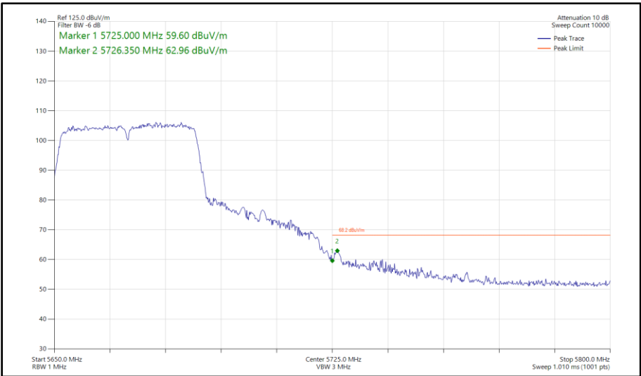
Figure 437 - 802.11n HT40, SISO, Core 1 - 5670 MHz Band Edge Frequency 5725 MHz
