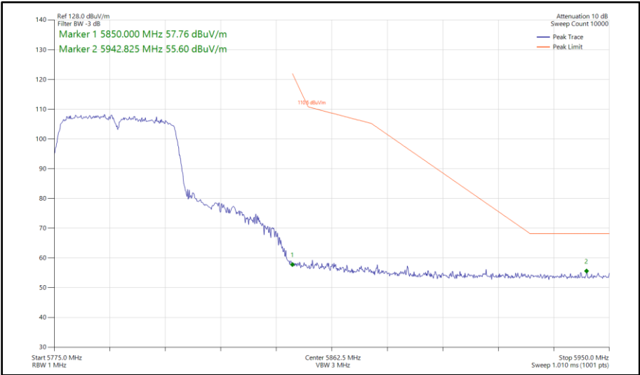
Figure 442 - 802.11n HT40, SISO, Core 1 - 5795 MHz Band Edge Frequency 5850 MHz
