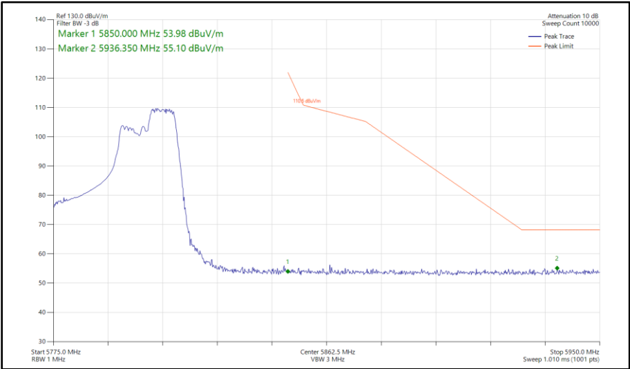
Figure 444 - 802.11ax HE40, RU 106-56, SISO, Core 1 - 5795 MHz Band Edge Frequency 5850 MHz
