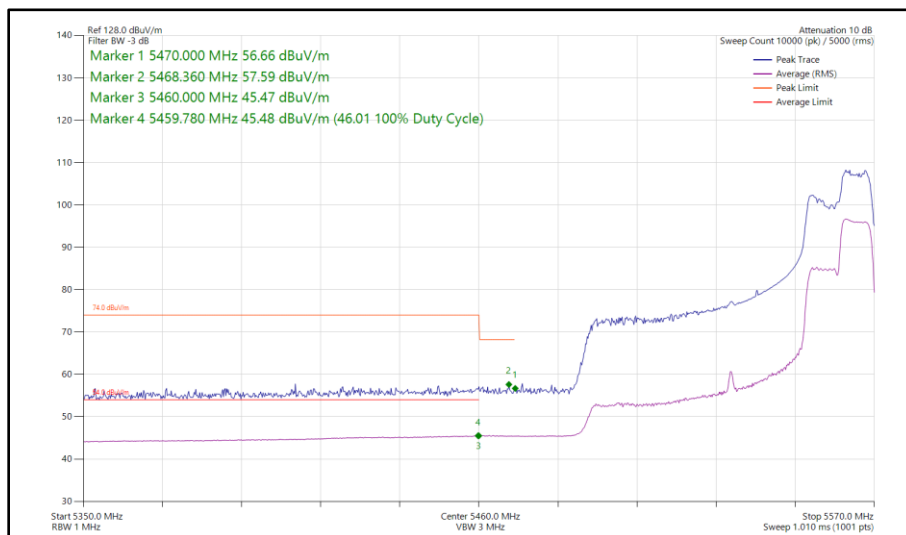
Figure 501 - 802.11ax HE80, RU 106-60, SISO, Core 1 - 5530 MHz Band Edge Frequency 5470 MHz
