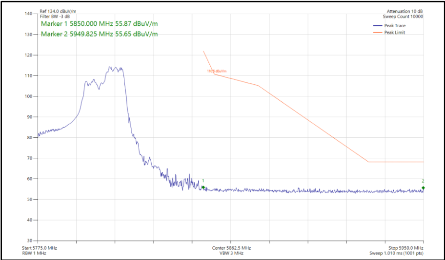
Figure 480 - 802.11ax HE40, RU 106-56, SDM, Core 0 - Core 1 - 5795 MHz Band Edge Frequency 5850 MHz
