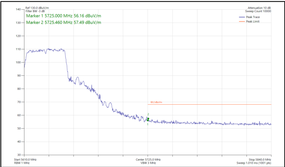
Figure 484 - 802.11ac VHT40, TxBF, Core 0 - Core 1 - 5630 MHz Band Edge Frequency 5725 MHz
