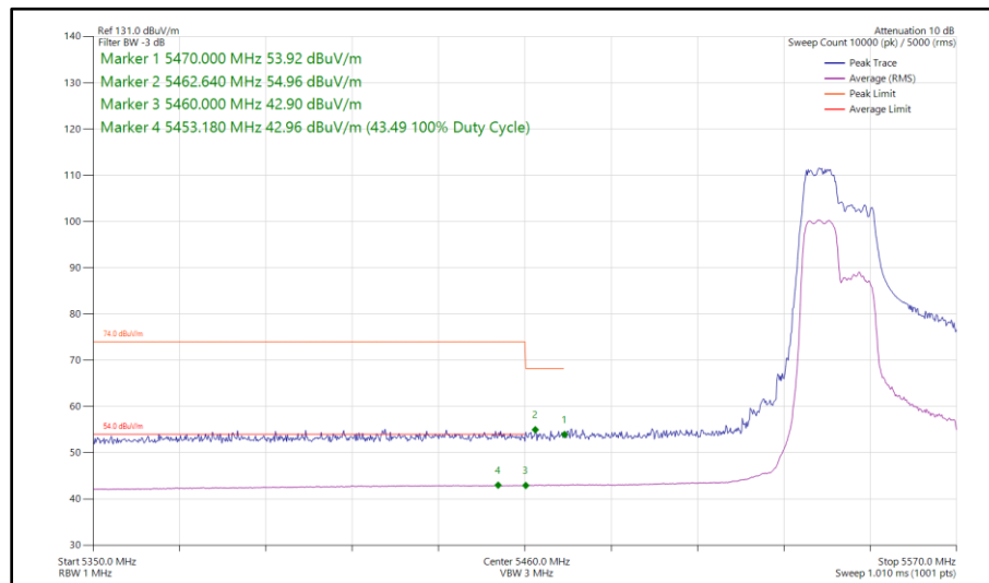
Figure 450 - 802.11ax HE40, RU 106-53, CDD, Core 0 - Core 1 - 5550 MHz Band Edge Frequency 5470 MHz
