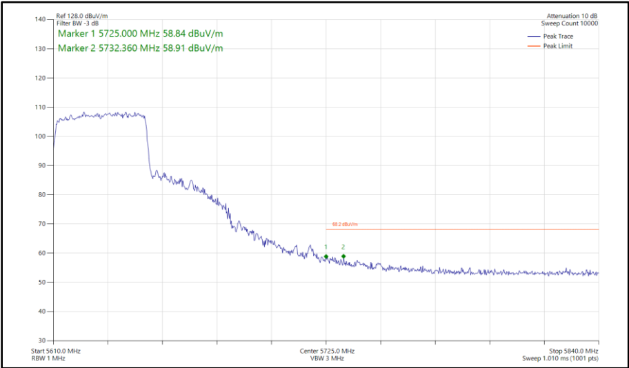
Figure 438 - 802.11ax HE40, SU, SISO, Core 1 - 5630 MHz Band Edge Frequency 5725 MHz
