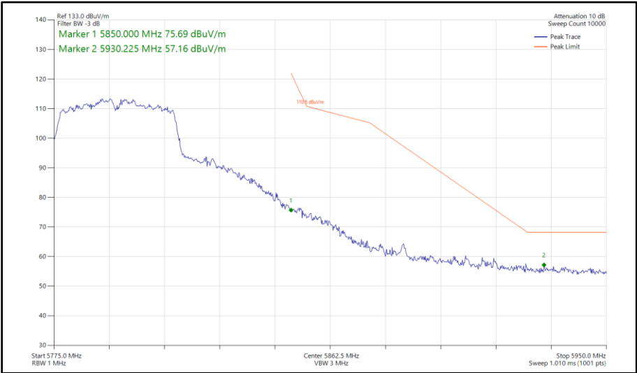
Figure 460 - 802.11n HT40, CDD, Core 0 - Core 1 - 5795 MHz Band Edge Frequency 5850 MHz
