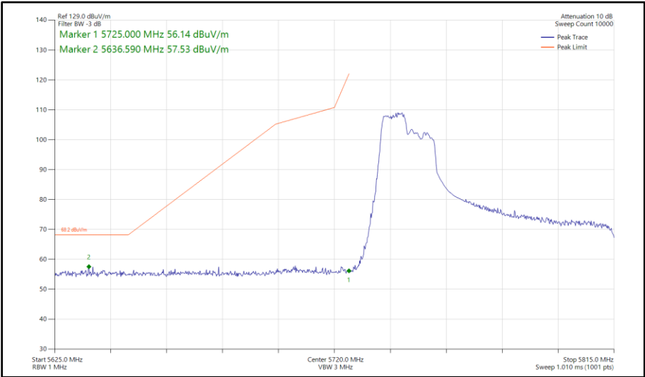
Figure 492 - 802.11ax HE80, RU 106-53, SISO, Core 0 - 5775 MHz Band Edge Frequency 5725 MHz
