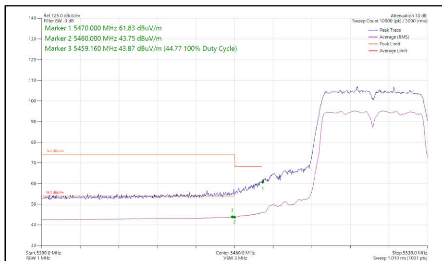
Figure 463 - 802.11n HT40, SDM, Core 0 - Core 1 - 5510 MHz Band Edge Frequency 5470 MHz
