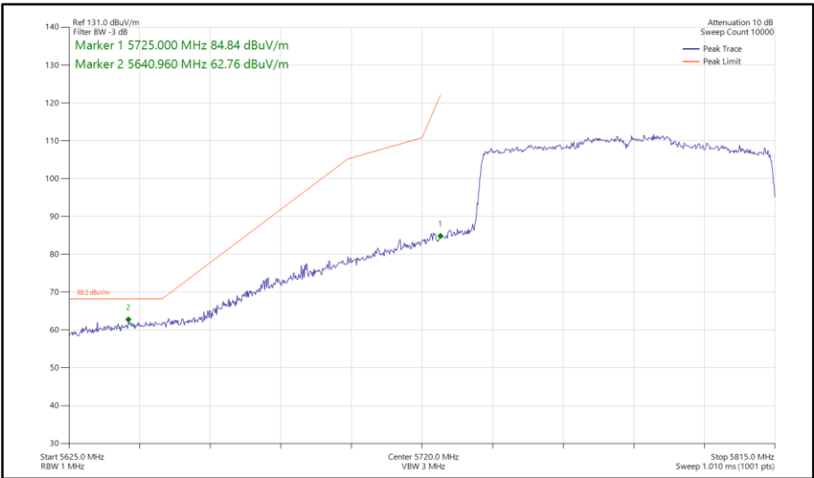
Figure 491 - 802.11ax HE80, SU, SISO, Core 0 - 5775 MHz Band Edge Frequency 5725 MHz
