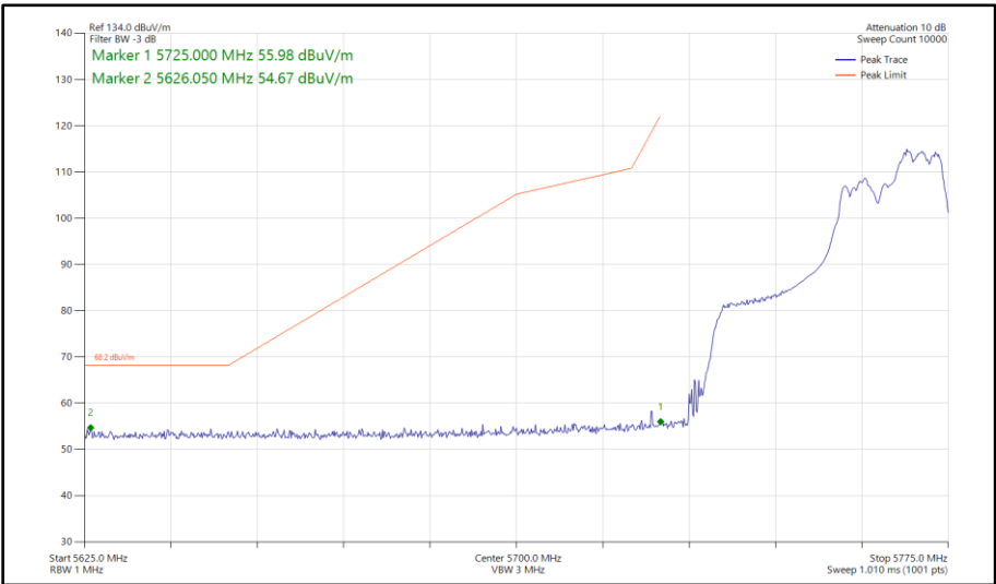
Figure 471 - 802.11ax HE40, RU 106-56, SDM, Core 0 - Core 1 - 5755 MHz Band Edge Frequency 5725 MHz
