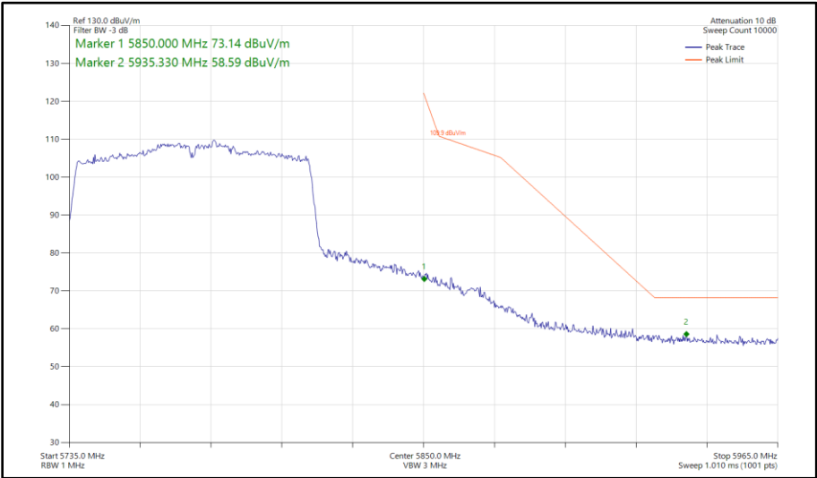
Figure 508 - 802.11ac VHT80, SISO, Core 1 - 5775 MHz Band Edge Frequency 5850 MHz
