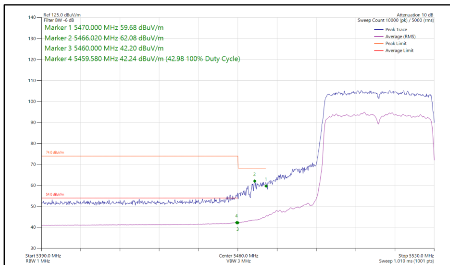
Figure 465 - 802.11ax HE40, SU, SDM, Core 0 - Core 1 - 5510 MHz Band Edge Frequency 5470 MHz
