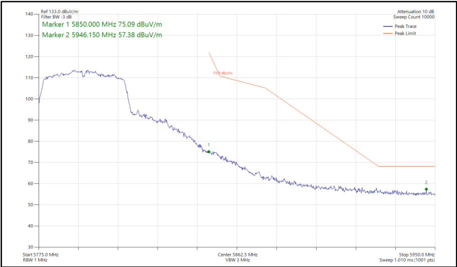
Figure 478 - 802.11n HT40, SDM, Core 0 - Core 1 - 5795 MHz Band Edge Frequency 5850 MHz
