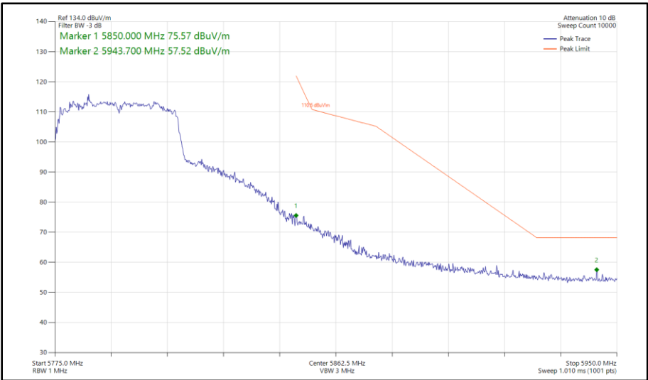
Figure 486 - 802.11ac VHT40, TxBF, Core 0 - Core 1 - 5795 MHz Band Edge Frequency 5850 MHz
