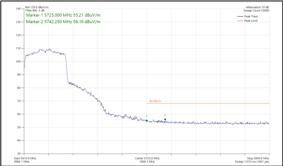
Figure 474 - 802.11ax HE40, SU, SDM, Core 0 - Core 1 - 5630 MHz Band Edge Frequency 5725 MHz
