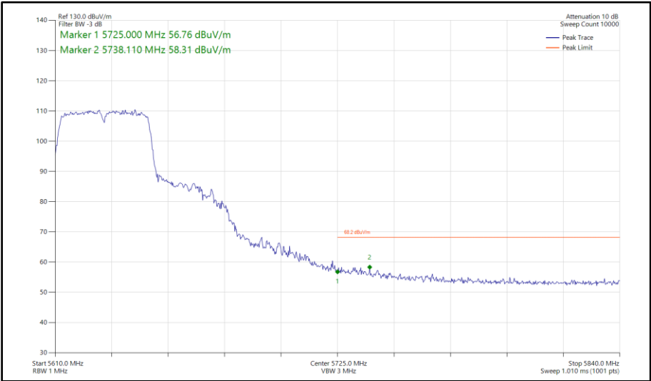
Figure 436 - 802.11n HT40, SISO, Core 1 - 5630 MHz Band Edge Frequency 5725 MHz
