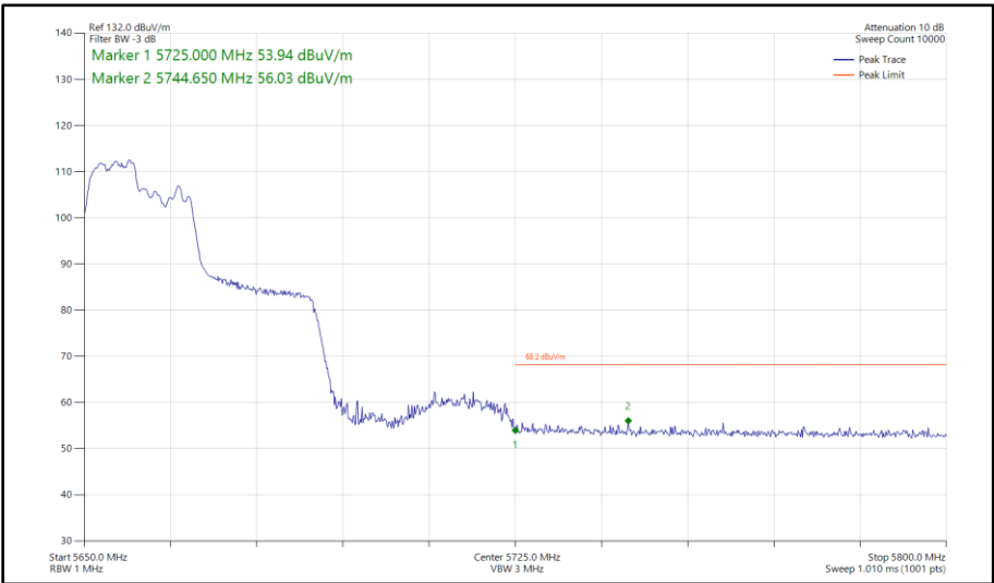
Figure 477 - 802.11ax HE40, RU 106-53, SDM, Core 0 - Core 1 - 5670 MHz Band Edge Frequency 5725 MHz
