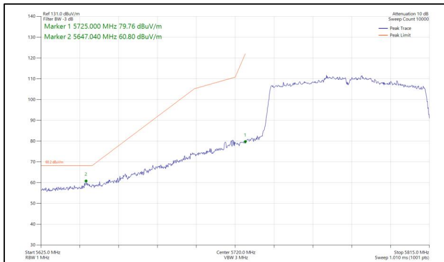
Figure 502 - 802.11ac VHT80, SISO, Core 1 - 5775 MHz Band Edge Frequency 5725 MHz
