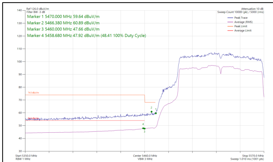
Figure 499 - 802.11ac VHT80, SISO, Core 1 - 5530 MHz Band Edge Frequency 5470 MHz
