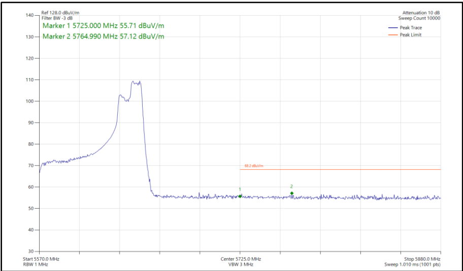
Figure 495 - 802.11ax HE80, RU 106-60, SISO, Core 0 - 5610 MHz Band Edge Frequency 5725 MHz
