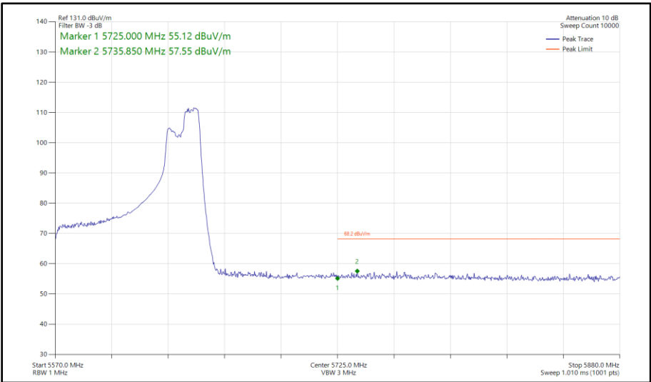
Figure 507 - 802.11ax HE80, RU 106-60, SISO, Core 1 - 5610 MHz Band Edge Frequency 5725 MHz
