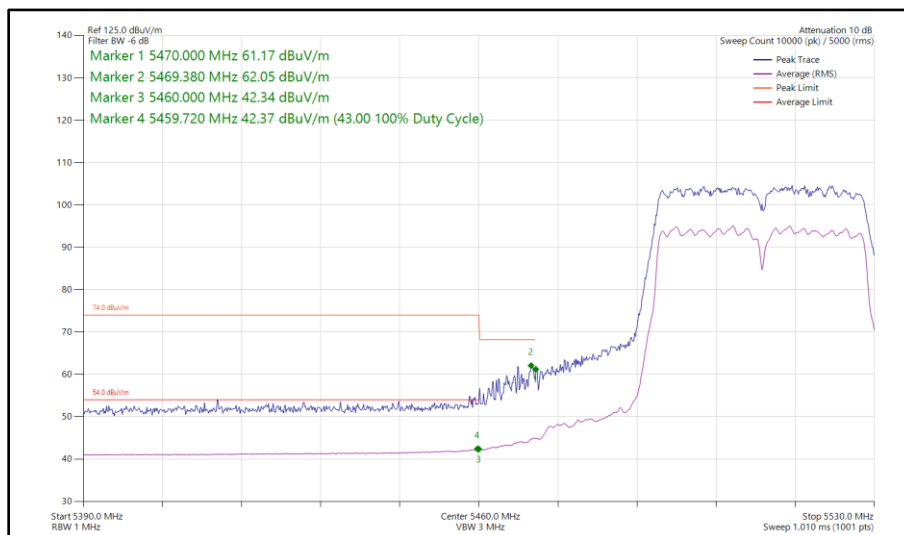
Figure 445 - 802.11n HT40, CDD, Core 0 - Core 1 - 5510 MHz Band Edge Frequency 5470 MHz
