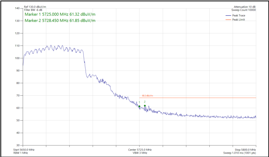
Figure 458 - 802.11ax HE40, SU, CDD, Core 0 - Core 1 - 5670 MHz Band Edge Frequency 5725 MHz
