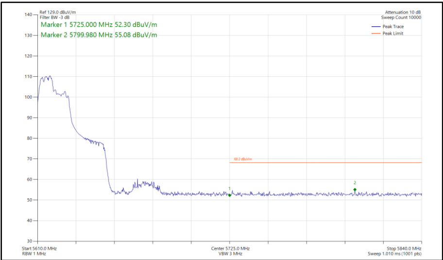
Figure 457 - 802.11ax HE40, RU 106-53, CDD, Core 0 - Core 1 - 5630 MHz Band Edge Frequency 5725 MHz
