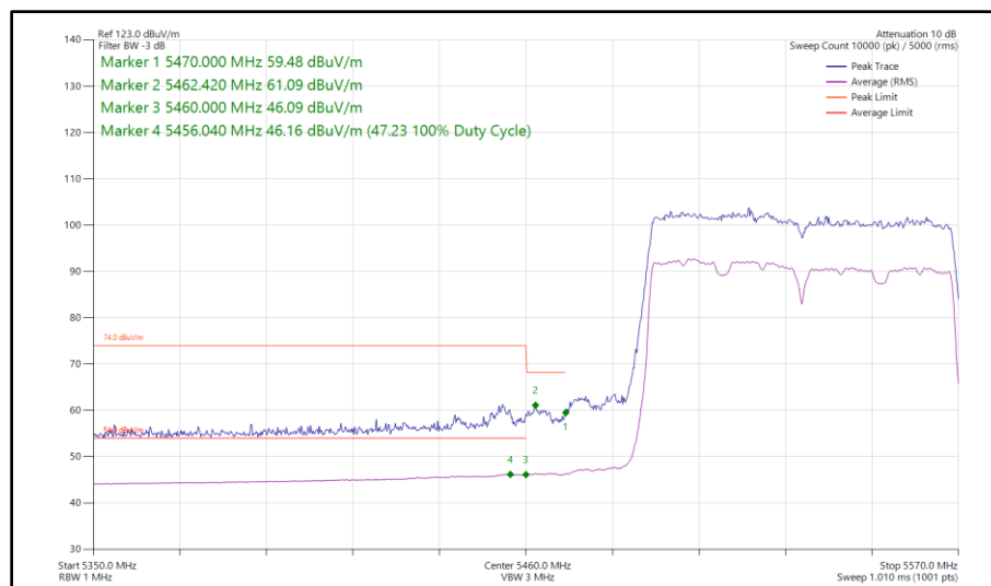
Figure 487 - 802.11ac VHT80, SISO, Core 0 - 5530 MHz Band Edge Frequency 5470 MHz
