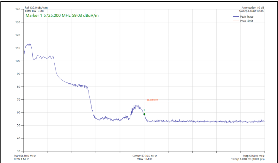
Figure 441 - 802.11ax HE40, RU 52-37, SISO, Core 1 - 5670 MHz Band Edge Frequency 5725 MHz
