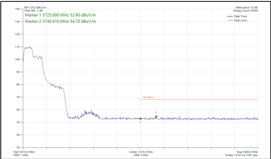
Figure 421 - 802.11ax HE40, RU 106-53, SISO, Core 0 - 5630 MHz Band Edge Frequency 5725 MHz
