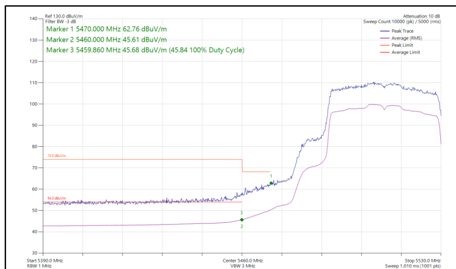
Figure 411 - 802.11ax HE40, SU, SISO, Core 0 - 5510 MHz Band Edge Frequency 5470 MHz
