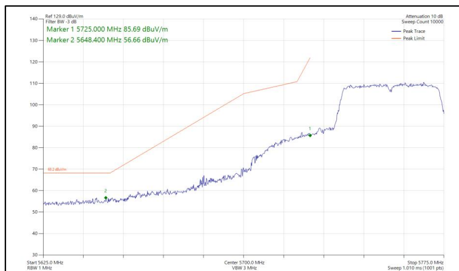
Figure 415 - 802.11n HT40, SISO, Core 0 - 5755 MHz Band Edge Frequency 5725 MHz
