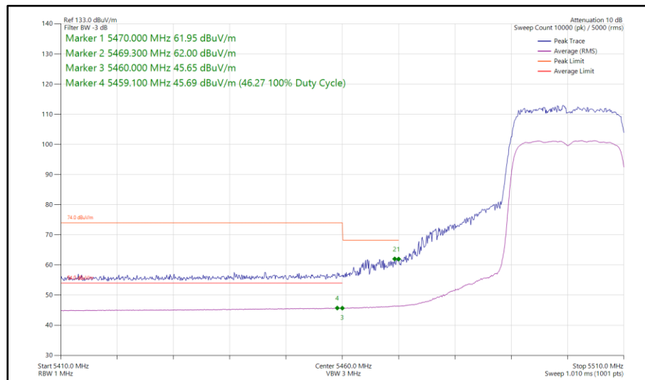
Figure 382 - 802.11ax HE20, SU, CDD, Core 0 - Core 1 - 5500 MHz Band Edge Frequency 5470 MHz
