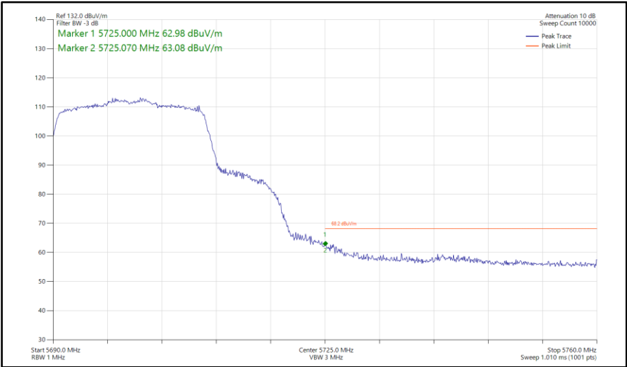
Figure 400 - 802.11ax HE20, SU, SDM, Core 0 - Core 1 - 5700 MHz Band Edge Frequency 5725 MHz
