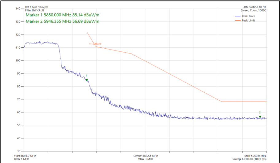
Figure 363 - 802.11ax HE20, SU, SISO, Core 0 - 5825 MHz Band Edge Frequency 5850 MHz
