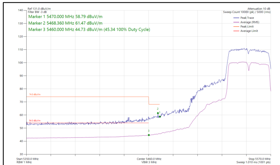
Figure 410 - 802.11n HT40, SISO, Core 0 - 5550 MHz Band Edge Frequency 5470 MHz
