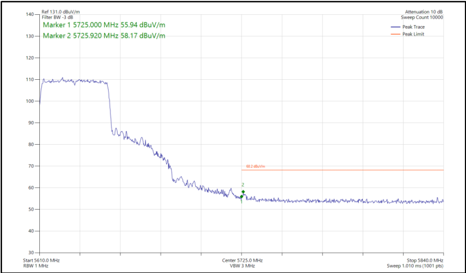
Figure 420 - 802.11ax HE40, SU, SISO, Core 0 - 5630 MHz Band Edge Frequency 5725 MHz
