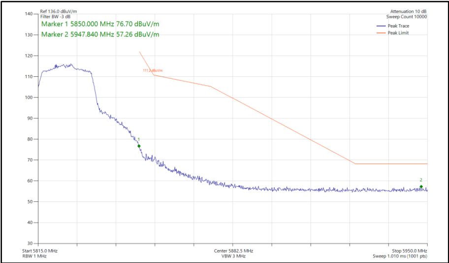
Figure 402 - 802.11n HT20, SDM, Core 0 - Core 1 - 5825 MHz Band Edge Frequency 5850 MHz
