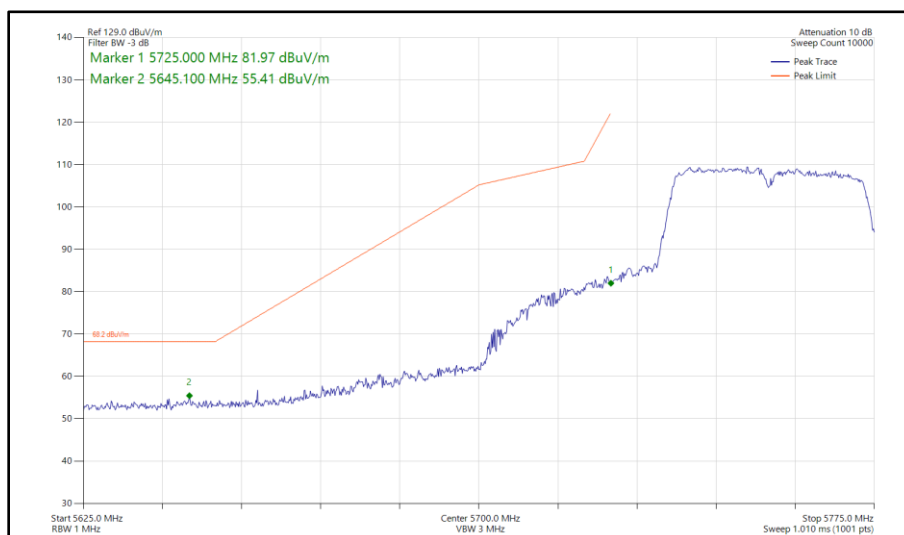
Figure 433 - 802.11n HT40, SISO, Core 1 - 5755 MHz Band Edge Frequency 5725 MHz
