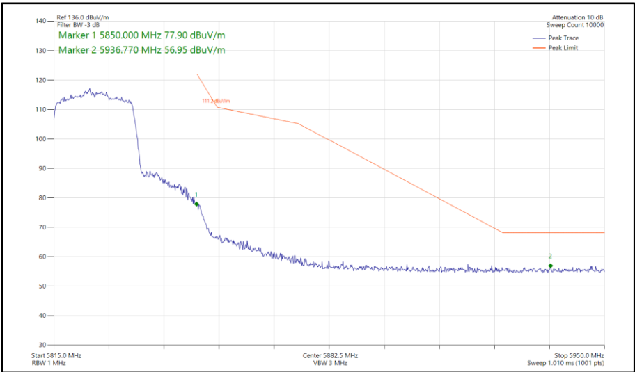
Figure 391 - 802.11ax HE20, SU, CDD, Core 0 - Core 1 - 5825 MHz Band Edge Frequency 5850 MHz
