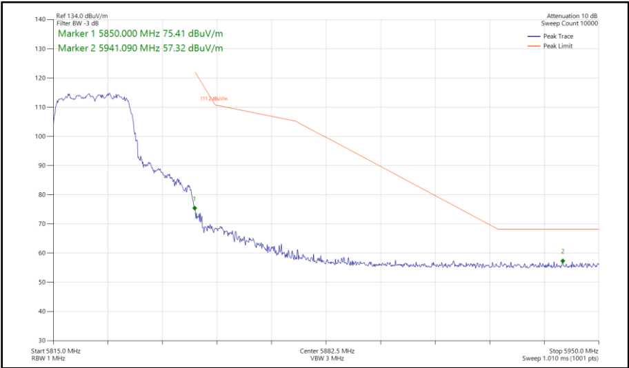
Figure 390 - 802.11n HT20, CDD, Core 0 - Core 1 - 5825 MHz Band Edge Frequency 5850 MHz
