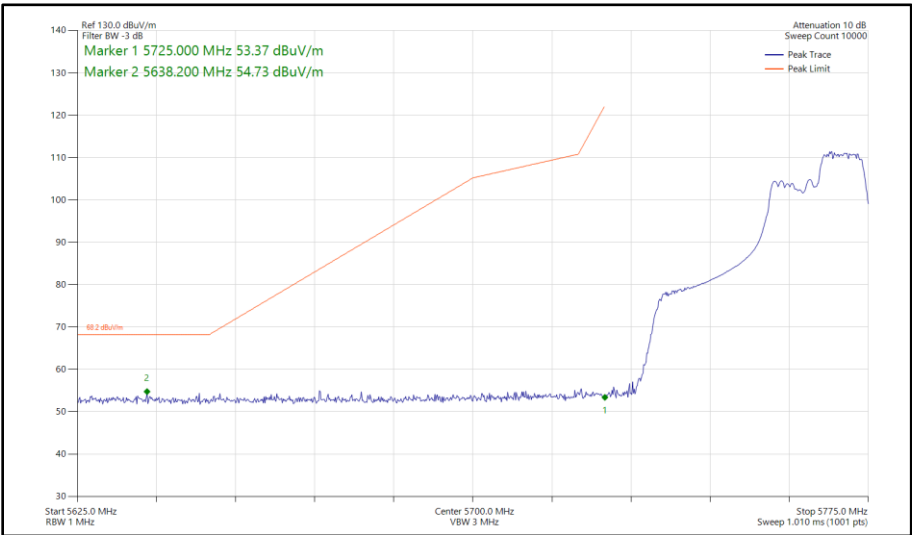
Figure 417 - 802.11ax HE40, RU 106-56, SISO, Core 0 - 5755 MHz Band Edge Frequency 5725 MHz
