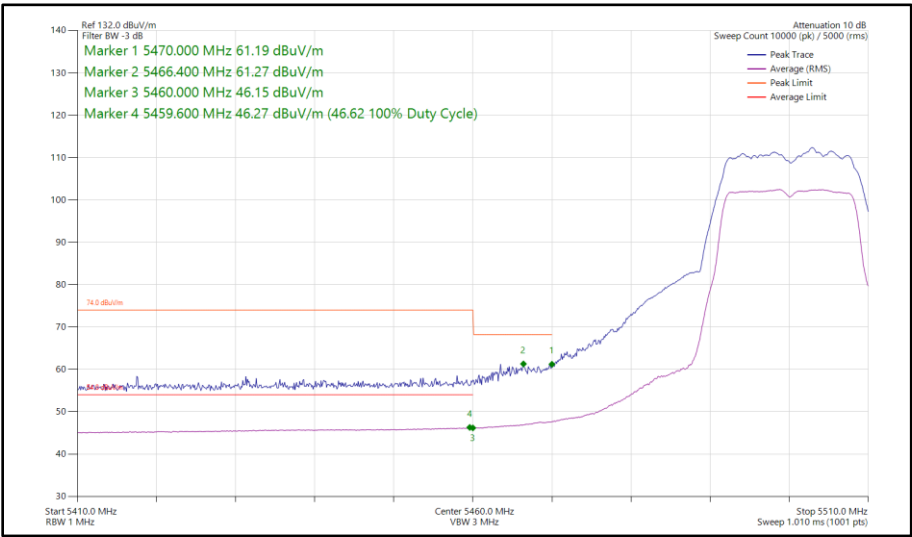
Figure 365 - 802.11a, SISO, Core 1 - 5500 MHz Band Edge Frequency 5470 MHz
