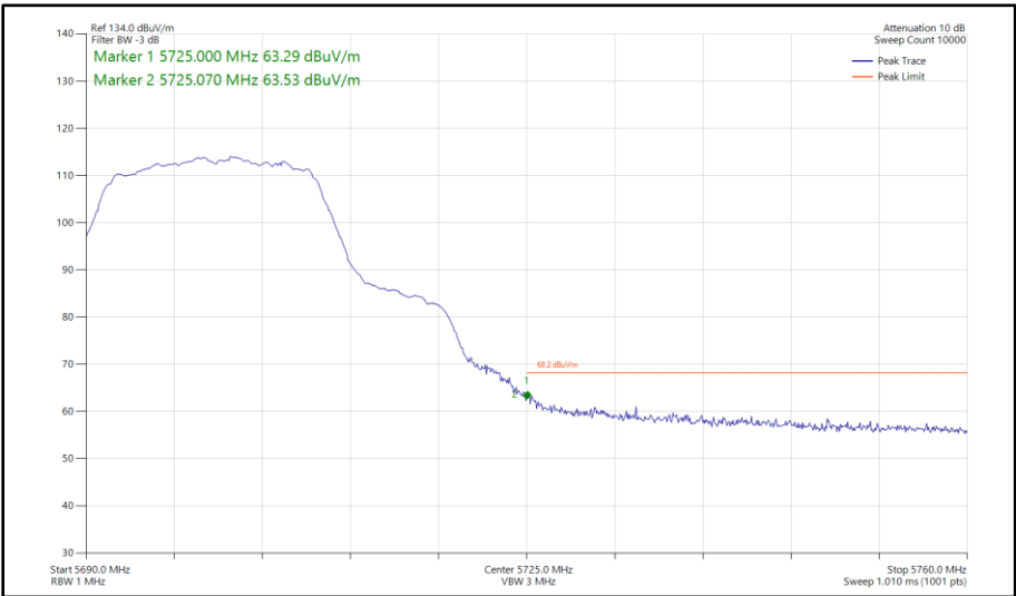
Figure 373 - 802.11a, SISO, Core 1 - 5700 MHz Band Edge Frequency 5725 MHz
