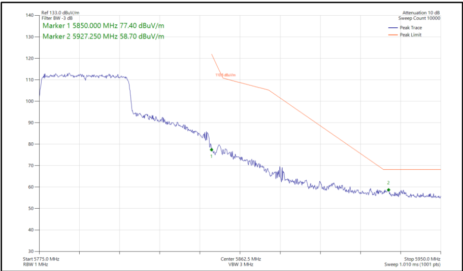
Figure 425 - 802.11ax HE40, SU, SISO, Core 0 - 5795 MHz Band Edge Frequency 5850 MHz
