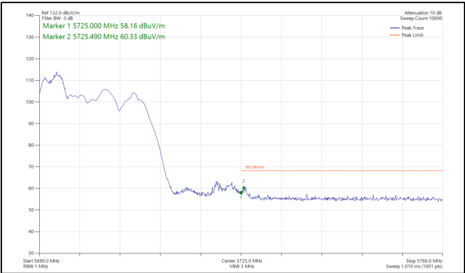
Figure 401 - 802.11ax HE20, RU 52-37, SDM, Core 0 - Core 1 - 5700 MHz Band Edge Frequency 5725 MHz
