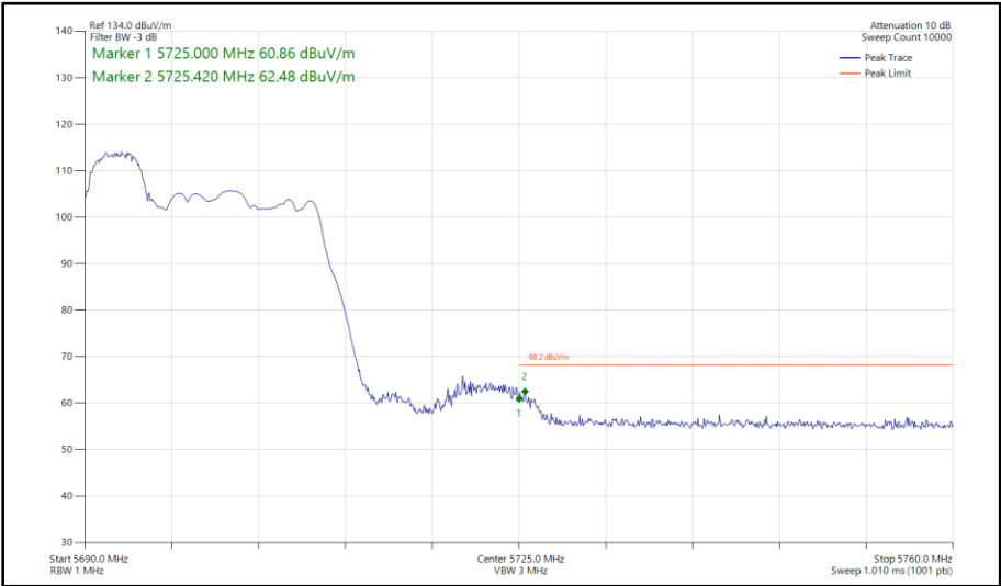
Figure 360 - 802.11ax HE20, RU 52-37, SISO, Core 0 - 5700 MHz Band Edge Frequency 5725 MHz
