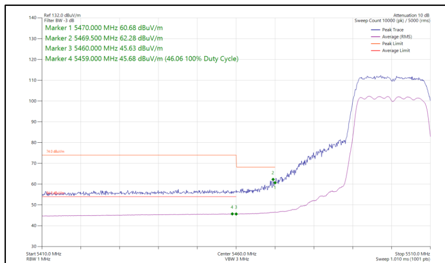
Figure 381 - 802.11n HT20, CDD, Core 0 - Core 1 - 5500 MHz Band Edge Frequency 5470 MHz
