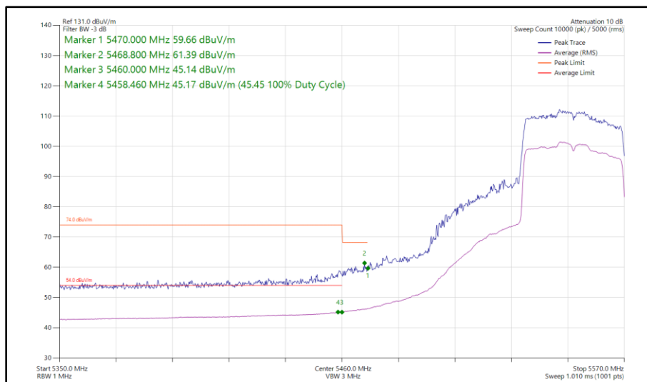
Figure 413 - 802.11ax HE40, SU, SISO, Core 0 - 5550 MHz Band Edge Frequency 5470 MHz
