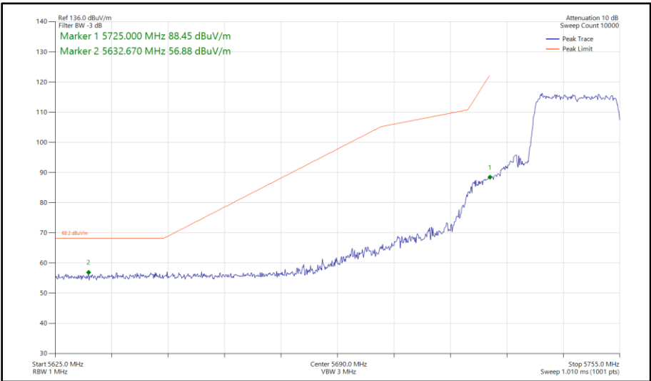
Figure 397 - 802.11ax HE20, SU, SDM, Core 0 - Core 1 - 5745 MHz Band Edge Frequency 5725 MHz
