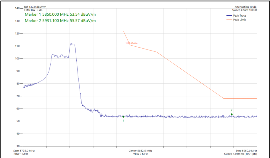
Figure 426 - 802.11ax HE40, RU 52-44, SISO, Core 0 - 5795 MHz Band Edge Frequency 5850 MHz
