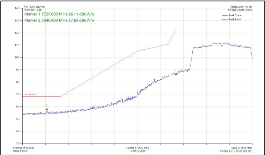
Figure 416 - 802.11ax HE40, SU, SISO, Core 0 - 5755 MHz Band Edge Frequency 5725 MHz
