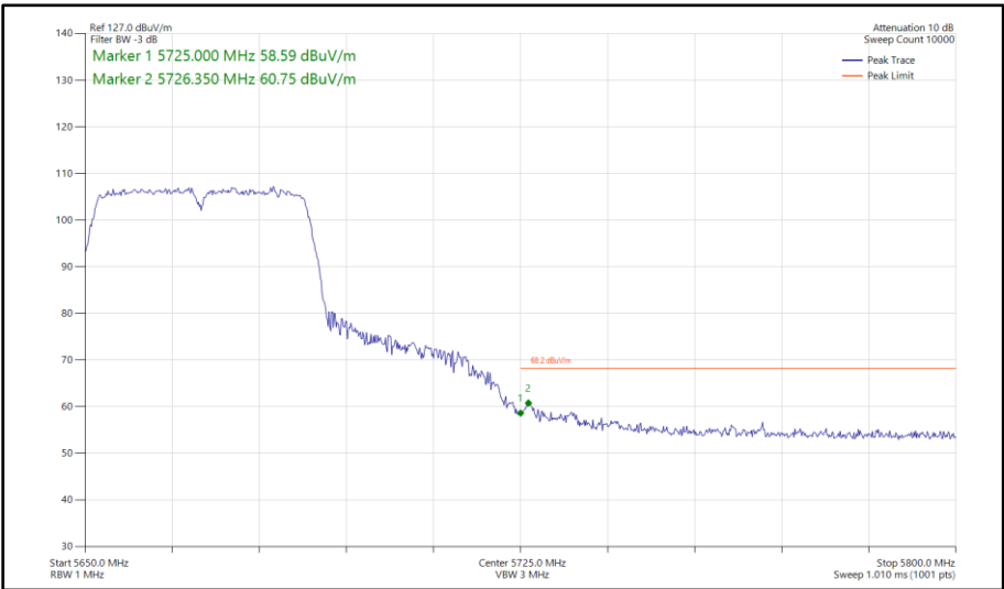
Figure 419 - 802.11n HT40, SISO, Core 0 - 5670 MHz Band Edge Frequency 5725 MHz
