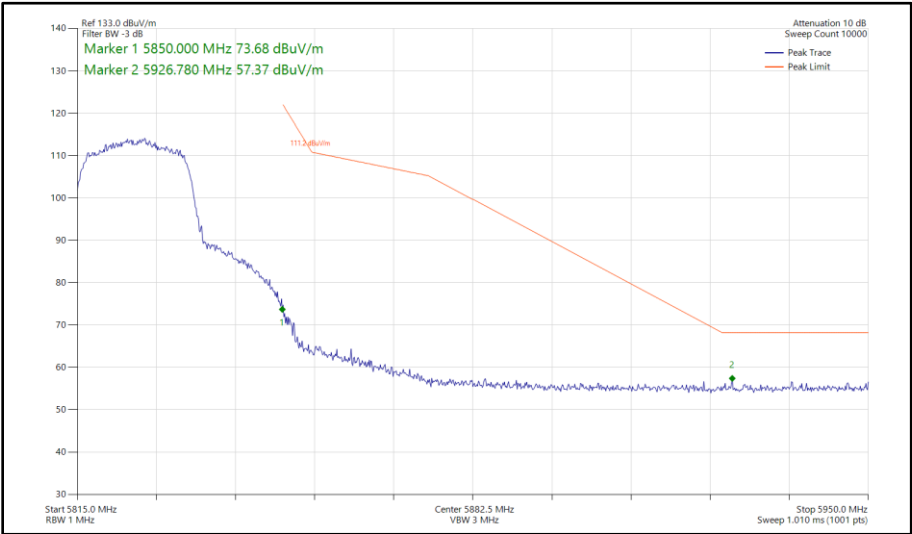
Figure 362 - 802.11n HT20, SISO, Core 0 - 5825 MHz Band Edge Frequency 5850 MHz
