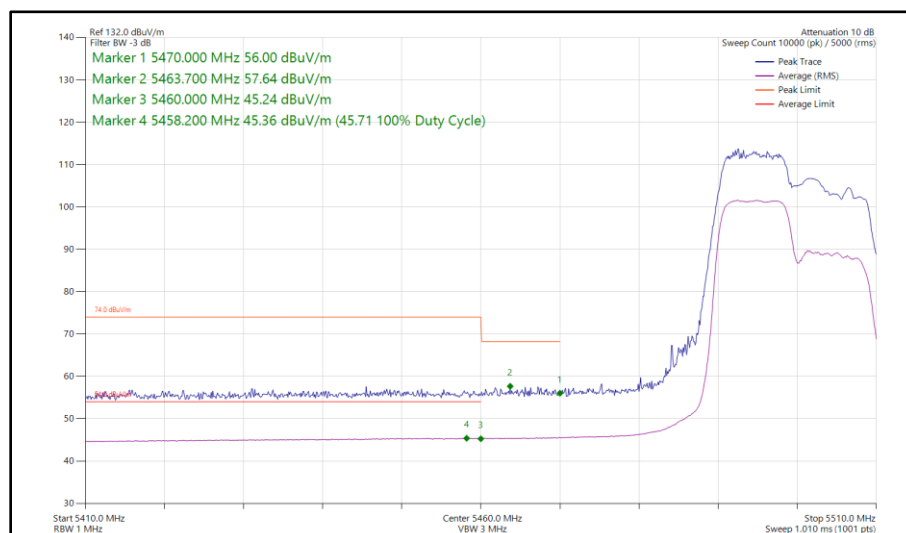
Figure 383 - 802.11ax HE20, RU 106-53, CDD, Core 0 - Core 1 - 5500 MHz Band Edge Frequency 5470 MHz
