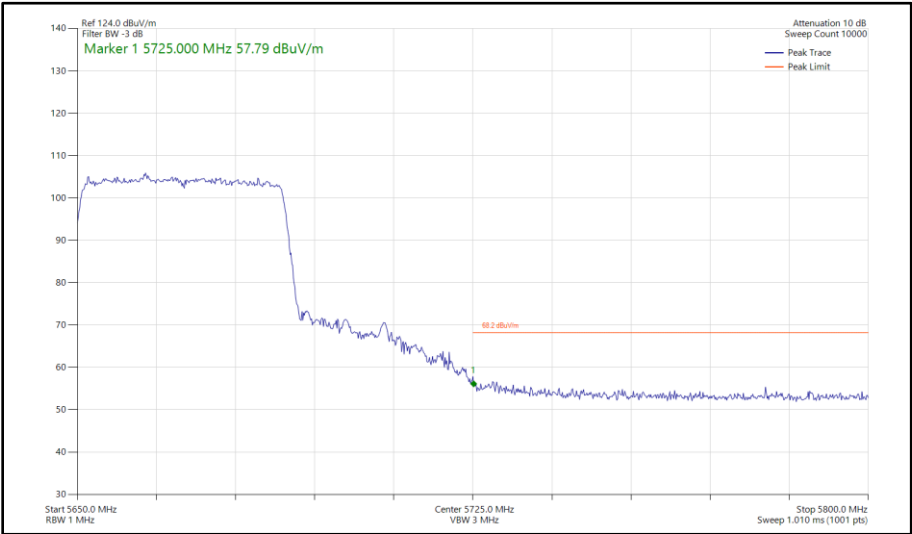
Figure 422 - 802.11ax HE40, SU, SISO, Core 0 - 5670 MHz Band Edge Frequency 5725 MHz
