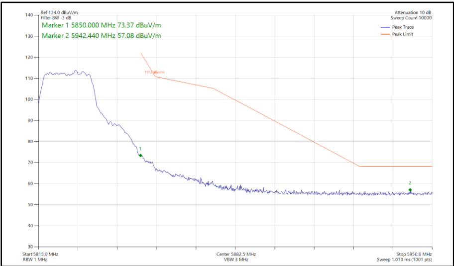
Figure 361 - 802.11a, SISO, Core 0 - 5825 MHz Band Edge Frequency 5850 MHz
