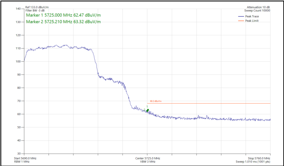
Figure 388 - 802.11ax HE20, SU, CDD, Core 0 - Core 1 - 5700 MHz Band Edge Frequency 5725 MHz
