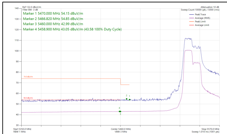
Figure 414 - 802.11ax HE40, RU 106-53, SISO, Core 0 - 5550 MHz Band Edge Frequency 5470 MHz
