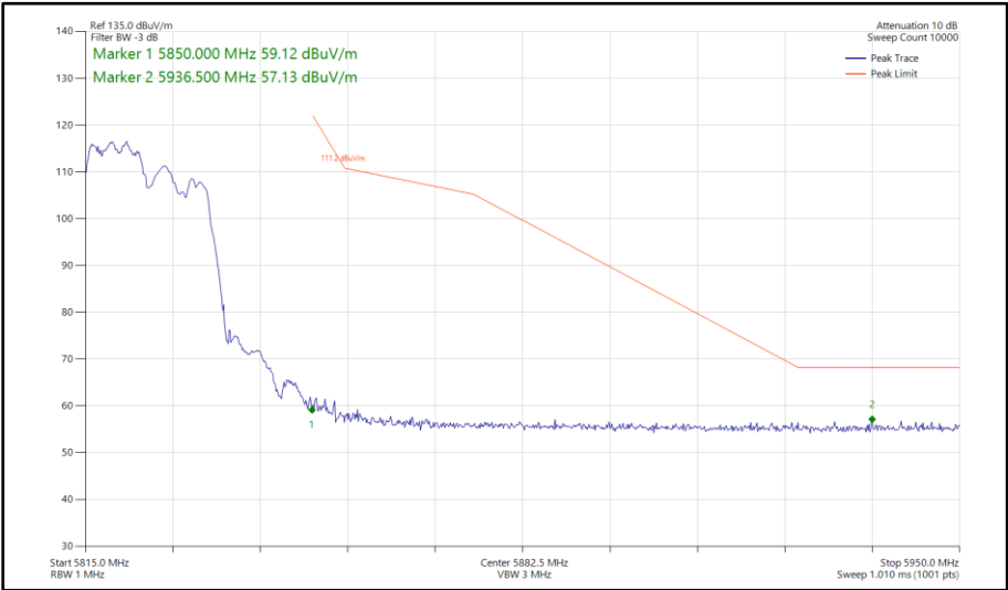
Figure 392 - 802.11ax HE20, RU 106-53, CDD, Core 0 - Core 1 - 5825 MHz Band Edge Frequency 5850 MHz
