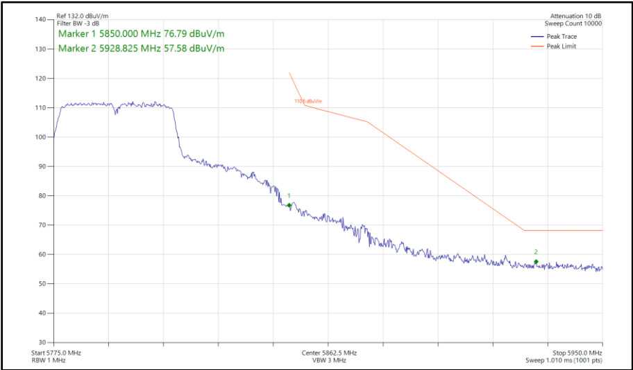
Figure 424 - 802.11n HT40, SISO, Core 0 - 5795 MHz Band Edge Frequency 5850 MHz
