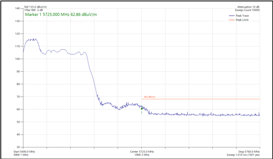
Figure 376 - 802.11ax HE20, RU 52-37, SISO, Core 1 - 5700 MHz Band Edge Frequency 5725 MHz
