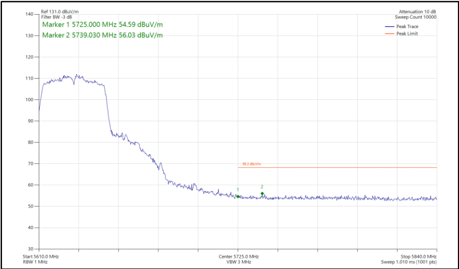
Figure 418 - 802.11n HT40, SISO, Core 0 - 5630 MHz Band Edge Frequency 5725 MHz
