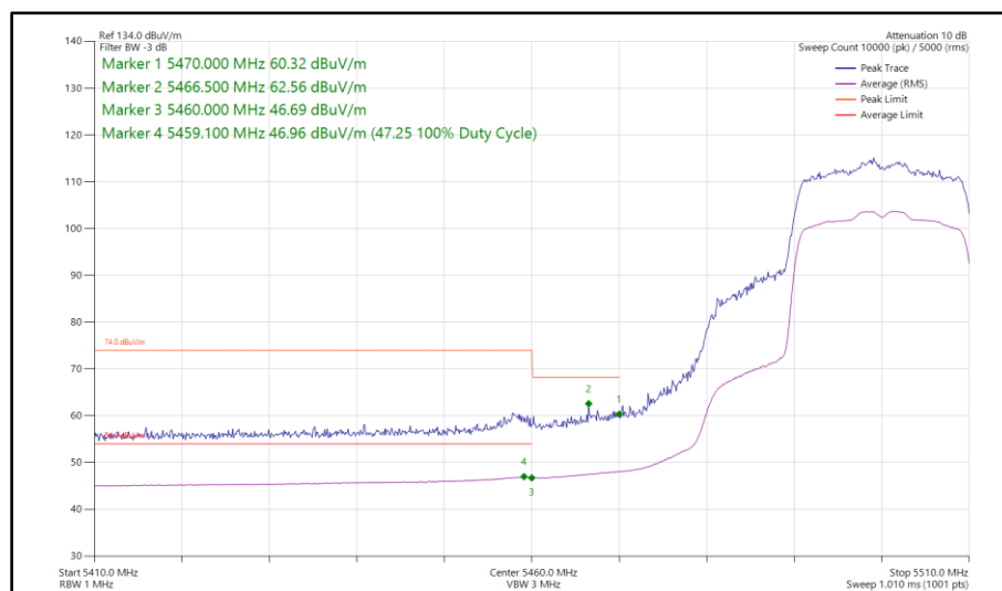
Figure 367 - 802.11ax HE20, SU, SISO, Core 1 - 5500 MHz Band Edge Frequency 5470 MHz
