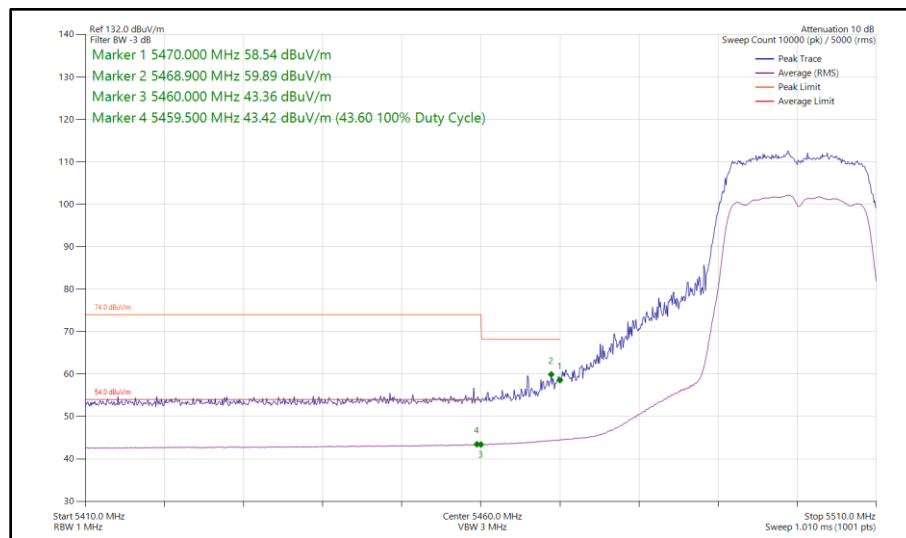
Figure 405 - 802.11ac VHT20, TxBF, Core 0 - Core 1 - 5500 MHz Band Edge Frequency 5470 MHz
