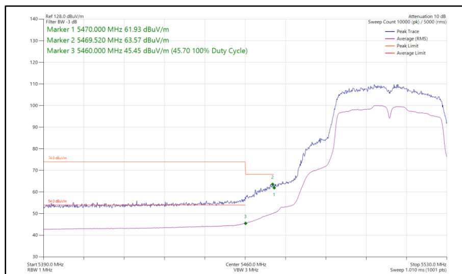
Figure 409 - 802.11n HT40, SISO, Core 0 - 5510 MHz Band Edge Frequency 5470 MHz
