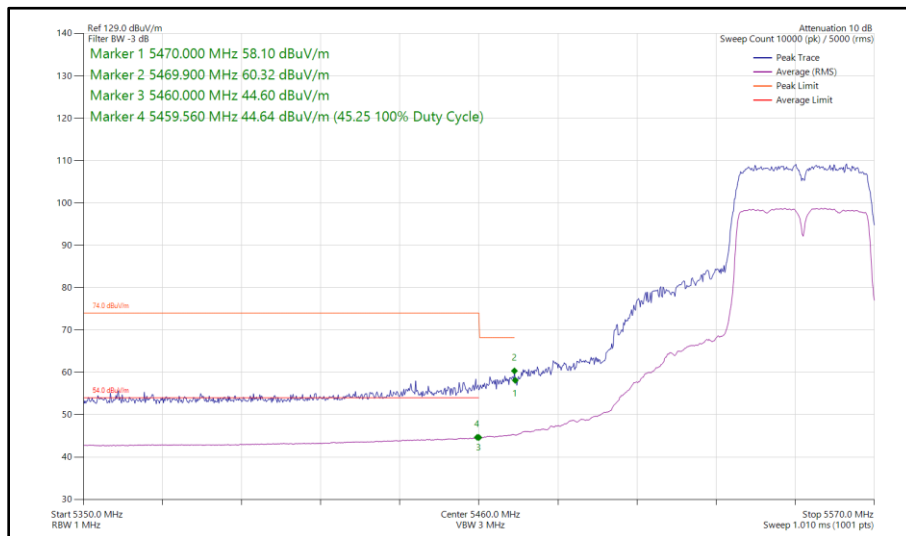
Figure 428 - 802.11n HT40, SISO, Core 1 - 5550 MHz Band Edge Frequency 5470 MHz
