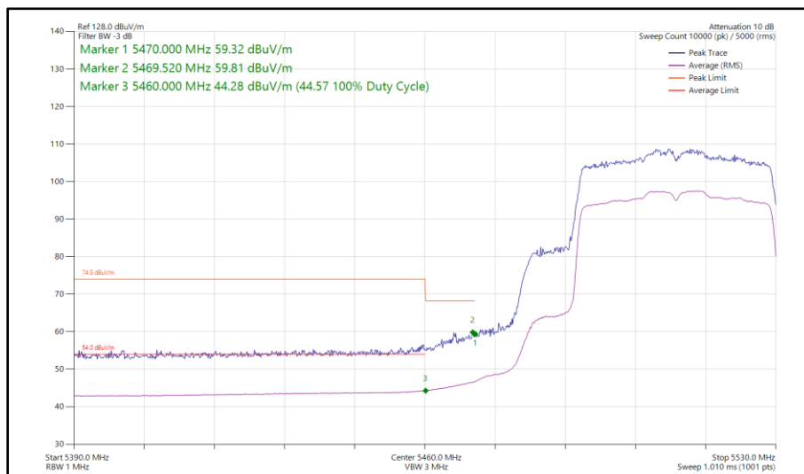
Figure 429 - 802.11ax HE40, SU, SISO, Core 1 - 5510 MHz Band Edge Frequency 5470 MHz
