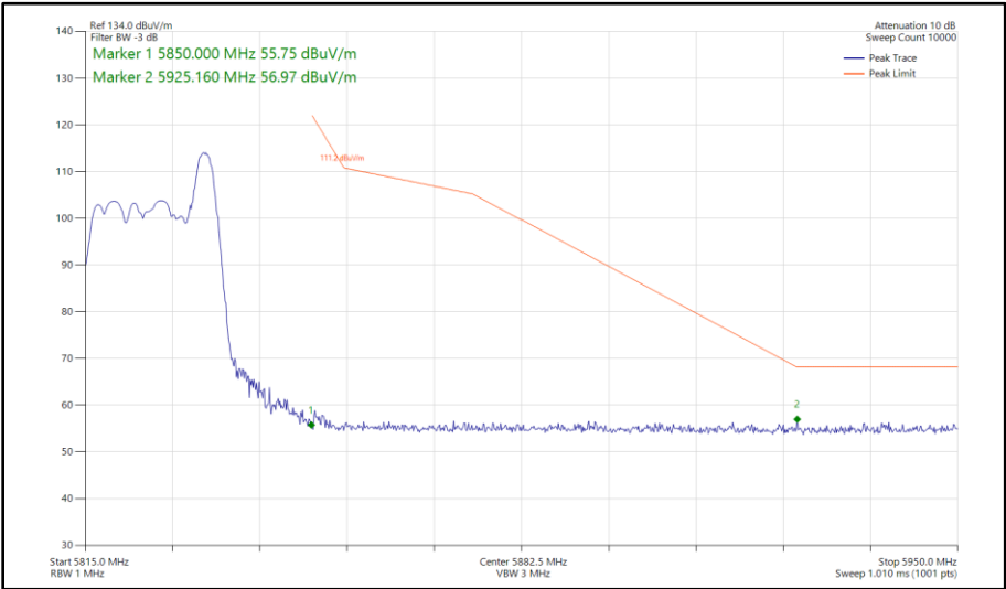
Figure 364 - 802.11ax HE20, RU 26-8, SISO, Core 0 - 5825 MHz Band Edge Frequency 5850 MHz
