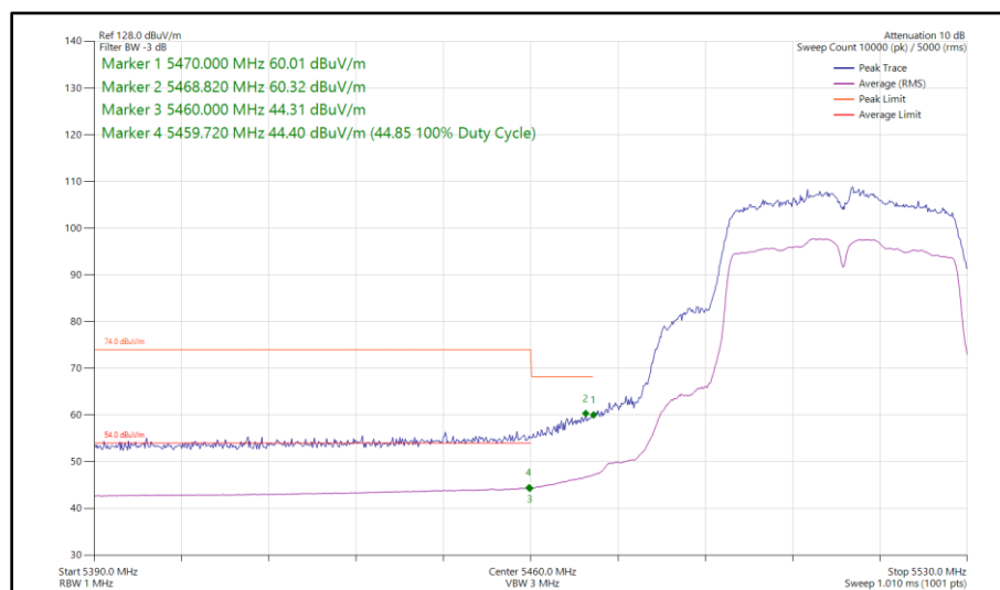
Figure 427 - 802.11n HT40, SISO, Core 1 - 5510 MHz Band Edge Frequency 5470 MHz
