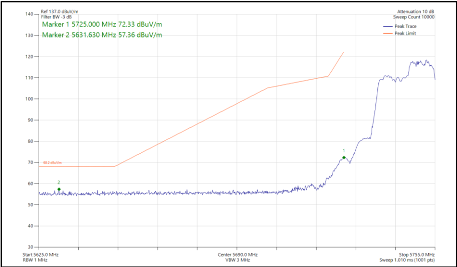
Figure 386 - 802.11ax HE20, RU 106-54, CDD, Core 0 - Core 1 - 5745 MHz Band Edge Frequency 5725 MHz
