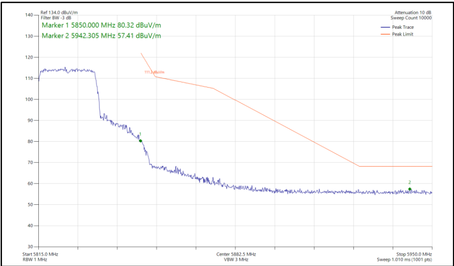
Figure 379 - 802.11ax HE20, SU, SISO, Core 1 - 5825 MHz Band Edge Frequency 5850 MHz
