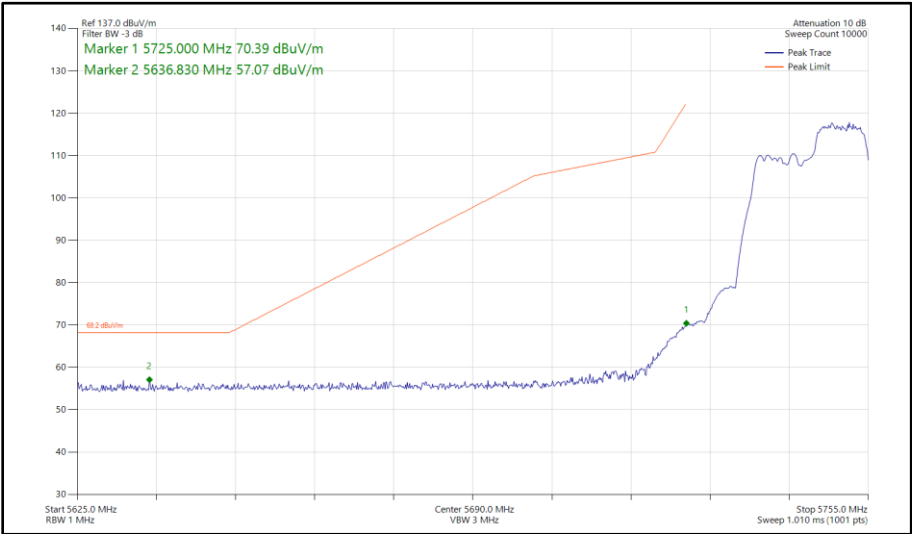
Figure 372 - 802.11ax HE20, RU 106-54, SISO, Core 1 - 5745 MHz Band Edge Frequency 5725 MHz
