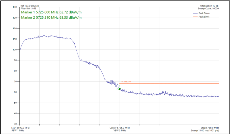
Figure 374 - 802.11n HT20, SISO, Core 1 - 5700 MHz Band Edge Frequency 5725 MHz
