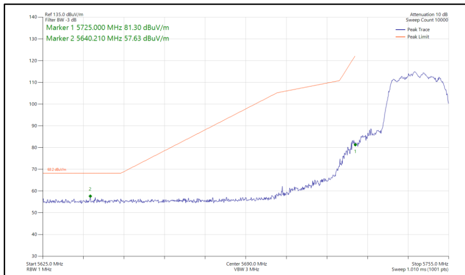
Figure 384 - 802.11n HT20, CDD, Core 0 - Core 1 - 5745 MHz Band Edge Frequency 5725 MHz
