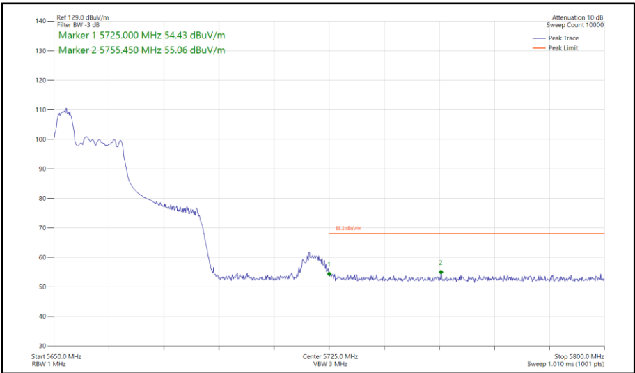
Figure 423 - 802.11ax HE40, RU 52-37, SISO, Core 0 - 5670 MHz Band Edge Frequency 5725 MHz
