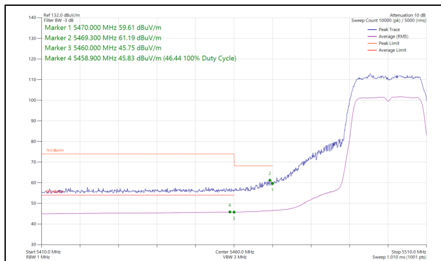
Figure 393 - 802.11n HT20, SDM, Core 0 - Core 1 - 5500 MHz Band Edge Frequency 5470 MHz
