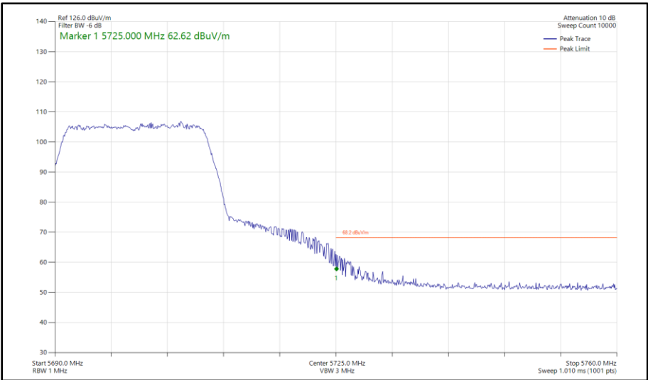
Figure 399 - 802.11n HT20, SDM, Core 0 - Core 1 - 5700 MHz Band Edge Frequency 5725 MHz
