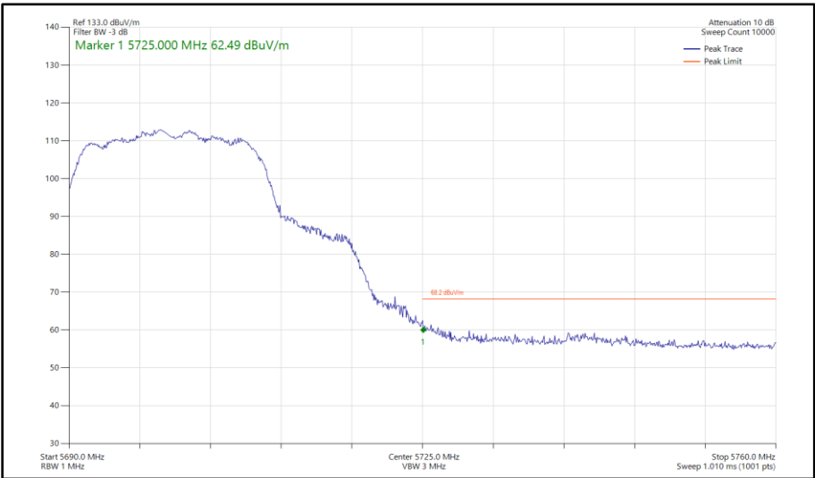
Figure 387 - 802.11n HT20, CDD, Core 0 - Core 1 - 5700 MHz Band Edge Frequency 5725 MHz
