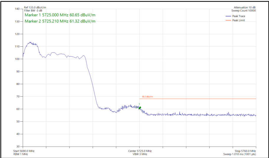
Figure 389 - 802.11ax HE20, RU 52-37, CDD, Core 0 - Core 1 - 5700 MHz Band Edge Frequency 5725 MHz
