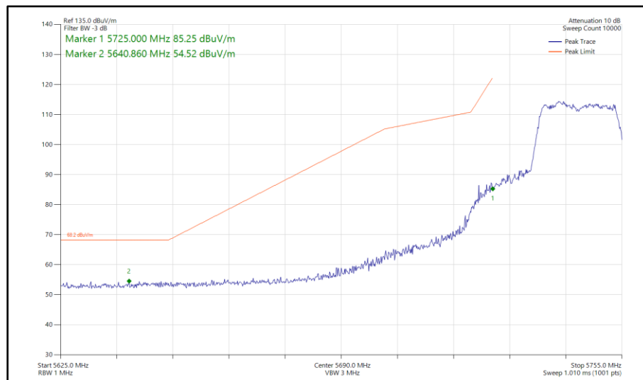
Figure 406 - 802.11ac VHT20, TxBF, Core 0 - Core 1 - 5745 MHz Band Edge Frequency 5725 MHz
