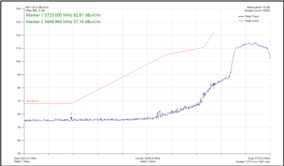
Figure 396 - 802.11n HT20, SDM, Core 0 - Core 1 - 5745 MHz Band Edge Frequency 5725 MHz
