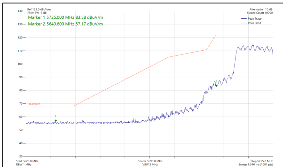
Figure 385 - 802.11ax HE20, SU, CDD, Core 0 - Core 1 - 5745 MHz Band Edge Frequency 5725 MHz
