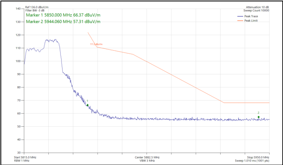
Figure 404 - 802.11ax HE20, RU 106-54, SDM, Core 0 - Core 1 - 5825 MHz Band Edge Frequency 5850 MHz
