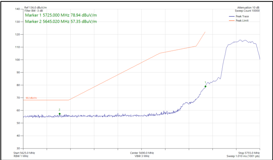
Figure 369 - 802.11a, SISO, Core 1 - 5745 MHz Band Edge Frequency 5725 MHz
