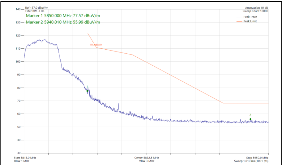
Figure 408 - 802.11ac VHT20, TxBF, Core 0 - Core 1 - 5825 MHz Band Edge Frequency 5850 MHz
