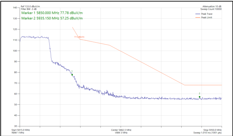
Figure 403 - 802.11ax HE20, SU, SDM, Core 0 - Core 1 - 5825 MHz Band Edge Frequency 5850 MHz
