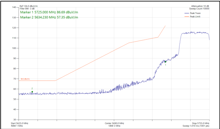
Figure 371 - 802.11ax HE20, SU, SISO, Core 1 - 5745 MHz Band Edge Frequency 5725 MHz
