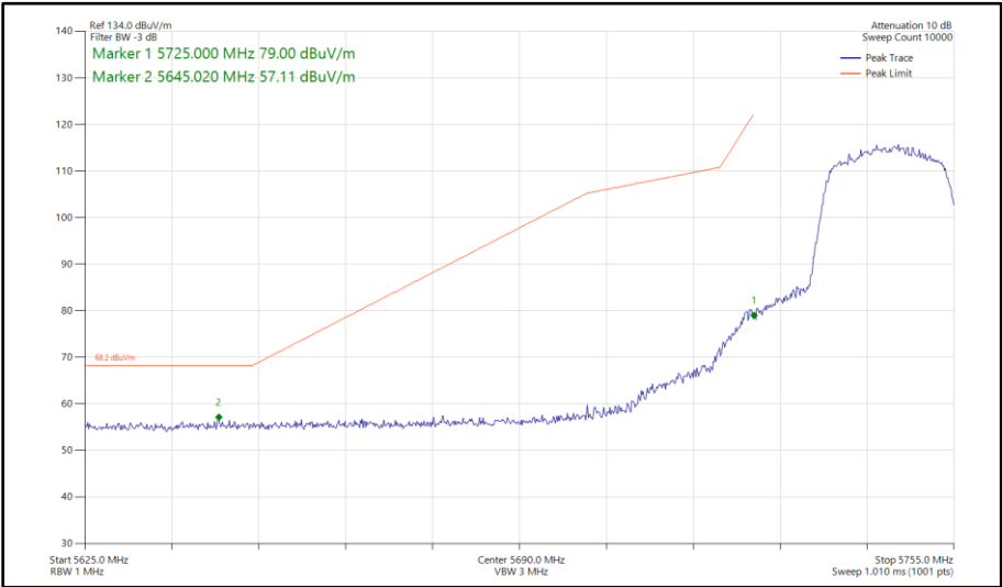
Figure 370 - 802.11n HT20, SISO, Core 1 - 5745 MHz Band Edge Frequency 5725 MHz
