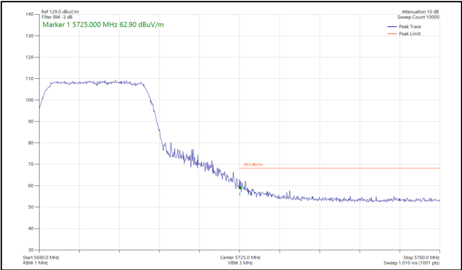
Figure 407 - 802.11ac VHT20, TxBF, Core 0 - Core 1 - 5700 MHz Band Edge Frequency 5725 MHz
