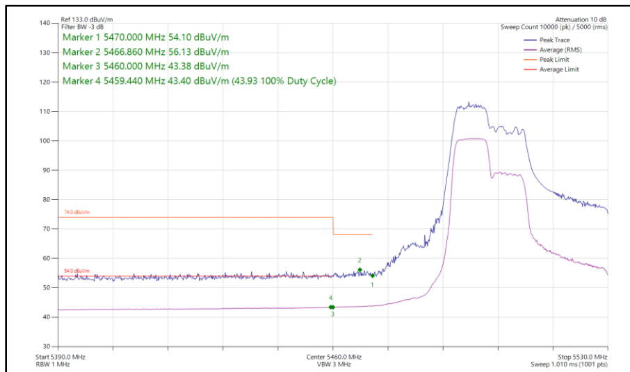
Figure 412 - 802.11ax HE40, RU 106-53, SISO, Core 0 - 5510 MHz Band Edge Frequency 5470 MHz
