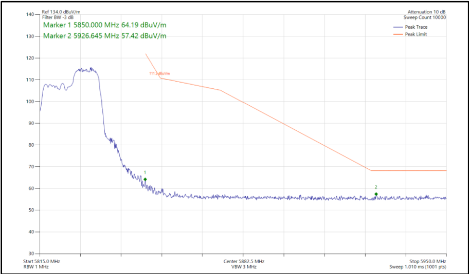
Figure 380 - 802.11ax HE20, RU 106-54, SISO, Core 1 - 5825 MHz Band Edge Frequency 5850 MHz
