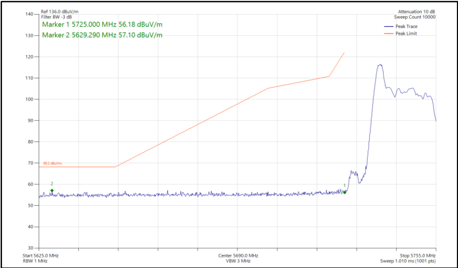
Figure 398 - 802.11ax HE20, RU 26-0, SDM, Core 0 - Core 1 - 5745 MHz Band Edge Frequency 5725 MHz
