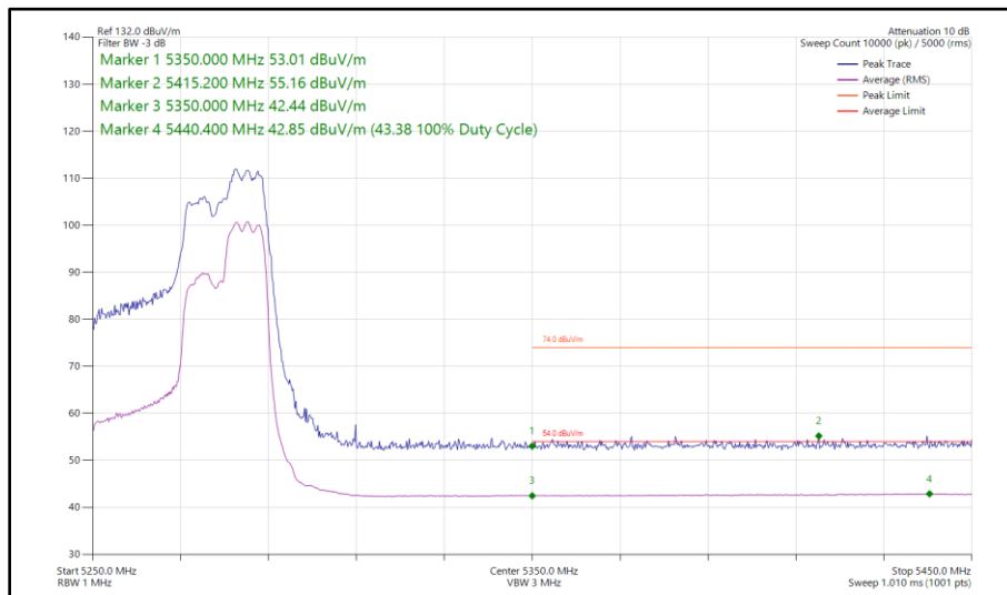
Figure 109 - 802.11ax HE40, RU 106-56, SDM, Core 0 - Core 1 - 5270 MHz Band Edge Frequency 5350 MHz
