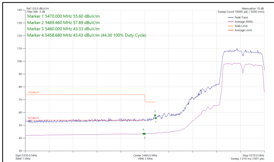
Figure 113 - 802.11n HT40, SDM, Core 0 - Core 1 - 5550 MHz Band Edge Frequency 5460 MHz
