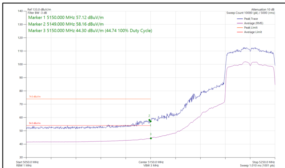
Figure 104 - 802.11ax HE40, SU, SDM, Core 0 - Core 1 - 5230 MHz Band Edge Frequency 5150 MHz
