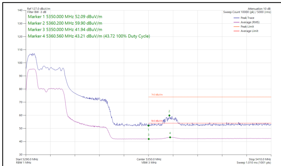
Figure 75 - 802.11ax HE40, RU 52-37, SISO, Core 1 - 5310 MHz Band Edge Frequency 5350 MHz
