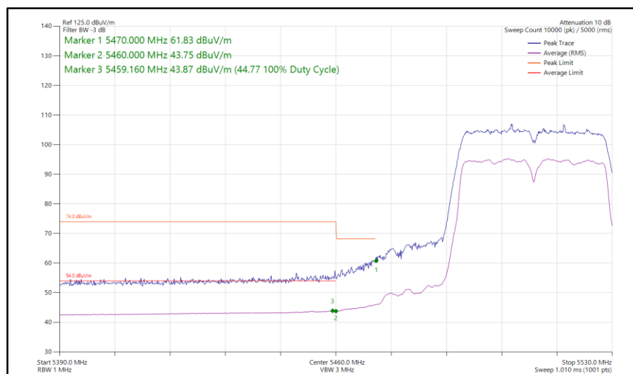
Figure 112 - 802.11n HT40, SDM, Core 0 - Core 1 - 5510 MHz Band Edge Frequency 5460 MHz
