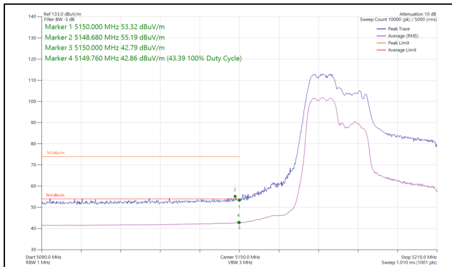
Figure 85 - 802.11ax HE40, RU 106-53, CDD, Core 0 - Core 1 - 5190 MHz Band Edge Frequency 5150 MHz
