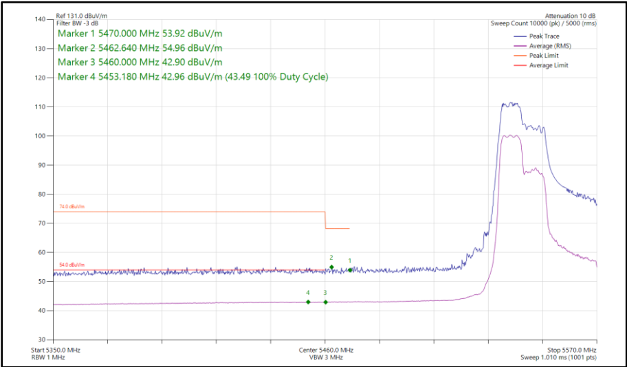
Figure 99 - 802.11ax HE40, RU 106-53, CDD, Core 0 - Core 1 - 5550 MHz Band Edge Frequency 5460 MHz
