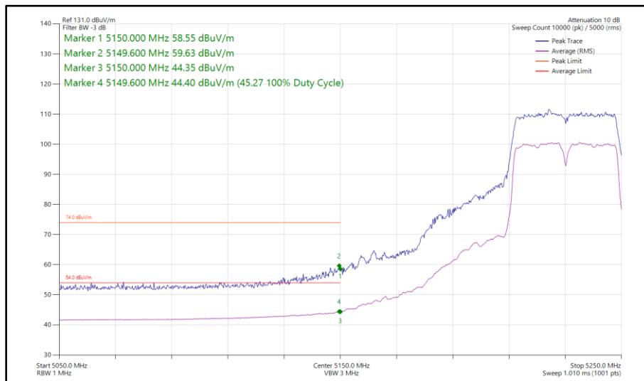
Figure 101 - 802.11n HT40, SDM, Core 0 - Core 1 - 5230 MHz Band Edge Frequency 5150 MHz
