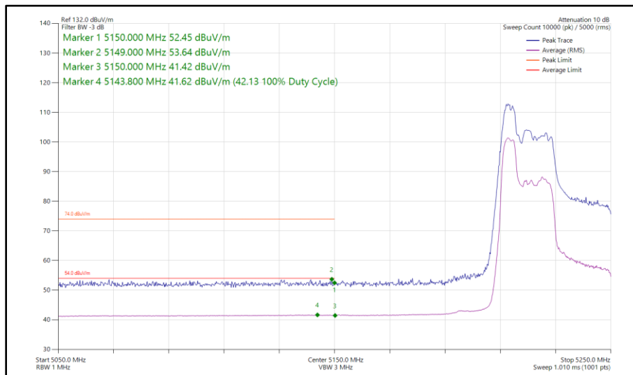
Figure 87 - 802.11ax HE40, RU 52-37, CDD, Core 0 - Core 1 - 5230 MHz Band Edge Frequency 5150 MHz
