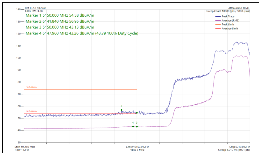
Figure 103 - 802.11ax HE40, RU 106-56, SDM, Core 0 - Core 1 - 5190 MHz Band Edge Frequency 5150 MHz
