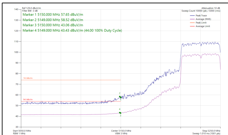
Figure 86 - 802.11ax HE40, SU, CDD, Core 0 - Core 1 - 5230 MHz Band Edge Frequency 5150 MHz
