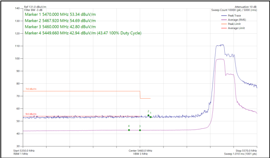
Figure 81 - 802.11ax HE40, RU 106-53, SISO, Core 1 - 5550 MHz Band Edge Frequency 5460 MHz
