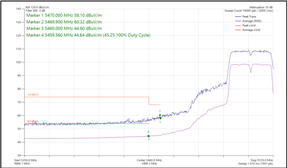
Figure 77 - 802.11n HT40, SISO, Core 1 - 5550 MHz Band Edge Frequency 5460 MHz
