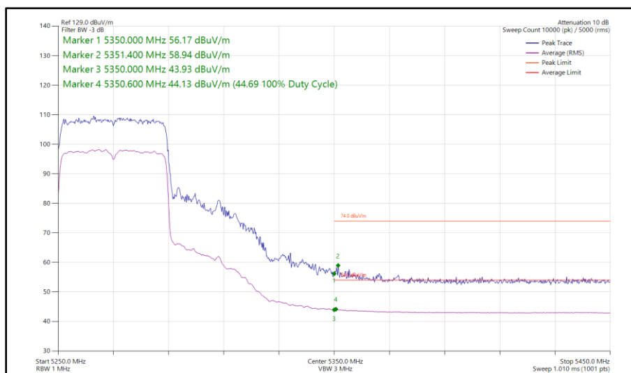
Figure 90 - 802.11ax HE40, SU, CDD, Core 0 - Core 1 - 5270 MHz Band Edge Frequency 5350 MHz
