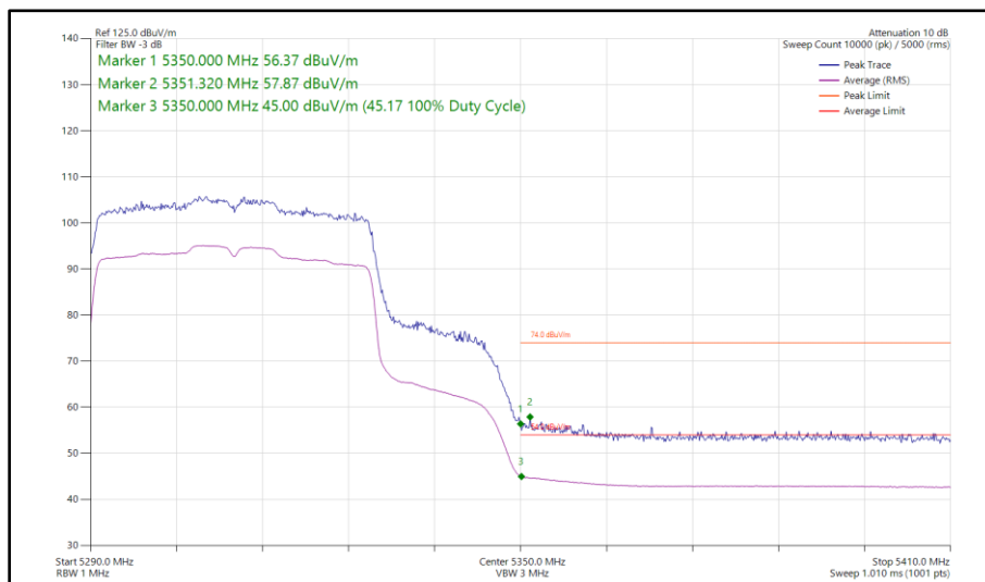
Figure 74 - 802.11ax HE40, SU, SISO, Core 1 - 5310 MHz Band Edge Frequency 5350 MHz
