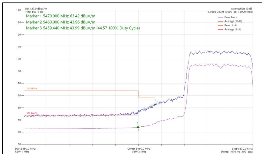
Figure 96 - 802.11ax HE40, SU, CDD, Core 0 - Core 1 - 5510 MHz Band Edge Frequency 5460 MHz
