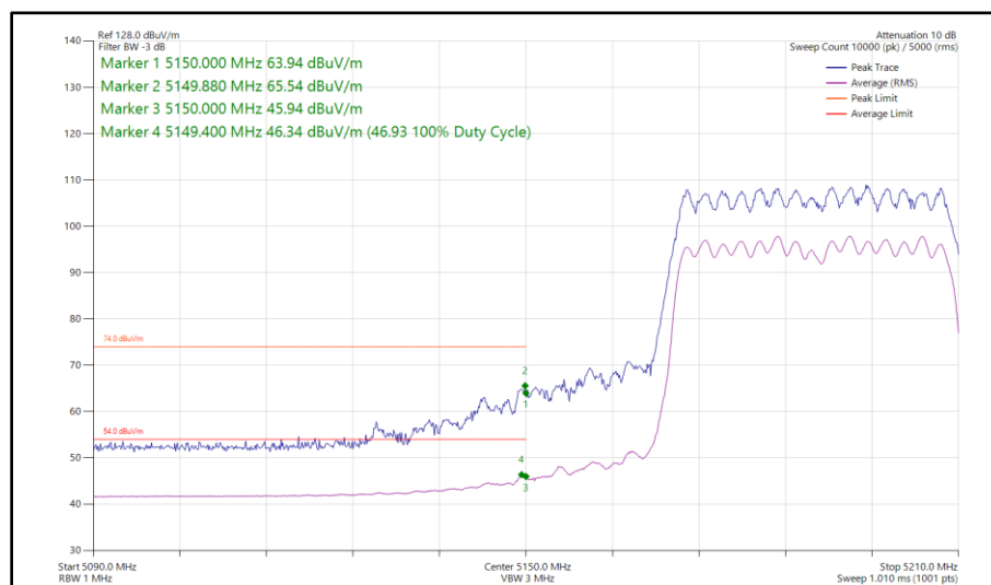
Figure 84 - 802.11ax HE40, SU, CDD, Core 0 - Core 1 - 5190 MHz Band Edge Frequency 5150 MHz
