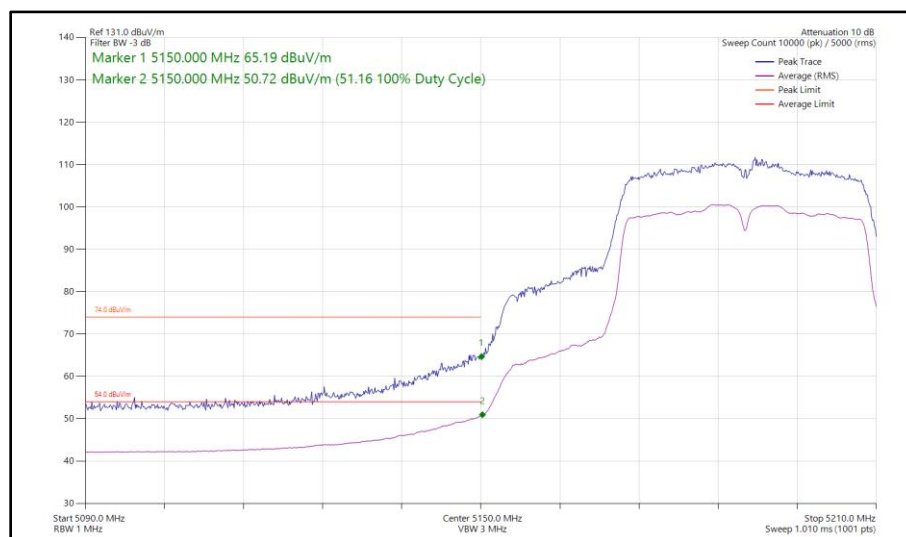
Figure 64 - 802.11n HT40, SISO, Core 1 - 5190 MHz Band Edge Frequency 5150 MHz
