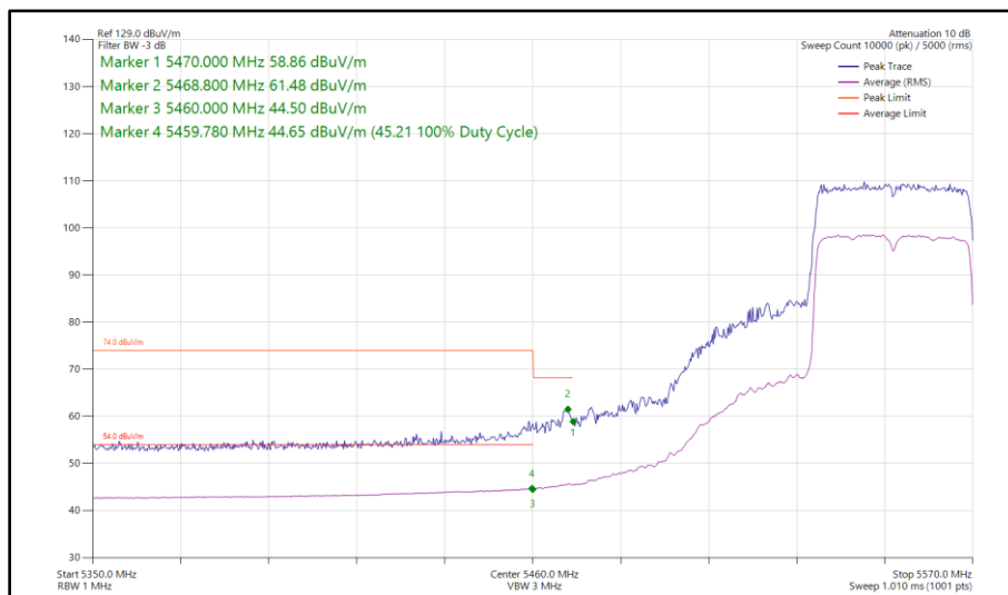
Figure 80 - 802.11ax HE40, SU, SISO, Core 1 - 5550 MHz Band Edge Frequency 5460 MHz
