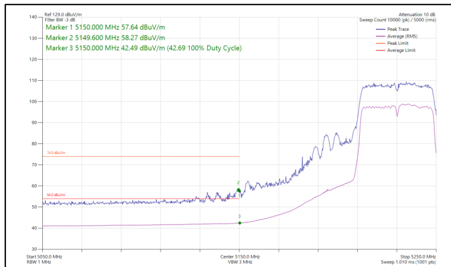
Figure 119 - 802.11ac VHT40, TxBF, Core 0 - Core 1 - 5230 MHz Band Edge Frequency 5150 MHz
