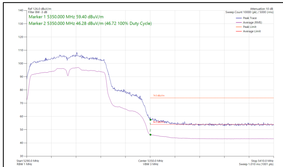
Figure 107 - 802.11n HT40, SDM, Core 0 - Core 1 - 5310 MHz Band Edge Frequency 5350 MHz
