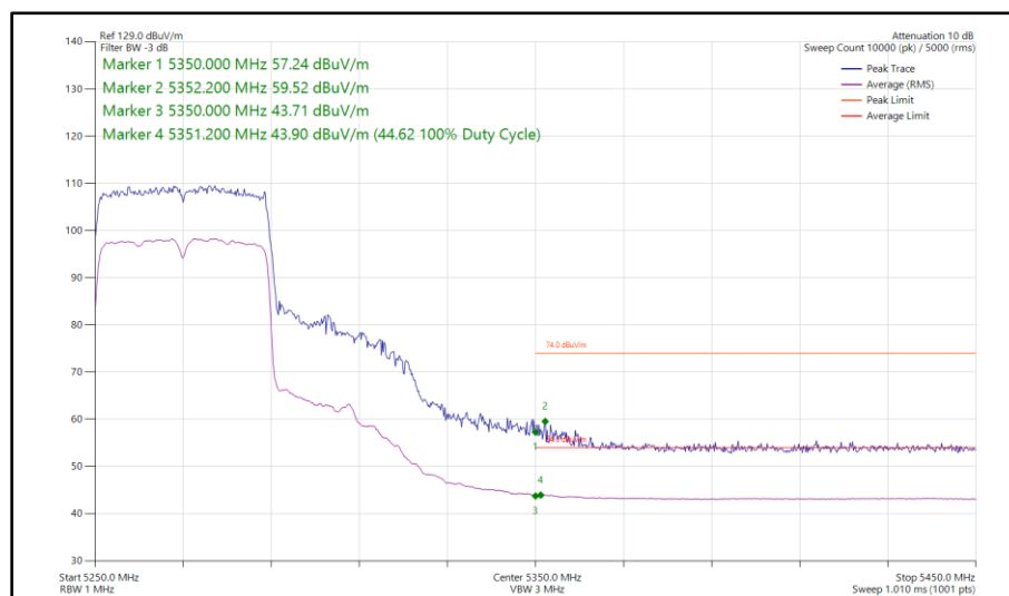
Figure 108 - 802.11ax HE40, SU, SDM, Core 0 - Core 1 - 5270 MHz Band Edge Frequency 5350 MHz
