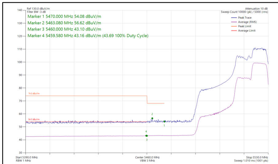
Figure 79 - 802.11ax HE40, RU 106-56, SISO, Core 1 - 5510 MHz Band Edge Frequency 5460 MHz
