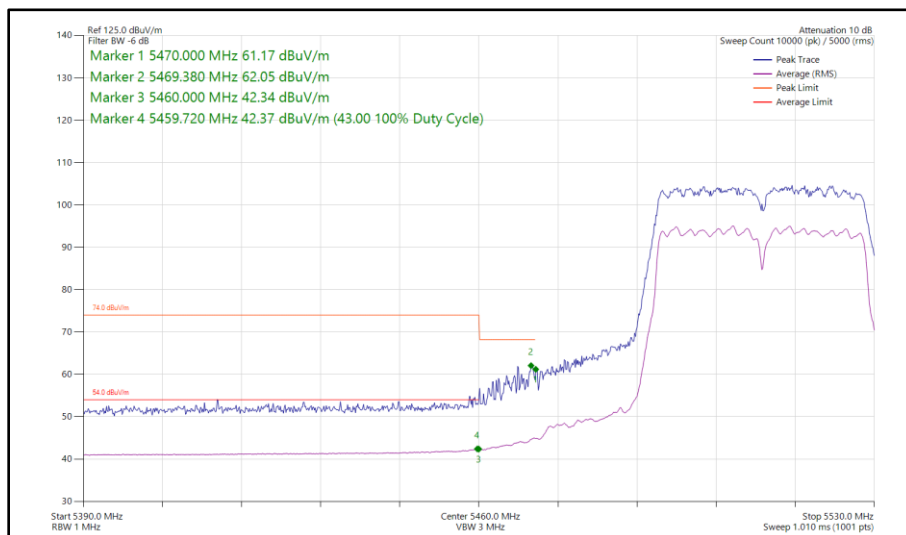
Figure 94 - 802.11n HT40, CDD, Core 0 - Core 1 - 5510 MHz Band Edge Frequency 5460 MHz
