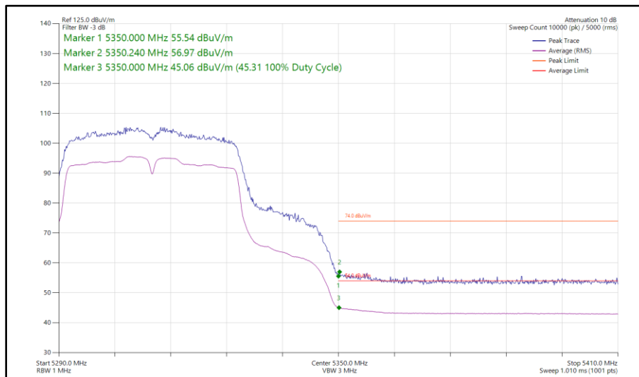
Figure 71 - 802.11n HT40, SISO, Core 1 - 5310 MHz Band Edge Frequency 5350 MHz
