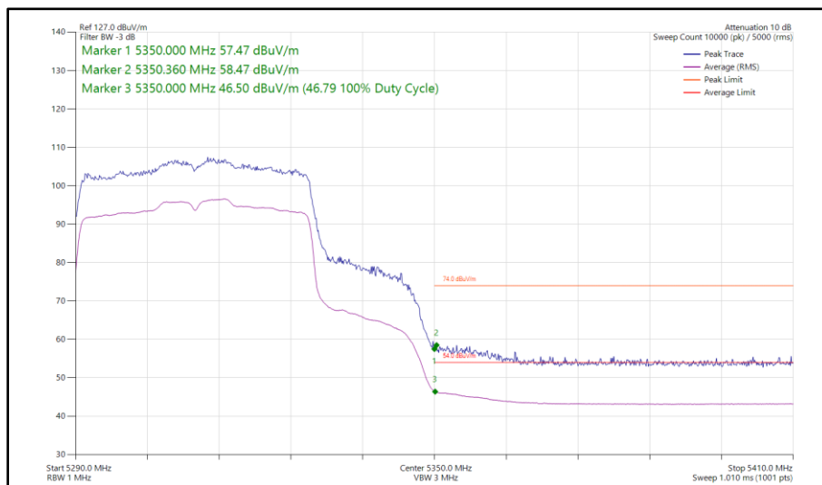
Figure 110 - 802.11ax HE40, SU, SDM, Core 0 - Core 1 - 5310 MHz Band Edge Frequency 5350 MHz
