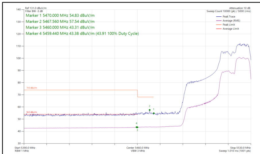
Figure 97 - 802.11ax HE40, RU 106-56, CDD, Core 0 - Core 1 - 5510 MHz Band Edge Frequency 5460 MHz
