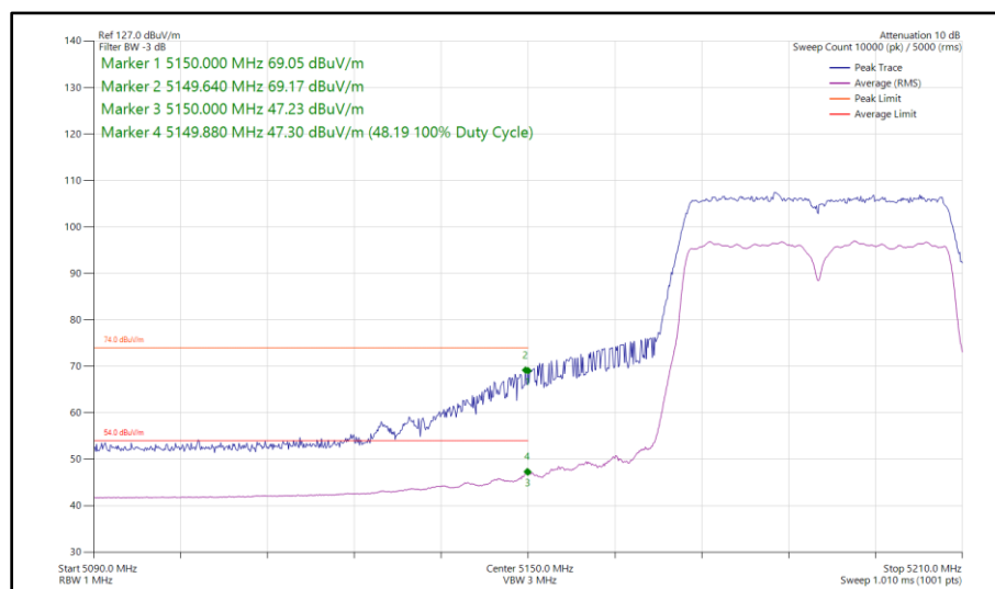
Figure 100 - 802.11n HT40, SDM, Core 0 - Core 1 - 5190 MHz Band Edge Frequency 5150 MHz
