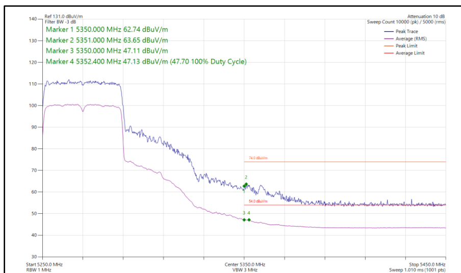
Figure 72 - 802.11ax HE40, SU, SISO, Core 1 - 5270 MHz Band Edge Frequency 5350 MHz
