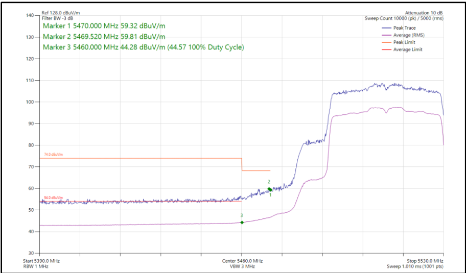
Figure 78 - 802.11ax HE40, SU, SISO, Core 1 - 5510 MHz Band Edge Frequency 5460 MHz
