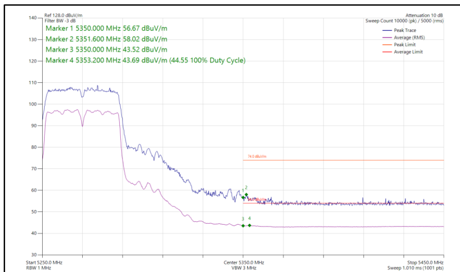
Figure 106 - 802.11n HT40, SDM, Core 0 - Core 1 - 5270 MHz Band Edge Frequency 5350 MHz
