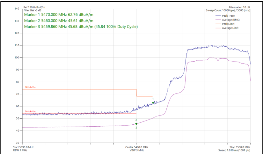
Figure 60 - 802.11ax HE40, SU, SISO, Core 0 - 5510 MHz Band Edge Frequency 5460 MHz
