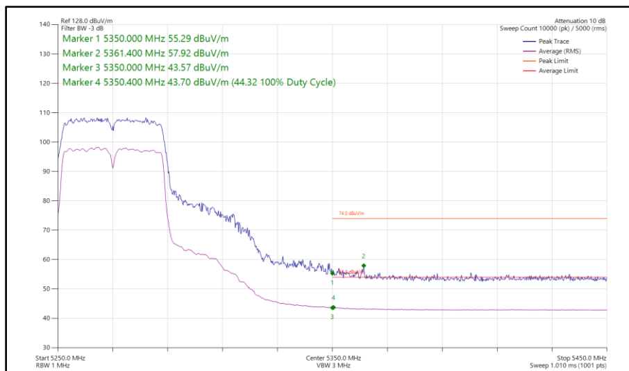
Figure 88 - 802.11n HT40, CDD, Core 0 - Core 1 - 5270 MHz Band Edge Frequency 5350 MHz
