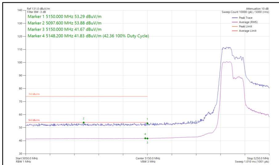
Figure 105 - 802.11ax HE40, RU 106-53, SDM, Core 0 - Core 1 - 5230 MHz Band Edge Frequency 5150 MHz
