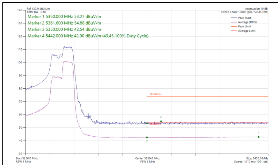
Figure 73 - 802.11ax HE40, RU 106-56, SISO, Core 1 - 5270 MHz Band Edge Frequency 5350 MHz
