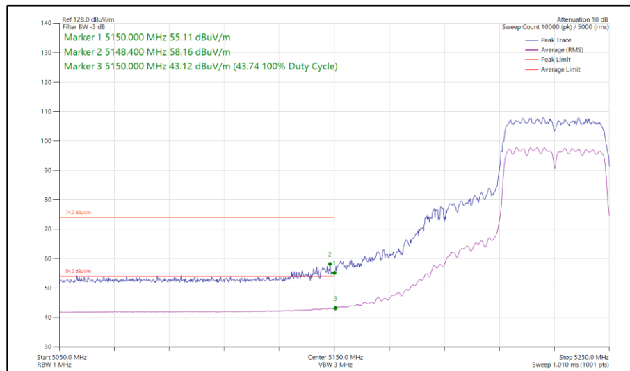
Figure 83 - 802.11n HT40, CDD, Core 0 - Core 1 - 5230 MHz Band Edge Frequency 5150 MHz
