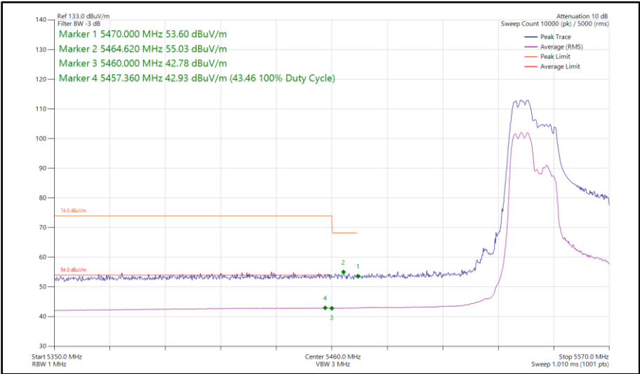
Figure 117 - 802.11ax HE40, RU 106-53, SDM, Core 0 - Core 1 - 5550 MHz Band Edge Frequency 5460 MHz
