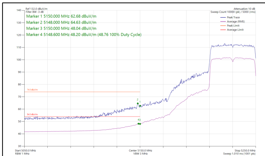
Figure 68 - 802.11ax HE40, SU, SISO, Core 1 - 5230 MHz Band Edge Frequency 5150 MHz
