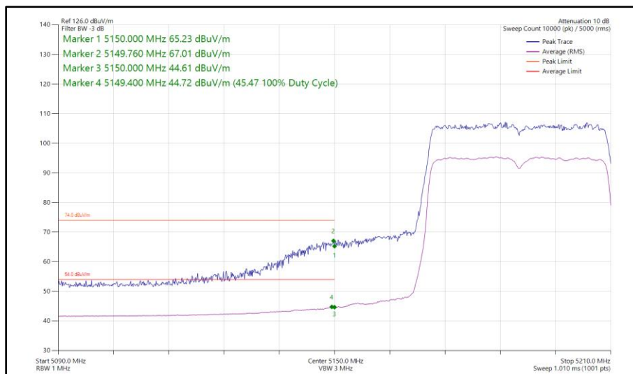
Figure 102 - 802.11ax HE40, SU, SDM, Core 0 - Core 1 - 5190 MHz Band Edge Frequency 5150 MHz
