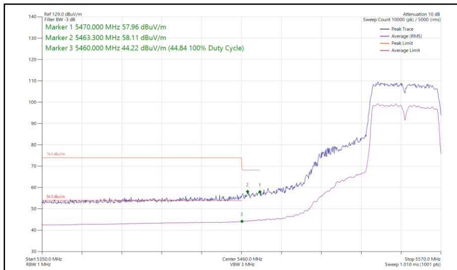
Figure 95 - 802.11n HT40, CDD, Core 0 - Core 1 - 5550 MHz Band Edge Frequency 5460 MHz
