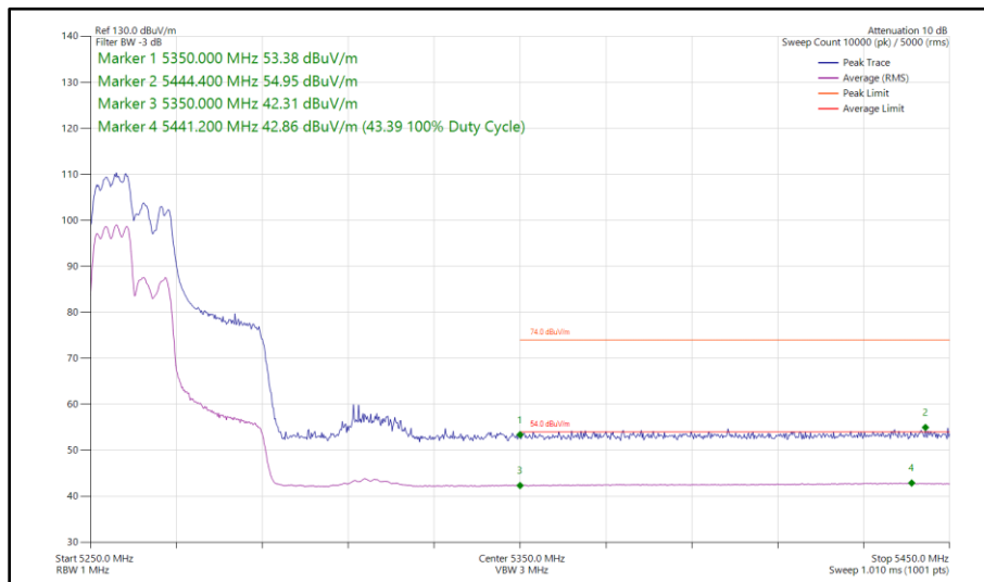
Figure 91 - 802.11ax HE40, RU 106-53, CDD, Core 0 - Core 1 - 5270 MHz Band Edge Frequency 5350 MHz
