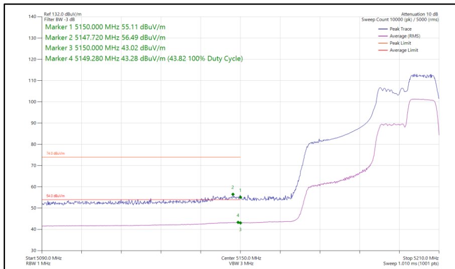
Figure 67 - 802.11ax HE40, RU 106-56, SISO, Core 1 - 5190 MHz Band Edge Frequency 5150 MHz
