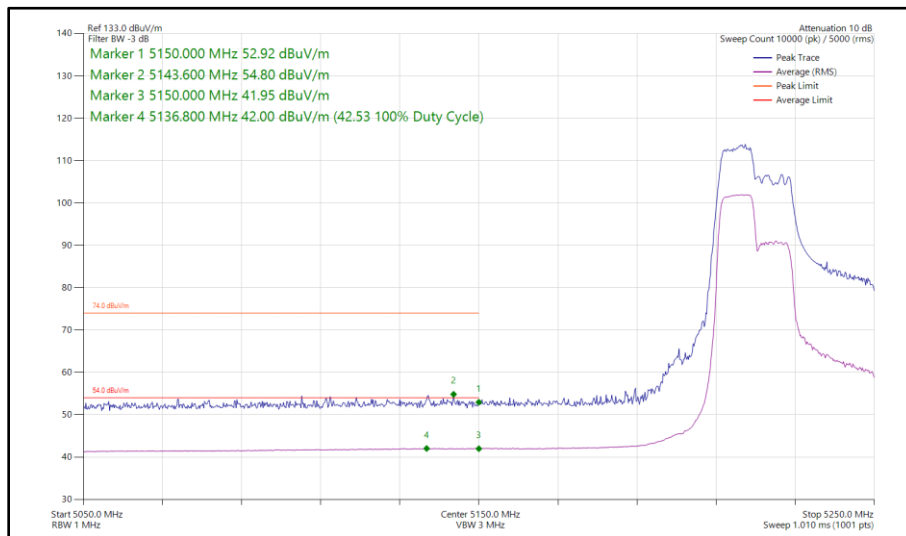
Figure 69 - 802.11ax HE40, RU 106-53, SISO, Core 1 - 5230 MHz Band Edge Frequency 5150 MHz
