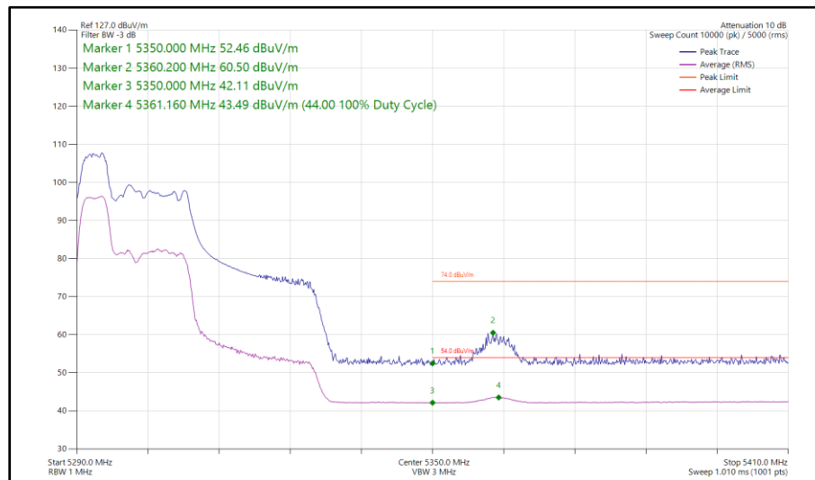
Figure 111 - 802.11ax HE40, RU 52-37, SDM, Core 0 - Core 1 - 5310 MHz Band Edge Frequency 5350 MHz
