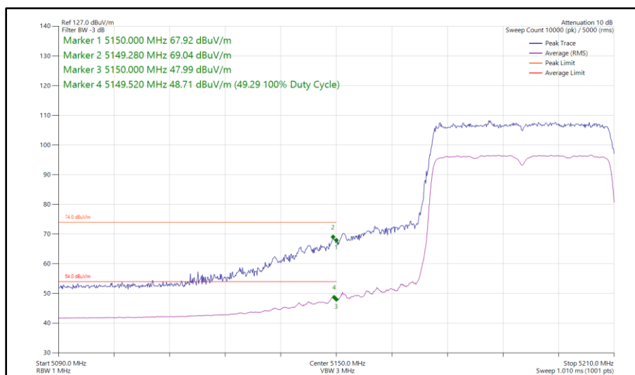
Figure 66 - 802.11ax HE40, SU, SISO, Core 1 - 5190 MHz Band Edge Frequency 5150 MHz
