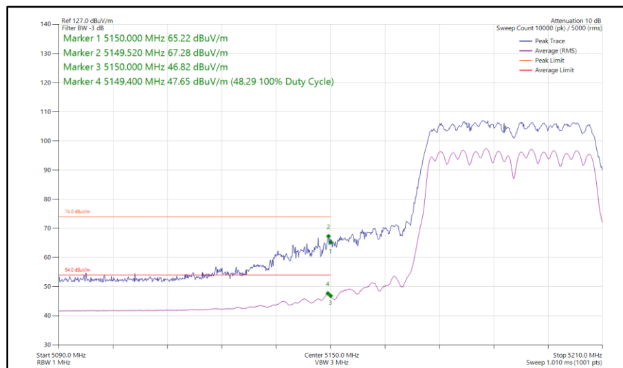
Figure 82 - 802.11n HT40, CDD, Core 0 - Core 1 - 5190 MHz Band Edge Frequency 5150 MHz
