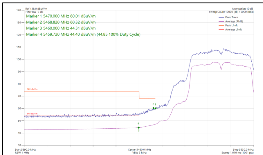
Figure 76 - 802.11n HT40, SISO, Core 1 - 5510 MHz Band Edge Frequency 5460 MHz
