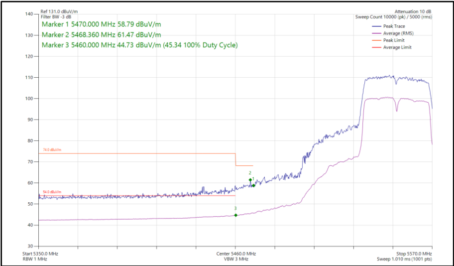
Figure 59 - 802.11n HT40, SISO, Core 0 - 5550 MHz Band Edge Frequency 5460 MHz
