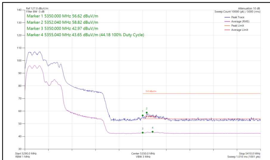
Figure 93 - 802.11ax HE40, RU 106-53, CDD, Core 0 - Core 1 - 5310 MHz Band Edge Frequency 5350 MHz
