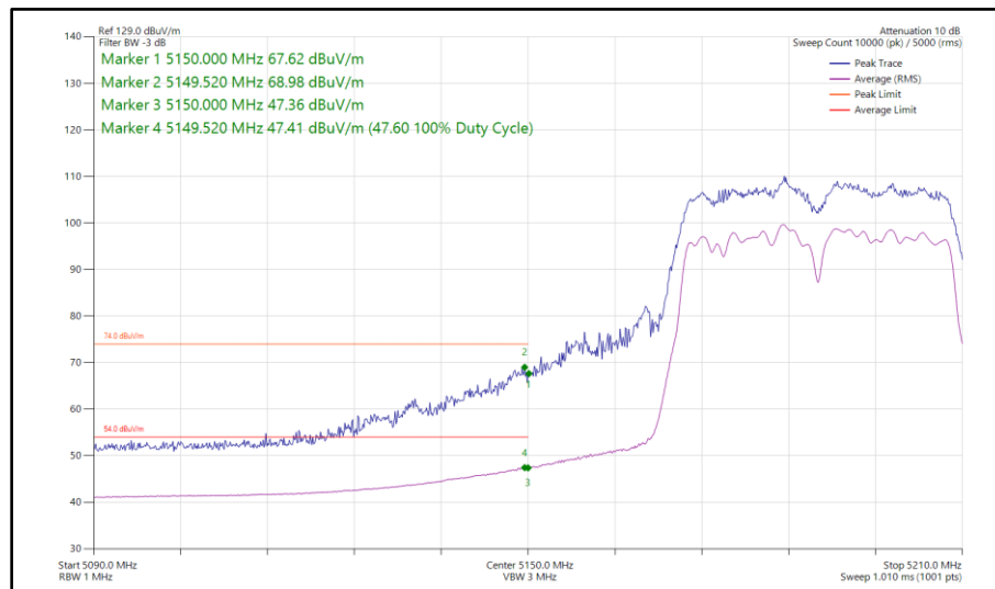
Figure 118 - 802.11ac VHT40, TxBF, Core 0 - Core 1 - 5190 MHz Band Edge Frequency 5150 MHz
