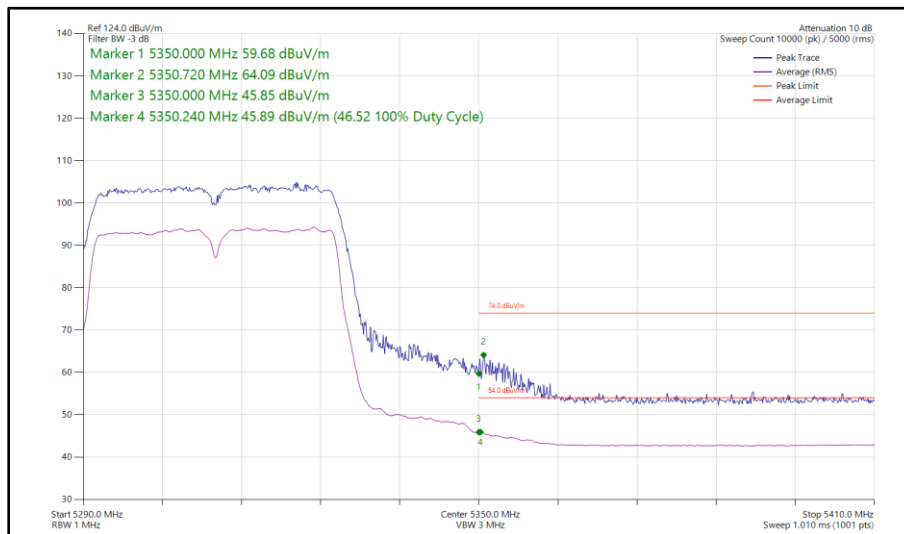
Figure 89 - 802.11n HT40, CDD, Core 0 - Core 1 - 5310 MHz Band Edge Frequency 5350 MHz
