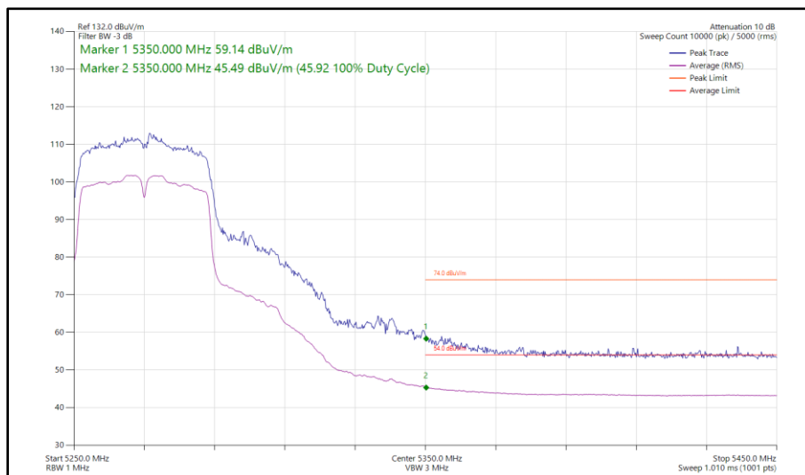
Figure 70 - 802.11n HT40, SISO, Core 1 - 5270 MHz Band Edge Frequency 5350 MHz
