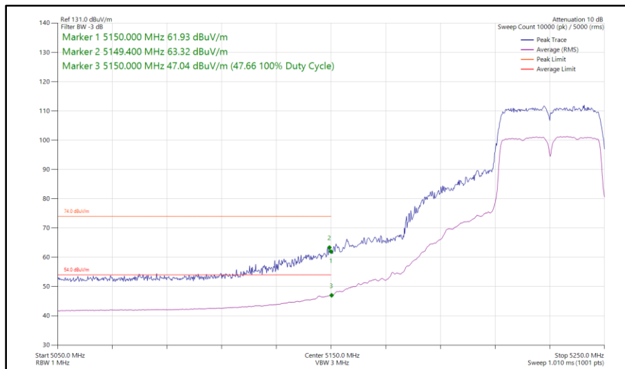
Figure 65 - 802.11n HT40, SISO, Core 1 - 5230 MHz Band Edge Frequency 5150 MHz
