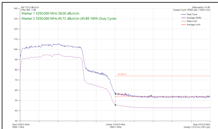
Figure 92 - 802.11ax HE40, SU, CDD, Core 0 - Core 1 - 5310 MHz Band Edge Frequency 5350 MHz
