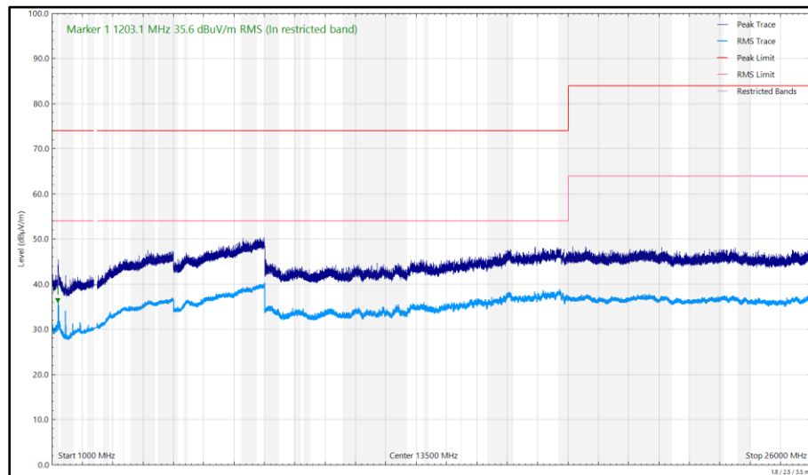
Figure 84 - 2405 MHz (CH11), Thread, iPA, Core 2, 1 GHz to 26 GHz, Vertical
