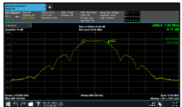
Figure 28 - Core 1 (B) 2475 MHz (CH25) 6 dB Bandwidth
