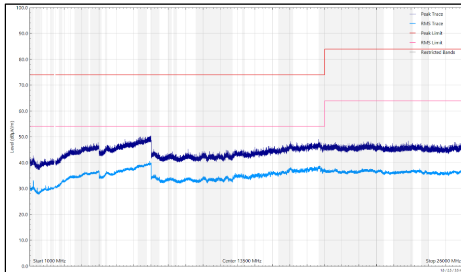
Figure 80 - 2440 MHz (CH18), Thread, iPA, Core 2, 1 GHz to 26 GHz, Horizontal
