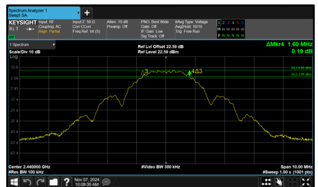
Figure 26 - Core 1 (B) 2440 MHz (CH18) 6 dB Bandwidth
