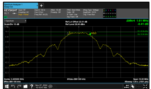
Figure 30 - Core 1 (B) 2405 MHz (CH11) 6 dB Bandwidth
