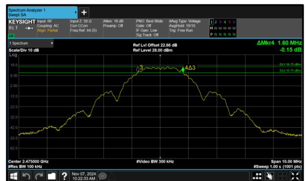
Figure 34 - Core 1 (B) 2475 MHz (CH25) 6 dB Bandwidth
