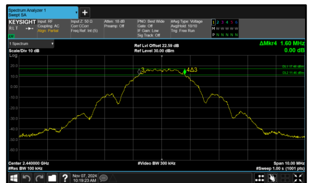
Figure 32 - Core 1 (B) 2440 MHz (CH18) 6 dB Bandwidth
