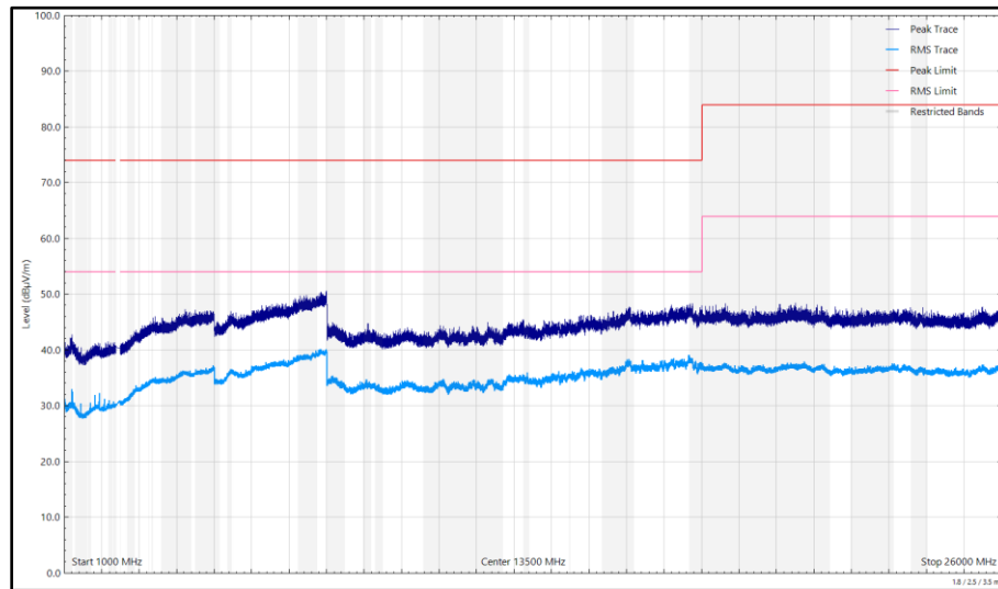
Figure 83 - 2405 MHz (CH11), Thread, iPA, Core 2, 1 GHz to 26 GHz, Horizontal
