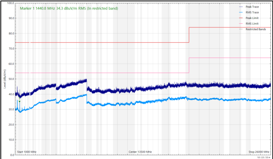
Figure 82 - 2440 MHz (CH18), Thread, iPA, Core 2, 1 GHz to 26 GHz, Vertical
