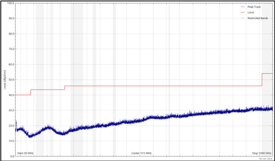
Figure 81 - 2440 MHz (CH18), Thread, iPA, Core 2, 30 MHz to 1 GHz, Vertical (Peak)
