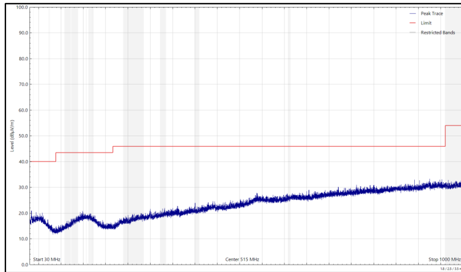
Figure 79 - 2440 MHz (CH18), Thread, iPA, Core 2, 30 MHz to 1 GHz, Horizontal (Peak)
