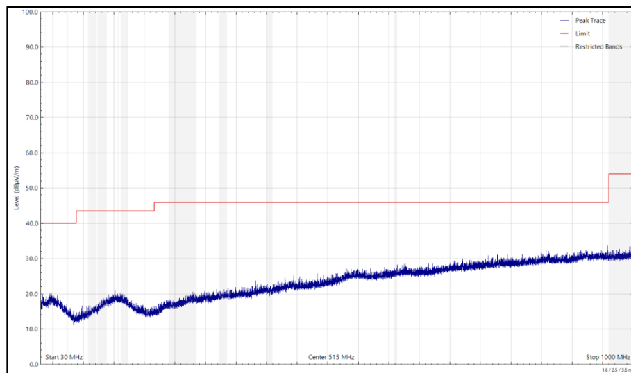
Figure 230 - 2441 MHz (CH39), 2-DH5, ePA, Core 0 + Core 1, 30 MHz to 1 GHz, Horizontal (Peak)
