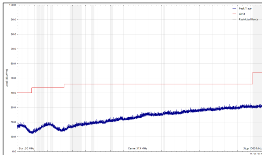
Figure 234 - 2441 MHz (CH39), DH5, iPA, Core 0 + Core 1, 30 MHz to 1 GHz, Horizontal (Peak)
