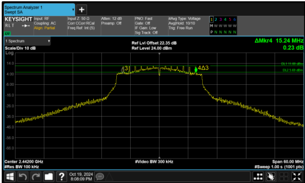
Figure 69 - 802.11n HT20 Minimum 6 dB EBW
