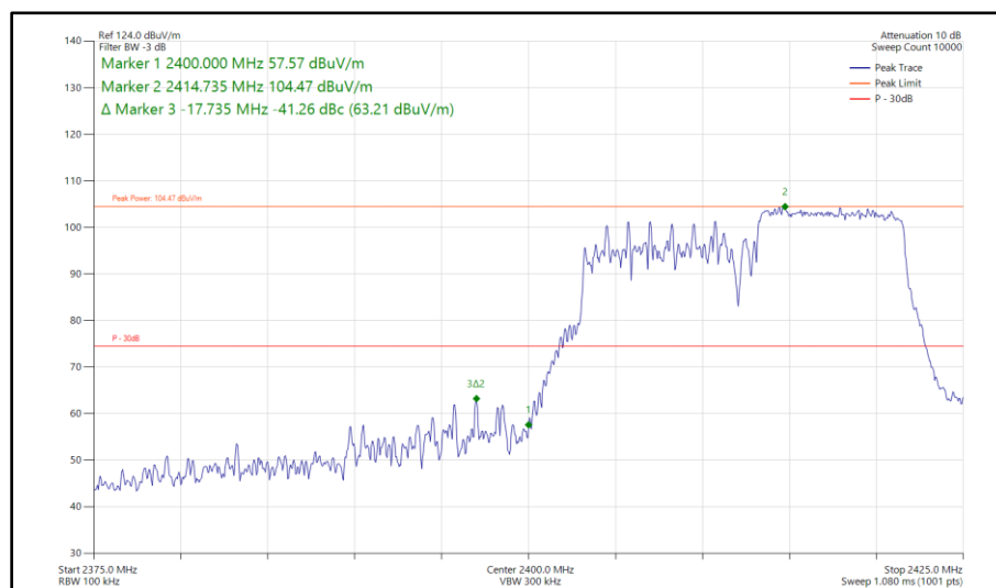
Figure 81 - 802.11ax HE20, RU 106-54, SISO, Core 0 - 2412 MHz Band Edge Frequency 2400 MHz
