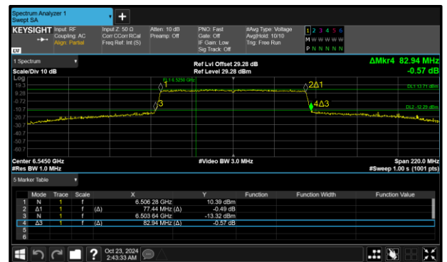
Figure 182 - 802.11ax HE80 SU SP Maximum 99% OBW
