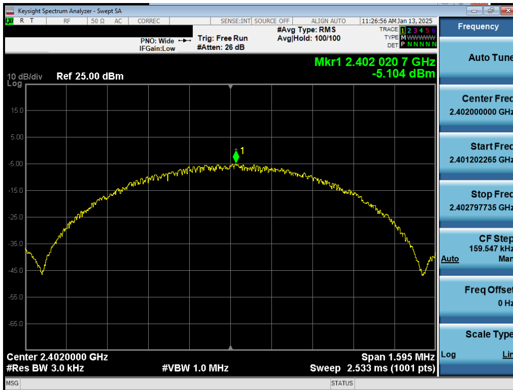
Plot 7-28. Power Spectral Density Plot Antenna 1a (Bluetooth (LE), 1Mbps, iPA – Ch. 0)
