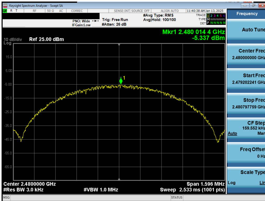
Plot 7-42. Power Spectral Density Plot Antenna 1a (Bluetooth (LE), 1Mbps, ePA – Ch. 39)
