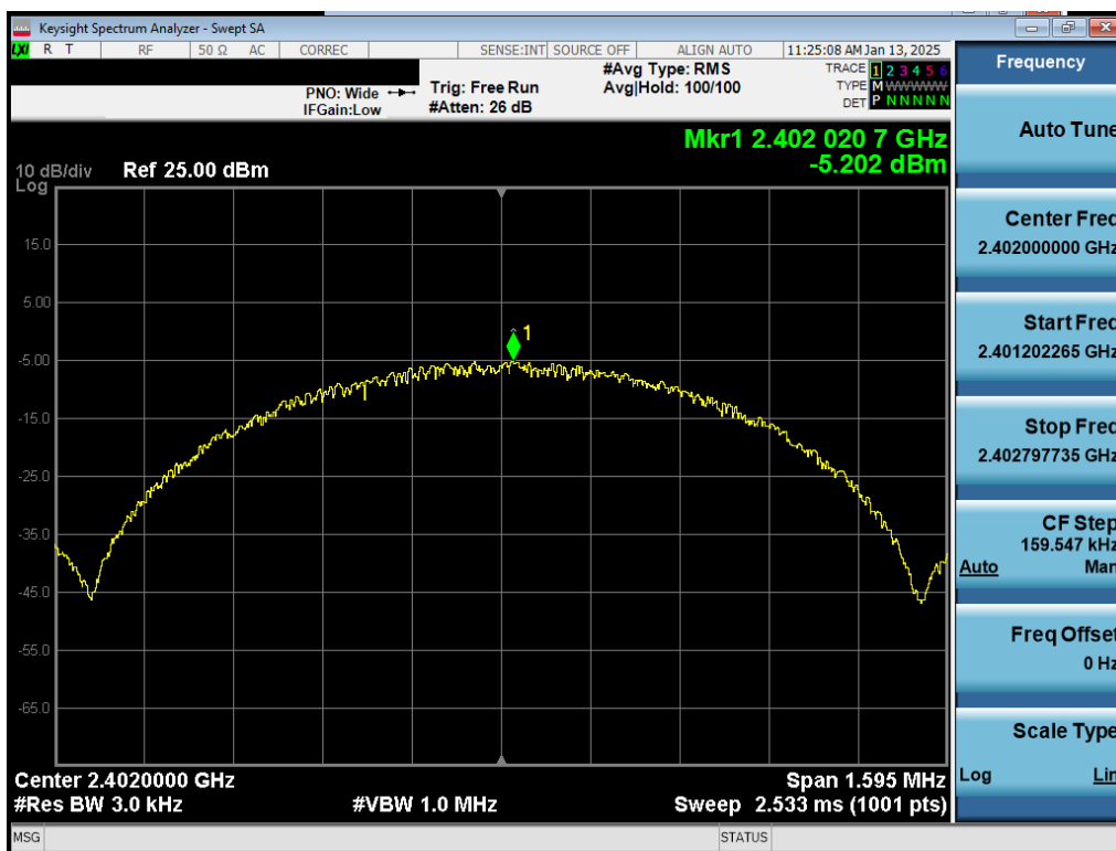
Plot 7-25. Power Spectral Density Plot Antenna 1a (Bluetooth (LE), 1Mbps, ePA – Ch. 0)
