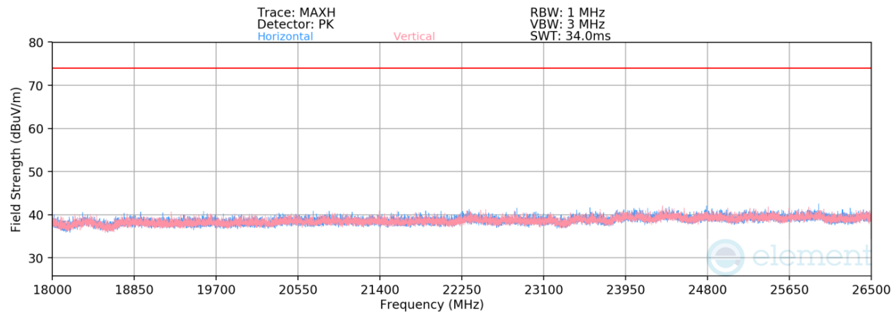
Plot 7-62. Radiated Spurious Emissions above 18GHz TxBF (BT GFSK ePA – Ch. 39)
