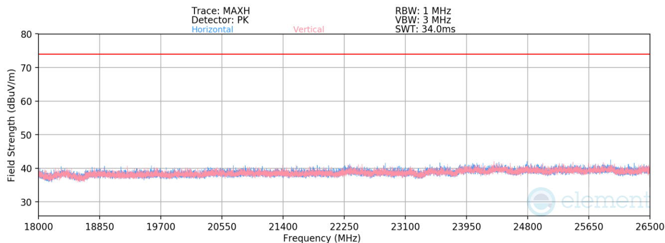
Plot 7-65. Radiated Spurious Emissions – Simultaneous Transmission Above 18GHz
