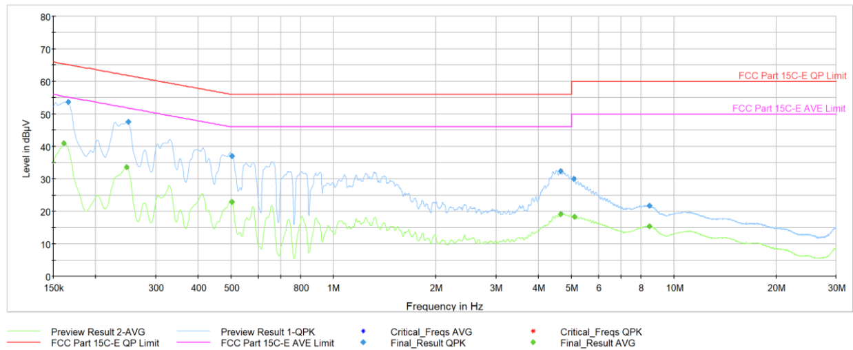
Plot 7-81. AC Line-Conducted Test Plot TxBF (N, GFSK ePA – Ch.39, via USB-C cable with wire charger)
