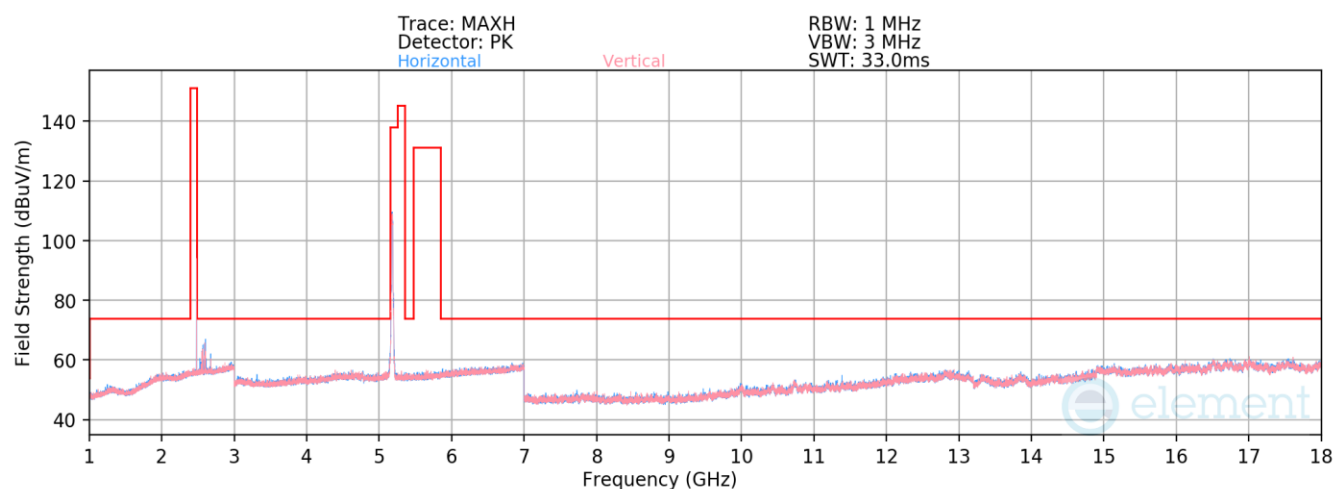
Plot 7-64. Radiated Spurious Emissions – Simultaneous Transmission Above 1GHz
