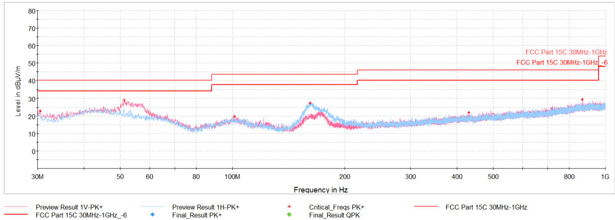
Plot 7-79. Radiated Spurious Emissions – Simultaneous Transmission Below 1GHz (via USB-C cable with wire charger)
