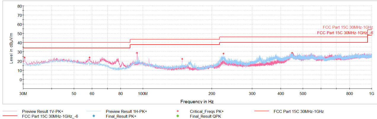
Plot 7-78. Radiated Spurious Emissions Below 1GHz TxBF (GFSK ePA – Ch.39, via USB-C cable with wire charger)
