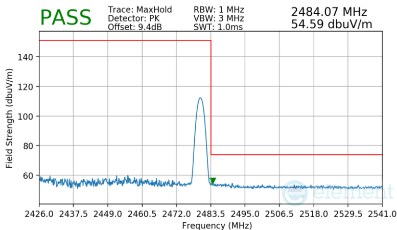
Plot 7-73. Radiated Restricted Upper Band Edge Measurement Antenna 1a
