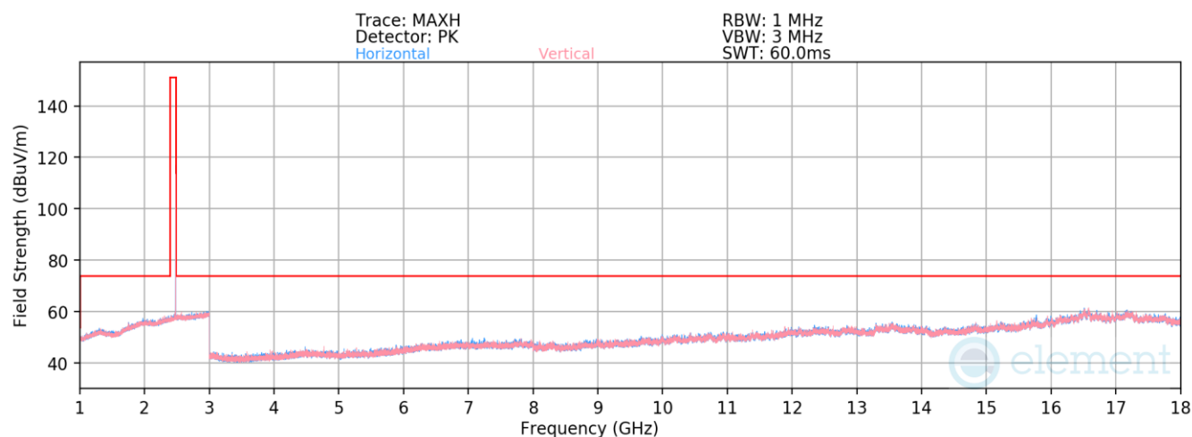
Plot 7-63. Radiated Spurious Emissions above 1GHz TxBF (BT GFSK ePA – Ch. 78)
