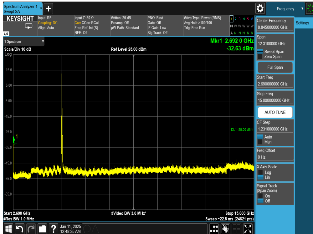
Plot 7-58. Conducted Simultaneous Tx Spurious Plots Antenna 3a (Bluetooth + LTE B41 + UNII)
