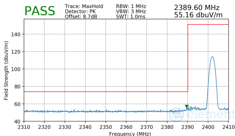
Plot 7-75. Radiated Restricted Lower Band Edge Measurement TxBF
