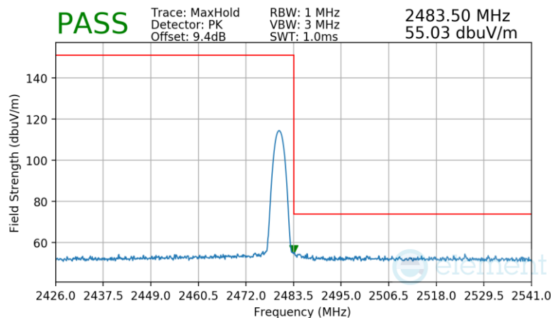
Plot 7-77. Radiated Restricted Upper Band Edge Measurement TxBF
