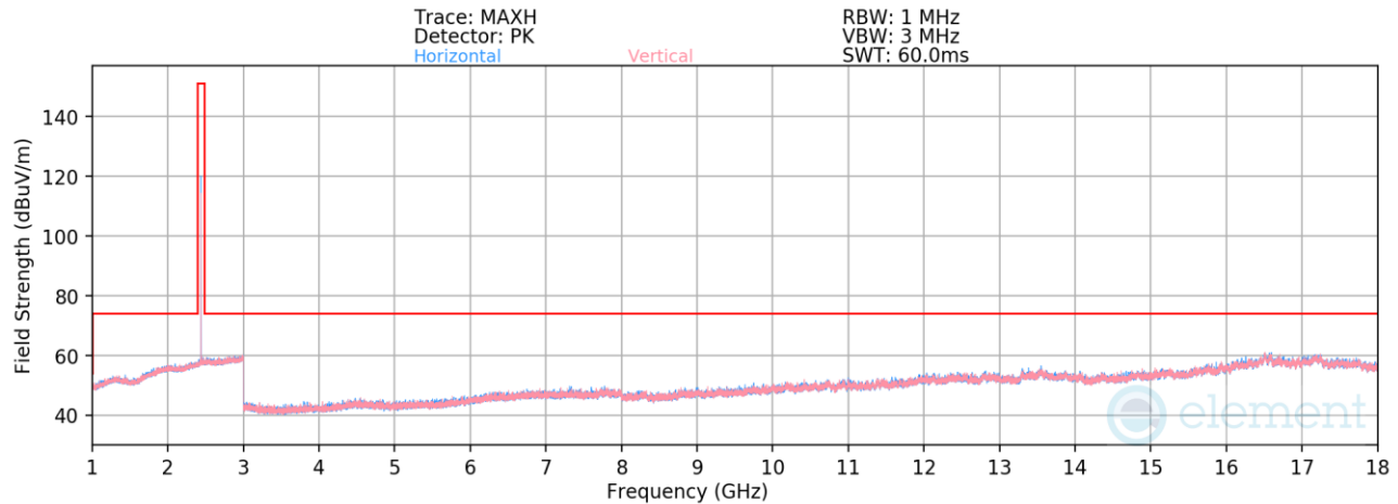
Plot 7-61. Radiated Spurious Emissions above 1GHz TxBF (BT GFSK ePA – Ch. 39)
