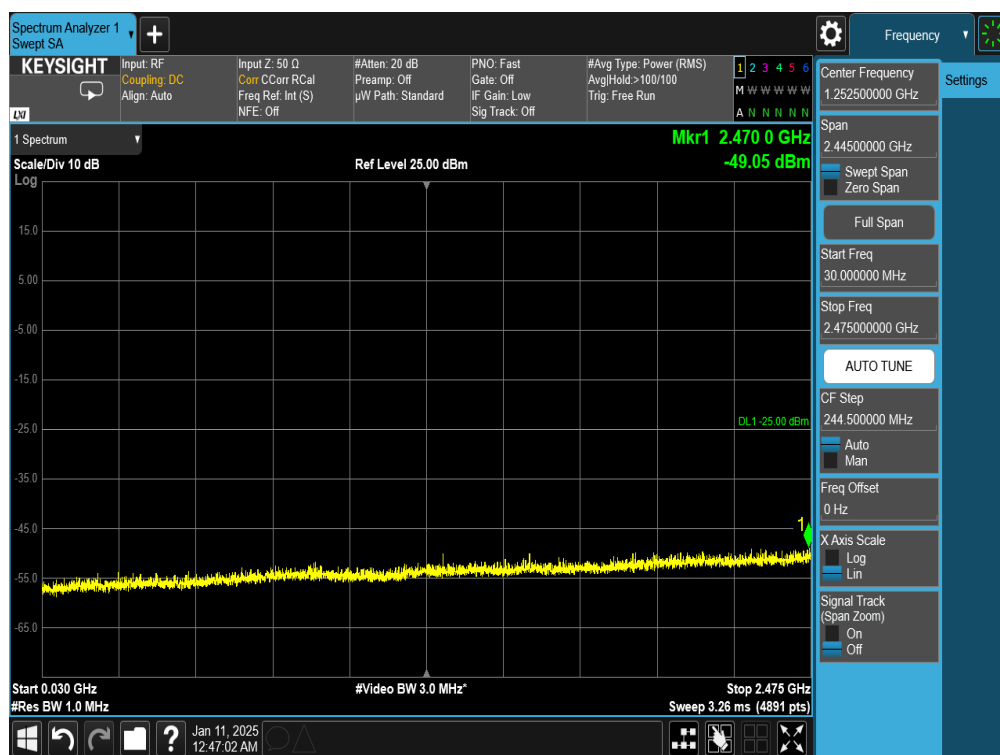
Plot 7-57. Conducted Simultaneous Tx Spurious Plots Antenna 3a (Bluetooth + LTE B41 + UNII)
