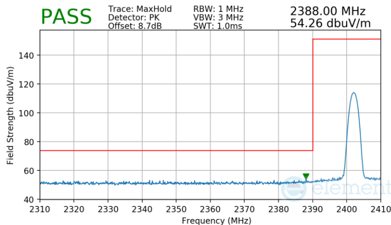
Plot 7-67. Radiated Restricted Lower Band Edge Measurement Antenna 3a
