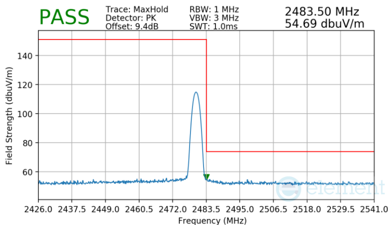
Plot 7-69. Radiated Restricted Upper Band Edge Measurement Antenna 3a
