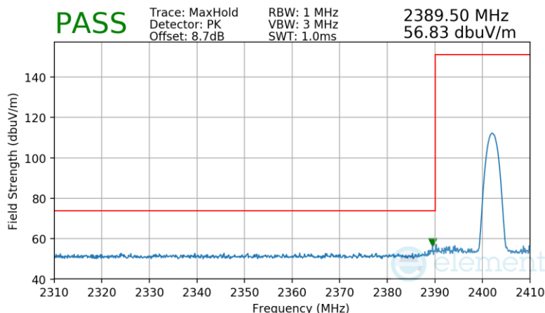
Plot 7-71. Radiated Restricted Lower Band Edge Measurement Antenna 1a
