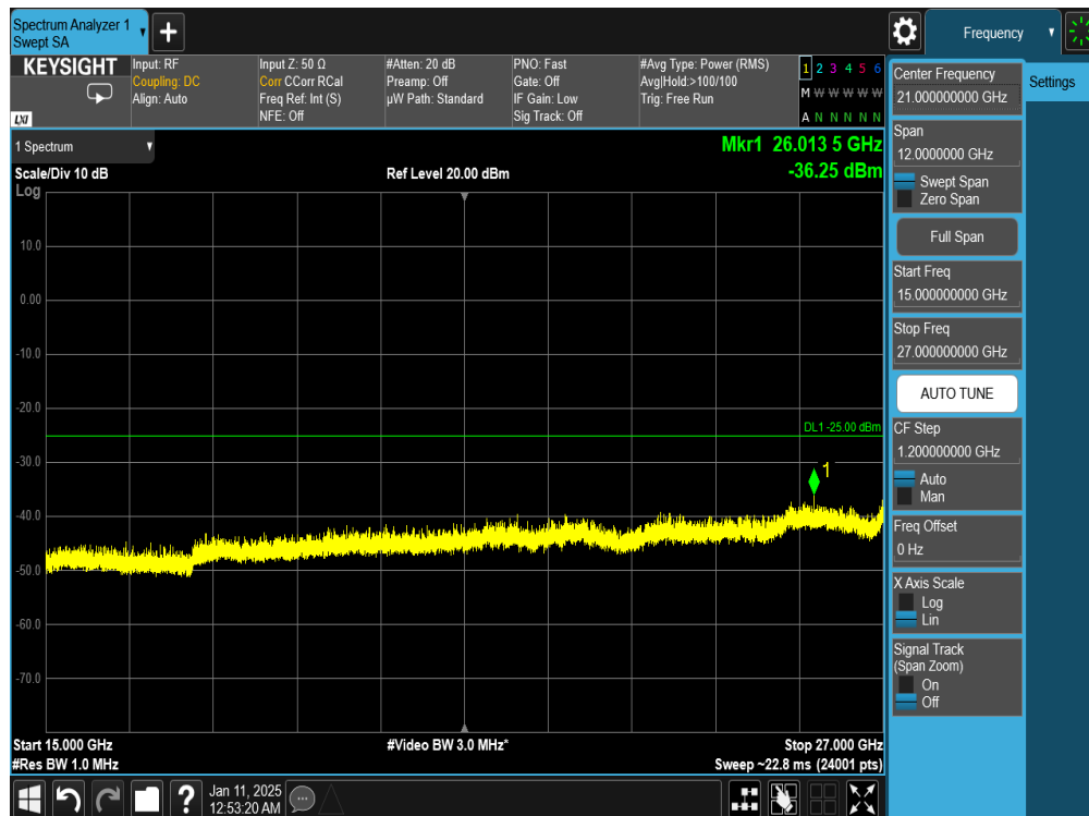
Plot 7-59. Conducted Simultaneous Tx Spurious Plots Antenna 3a (Bluetooth + LTE B41 + UNII)
