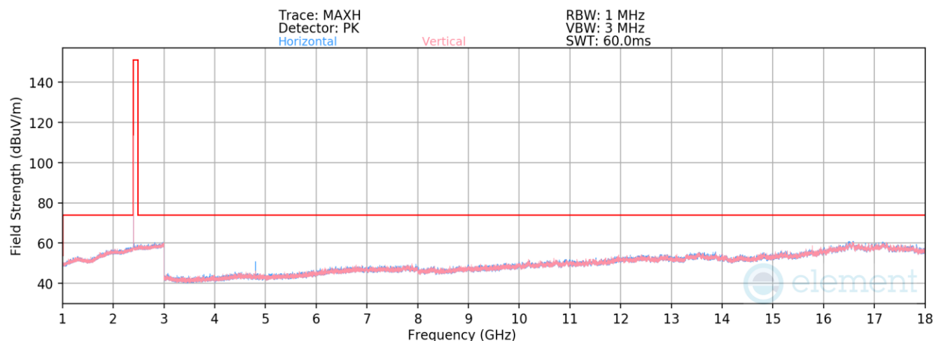
Plot 7-60. Radiated Spurious Emissions above 1GHz TxBF (BT GFSK ePA – Ch. 0)
