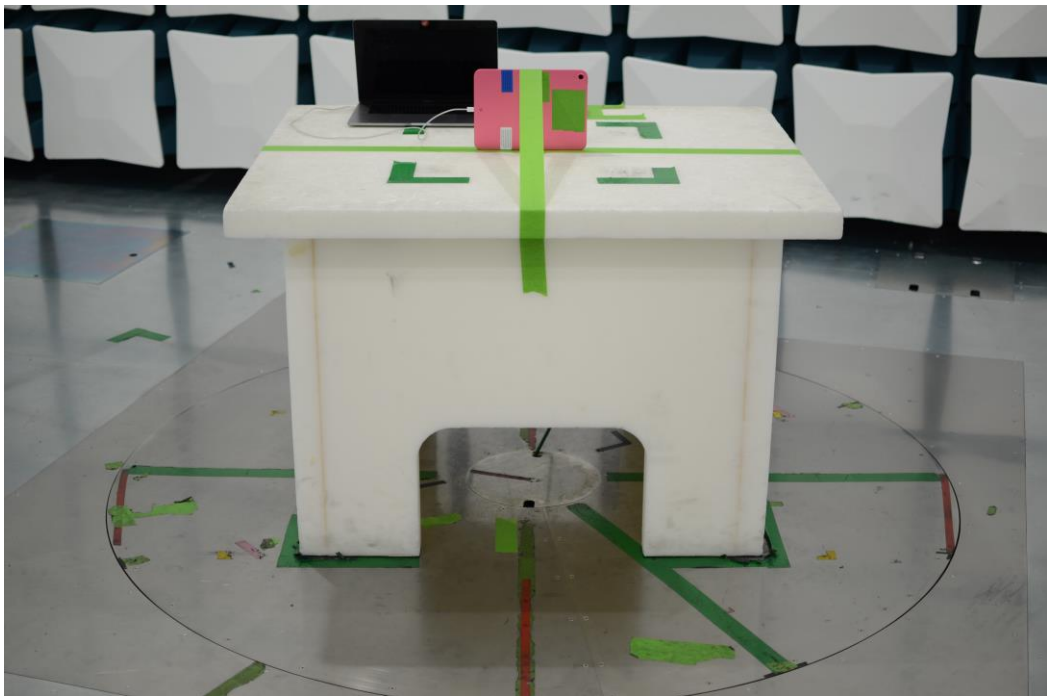
Figure 19: 30MHz-1GHz Test Setup (Front View)
