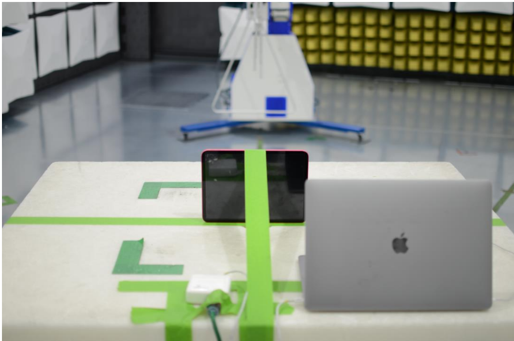
Figure 20: 30MHz-1GHz Test Setup (Rear View)
