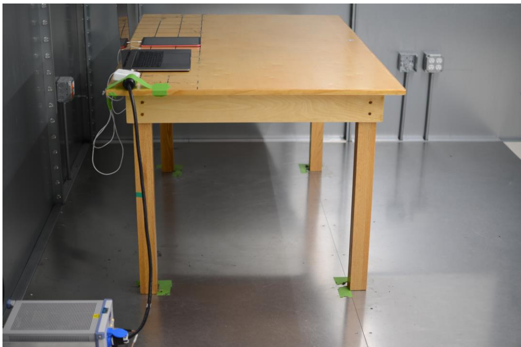
Figure 4: AC Line Conducted Emissions (Side View)
