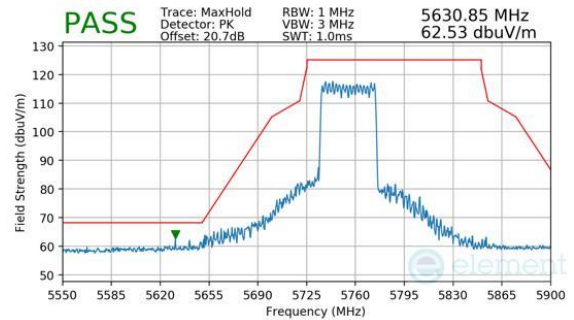
Plot 7-263. CDD (Peak, RU484, Index 65, Ch.151, MCS11)
