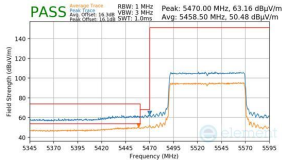
Plot 7-206. Antenna WF8 (Peak & Average, RU996, Index 67, Ch.106, MCS11)
