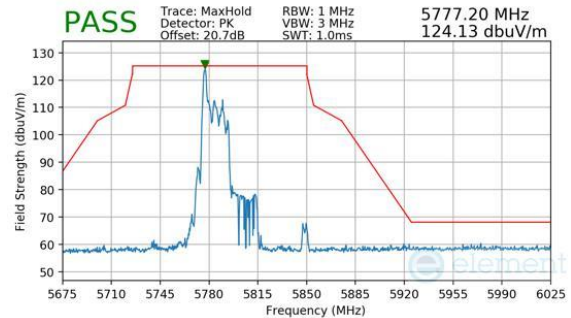
Plot 7-243. CDD (Peak, RU26, Index 0, Ch.159, MCS11)
