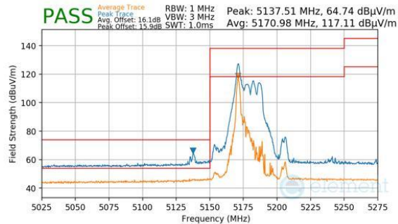
Plot 7-211. SDM (Peak & Average, RU26, Index 0, Ch.36, MCS11)
