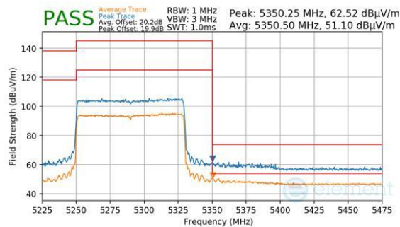
Plot 7-205. Antenna WF8 (Peak & Average, RU996, Index 67, Ch.58, MCS11)
