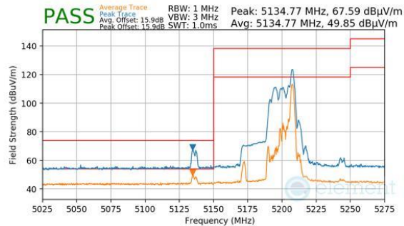
Plot 7-240. SDM (Peak & Average, RU26, Index 17, Ch.38, MCS11)
