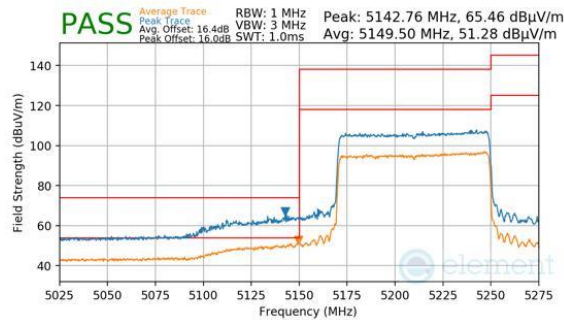
Plot 7-204. Antenna WF8 (Peak & Average, RU996, Index 67, Ch.42, MCS11)
