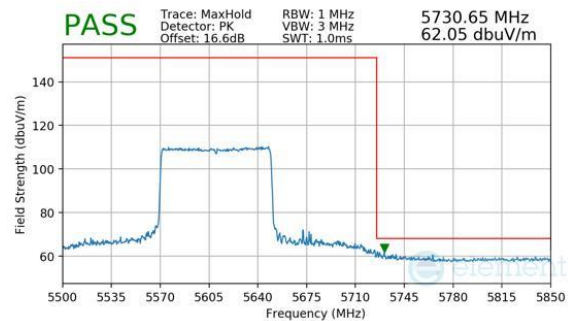
Plot 7-208. (FCC Only) Antenna WF8 (Peak, RU996, Index 67, Ch.122, MCS11)
