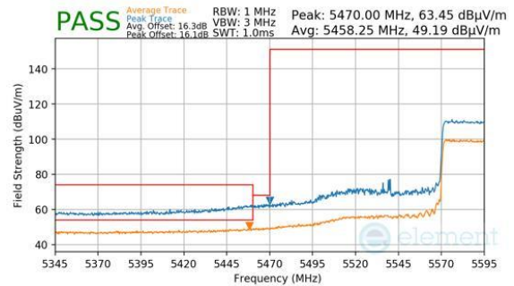
Plot 7-207. (FCC Only) Antenna WF8 (Peak & Average, RU996, Index 67, Ch.122, MCS11)
