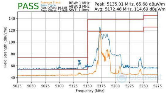
Plot 7-239. SDM (Peak & Average, RU26, Index 0, Ch.38, MCS11)
