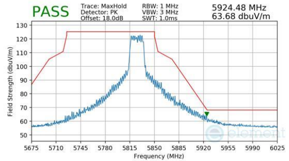
Plot 7-238. CDD (Peak, RU242, Index 61, Ch.165, MCS11)
