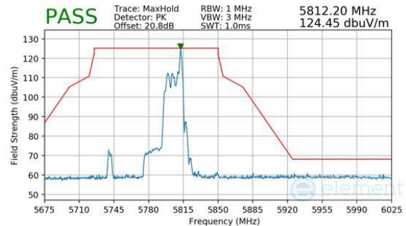
Plot 7-244. CDD (Peak, RU26, Index 17, Ch.159, MCS11)
