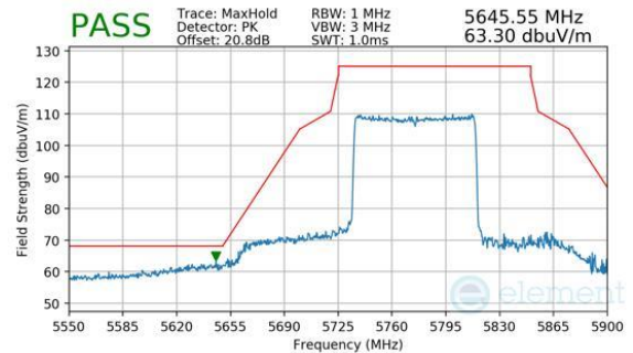
Plot 7-209. Antenna WF8 (Peak, RU996, Index 67, Ch.155, MCS11)
