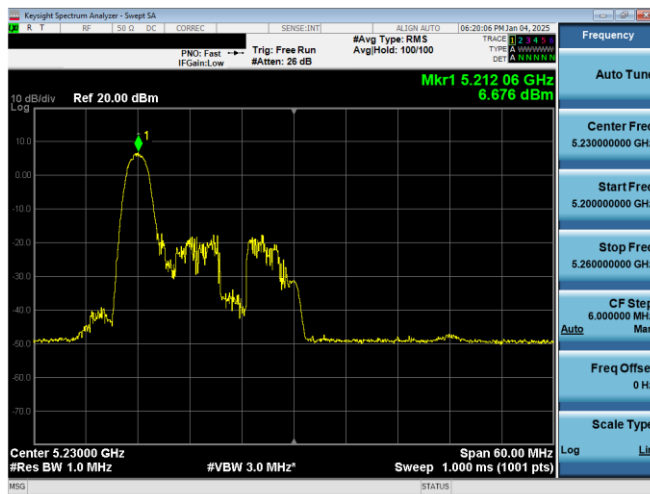
Plot 7-21. PSD SDM Antenna WF7a (20MHz BW 11ax Index 0 - RU26 - Ch.46)
