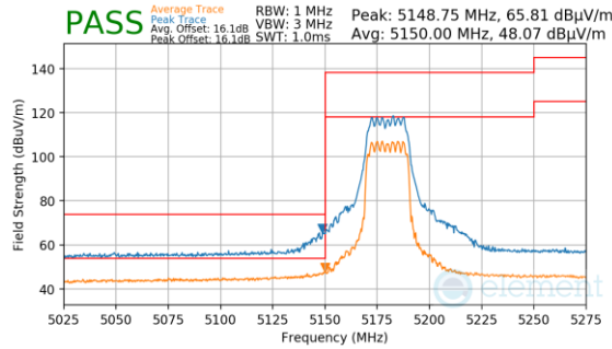
Plot 7-229. CDD (Peak & Average, Ch.36, 802.11ax(SU), MCS15)
