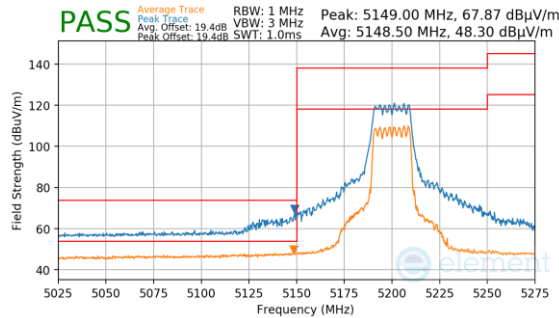
Plot 7-230. CDD (Peak & Average, Ch.40, 802.11ax(SU), MCS15)
