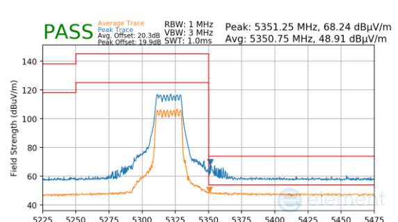
Plot 7-234. CDD (Peak & Average, Ch.64, 802.11ax(SU), MCS15)
