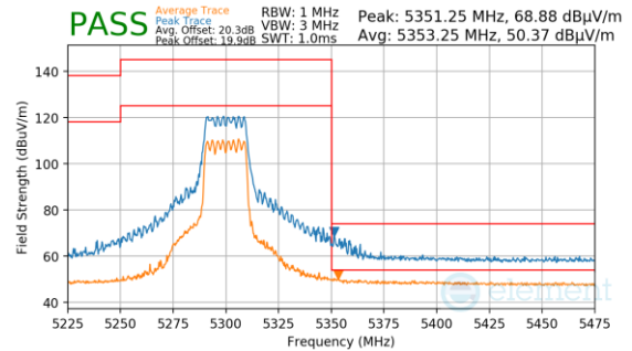
Plot 7-233. SDM (Peak & Average, Ch.60, 802.11ax(SU), MCS15)
