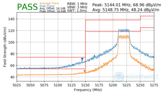
Plot 7-231. SDM (Peak & Average, Ch.44, 802.11ax(SU), MCS15)
