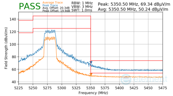
Plot 7-232. SDM (Peak & Average, Ch.56, 802.11ax(SU), MCS15)
