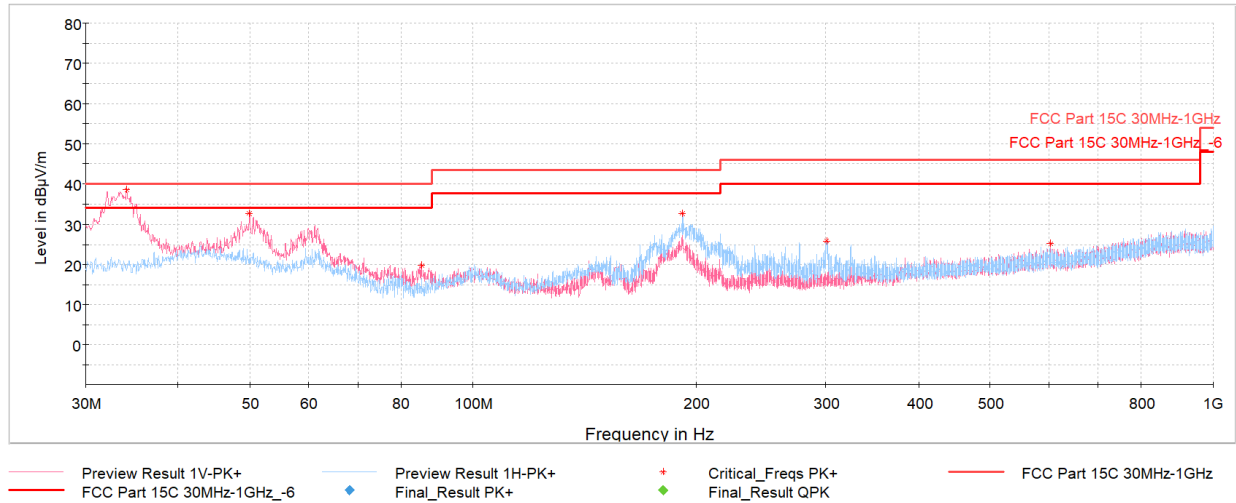
Plot 7-283. Radiated Spurious Emissions below 1GHz SDM, 802.11n, Ch.40 with AC/DC Adapter
