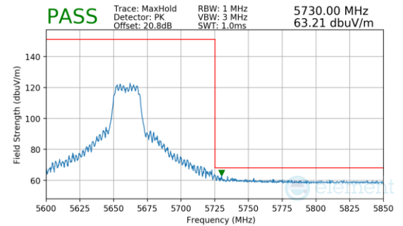
Plot 7-240. SDM (Peak, Ch.132, 802.11ax(SU), MCS15)
