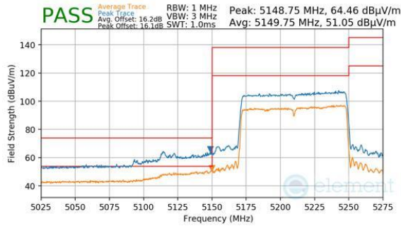
Plot 7-203. Antenna WF8 (Peak & Average, Ch.42, 802.11ac, MCS9)
