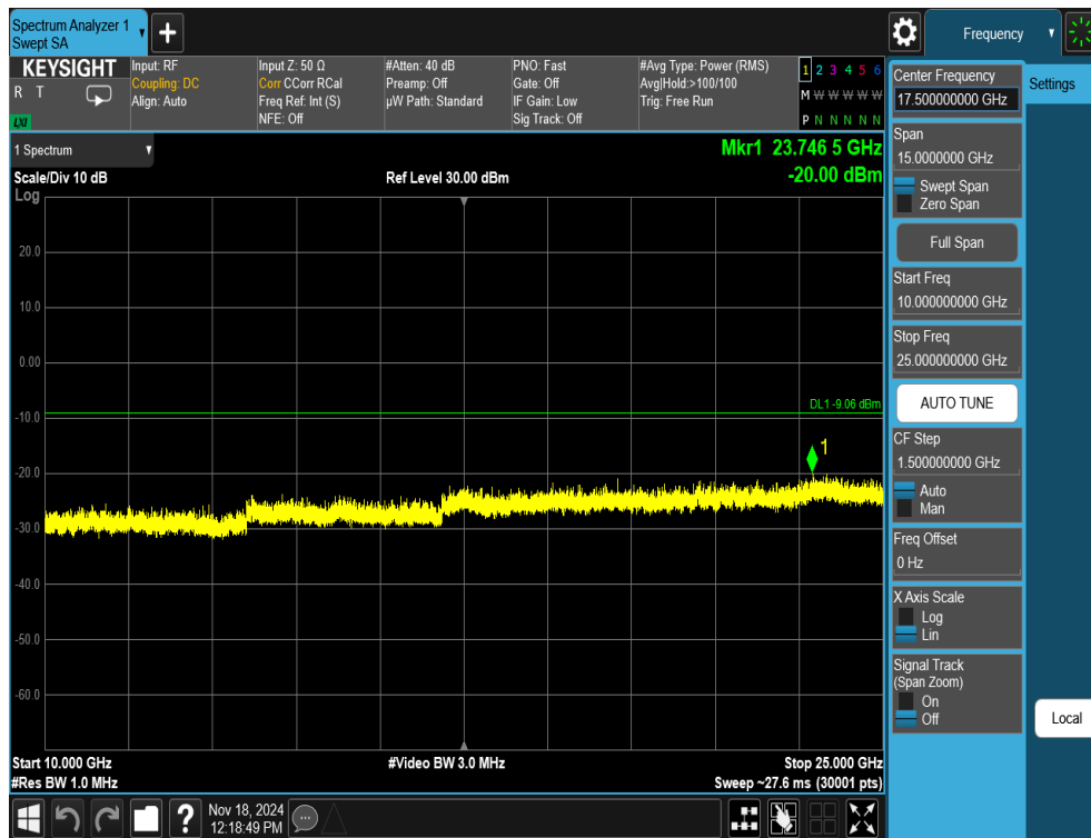
Plot 7-69. Conducted Spurious Plot Antenna WF8 (802.11ax OFDMA – RU242 – Ch. 1)
