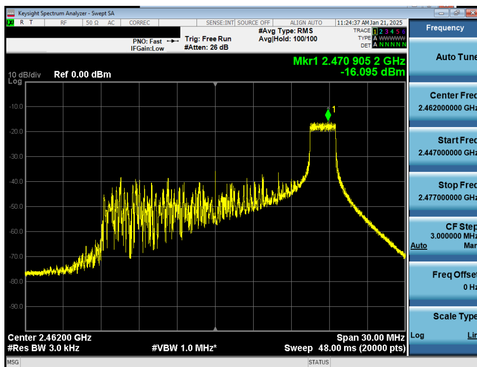
Plot 7-14. Power Spectral Density Plot Antenna WF7b (802.11ax OFDMA – RU26 – Ch. 11)
