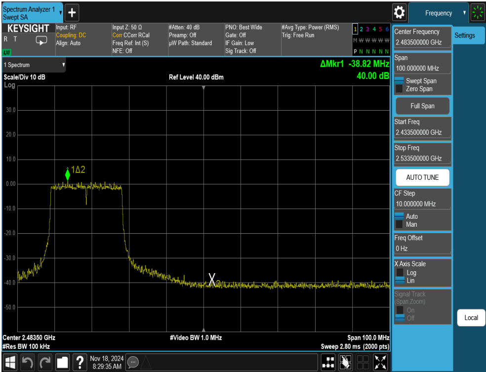
Plot 7-45. Band Edge Antenna WF8 (Common) (802.11ax OFDMA – RU242 – Ch. 9)
