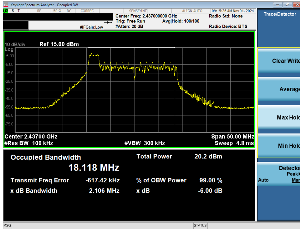
Plot 7-1. 6dB BW & 99% OBW Plot Antenna WF8 (802.11ax OFDMA – RU26 – Ch. 6)
