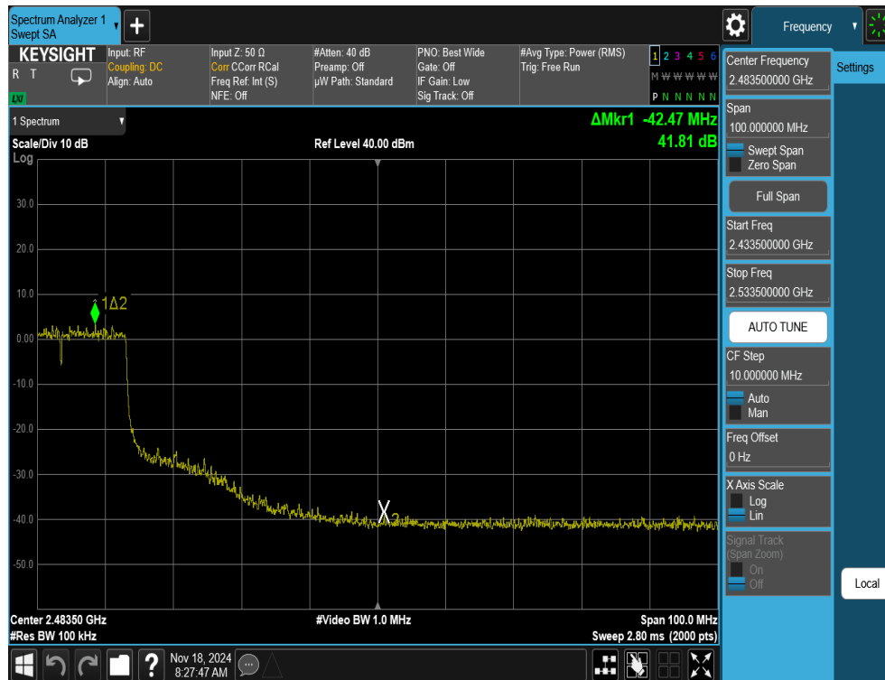
Plot 7-42. Band Edge Antenna WF8 (Common) (802.11ax OFDMA – RU242 – Ch. 6(High Channel))
