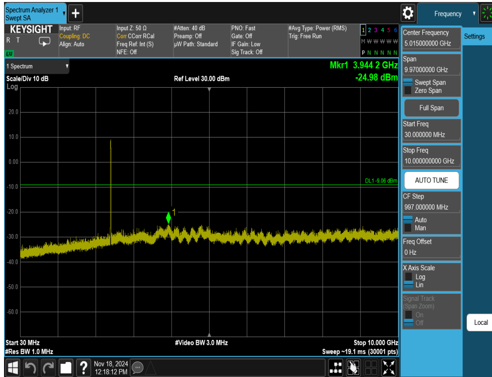
Plot 7-68. Conducted Spurious Plot Antenna WF8 (802.11ax OFDMA – RU242 – Ch. 1)
