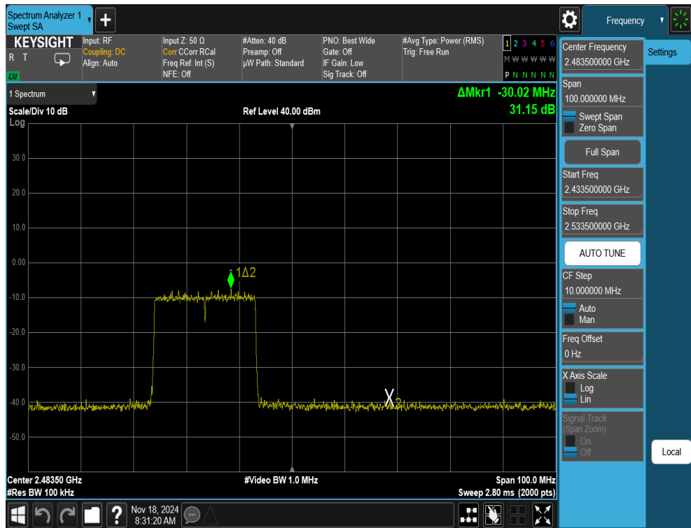
Plot 7-48. Band Edge Antenna WF8 (Common) (802.11ax OFDMA – RU242 – Ch. 12)
