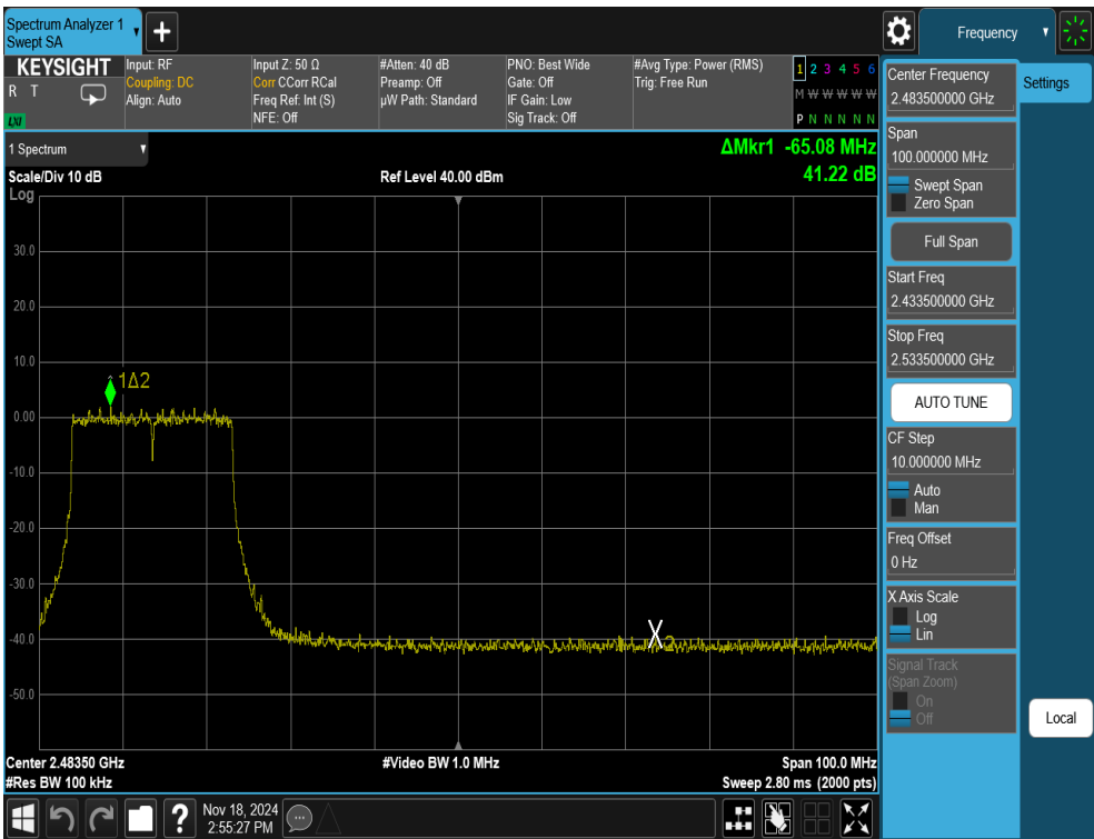
Plot 7-57. Band Edge Antenna WF7b (802.11ax OFDMA – RU242 – Ch. 8)
