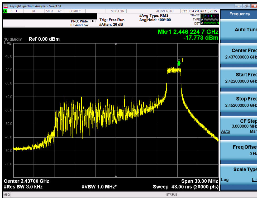
Plot 7-9. Power Spectral Density Plot Antenna WF8 (Common) (802.11ax OFDMA – RU26 – Ch. 6)
