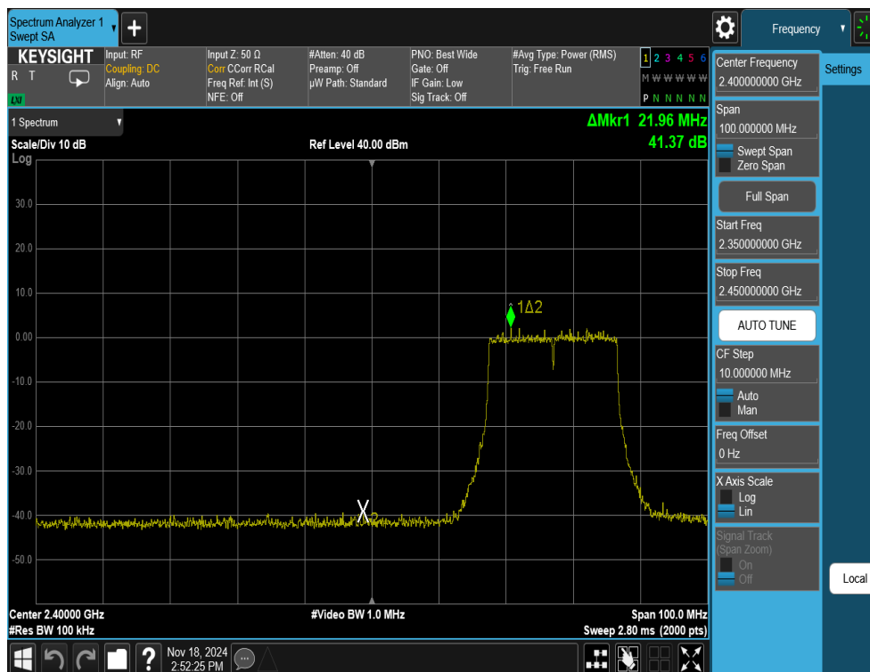
Plot 7-54. Band Edge Antenna WF7b (802.11ax OFDMA – RU242 – Ch. 4)
