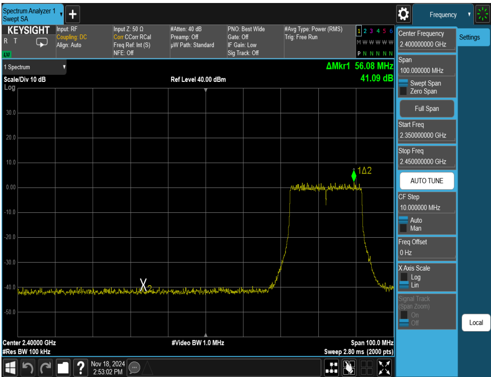
Plot 7-55. Band Edge Antenna WF7b (802.11ax OFDMA – RU242 – Ch. 5)
