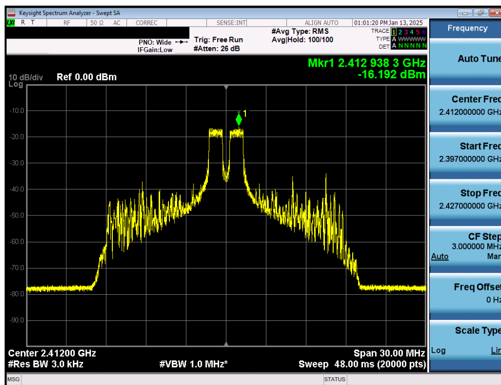
Plot 7-7. Power Spectral Density Plot Antenna WF8 (Dedicated) (802.11ax OFDMA – RU26 – Ch. 1)
