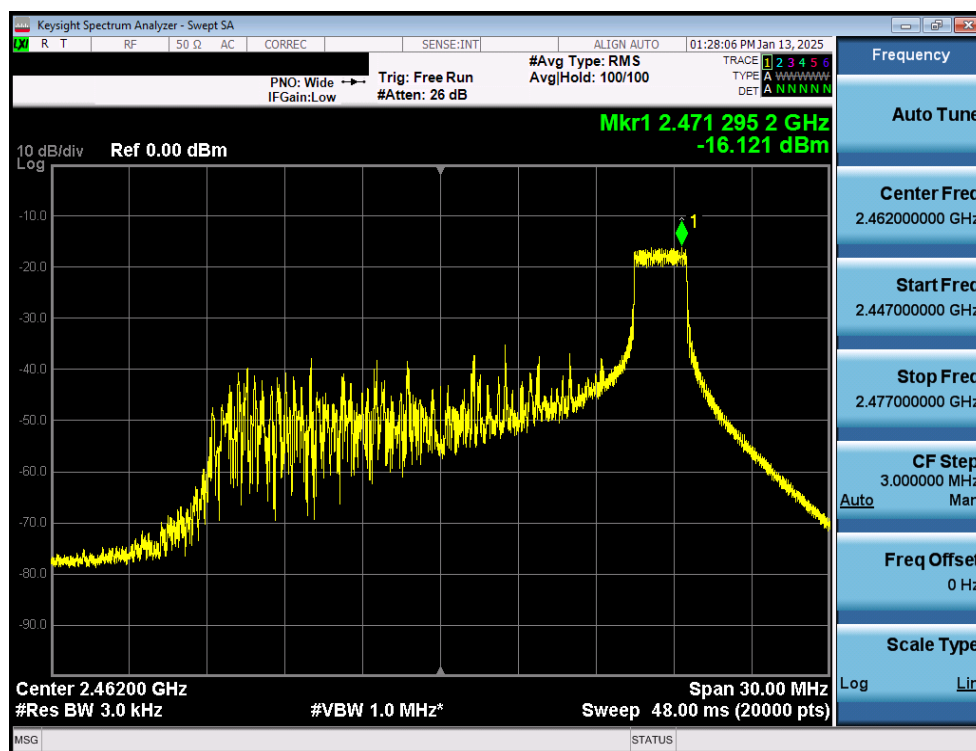
Plot 7-13. Power Spectral Density Plot Antenna WF8 (802.11ax OFDMA – RU26 – Ch. 11)
