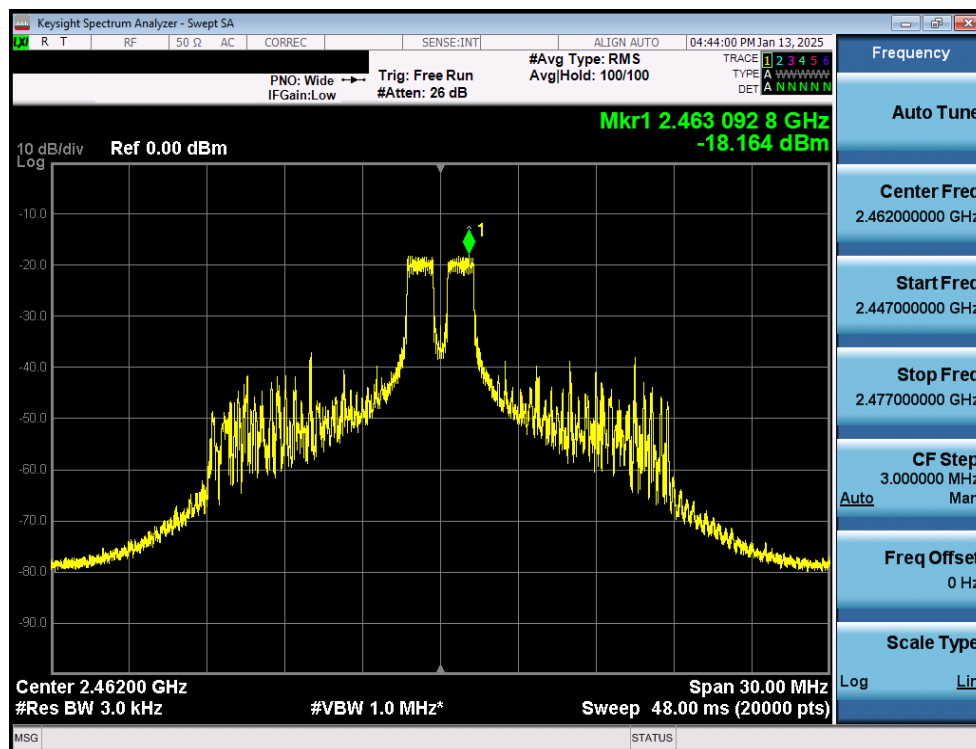
Plot 7-17. Power Spectral Density Plot Antenna WF8 (802.11ax OFDMA – RU26 – Ch. 11)
