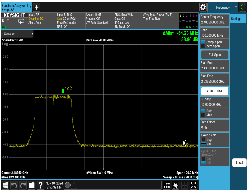
Plot 7-59. Band Edge Antenna WF7b (802.11ax OFDMA – RU242 – Ch. 10)
