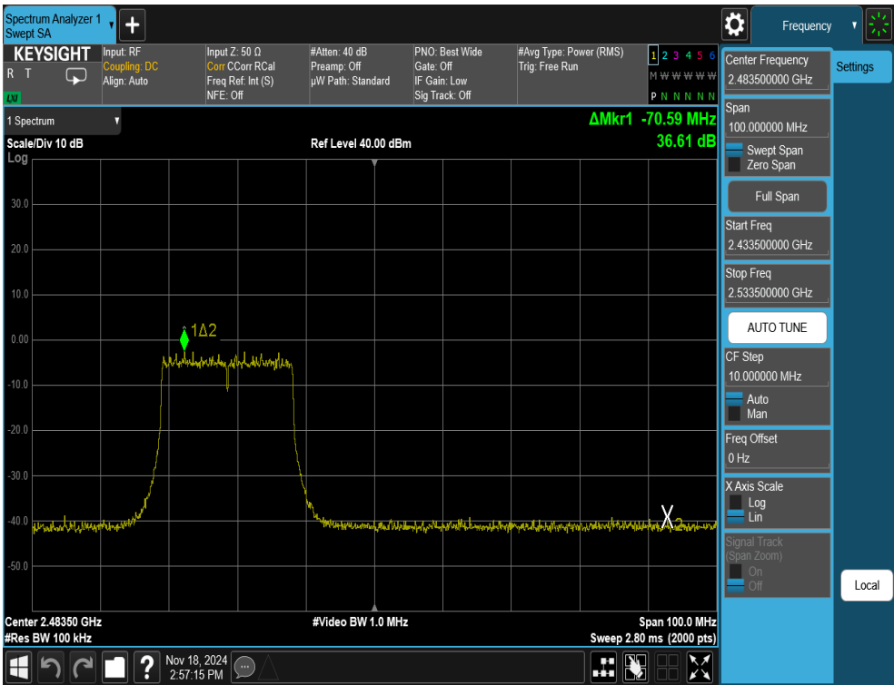
Plot 7-60. Band Edge Antenna WF7b (802.11ax OFDMA – RU242 – Ch. 11)
