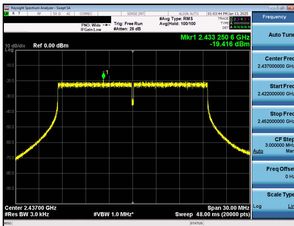
Plot 7-8. Power Spectral Density Plot Antenna WF8 (Dedicated) (802.11ax OFDMA – RU242 – Ch. 6)
