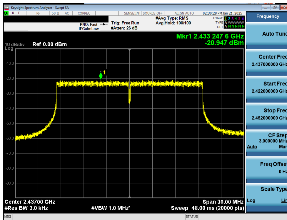
Plot 7-19. Power Spectral Density Plot Antenna WF8 (802.11ax OFDMA – RU242 – Ch. 6)
