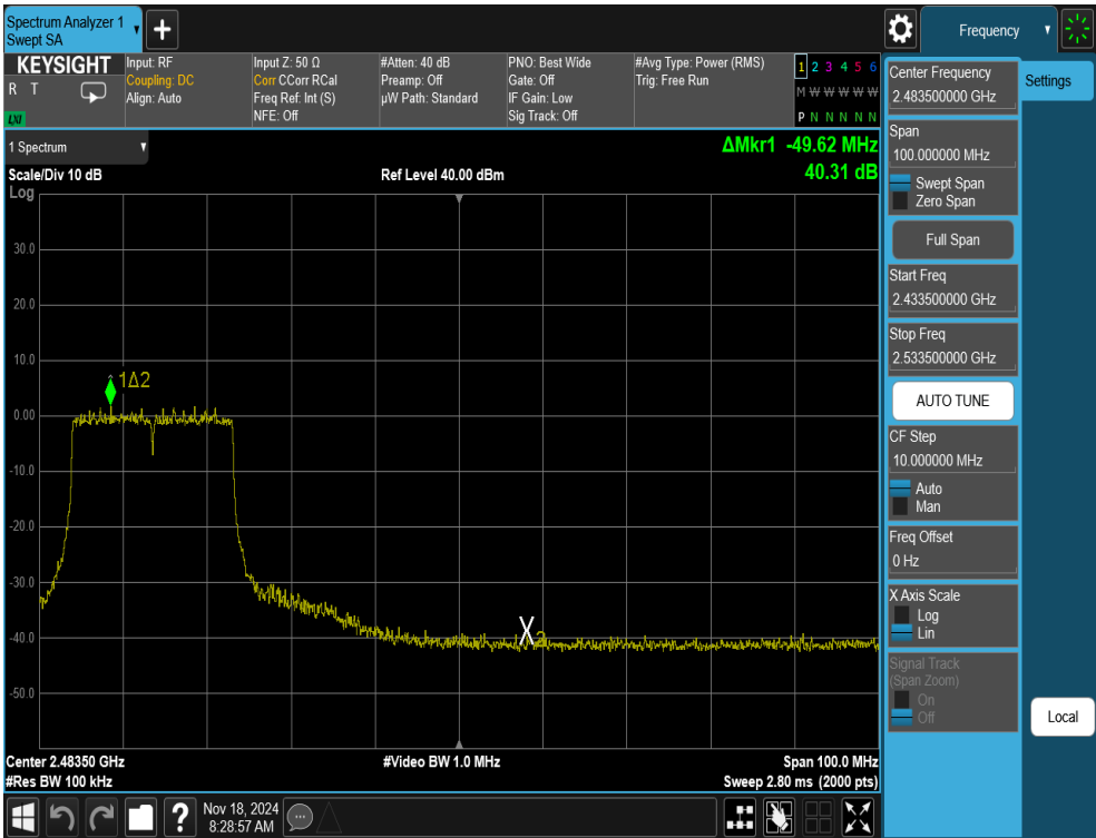
Plot 7-44. Band Edge Antenna WF8 (Common) (802.11ax OFDMA – RU242 – Ch. 8)
