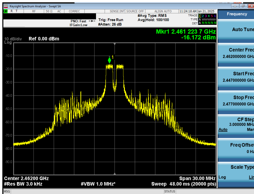
Plot 7-18. Power Spectral Density Plot Antenna WF7b (802.11ax OFDMA – RU26 – Ch. 11)
