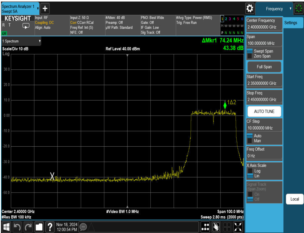
Plot 7-28. Band Edge Antenna WF8 (802.11ax OFDMA – RU242 – Ch. 6(Low Channel))
