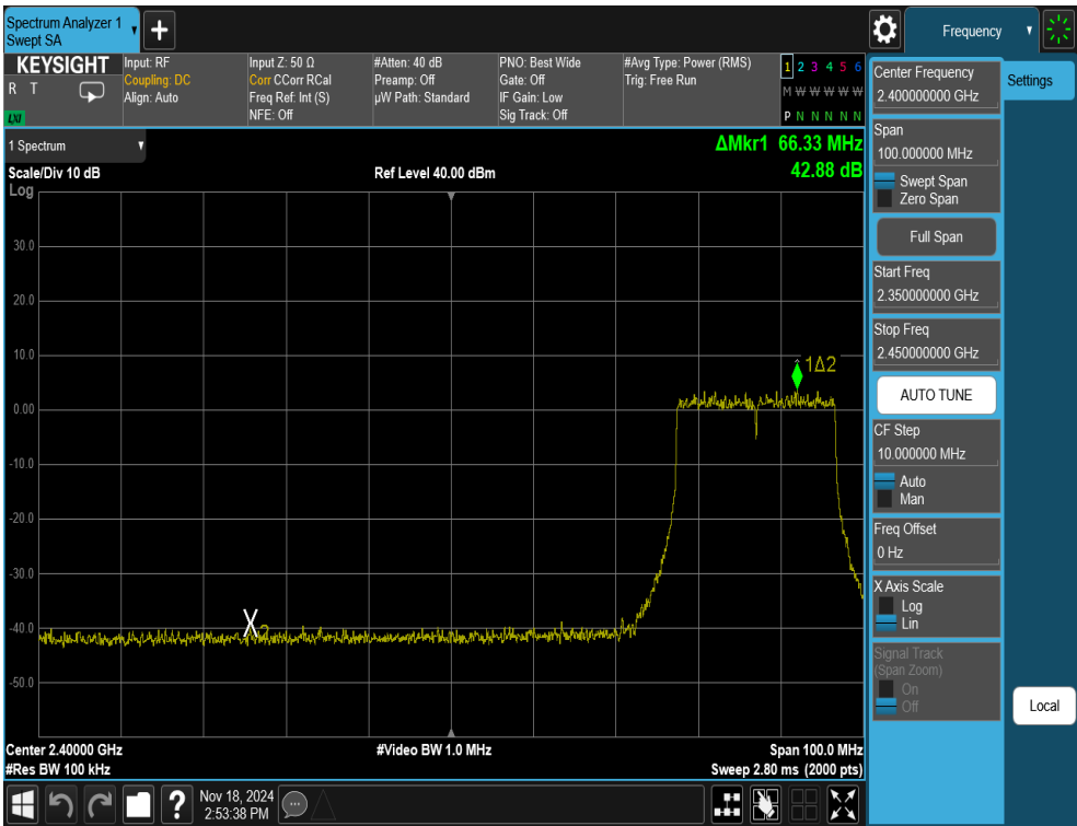
Plot 7-56. Band Edge Antenna WF7b (802.11ax OFDMA – RU242 – Ch. 6(Low Channel))
