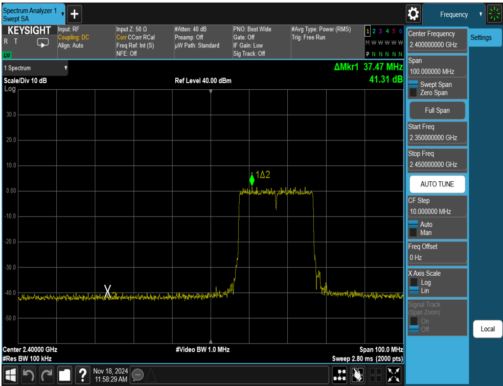
Plot 7-24. Band Edge Antenna WF8 (802.11ax OFDMA – RU242 – Ch. 2)
