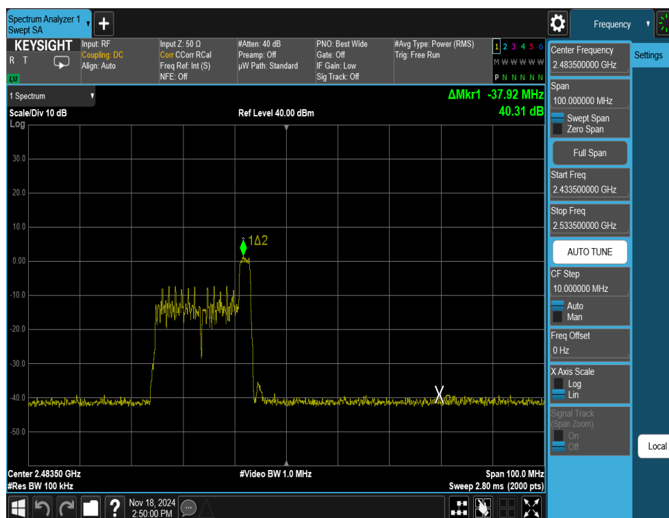
Plot 7-50. Band Edge Antenna WF7b (802.11ax OFDMA – RU26 Index 8 – Ch. 12)
