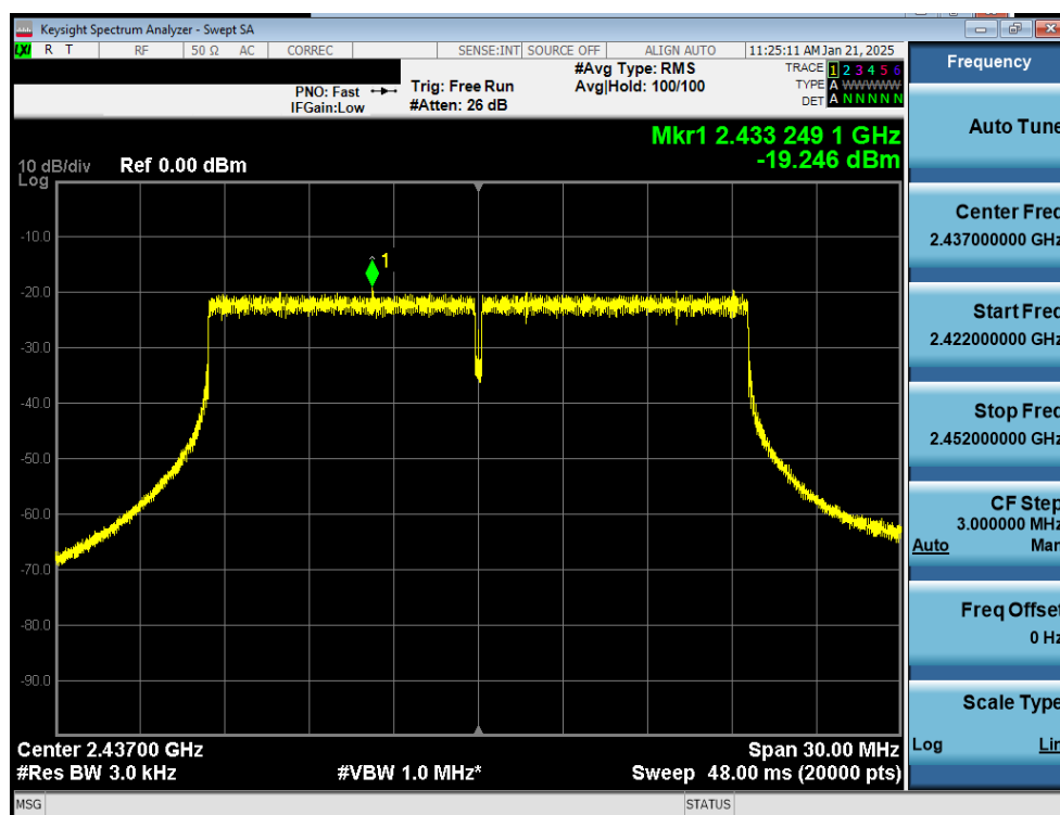
Plot 7-16. Power Spectral Density Plot Antenna WF7b (802.11ax OFDMA – RU242 – Ch. 6)
