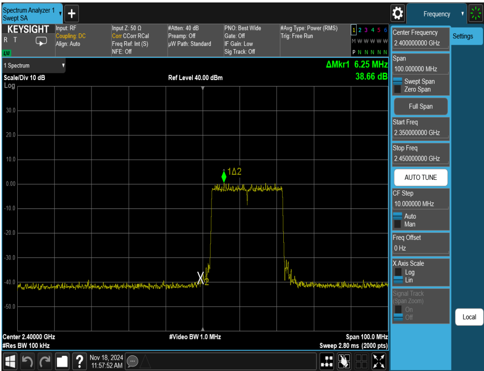
Plot 7-23. Band Edge Antenna WF8 (802.11ax OFDMA – RU242 – Ch. 1)
