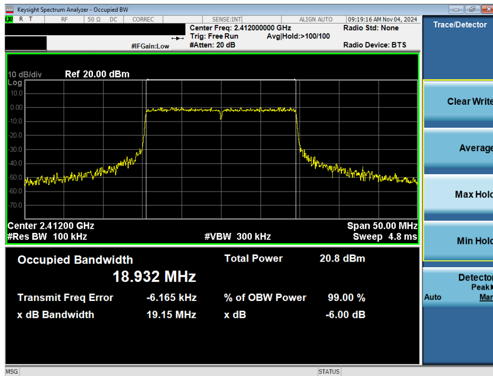
Plot 7-2. 6dB BW & 99% OBW Plot Antenna WF8 (802.11ax OFDMA – RU242 – Ch. 1)
