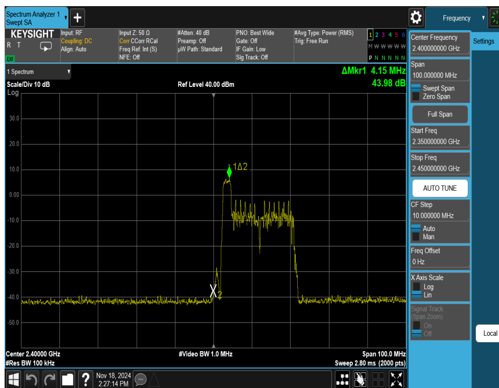
Plot 7-49. Band Edge Antenna WF7b (802.11ax OFDMA – RU26 Index 0 – Ch. 1)
