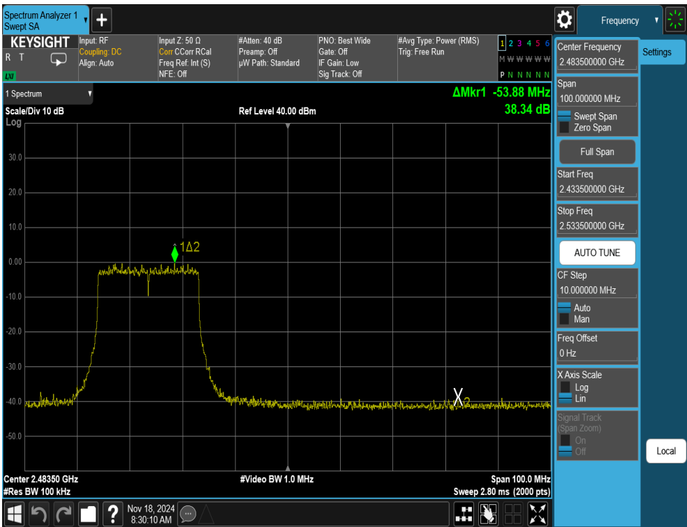
Plot 7-46. Band Edge Antenna WF8 (Common) (802.11ax OFDMA – RU242 – Ch. 10)
