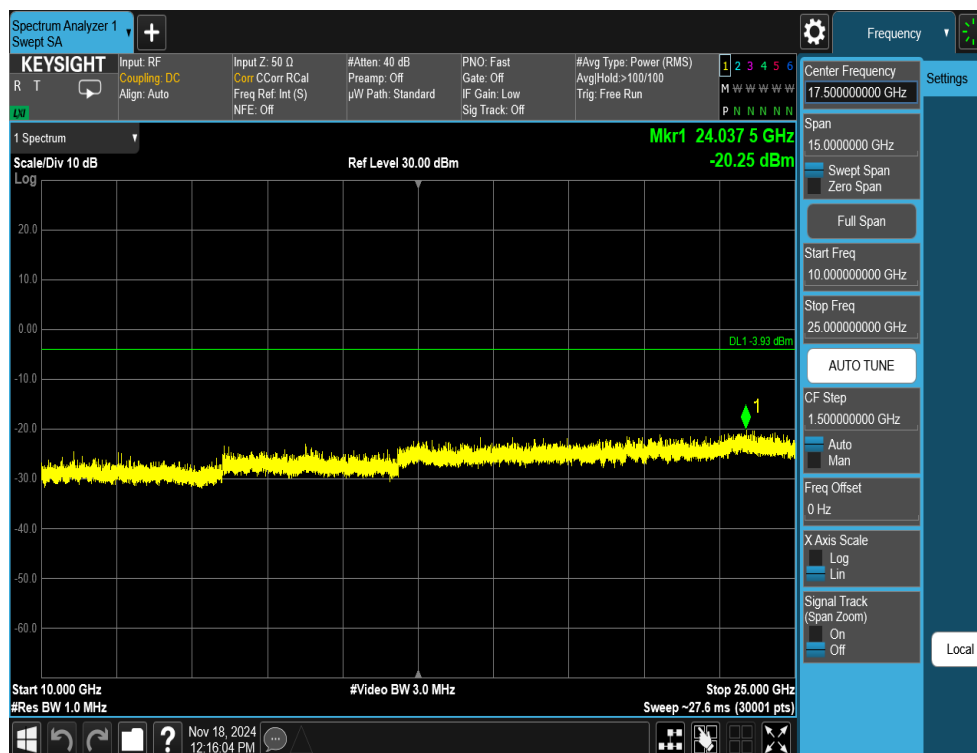
Plot 7-67. Conducted Spurious Plot Antenna WF8 (802.11ax OFDMA – RU26 – Ch. 11)
