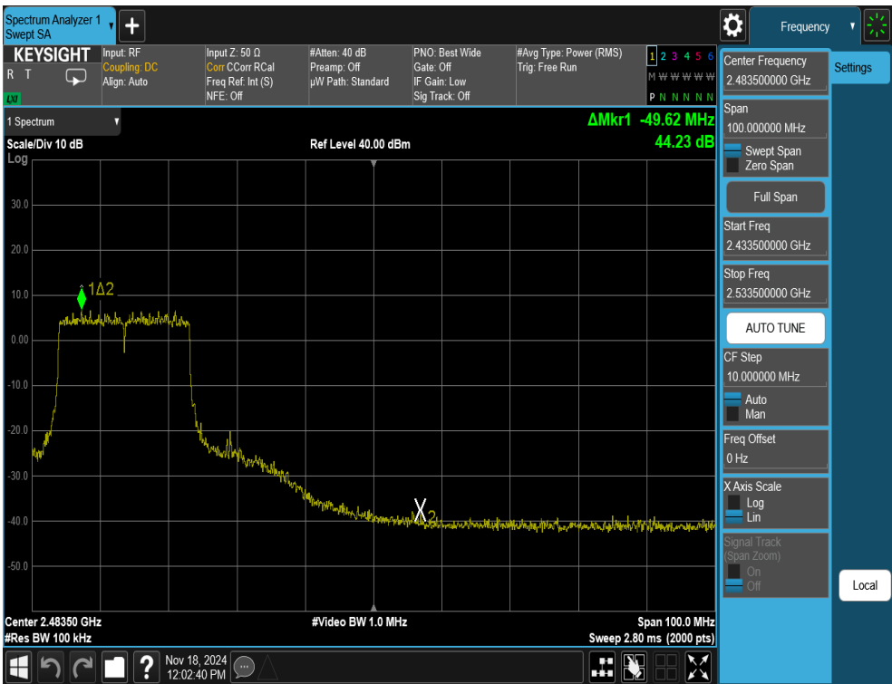
Plot 7-29. Band Edge Antenna WF8 (802.11ax OFDMA – RU242 – Ch. 8)
