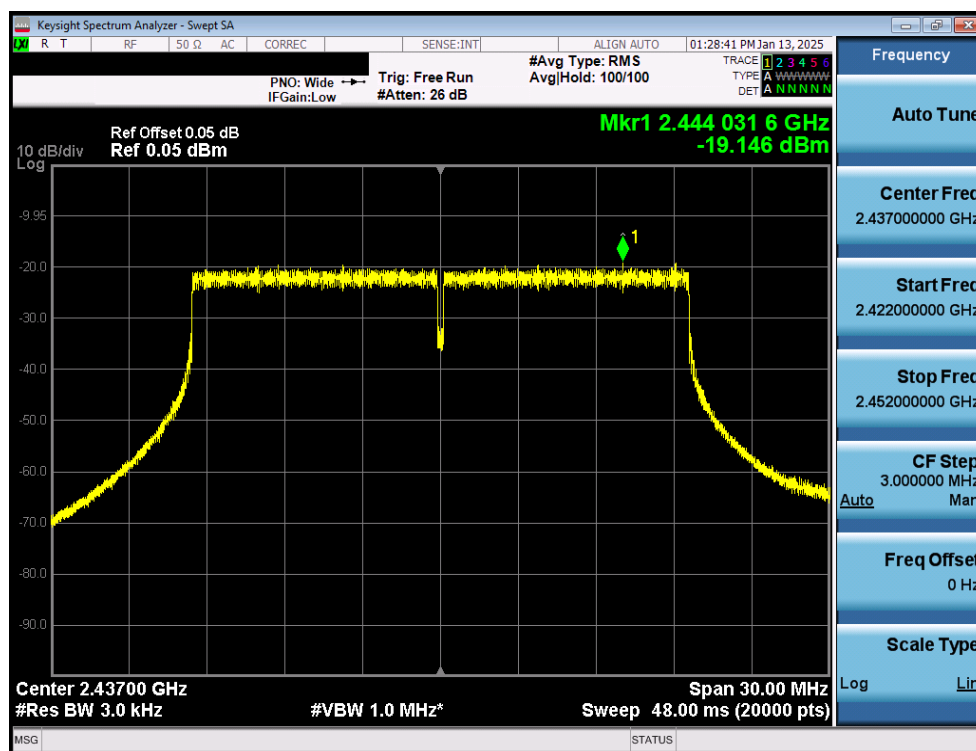
Plot 7-15. Power Spectral Density Plot Antenna WF8 (802.11ax OFDMA – RU242 – Ch. 6)
