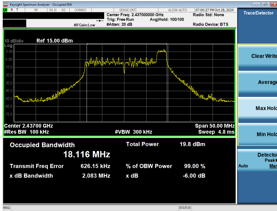
Plot 7-3. 6dB BW & 99% OBW Plot Antenna WF8 (Common) (802.11ax OFDMA – RU26 – Ch. 6)
