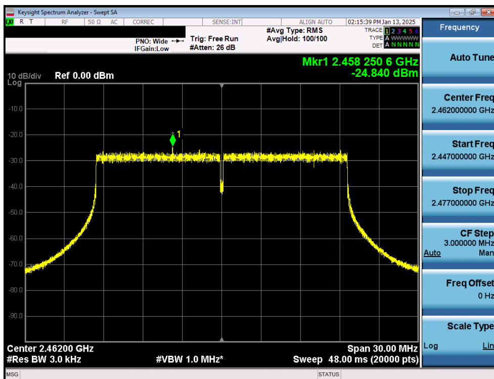
Plot 7-10. Power Spectral Density Plot Antenna WF8 (Common) (802.11ax OFDMA – RU242 – Ch. 11)
