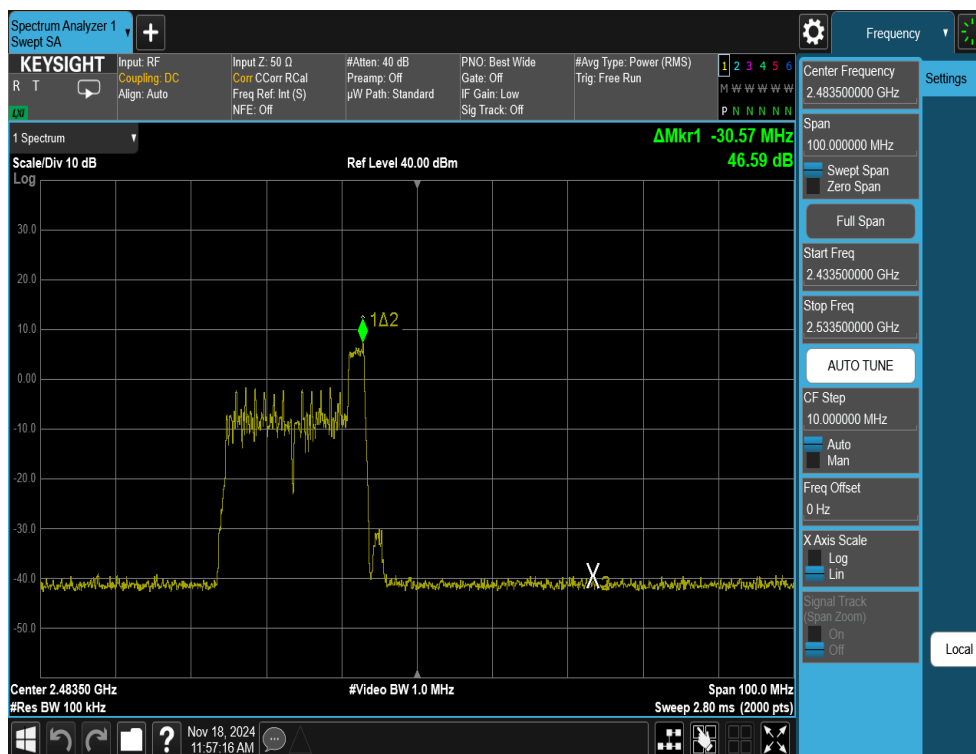
Plot 7-22. Band Edge Antenna WF8 (802.11ax OFDMA – RU26 Index 8 – Ch. 12)
