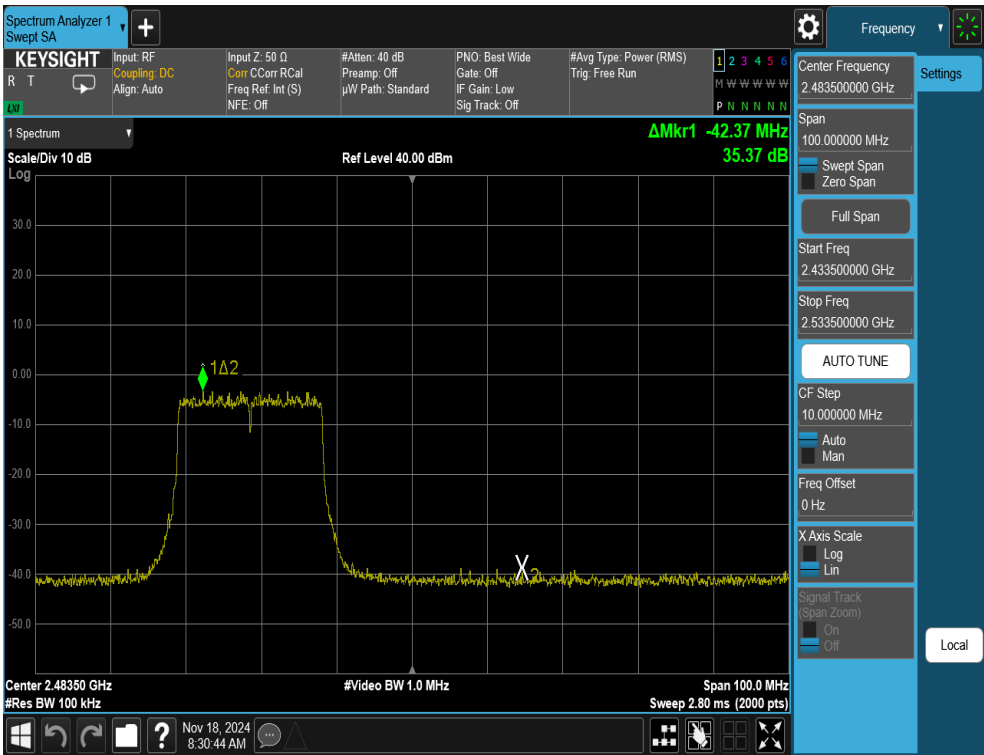
Plot 7-47. Band Edge Antenna WF8 (Common) (802.11ax OFDMA – RU242 – Ch. 11)
