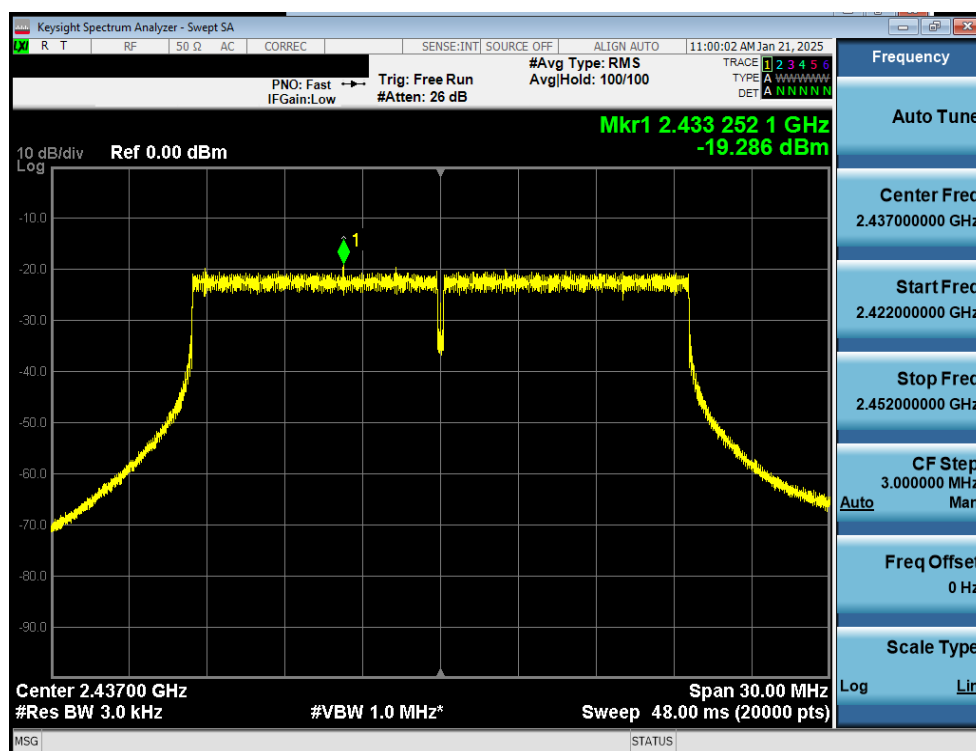
Plot 7-12. Power Spectral Density Plot Antenna WF7b (802.11ax OFDMA – RU242 – Ch. 6)
