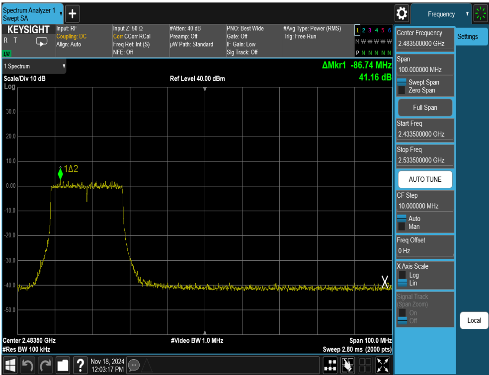
Plot 7-30. Band Edge Antenna WF8 (802.11ax OFDMA – RU242 – Ch. 9)
