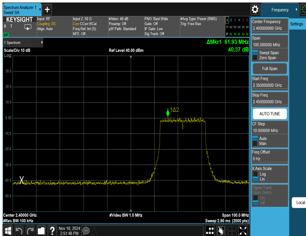
Plot 7-53. Band Edge Antenna WF7b (802.11ax OFDMA – RU242 – Ch. 3)
