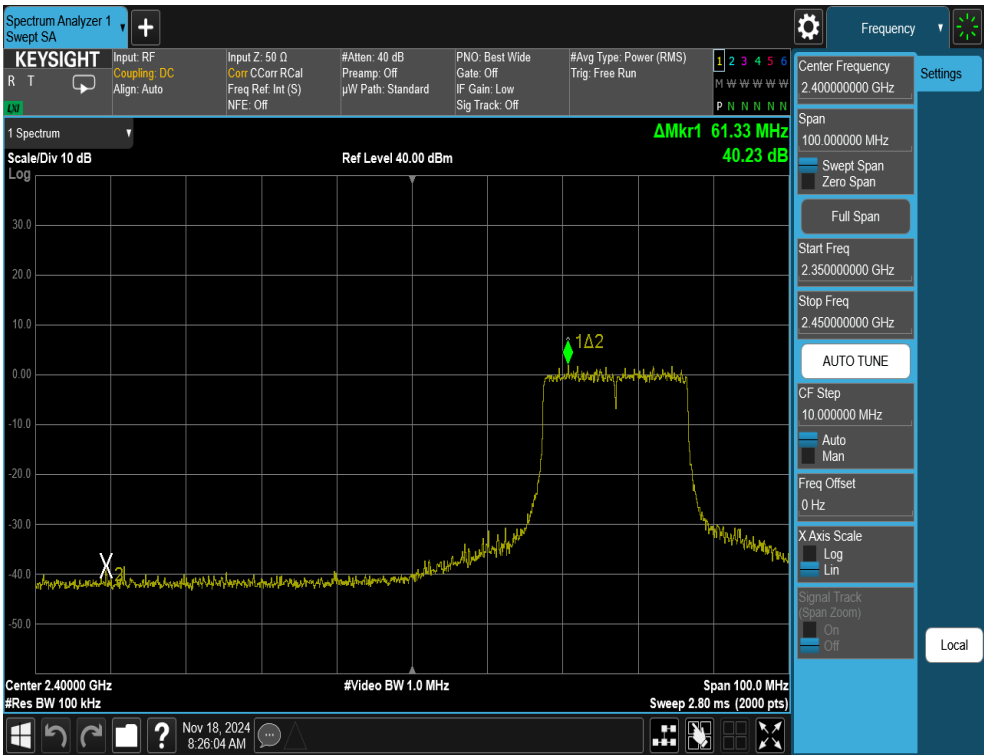
Plot 7-39. Band Edge Antenna WF8 (Common) (802.11ax OFDMA – RU242 – Ch. 4)
