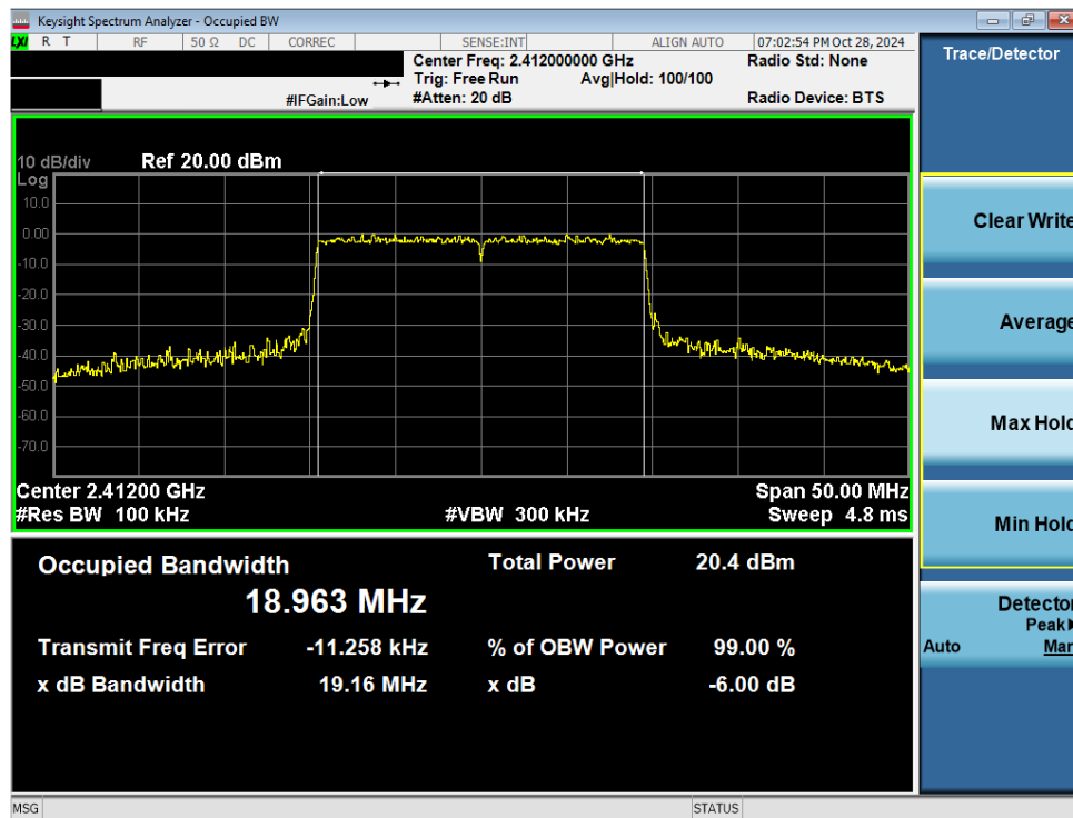
Plot 7-4. 6dB BW & 99% OBW Plot Antenna WF8 (Common) (802.11ax OFDMA – RU242 – Ch. 1)
