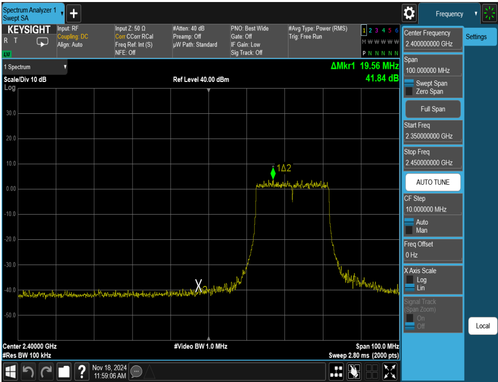
Plot 7-25. Band Edge Antenna WF8 (802.11ax OFDMA – RU242 – Ch. 3)
