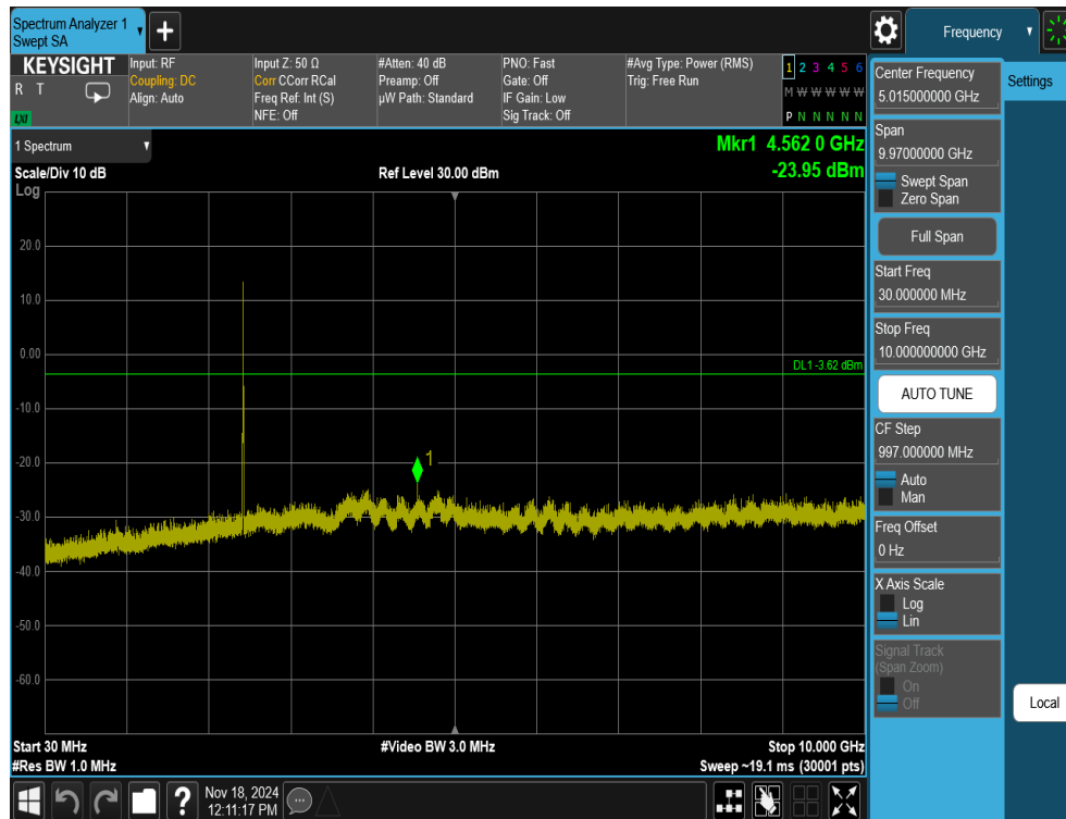
Plot 7-64. Conducted Spurious Plot Antenna WF8 (802.11ax OFDMA – RU26 – Ch. 6)
