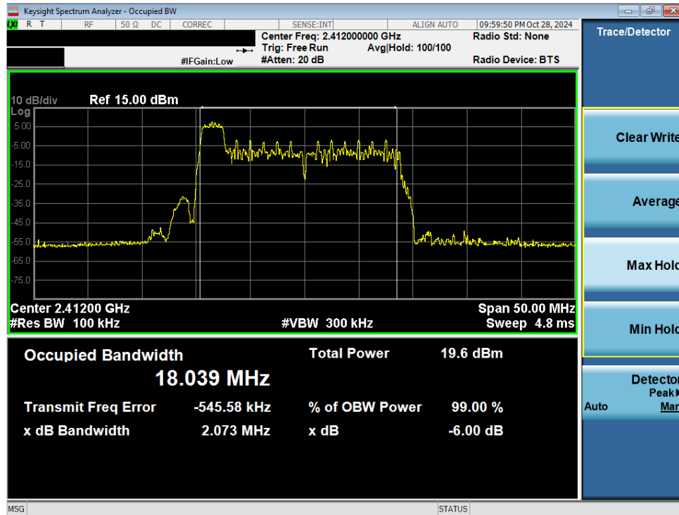
Plot 7-5. 6dB BW & 99% OBW Antenna WF7b (802.11ax OFDMA – RU26 – Ch. 1)
