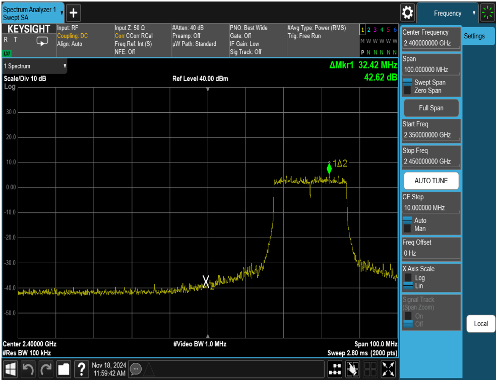
Plot 7-26. Band Edge Antenna WF8 (802.11ax OFDMA – RU242 – Ch. 4)
