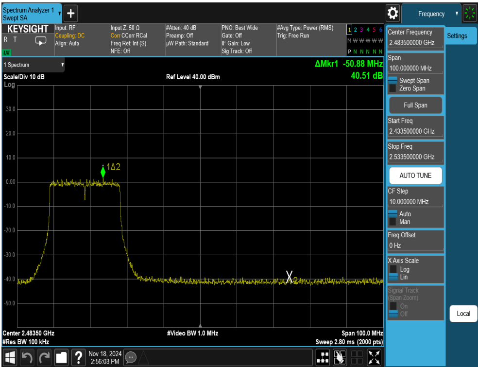
Plot 7-58. Band Edge Antenna WF7b (802.11ax OFDMA – RU242 – Ch. 9)
