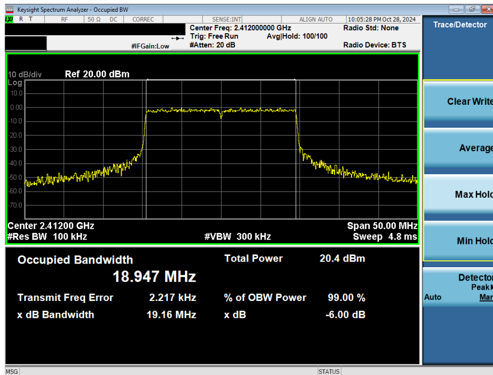
Plot 7-6. 6dB BW & 99% OBW Plot Antenna WF7b (802.11ax OFDMA – RU242 – Ch. 1)
