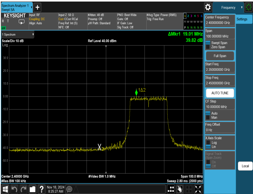
Plot 7-38. Band Edge Antenna WF8 (Common) (802.11ax OFDMA – RU242 – Ch. 3)
