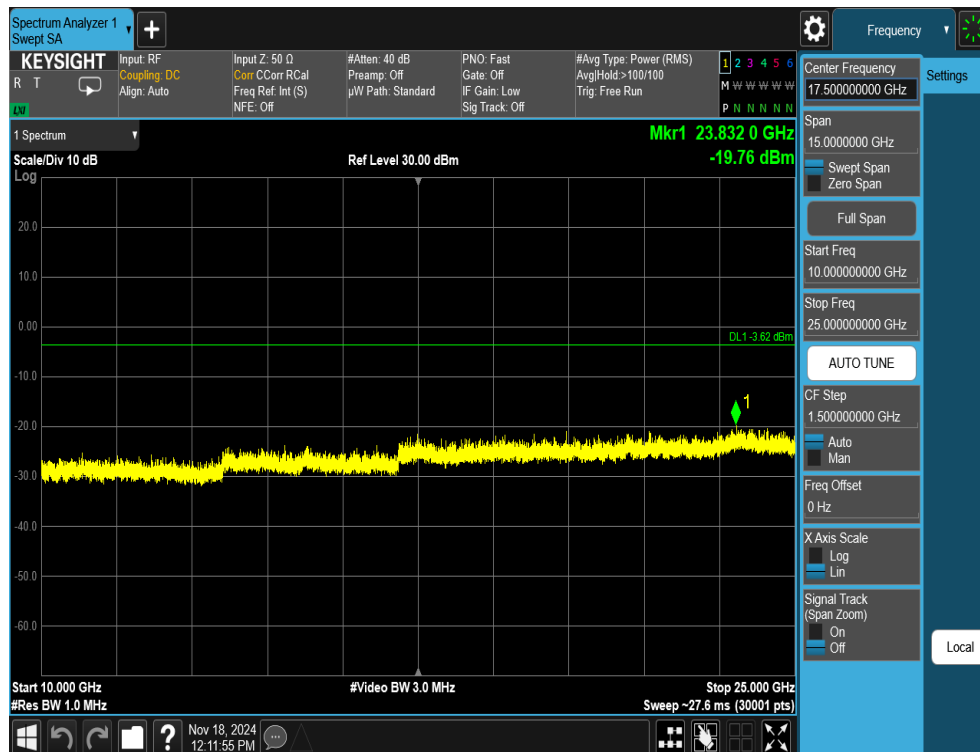
Plot 7-65. Conducted Spurious Plot Antenna WF8 (802.11ax OFDMA – RU26 – Ch. 6)
