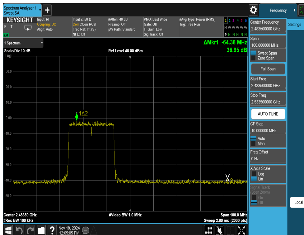
Plot 7-33. Band Edge Antenna WF8 (802.11ax OFDMA – RU242 – Ch. 12)
