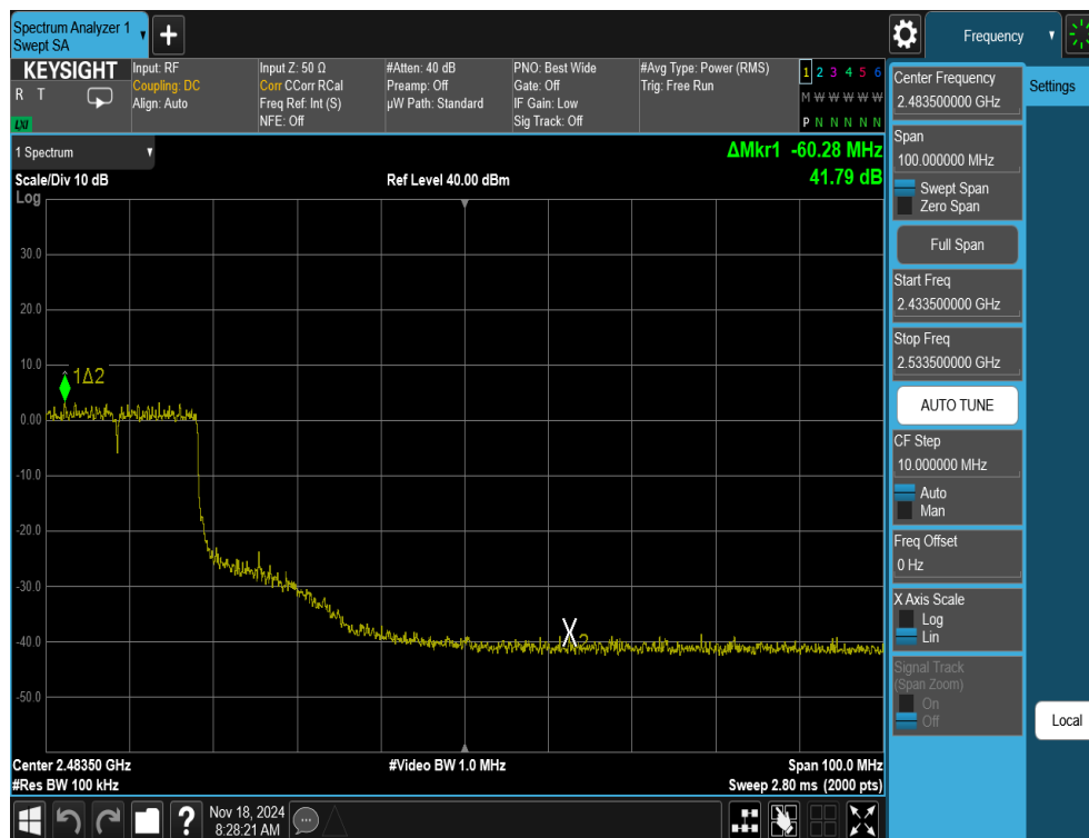
Plot 7-43. Band Edge Antenna WF8 (Common) (802.11ax OFDMA – RU242 – Ch. 7)
