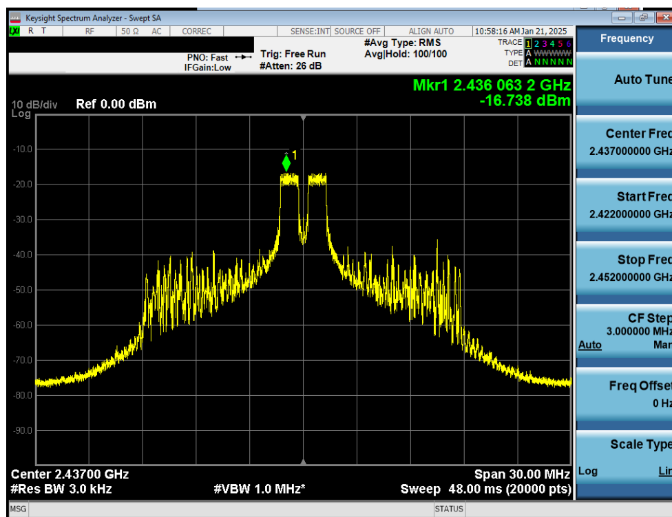
Plot 7-11. Power Spectral Density Plot Antenna WF7b (802.11ax OFDMA – RU26 – Ch. 6)
