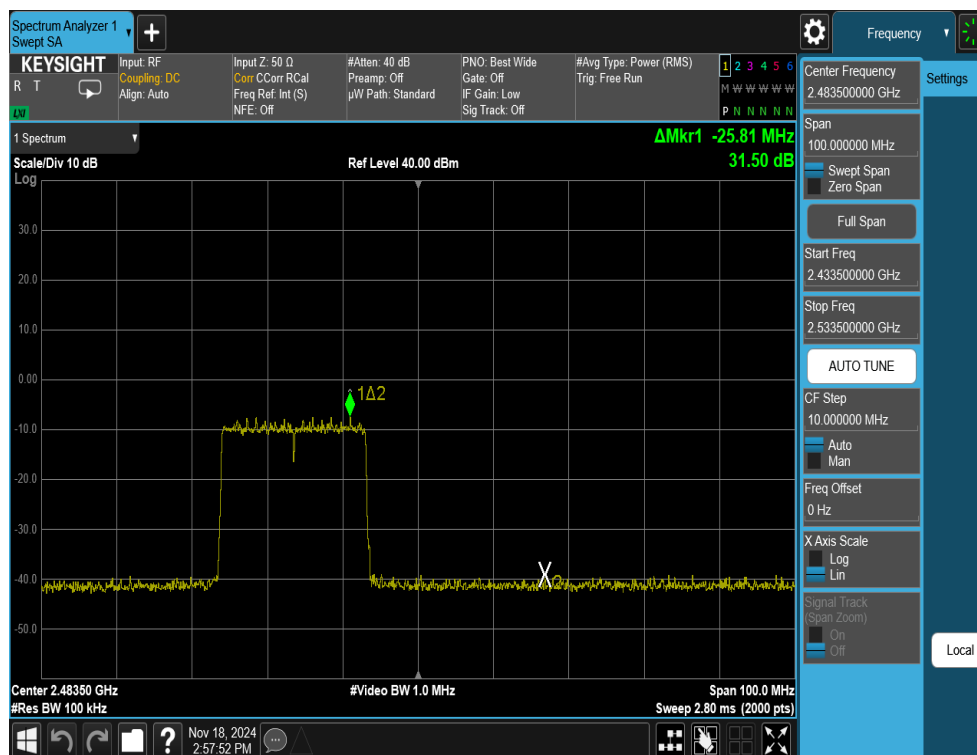
Plot 7-61. Band Edge Antenna WF7b (802.11ax OFDMA – RU242 – Ch. 12)
