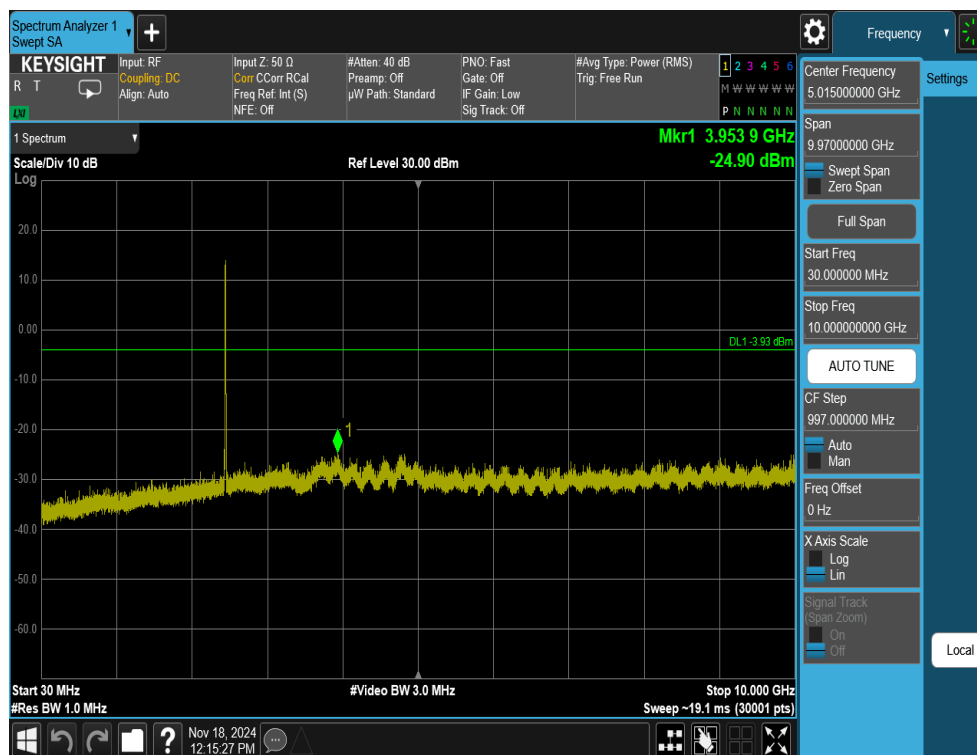
Plot 7-66. Conducted Spurious Plot Antenna WF8 (802.11ax OFDMA – RU26 – Ch. 11)
