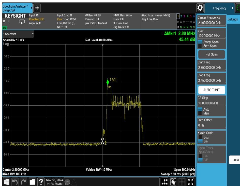
Plot 7-21. Band Edge Antenna WF8 (802.11ax OFDMA – RU26 Index 0 – Ch. 1)
