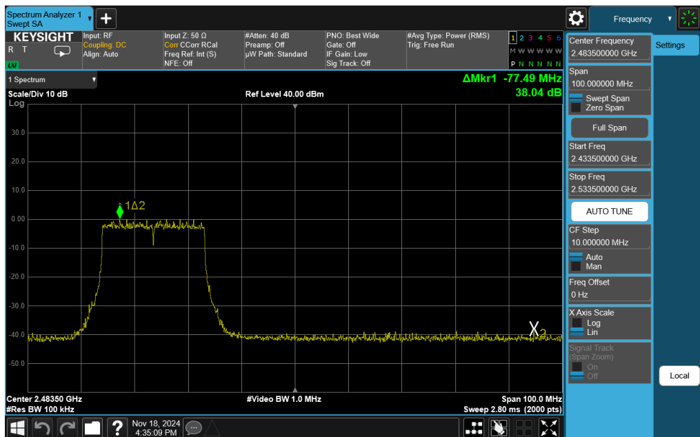
Plot 7-120. Band Edge Plot Antenna WF7b (802.11ax (SU - 2.4GHz) – Ch. 10)
