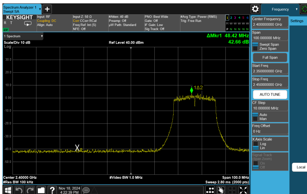
Plot 7-99. Band Edge Plot Antenna WF7b (802.11n (2.4GHz) – Ch. 4)
