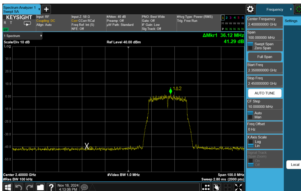
Plot 7-83. Band Edge Plot Antenna WF7b (802.11g – Ch. 2)
