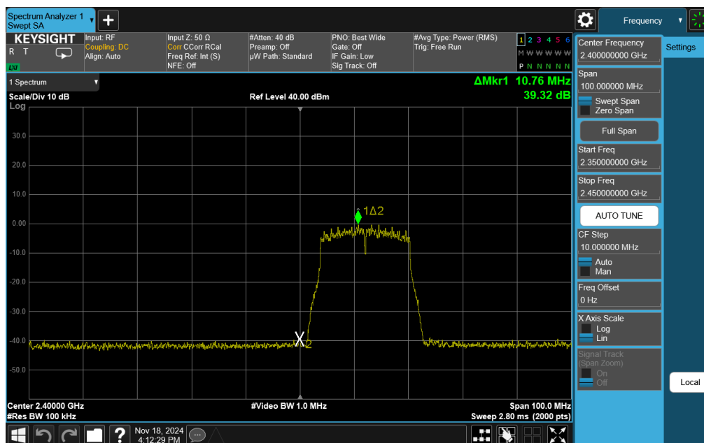
Plot 7-82. Band Edge Plot Antenna WF7b (802.11g – Ch. 1)
