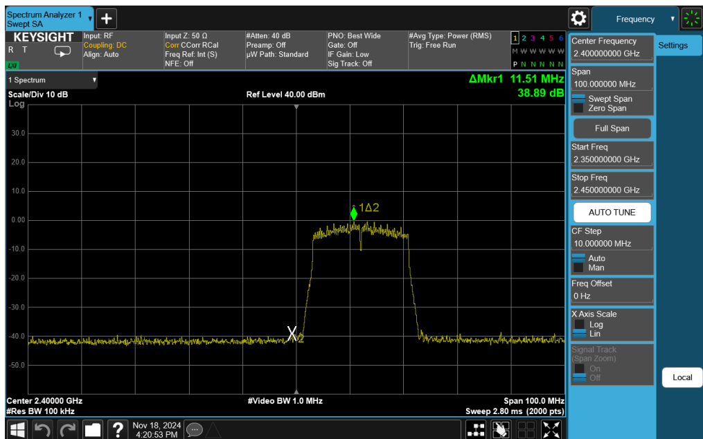
Plot 7-96. Band Edge Plot Antenna WF7b (802.11n (2.4GHz) – Ch. 1)
