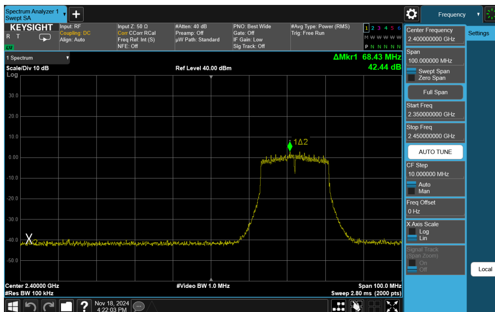
Plot 7-98. Band Edge Plot Antenna WF7b (802.11n (2.4GHz) – Ch. 3)
