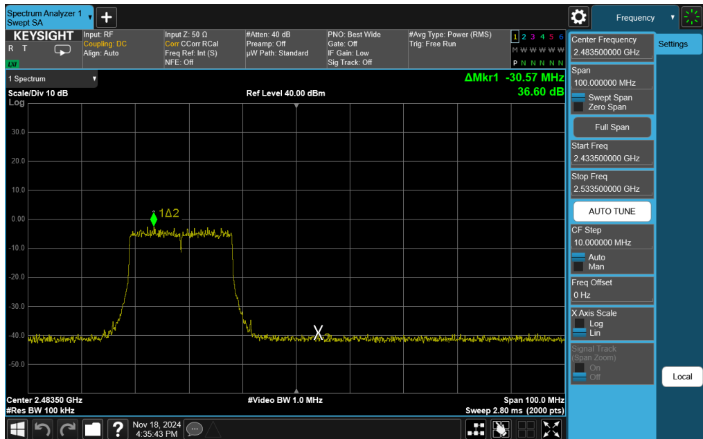
Plot 7-121. Band Edge Plot Antenna WF7b (802.11ax (SU - 2.4GHz) – Ch. 11)
