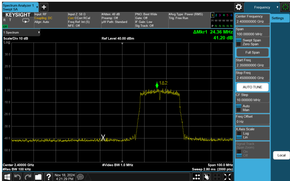
Plot 7-97. Band Edge Plot Antenna WF7b (802.11n (2.4GHz) – Ch. 2)
