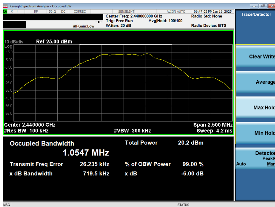
Plot 7-20. 6dB BW & 99% OBW Plot Antenna WF7b (Bluetooth (LE), 1Mbps, iPA – Ch. 19)
