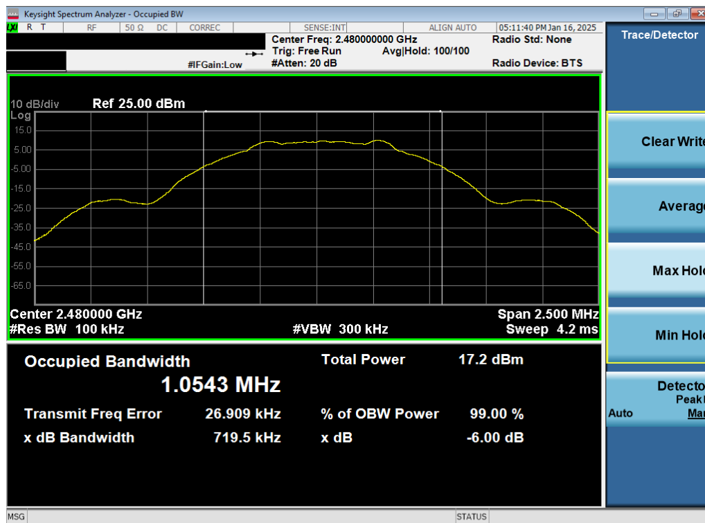
Plot 7-3. 6dB BW & 99% OBW Plot Antenna WF8 (Bluetooth (LE), 1Mbps, iPA – Ch. 39)
