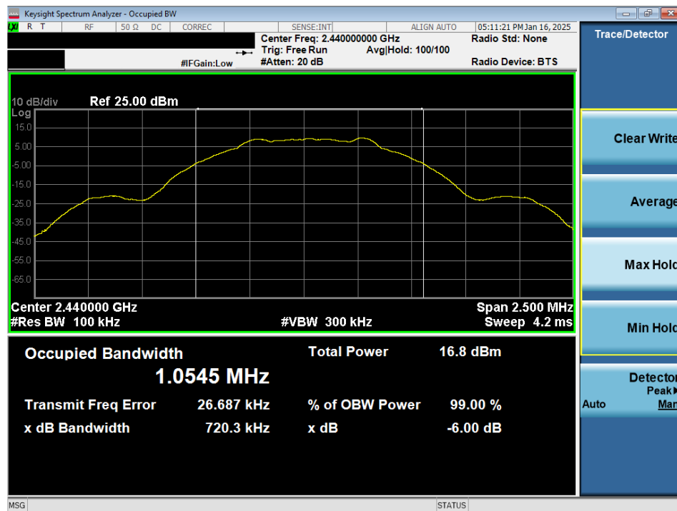
Plot 7-2. 6dB BW & 99% OBW Plot Antenna WF8 (Bluetooth (LE), 1Mbps, iPA – Ch. 19)
