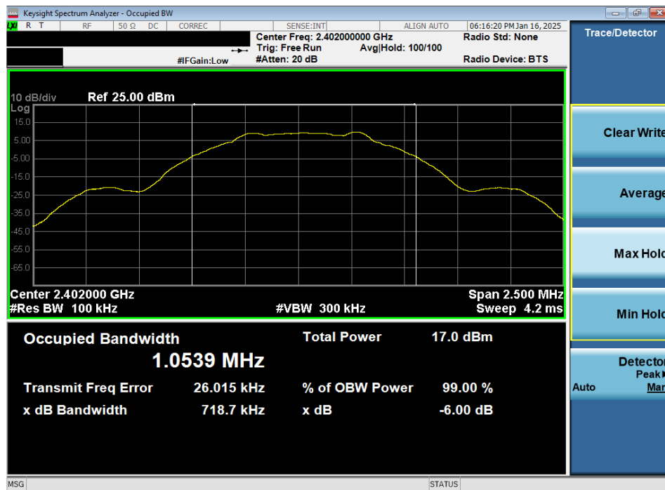
Plot 7-13. 6dB BW & 99% OBW Plot Antenna WF7b (Bluetooth (LE), 1Mbps, iPA – Ch. 0)
