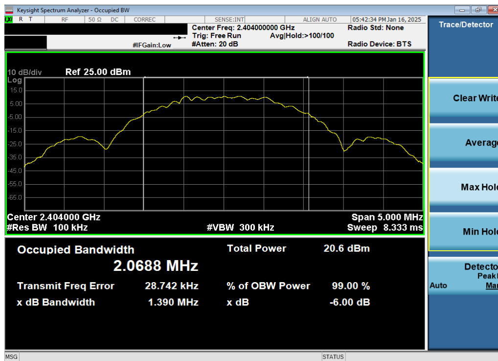
Plot 7-10. 6dB BW & 99% OBW Plot Antenna WF8 (Bluetooth (LE), 2Mbps, iPA – Ch. 1)
