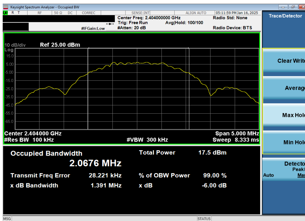
Plot 7-4. 6dB BW & 99% OBW Plot Antenna WF8 (Bluetooth (LE), 2Mbps, iPA – Ch. 1)
