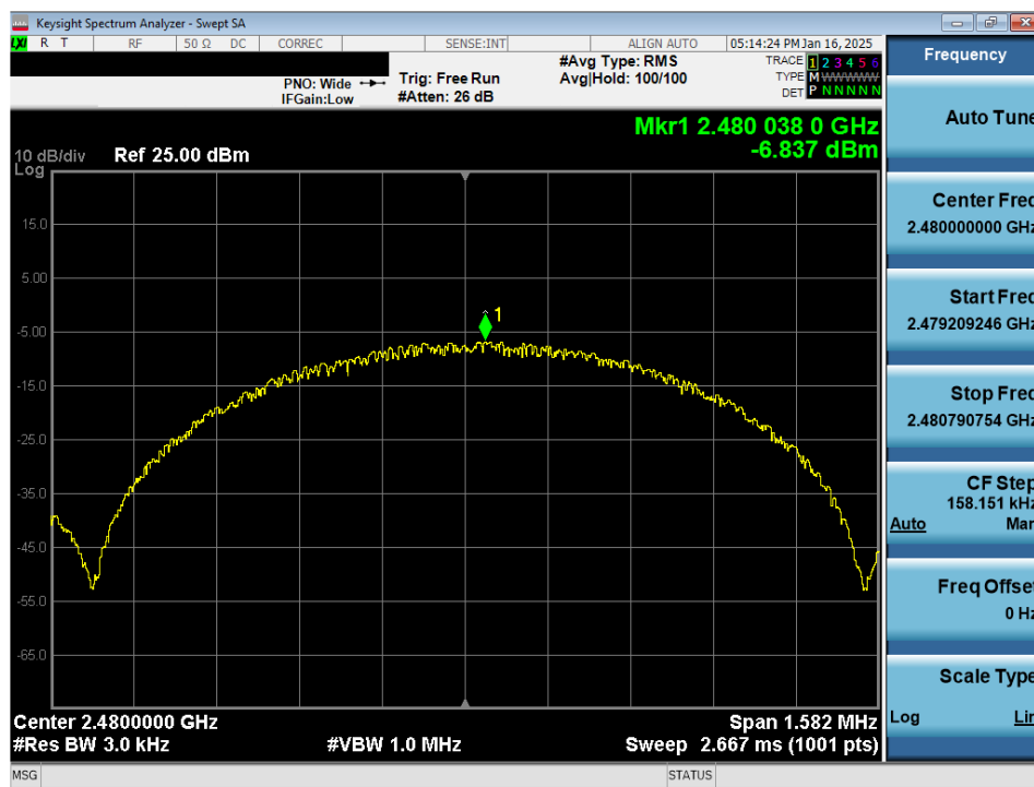
Plot 7-27. Power Spectral Density Plot Antenna WF8 (Common) (Bluetooth (LE), 1Mbps, iPA – Ch. 39)
