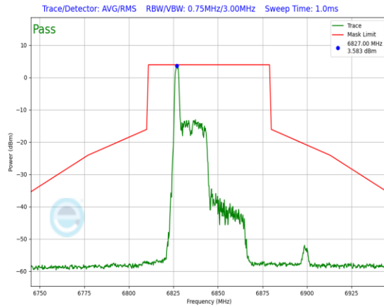
Plot 7-690. In-Band Emission Plot Antenna 1b (40MHz 802.11ax RU26 (UNII Band 7) – Ch. 179)
