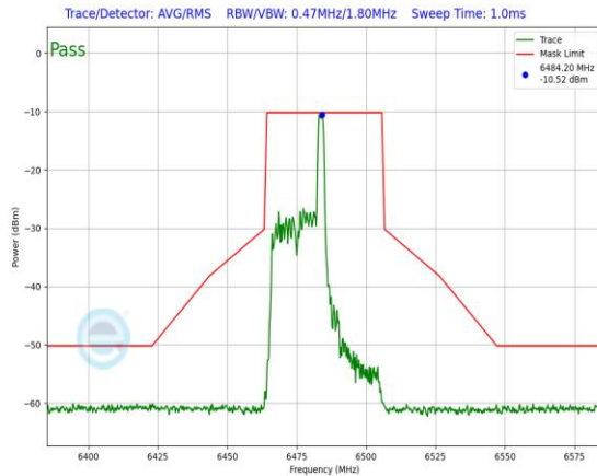
Plot 7-650. In-Band Emission Plot Antenna 3b (40MHz 802.11ax RU26 (UNII Band 6) – Ch. 107)
