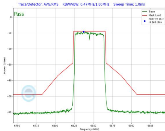
Plot 7-662. In-Band Emission Plot Antenna 3b (40MHz 802.11ax RU484 (UNII Band 7) – Ch. 179)
