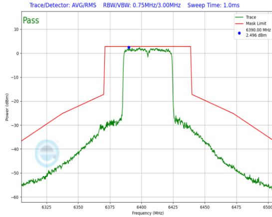
Plot 7-678. In-Band Emission Plot Antenna 1b (40MHz 802.11ax RU484 (UNII Band 5) – Ch. 91)
