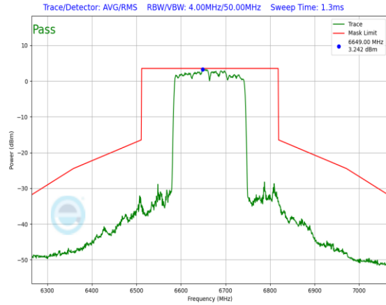
Plot 7-584. In-Band Emission Plot Antenna 5T (160MHz 802.11ax RU996x2 (UNII Band 7) – Ch. 143)
