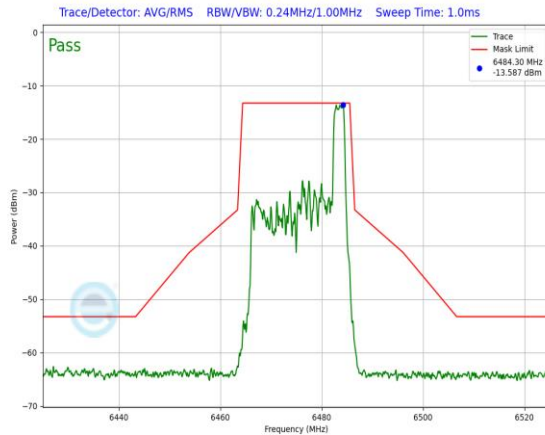
Plot 7-649. In-Band Emission Plot Antenna 3b (20MHz 802.11ax RU26 (UNII Band 6) – Ch. 105)
