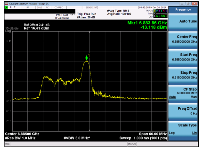
Plot 7-548. PSD Plot SDM Diversity Antenna 1b (40MHz 802.11ax RU26 (UNII Band 8) – Ch. 187)
