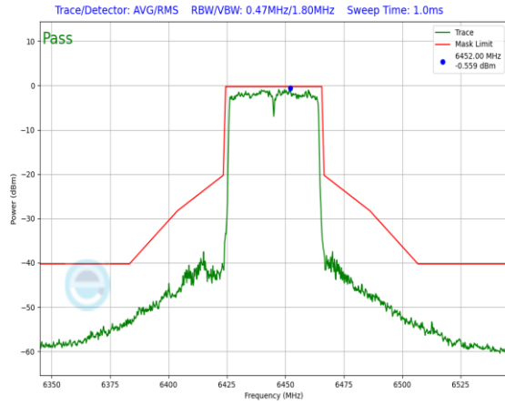
Plot 7-574. In-Band Emission Plot Antenna 5T (40MHz 802.11ax RU484 (UNII Band 6) – Ch. 99)
